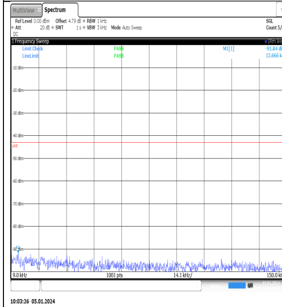
NTNV_N77-3700- 3980_PC2_30_10_H_TID7_NS_01_0.009_0.15_#1
