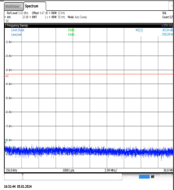
NTNV_N77-3700- 3980_PC2_30_10_M_TID12_NS_01_0.15_30_#1
