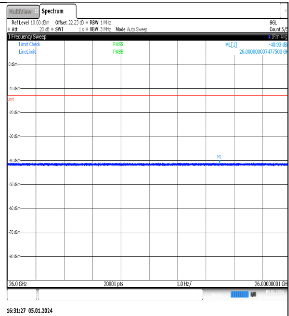
NTNV_N77-3700- 3980_PC2_30_10_M_TID11_NS_01_26000_4000 0_#1
