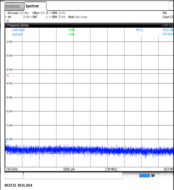
NTNV_N77-3700- 3980_PC2_30_10_H_TID5_NS_01_0.15_30_#1
