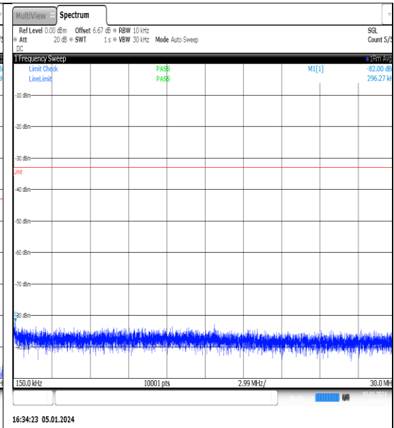
NTNV_N77-3700- 3980_PC2_30_10_M_TID15_NS_01_0.15_30_#1
