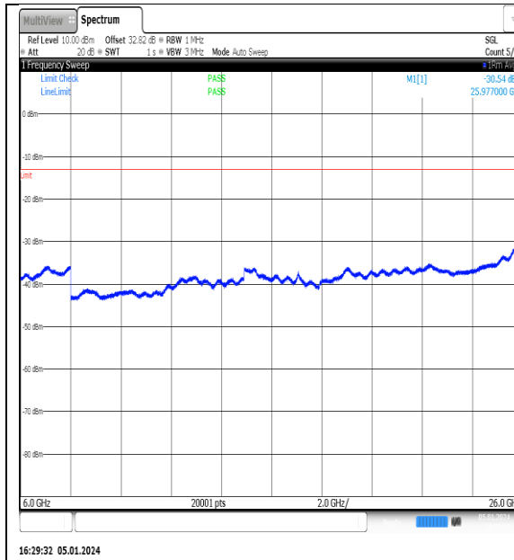
NTNV_N77-3700- 3980_PC2_30_10_M_TID9_NS_01_6000_26000_#1
