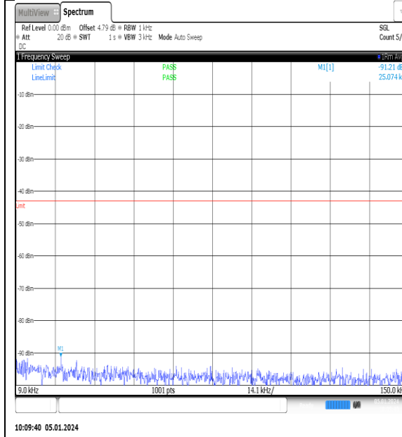
NTNV_N77-3700- 3980_PC2_30_10_H_TID9_NS_01_0.009_0.15_#1
