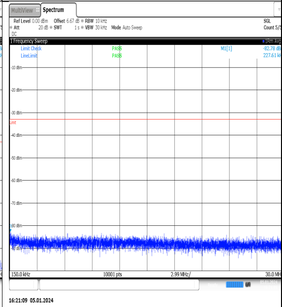
NTNV_N77-3700- 3980_PC2_30_10_L_TID15_NS_01_0.15_30_#1
