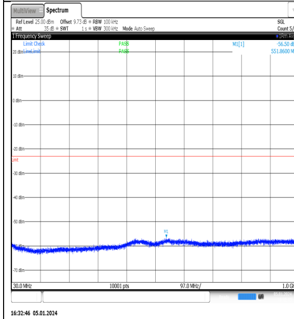
NTN_V_N77-3700- 3980_PC2_30_10_M_TID13_NS_01_30_1000_#1
