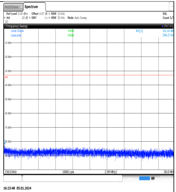
NTNV_N77-3700- 3980_PC2_30_10_M_TID3_NS_01_0.15_30_#1
