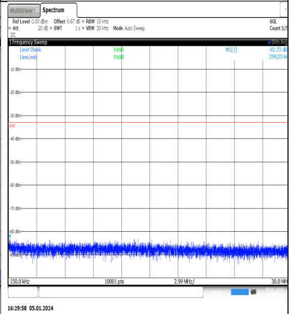
NTNV_N77-3700- 3980_PC2_30_10_M_TID10_NS_01_0.15_30_#1
