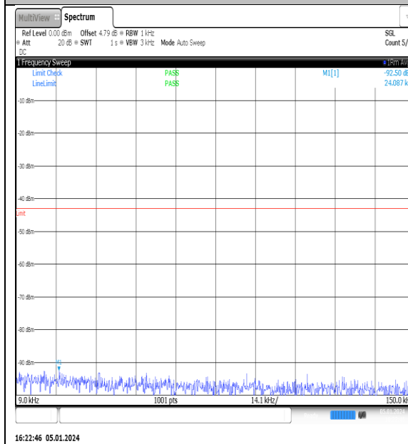
NTNV_N77-3700- 3980_PC2_30_10_M_TID2_NS_01_0.009_0.15_#1
