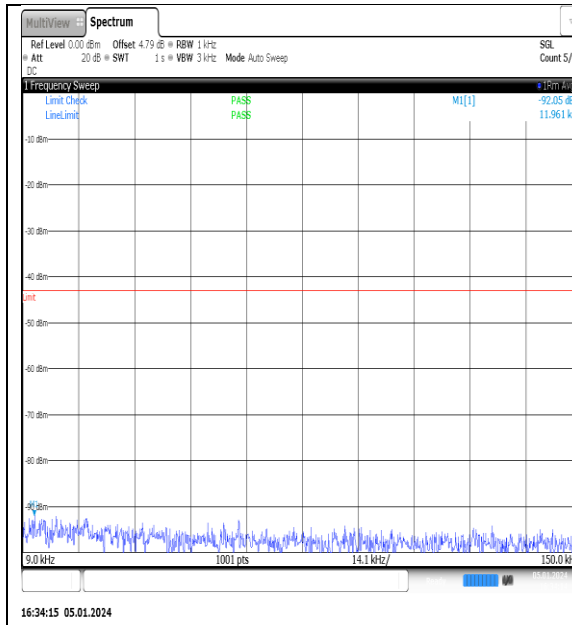
NTNV_N77-3700- 3980_PC2_30_10_M_TID15_NS_01_0.009_0.15_ #1
