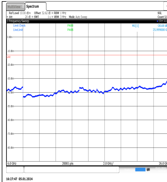
NTNV_N77-3700- 3980_PC2_30_10_M_TID7_NS_01_6000_26000_#1
