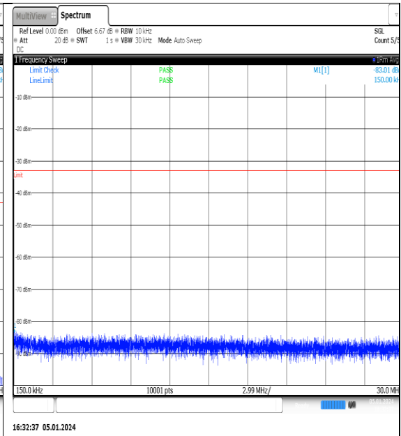
NTN_V_N77-3700- 3980_PC2_30_10_M_TID13_NS_01_0.15_30_#1
