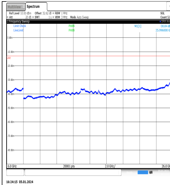
NTNV_N77-3700- 3980_PC2_30_10_M_TID3_NS_01_6000_26000_#1
