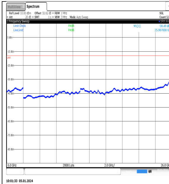
NTNV_N77-3700- 3980_PC2_30_10_H_TID6_NS_01_6000_26000_#1
