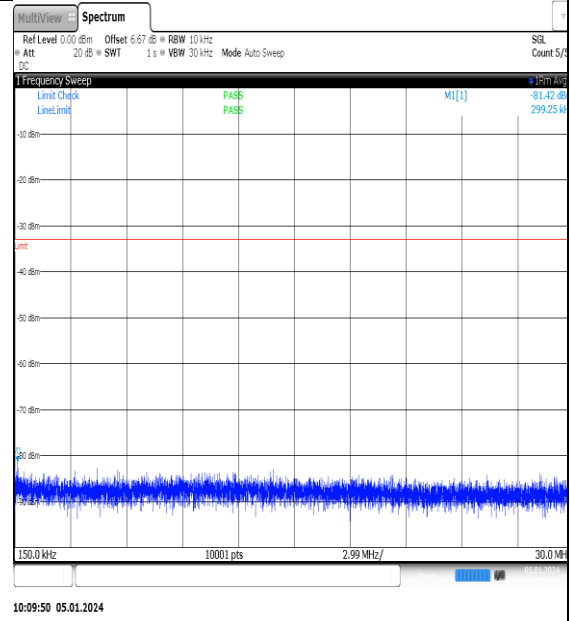
NTNV_N77-3700- 3980_PC2_30_10_H_TID9_NS_01_0.15_30_#1
