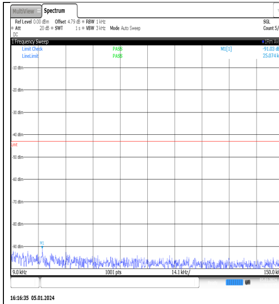
NTNV_N77-3700- 3980_PC2_30_10_L_TID10_NS_01_0.009_0.15_ #1
