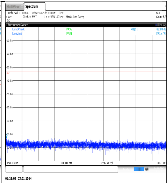
NTNV_N77-3450- 3550_PC2_30_100_M_TID14_NS_01_0.15_30_# 1
