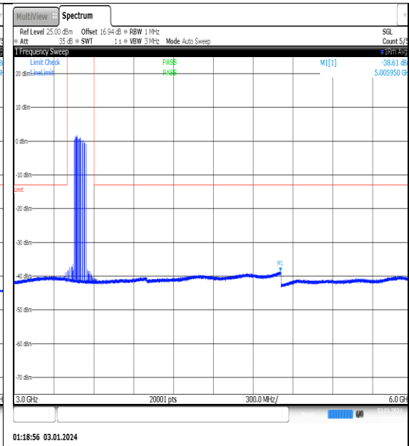
NTNV_N77-3450- 3550_PC2_30_100_M_TID13_NS_01_3000_6000 _#1
