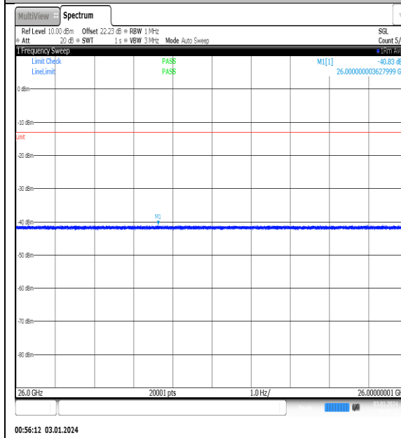
NTNV_N77-3450- 3550_PC2_30_100_M_TID6_NS_01_26000_4000_0_#1
