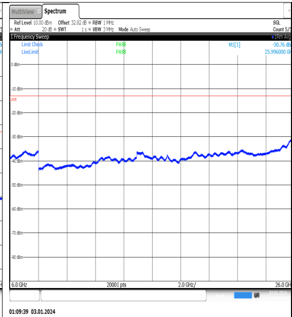
NTNV_N77-3450- 3550_PC2_30_100_M_TID10_NS_01_6000_2600 0_#1
