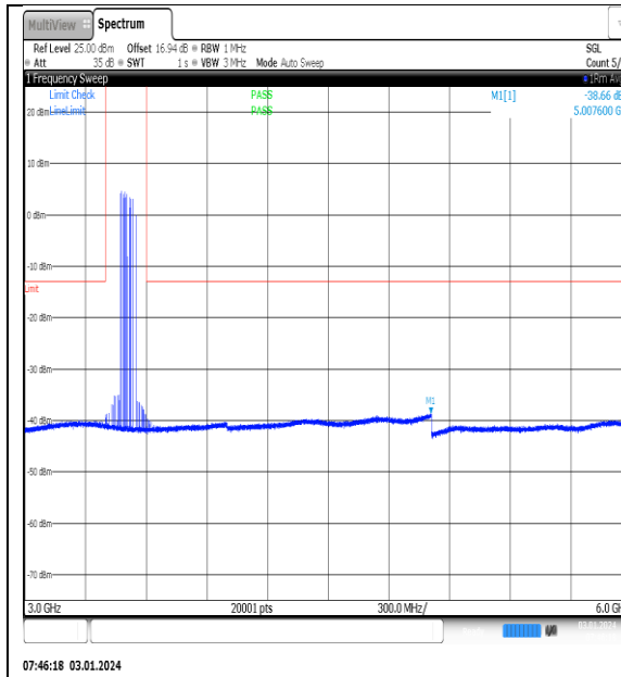
NTNV_N77-3450- 3550_PC2_30_80_H_TID10_NS_01_3000_6000_#1
