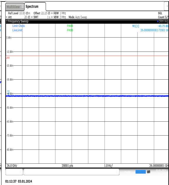
NTNV_N77-3450- 3550_PC2_30_100_M_TID11_NS_01_26000_400 _00_#1
