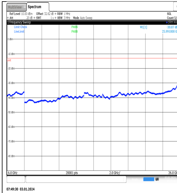
NTNV_N77-3450- 3550_PC2_30_80_H_TID13_NS_01_6000_26000 _#1
