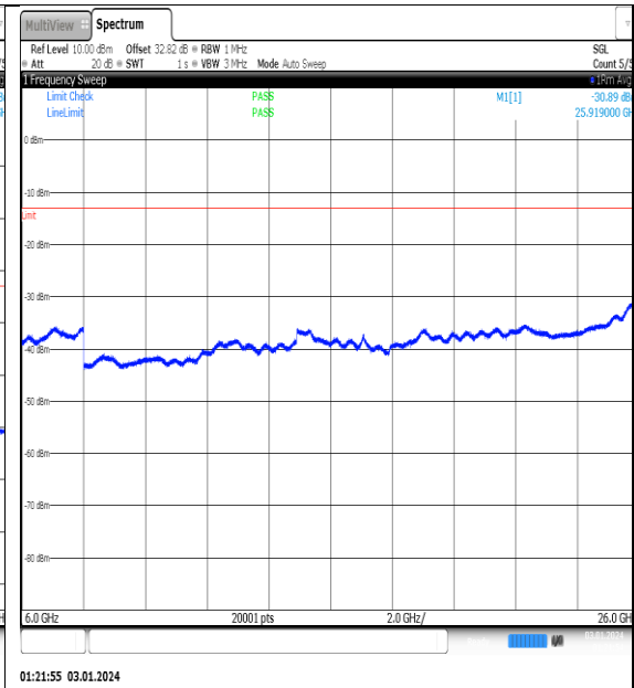
NTNV_N77-3450- 3550_PC2_30_100_M_TID14_NS_01_6000_2600 0_#1
