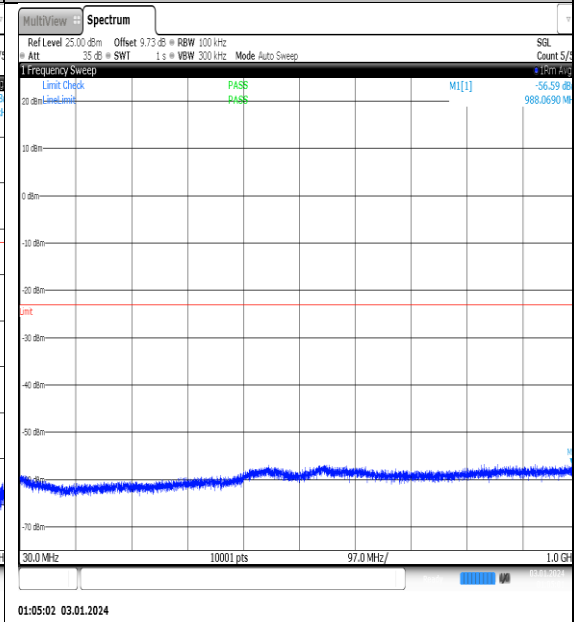
NTNV_N77-3450- 3550_PC2_30_100_M_TID9_NS_01_30_1000_#1
