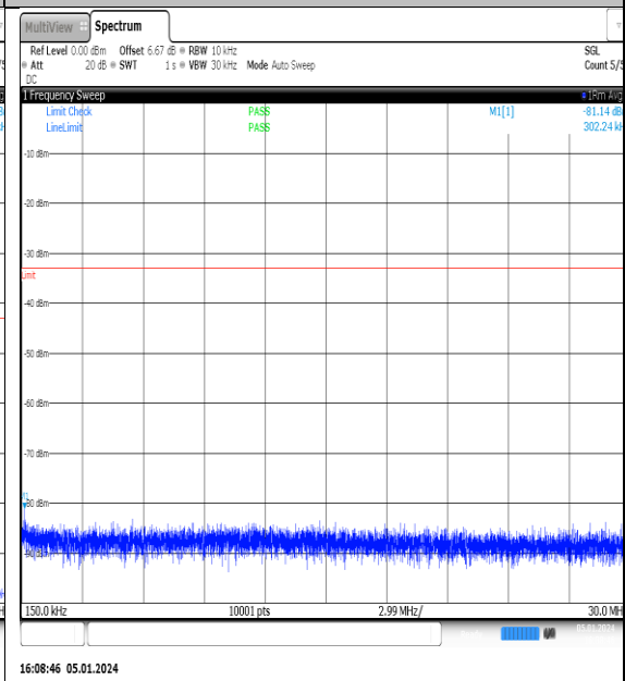
NTNV_N77-3700- 3980_PC2_30_10_L_TID1_NS_01_0.15_30_#1
