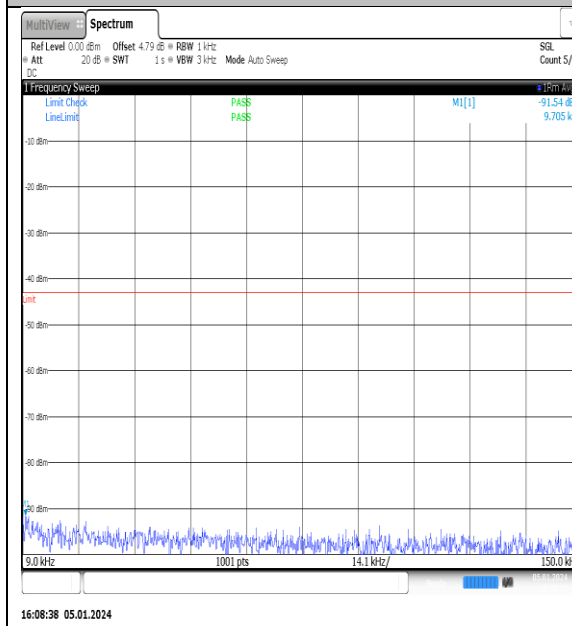
NTNV_N77-3700- 3980_PC2_30_10_L_TID1_NS_01_0.009_0.15_# 1
