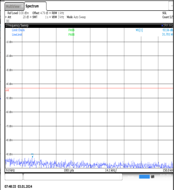
NTNV_N77-3450- 3550_PC2_30_80_H_TID13_NS_01_0.009_0.15_#1
