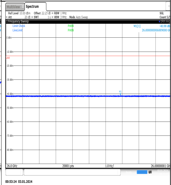
NTNV_N77-3450- 3550_PC2_30_100_M_TID5_NS_01_26000_4000_ 0_#1
