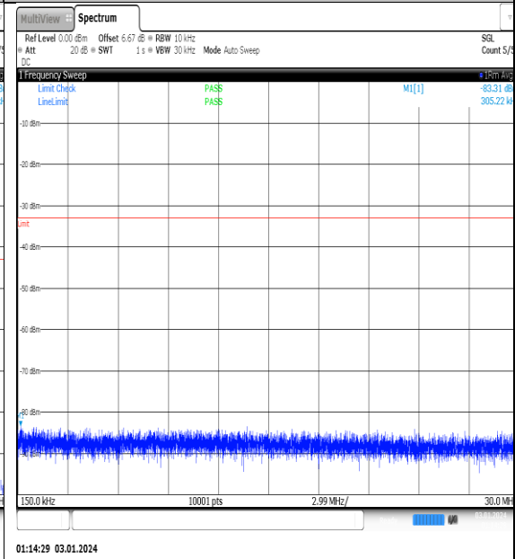
NTNV_N77-3450- 3550_PC2_30_100_M_TID12_NS_01_0.15_30_# _1
