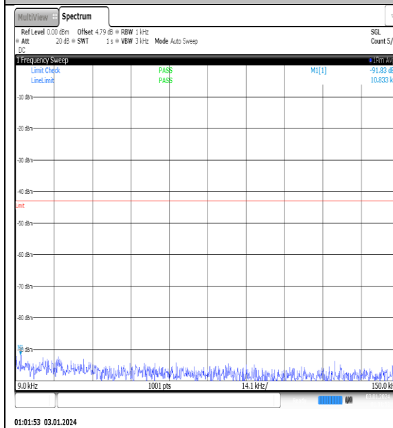
NTNV_N77-3450- 3550_PC2_30_100_M_TID8_NS_01_0.009_0.15_#1
