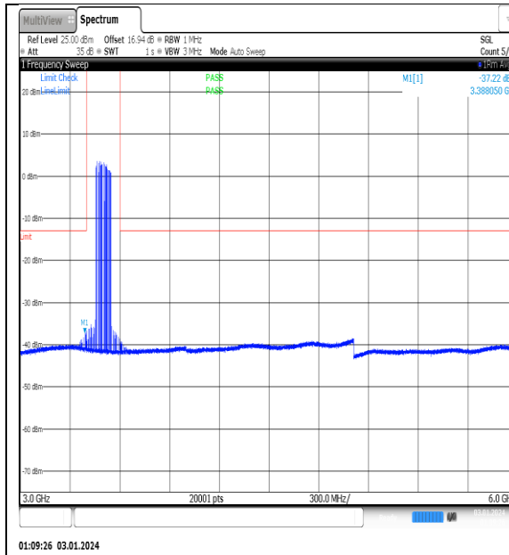
NTNV_N77-3450- 3550_PC2_30_100_M_TID10_NS_01_3000_6000 _#1
