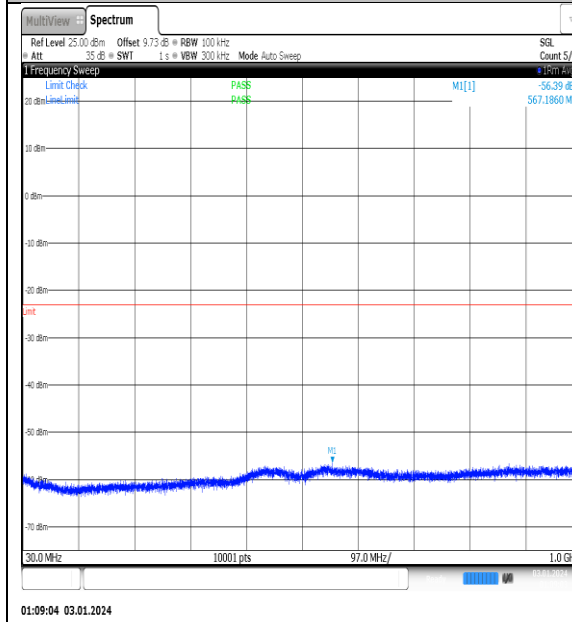
NTNV_N77-3450- 3550_PC2_30_100_M_TID10_NS_01_30_1000_# 1
