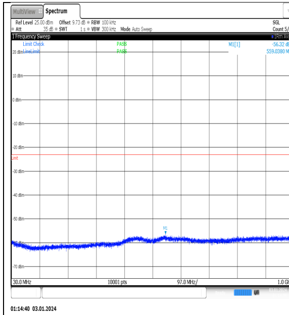
NTNV_N77-3450- 3550_PC2_30_100_M_TID12_NS_01_30_1000_# 1
