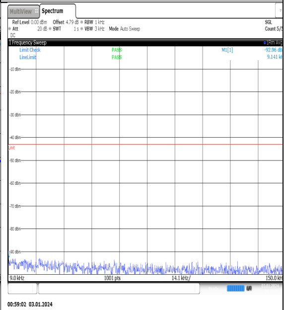
NTNV_N77-3450- 3550_PC2_30_100_M_TID7_NS_01_0.009_0.15_#1
