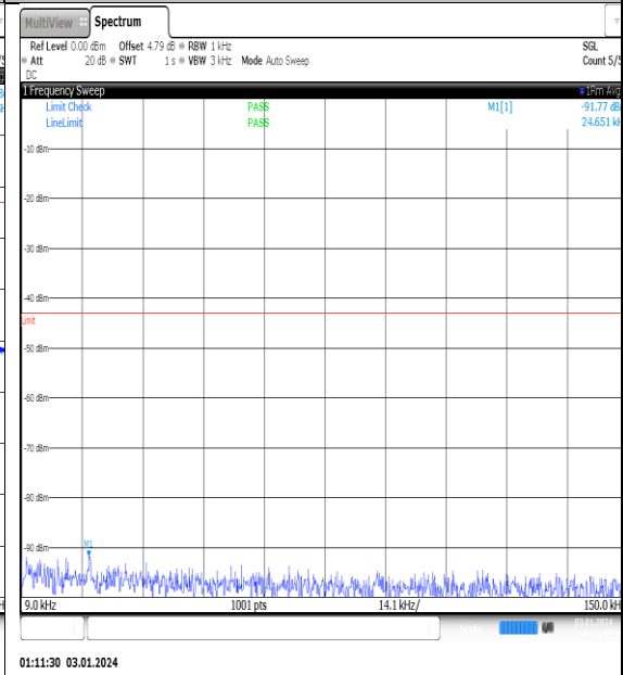
NTNV_N77-3450- 3550_PC2_30_100_M_TID11_NS_01_0.009_0.15 _#1
