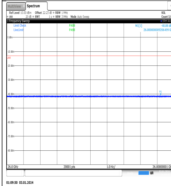
NTNV_N77-3450- 3550_PC2_30_100_M_TID10_NS_01_26000_400 00_#1
