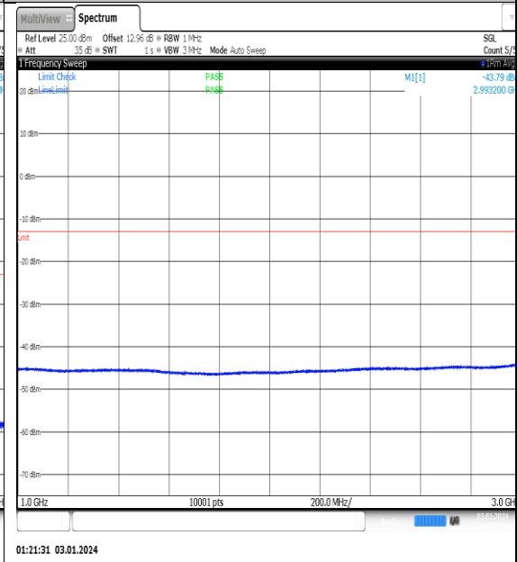
NTNV_N77-3450- 3550_PC2_30_100_M_TID14_NS_01_1000_3000 #1
