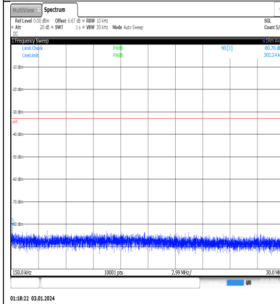
NTNV_N77-3450- 3550_PC2_30_100_M_TID13_NS_01_0.15_30_# 1
