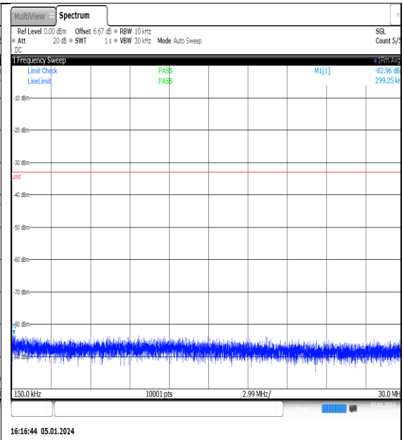
NTNV_N77-3700- 3980_PC2_30_10_L_TID10_NS_01_0.15_30_#1
