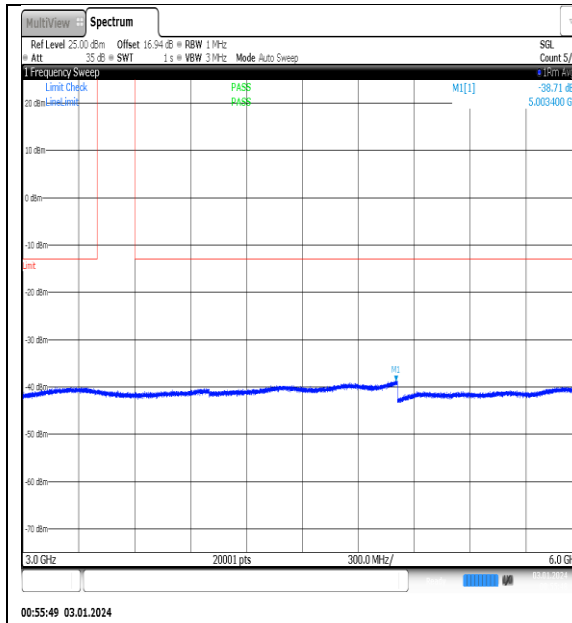
NTNV_N77-3450- 3550_PC2_30_100_M_TID6_NS_01_3000_6000_#1
