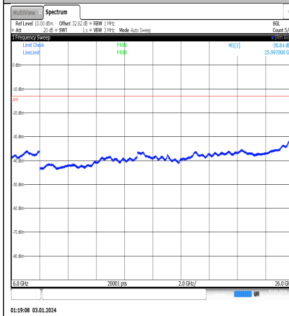
NTNV_N77-3450- 3550_PC2_30_100_M_TID13_NS_01_6000_2600 0_#1
