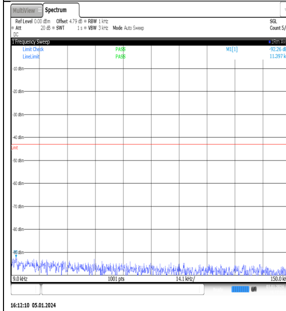
NTNV_N77-3700- 3980_PC2_30_10_L_TID5_NS_01_0.009_0.15_# 1
