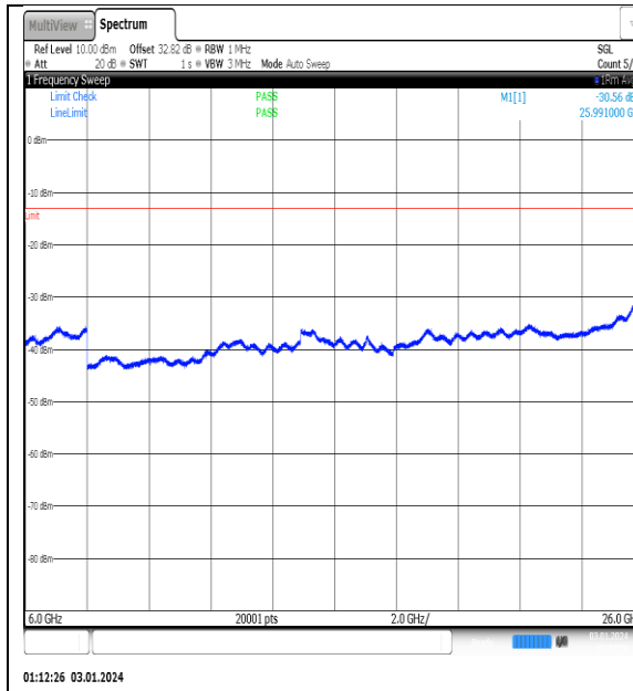
NTNV_N77-3450- 3550_PC2_30_100_M_TID11_NS_01_6000_2600 _0_#1
