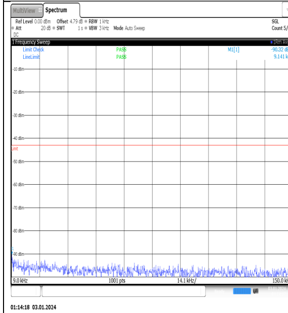
NTNV_N77-3450- 3550_PC2_30_100_M_TID12_NS_01_0.009_0.15 _#1
