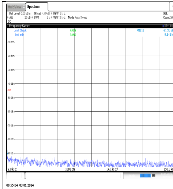
NTNV_N77-3450- 3550_PC2_30_100_M_TID6_NS_01_0.009_0.15_ #1
