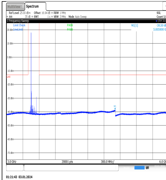
NTNV_N77-3450- 3550_PC2_30_100_M_TID14_NS_01_3000_6000 _#1
