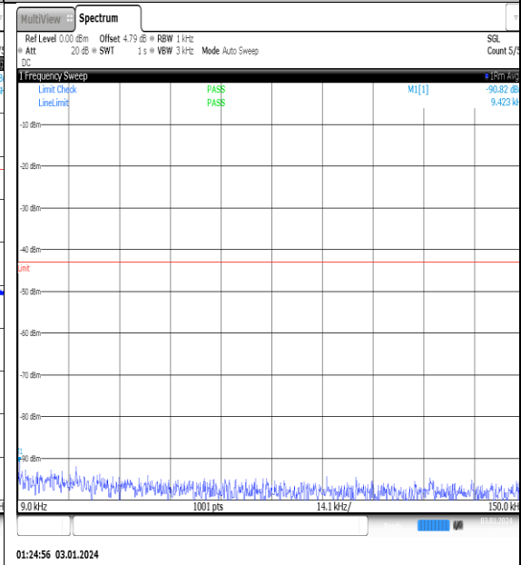
NTNV_N77-3450- 3550_PC2_30_100_M_TID15_NS_01_0.009_0.15 _#1
