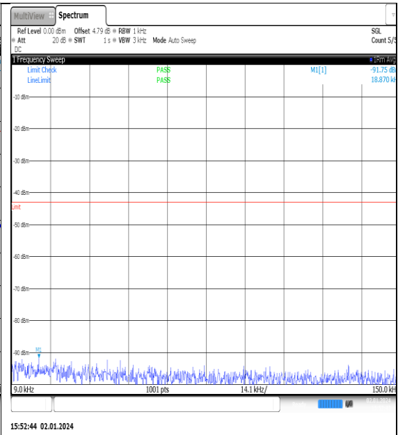
NTNV_N77-3450- 3550_PC2_30_90_L_TID11_NS_01_0.009_0.15_ #1
