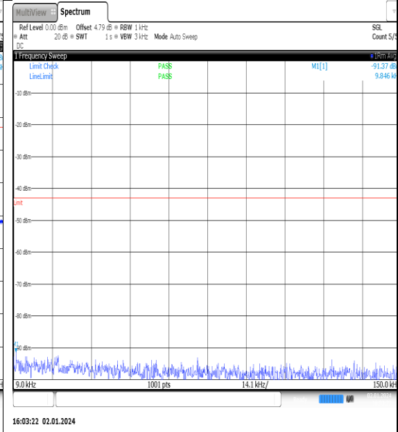
NTNV_N77-3450- 3550_PC2_30_90_L_TID13_NS_01_0.009_0.15_ #1
