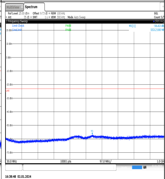
NTNV_N77-3450- 3550_PC2_30_90_M_TID8_NS_01_30_1000_#1
