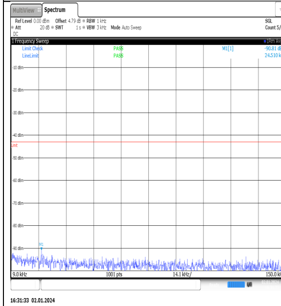
NTNV_N77-3450- 3550_PC2_30_90_M_TID7_NS_01_0.009_0.15_#1
