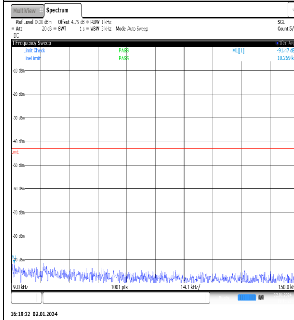
NTNV_N77-3450- 3550_PC2_30_90_M_TID3_NS_01_0.009_0.15_#1
