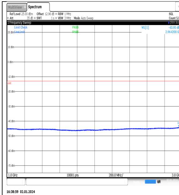
NTNV_N77-3450- 3550_PC2_30_90_M_TID8_NS_01_1000_3000_# 1
