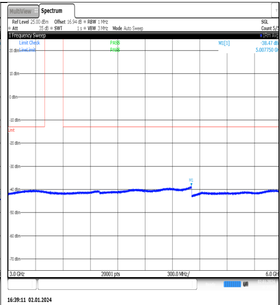
NTNV_N77-3450- 3550_PC2_30_90_M_TID8_NS_01_3000_6000_# 1
