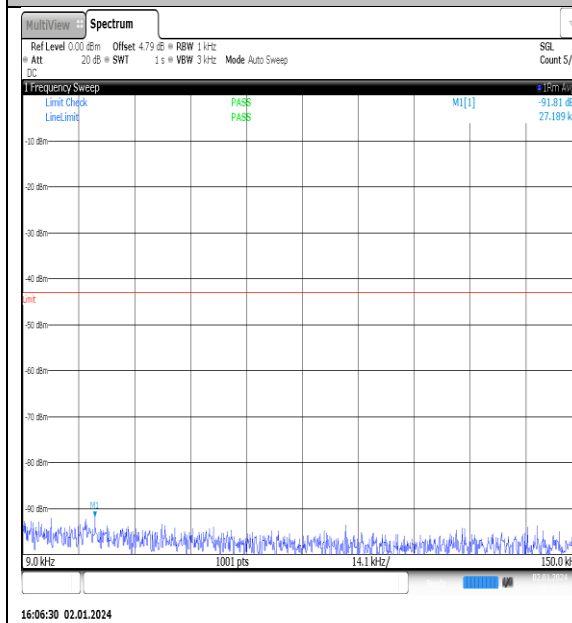
NTNV_N77-3450- 3550_PC2_30_90_L_TID14_NS_01_0.009_0.15_#1
