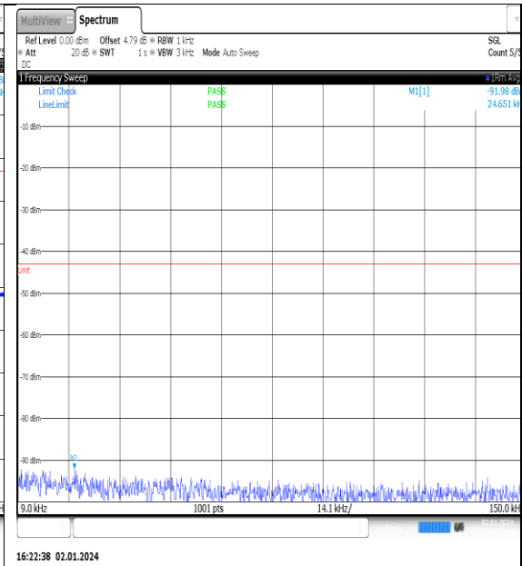
NTNV_N77-3450- 3550_PC2_30_90_M_TID4_NS_01_0.009_0.15_# 1
