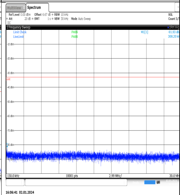
NTNV_N77-3450- 3550_PC2_30_90_L_TID14_NS_01_0.15_30_#1
