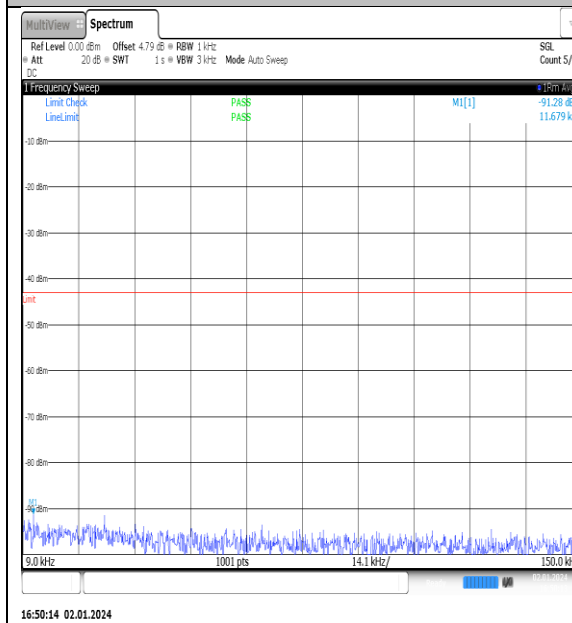
NTNV_N77-3450- 3550_PC2_30_90_M_TID11_NS_01_0.009_0.15_#1
