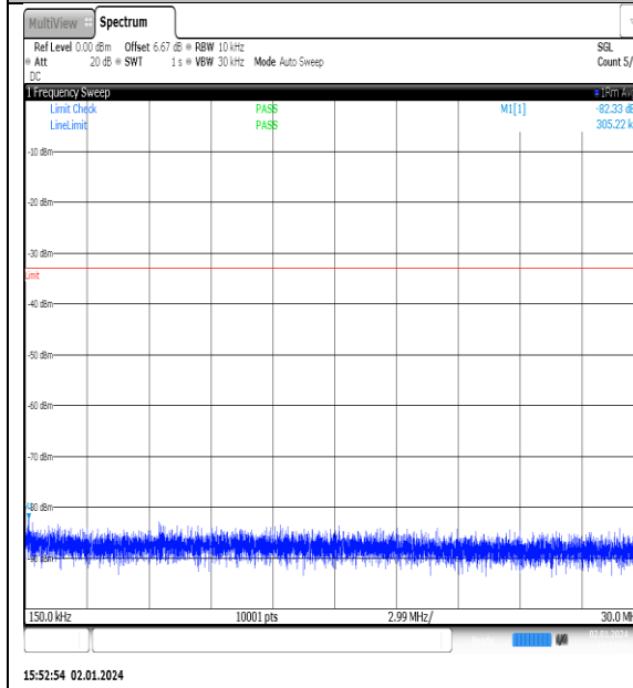
NTNV_N77-3450- 3550_PC2_30_90_L_TID11_NS_01_0.15_30_#1
