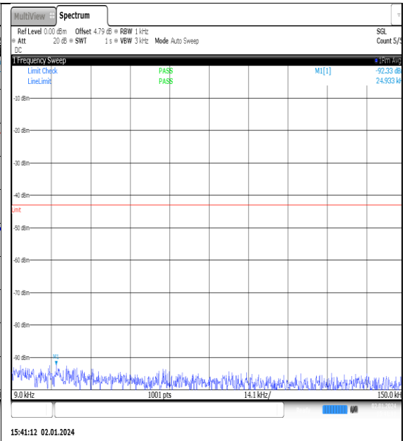
NTNV_N77-3450- 3550_PC2_30_90_L_TID7_NS_01_0.009_0.15_# 1
