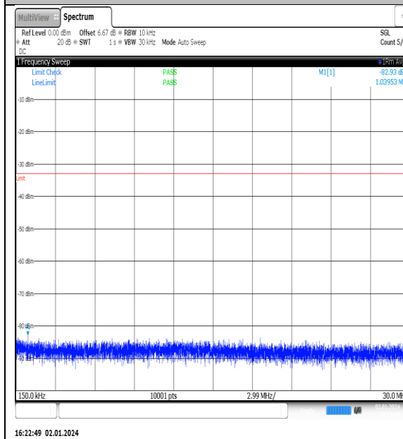
NTNV_N77-3450- 3550_PC2_30_90_M_TID4_NS_01_0.15_30_#1
