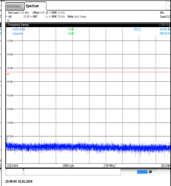
NTNV_N77-3450- 3550_PC2_30_90_L_TID10_NS_01_0.15_30_#1
