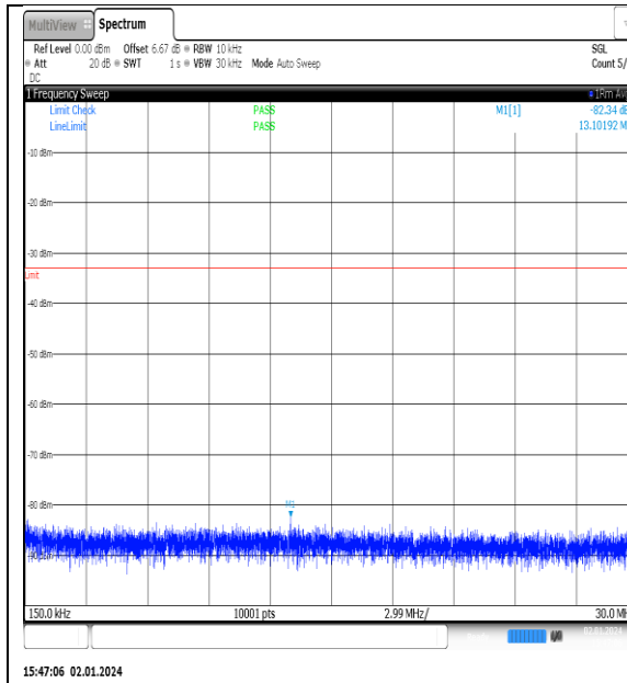
NTNV_N77-3450- 3550_PC2_30_90_L_TID9_NS_01_0.15_30_#1
