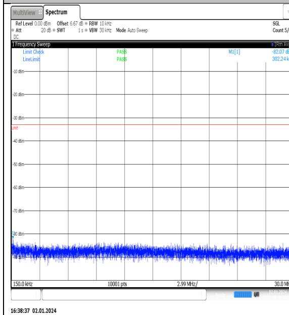
NTNV_N77-3450- 3550_PC2_30_90_M_TID8_NS_01_0.15_30_#1
