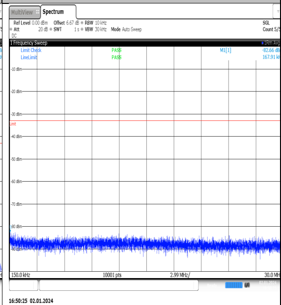
NTNV_N77-3450- 3550_PC2_30_90_M_TID11_NS_01_0.15_30_#1
