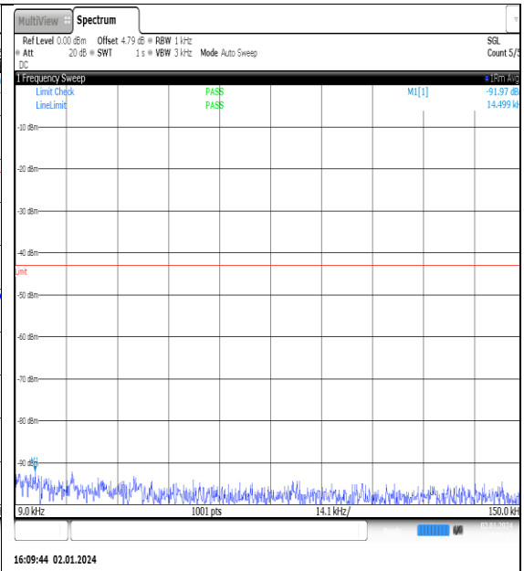
NTNV_N77-3450- 3550_PC2_30_90_L_TID15_NS_01_0.009_0.15_#1
