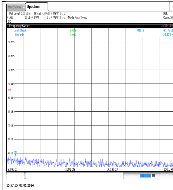
NTNV_N77-3450- 3550_PC2_30_90_L_TID12_NS_01_0.009_0.15_#1
