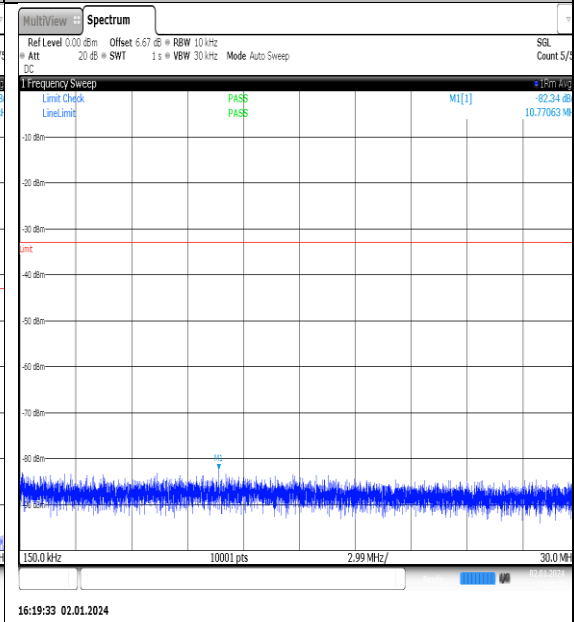
NTNV_N77-3450- 3550_PC2_30_90_M_TID3_NS_01_0.15_30_#1
