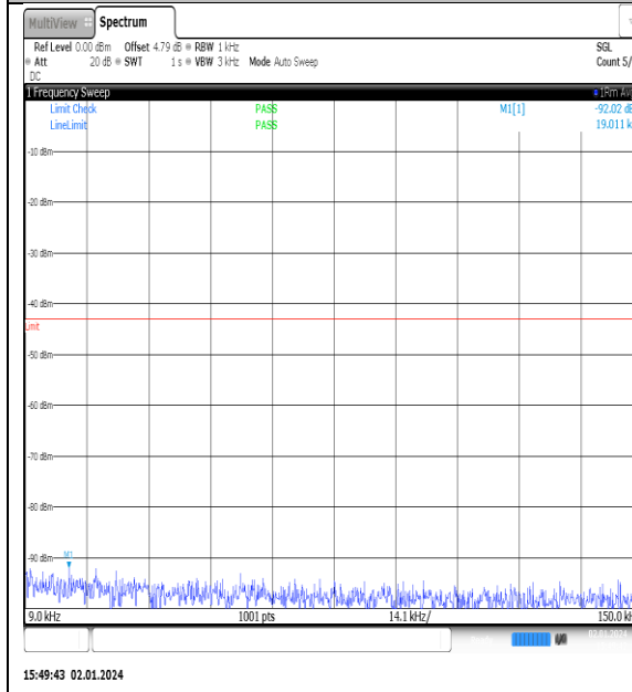
NTNV_N77-3450- 3550_PC2_30_90_L_TID10_NS_01_0.009_0.15_ #1
