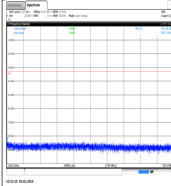
NTNV_N77-3450- 3550_PC2_30_90_L_TID3_NS_01_0.15_30_#1
