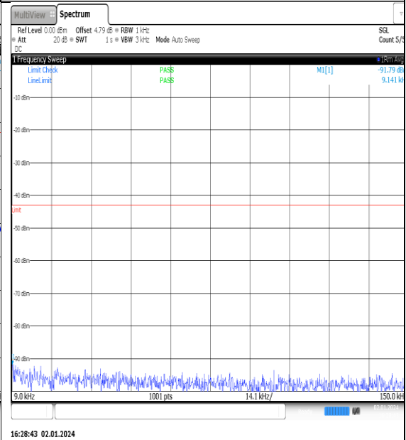
NTNV_N77-3450- 3550_PC2_30_90_M_TID6_NS_01_0.009_0.15_# 1
