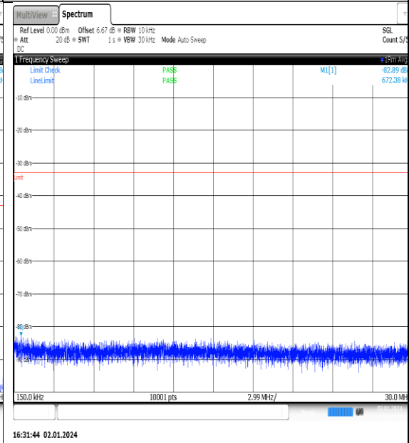
NTNV_N77-3450- 3550_PC2_30_90_M_TID7_NS_01_0.15_30_#1
