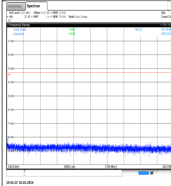
NTNV_N77-3450- 3550_PC2_30_90_L_TID7_NS_01_0.15_30_#1
