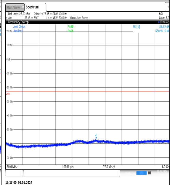
NTNV_N77-3450- 3550_PC2_30_90_M_TID4_NS_01_30_1000_#1
