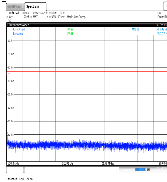
NTNV_N77-3450- 3550_PC2_30_90_L_TID5_NS_01_0.15_30_#1
