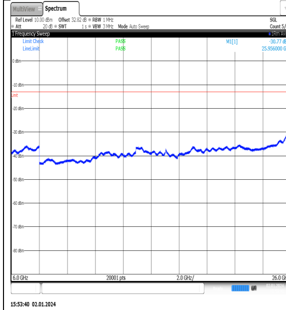
NTNV_N77-3450- 3550_PC2_30_90_L_TID11_NS_01_6000_26000 #1
