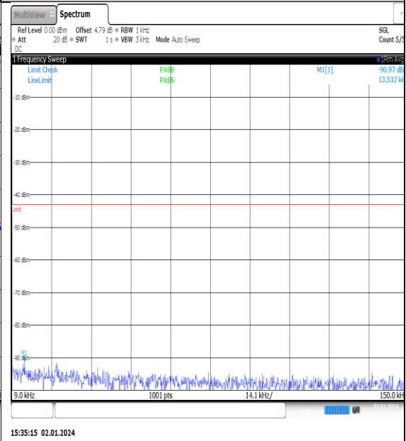
NTN_V_N77-3450- 3550_PC2_30_90_L_TID5_NS_01_0.009_0.15_# 1
