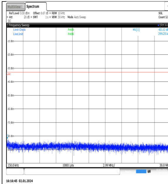
NTNV_N77-3450- 3550_PC2_30_90_M_TID2_NS_01_0.15_30_#1
