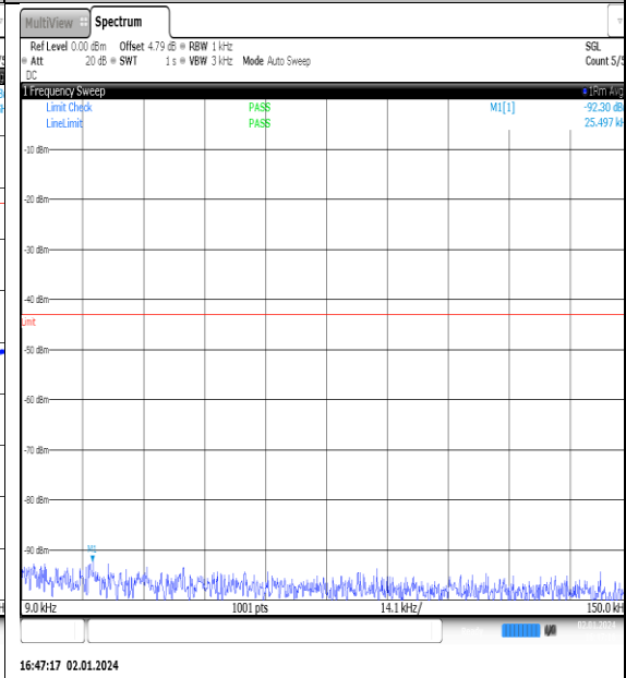
NTN_V_N77-3450- 3550_PC2_30_90_M_TID10_NS_01_0.009_0.15_# #1
