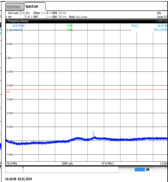
NTNV_N77-3450- 3550_PC2_30_90_M_TID2_NS_01_30_1000_#1
