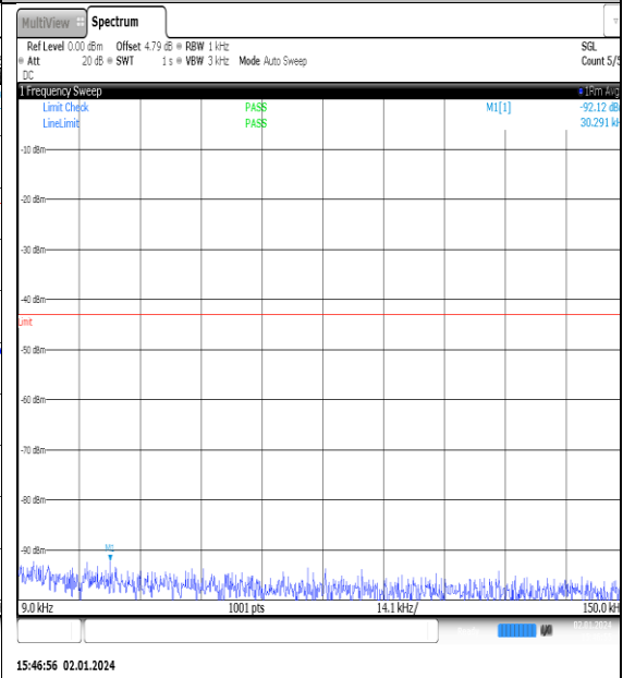
NTNV_N77-3450- 3550_PC2_30_90_L_TID9_NS_01_0.009_0.15_# 1
