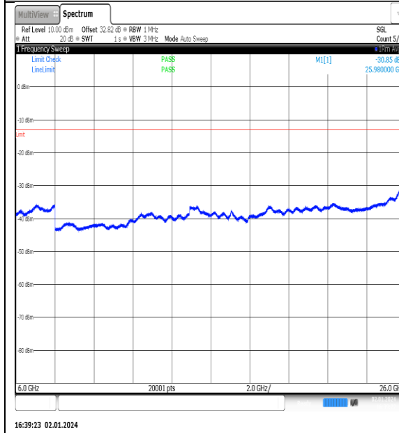
NTNV_N77-3450- 3550_PC2_30_90_M_TID8_NS_01_6000_26000_# 1
