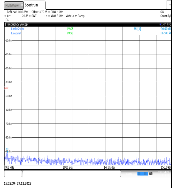
15:28:34 29.12.2023 NTNV_N77-3450- 3550_PC2_30_80_H_TID2_NS_01_0.009_0.15_# 1
