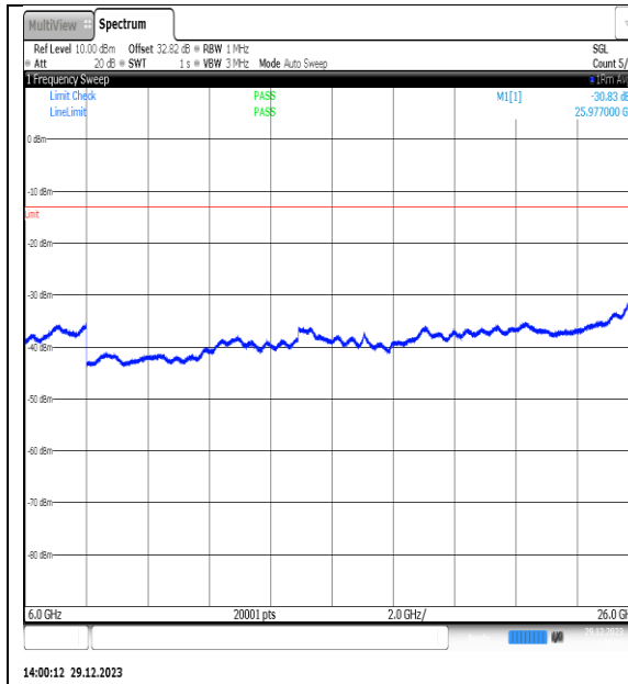
NTNV_N77-3450- 3550_PC2_30_80_M_TID14_NS_01_6000_26000 #1
