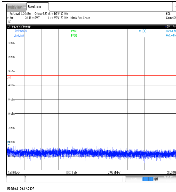
NTNV_N77-3450- 3550_PC2_30_80_H_TID2_NS_01_0.15_30_#1
