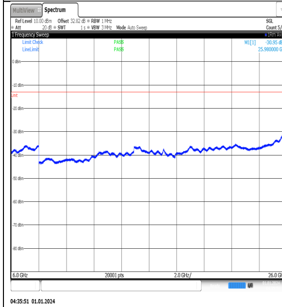
NTNV_N77-3450- 3550_PC2_30_80_H_TID11_NS_01_6000_26000_#1
