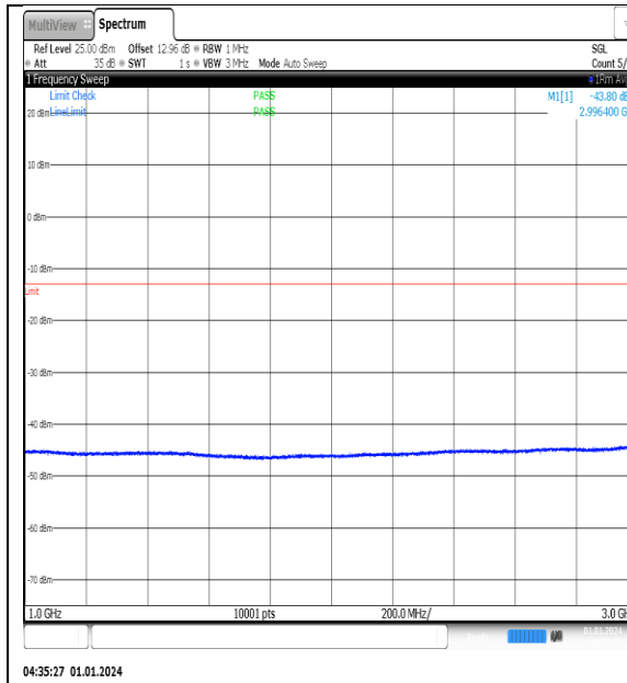
NTNV_N77-3450- 3550_PC2_30_80_H_TID11_NS_01_1000_3000_#1
