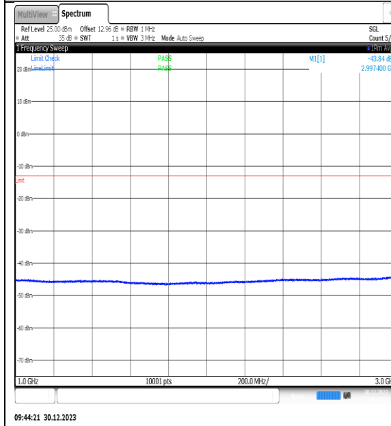
NTNV_N77-3450- 3550_PC2_30_80_H_TID9_NS_01_1000_3000_#1
