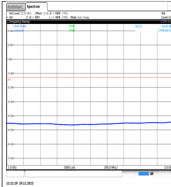
NTNV_N77-3450- 3550_PC2_30_80_M_TID5_NS_01_1000_3000_# 1
