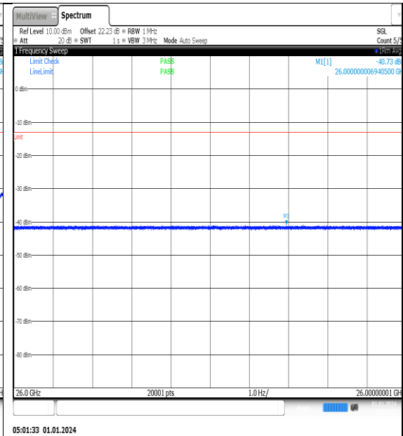
NTNV_N77-3450- 3550_PC2_30_80_H_TID14_NS_01_26000_4000 0_#1
