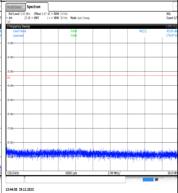
NTNV_N77-3450- 3550_PC2_30_80_M_TID11_NS_01_0.15_30_#1
