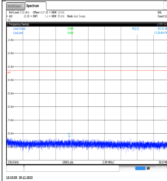
NTNV_N77-3450- 3550_PC2_30_80_M_TID8_NS_01_0.15_30_#1
