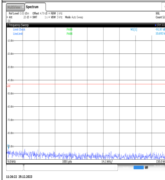
NTNV_N77-3450- 3550_PC2_30_80_L_TID11_NS_01_0.009_0.15_#1
