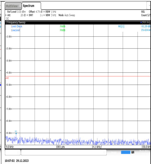
NTNV_N77-3450- 3550_PC2_30_80_L_TID8_NS_01_0.009_0.15_# 1
