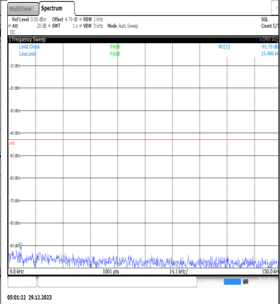
05:01:22 29.12.2023 NTNV_N77-3450- 3550_PC2_30_70_H_TID13_NS_01_0.009_0.15_ #1
