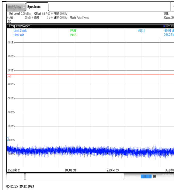
NTNV_N77-3450- 3550_PC2_30_70_H_TID13_NS_01_0.15_30_#1
