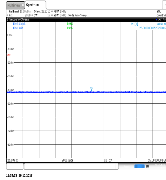
NTNV_N77-3450- 3550_PC2_30_80_L_TID13_NS_01_26000_4000_0_#1
