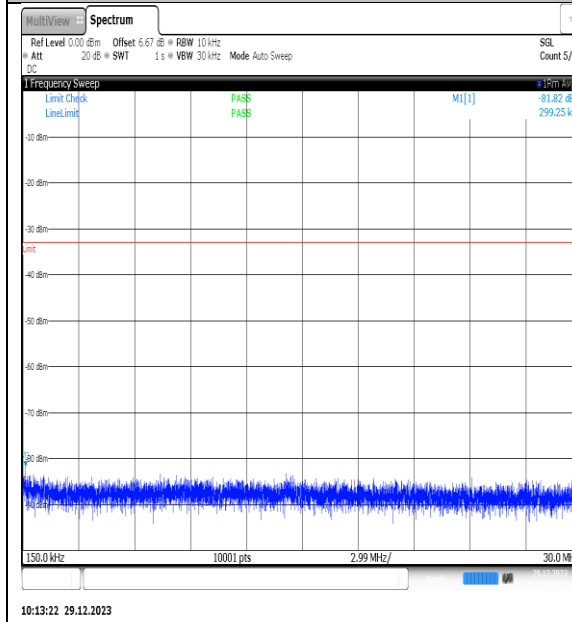
NTNV_N77-3450- 3550_PC2_30_80_L_TID8_NS_01_0.15_30_#1
