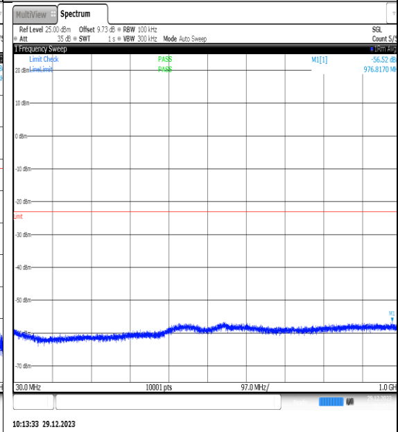
NTNV_N77-3450- 3550_PC2_30_80_L_TID8_NS_01_30_1000_#1
