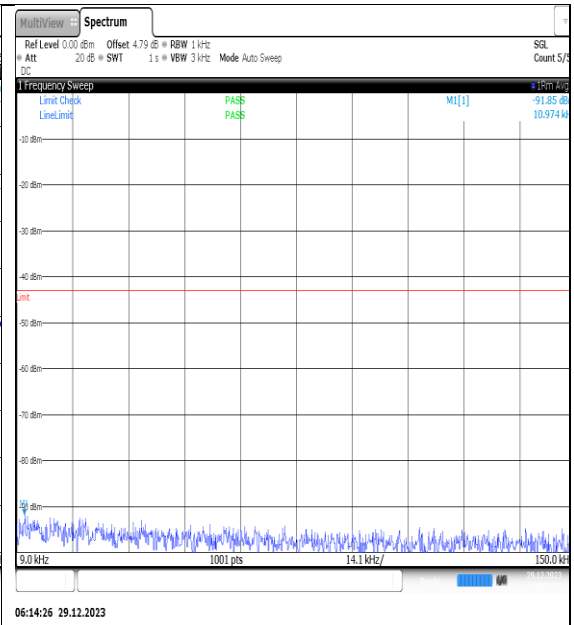
NTNV_N77-3450- 3550_PC2_30_70_H_TID15_NS_01_0.009_0.15_#1
