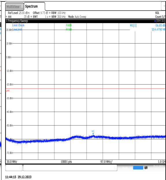
NTNV_N77-3450-3550_PC2_30_80_L_TID14_NS_01_30_1000_#1
