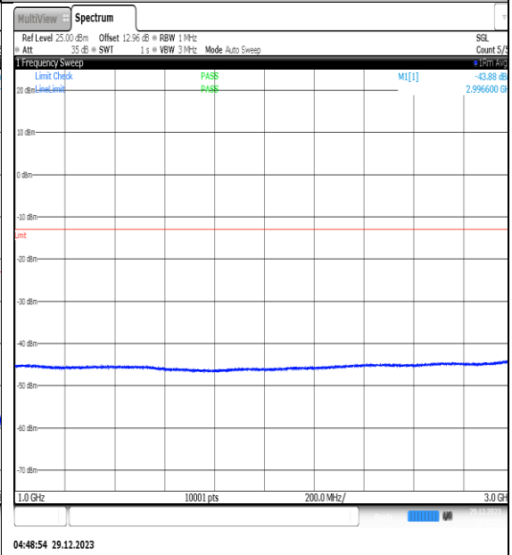
NTNV_N77-3450- 3550_PC2_30_70_H_TID12_NS_01_1000_3000_ #1
