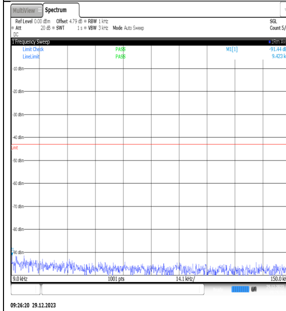
NTNV_N77-3450- 3550_PC2_30_80_L_TID7_NS_01_0.009_0.15_# 1
