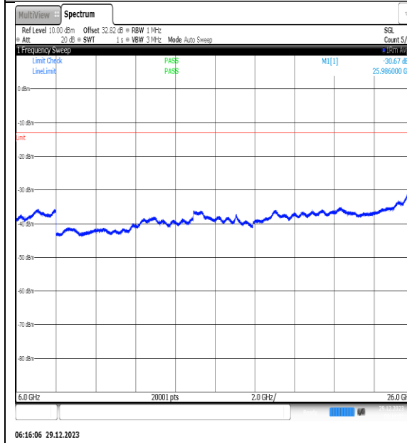
NTNV_N77-3450- 3550_PC2_30_70_H_TID15_NS_01_6000_26000 _#1
