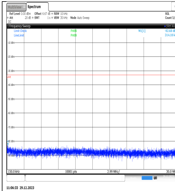
NTNV_N77-3450-3550_PC2_30_80_L_TID10_NS_01_0.15_30_#1
