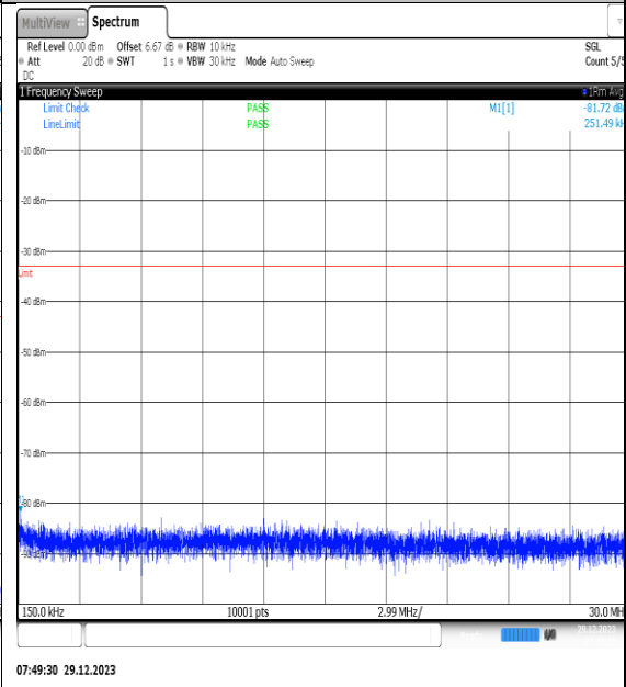
NTNV_N77-3450- 3550_PC2_30_80_L_TID3_NS_01_0.15_30_#1
