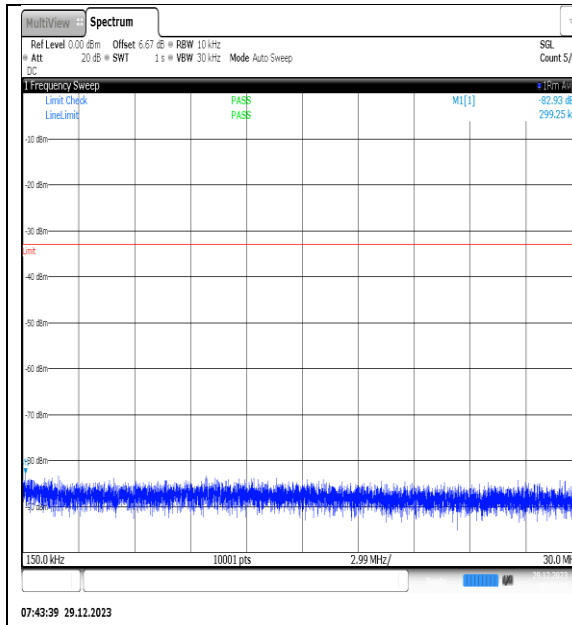
NTNV_N77-3450- 3550_PC2_30_80_L_TID2_NS_01_0.15_30_#1
