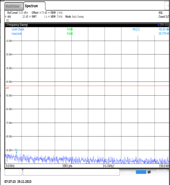
NTNV_N77-3450- 3550_PC2_30_80_L_TID2_NS_01_0.009_0.15_# 1
