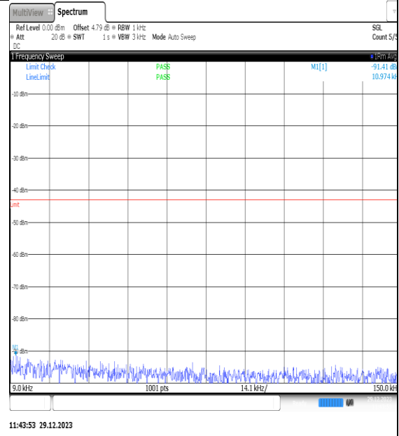
NTNV_N77-3450- 3550_PC2_30_80_L_TID14_NS_01_0.009_0.15_#1
