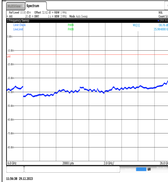
NTN_V_N77-3450- 3550_PC2_30_80_M_TID1_NS_01_6000_26000_# #1
