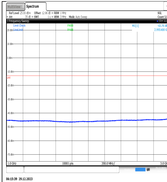
NTNV_N77-3450- 3550_PC2_30_70_H_TID15_NS_01_1000_3000_ #1
