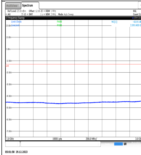
NTNV_N77-3450- 3550_PC2_30_70_H_TID13_NS_01_1000_3000_#1
