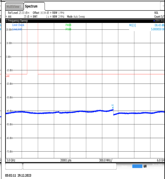
NTNV_N77-3450- 3550_PC2_30_70_H_TID13_NS_01_3000_6000_#1
