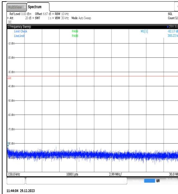
NTNV_N77-3450-3550_PC2_30_80_L_TID14_NS_01_0.15_30_#1
