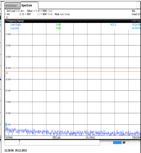
NTNV_N77-3450- 3550_PC2_30_80_M_TID5_NS_01_0.009_0.15_# 1
