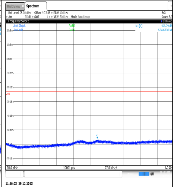
NTNV_N77-3450- 3550_PC2_30_80_M_TID1_NS_01_30_1000_#1
