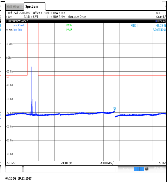
NTNV_N77-3450- 3550_PC2_30_70_H_TID11_NS_01_3000_6000_#1
