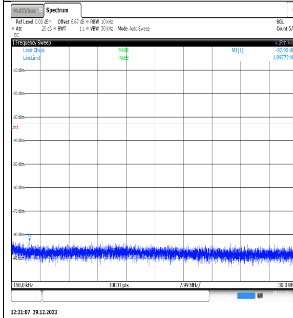
NTNV_N77-3450- 3550_PC2_30_80_M_TID5_NS_01_0.15_30_#1
