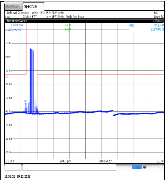
NTN_V_N77-3450- 3550_PC2_30_80_M_TID1_NS_01_3000_6000_# 1
