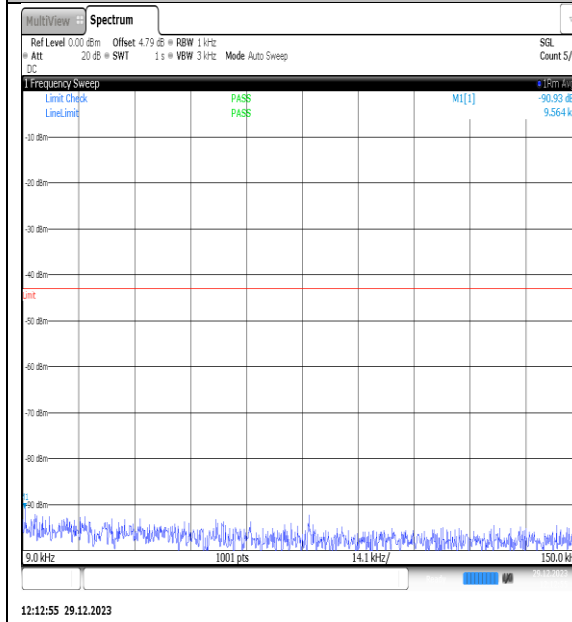
NTNV_N77-3450- 3550_PC2_30_80_M_TID4_NS_01_0.009_0.15_#1
