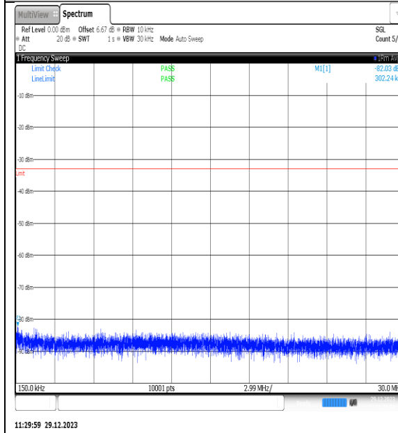
NTNV_N77-3450- 3550_PC2_30_80_L_TID12_NS_01_0.15_30_#1
