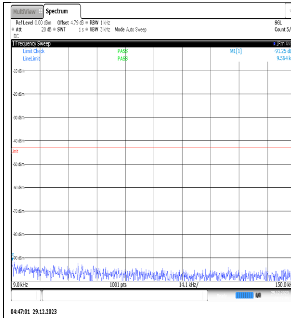
NTNV_N77-3450- 3550_PC2_30_70_H_TID12_NS_01_0.009_0.15_ #1
