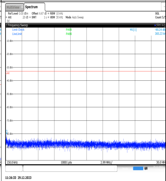
NTNV_N77-3450- 3550_PC2_30_80_L_TID11_NS_01_0.15_30_#1
