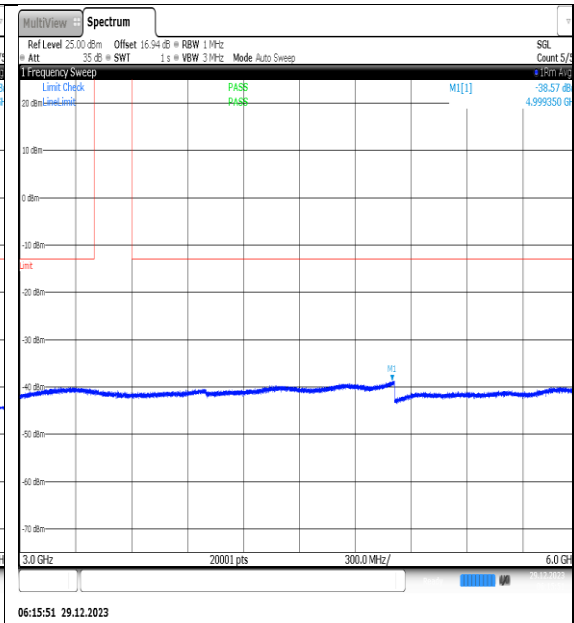
NTNV_N77-3450- 3550_PC2_30_70_H_TID15_NS_01_3000_6000_ #1
