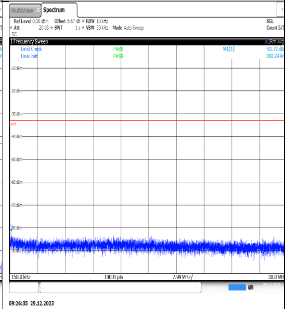
NTNV_N77-3450- 3550_PC2_30_80_L_TID7_NS_01_0.15_30_#1
