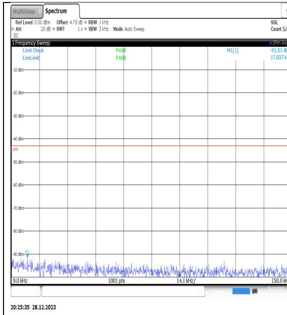
NTNV_N77-3450- 3550_PC2_30_70_M_TID11_NS_01_0.009_0.15_ #1
