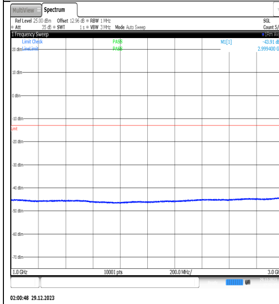
NTNV_N77-3450- 3550_PC2_30_70_H_TID5_NS_01_1000_3000_#1
