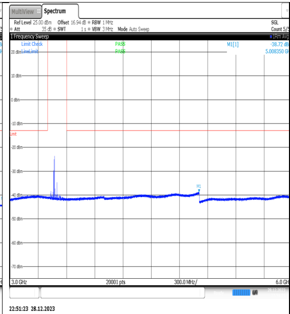
NTNV_N77-3450- 3550_PC2_30_70_M_TID14_NS_01_3000_6000_ #1
