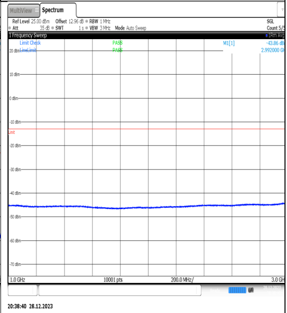
NTNV_N77-3450- 3550_PC2_30_70_M_TID11_NS_01_1000_3000_ #1
