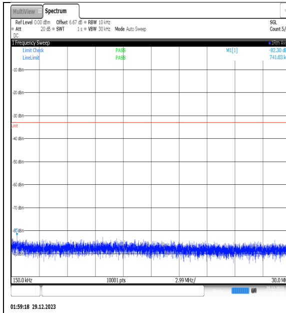
NTNV_N77-3450- 3550_PC2_30_70_H_TID5_NS_01_0.15_30_#1
