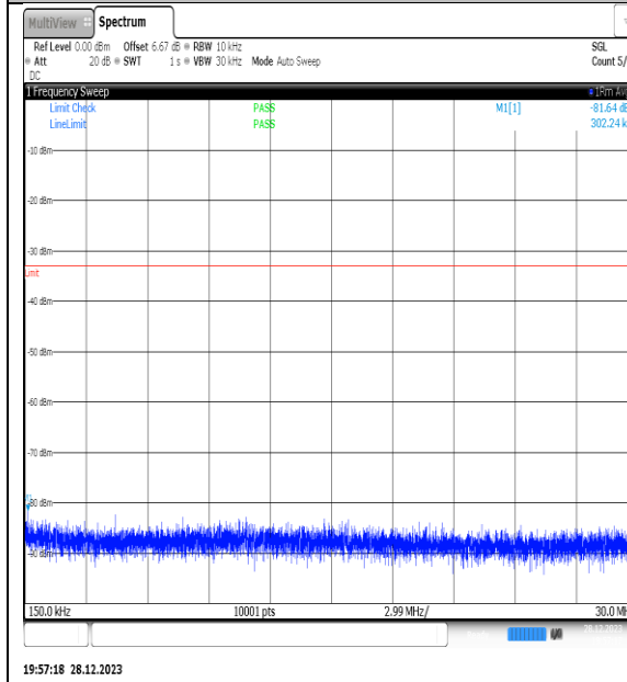
NTNV_N77-3450- 3550_PC2_30_70_M_TID10_NS_01_0.15_30_#1
