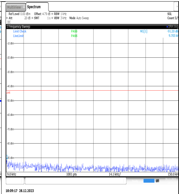
NTNV_N77-3450- 3550_PC2_30_70_M_TID6_NS_01_0.009_0.15_# 1
