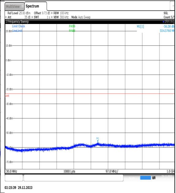
NTNV_N77-3450- 3550_PC2_30_70_H_TID7_NS_01_30_1000_#1
