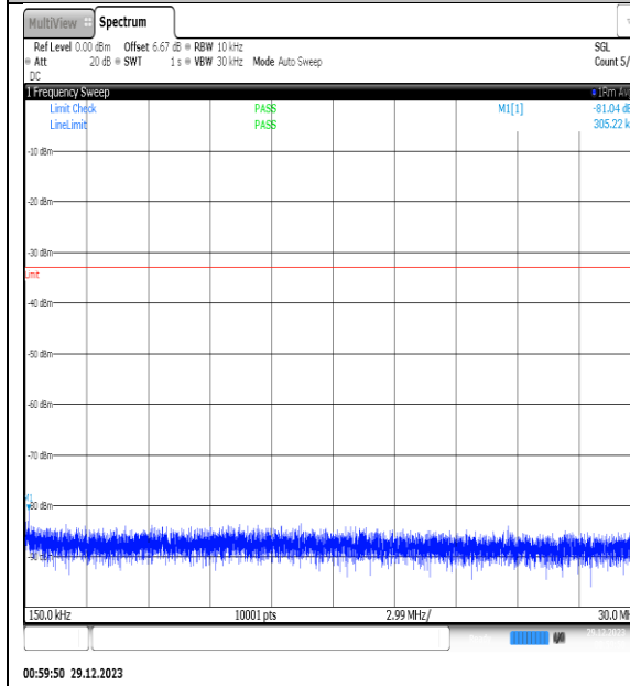
NTNV_N77-3450- 3550_PC2_30_70_H_TID3_NS_01_0.15_30_#1
