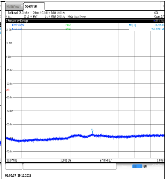
NTNV_N77-3450- 3550_PC2_30_70_H_TID5_NS_01_30_1000_#1
