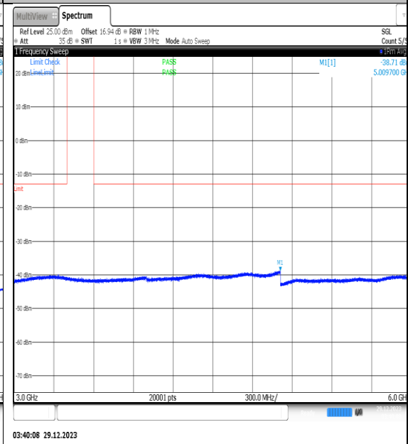
NTNV_N77-3450-3550_PC2_30_70_H_TID9_NS_01_3000_6000_#1
