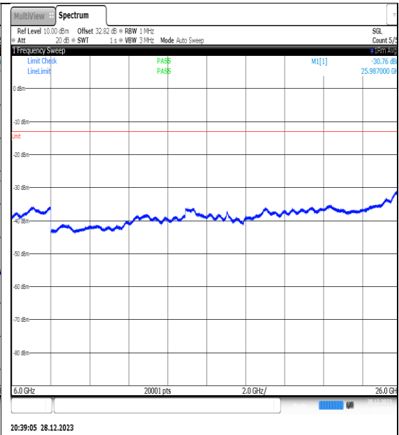
NTN_V_N77-3450- 3550_PC2_30_70_M_TID11_NS_01_6000_26000_ #1
