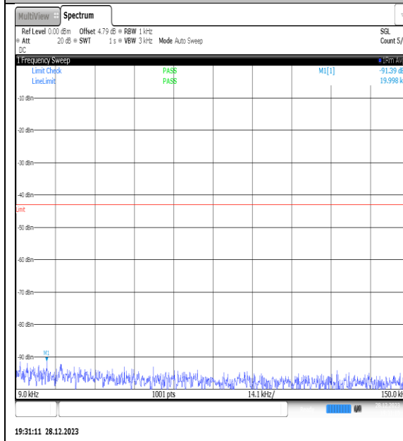
NTNV_N77-3450- 3550_PC2_30_70_M_TID9_NS_01_0.009_0.15_# 1
