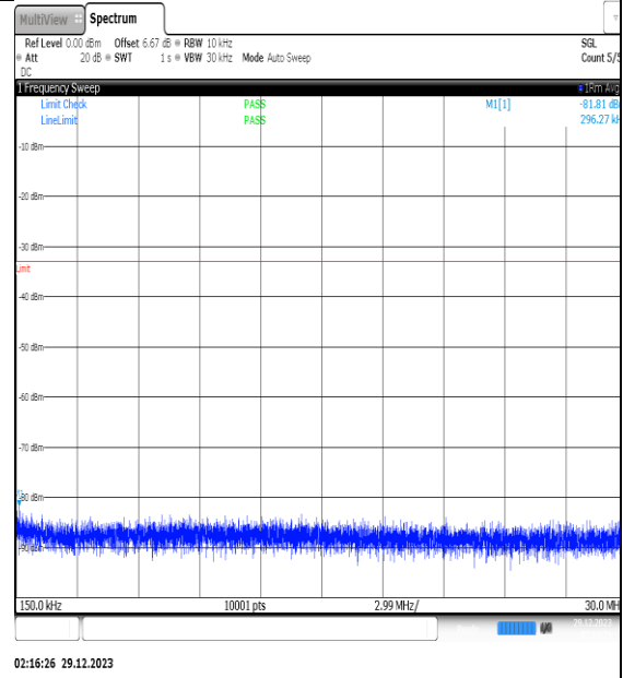
NTNV_N77-3450- 3550_PC2_30_70_H_TID6_NS_01_0.15_30_#1
