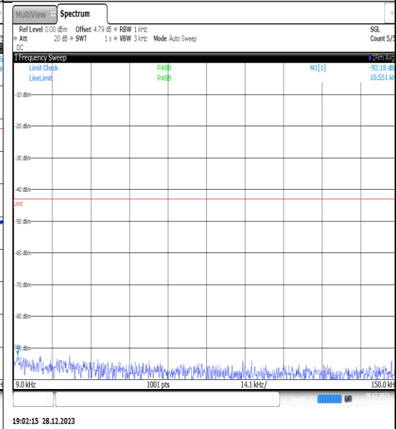
NTNV_N77-3450- 3550_PC2_30_70_M_TID8_NS_01_0.009_0.15_# 1
