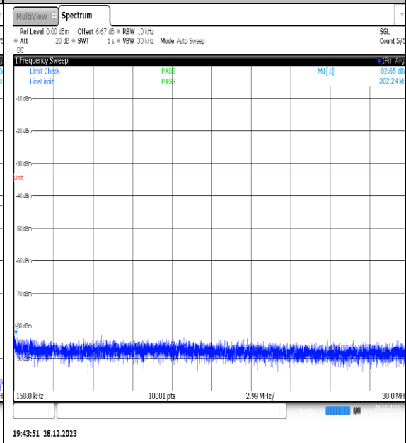
NTNV_N77-3450- 3550_PC2_30_70_M_TID9_NS_01_0.15_30_#1
