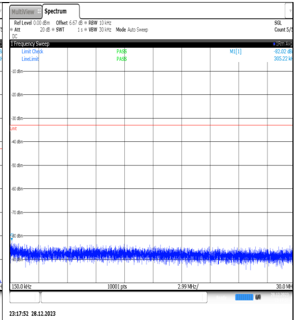
NTNV_N77-3450- 3550_PC2_30_70_M_TID15_NS_01_0.15_30_#1
