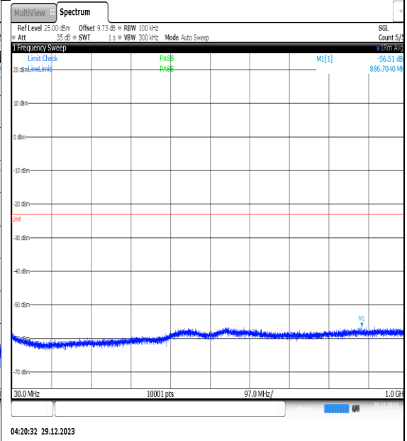
NTNV_N77-3450- 3550_PC2_30_70_H_TID11_NS_01_30_1000_#1
