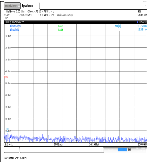
NTNV_N77-3450- 3550_PC2_30_70_H_TID11_NS_01_0.009_0.15_#1
