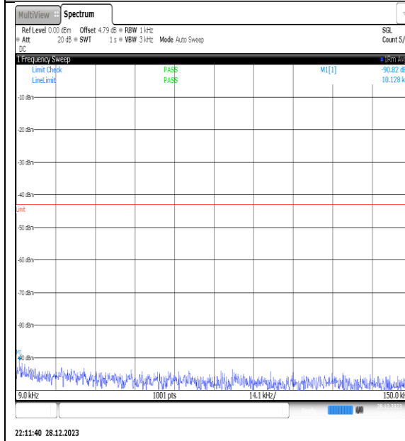
NTNV_N77-3450- 3550_PC2_30_70_M_TID13_NS_01_0.009_0.15_ _#1
