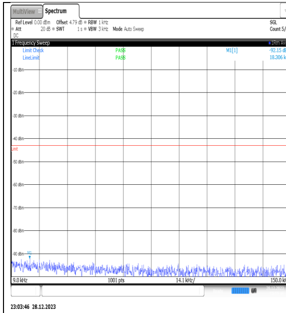
NTNV_N77-3450- 3550_PC2_30_70_M_TID15_NS_01_0.009_0.15_ #1
