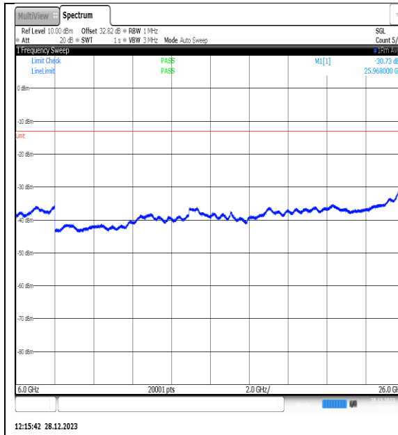
NTNV_N77-3450- 3550_PC2_30_60_H_TID2_NS_01_6000_26000_#1
