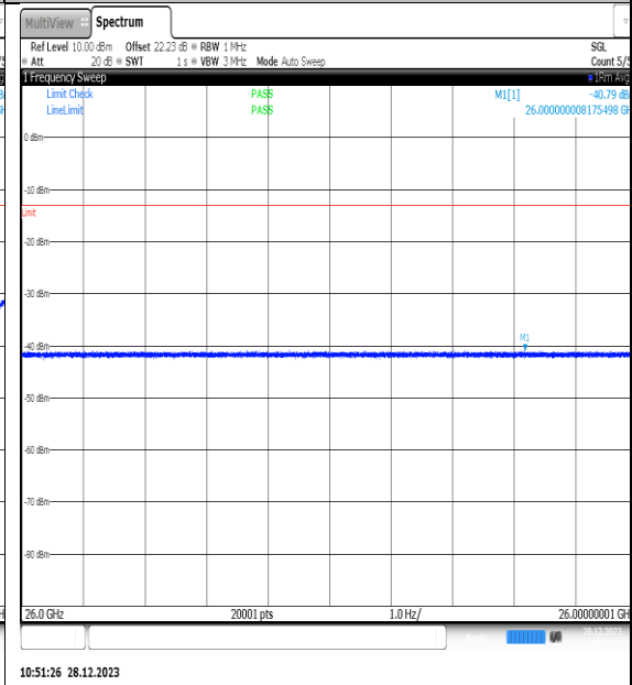
NTN_V_N77-3450- 3550_PC2_30_60_M_TID3_NS_01_26000_40000_# #1
