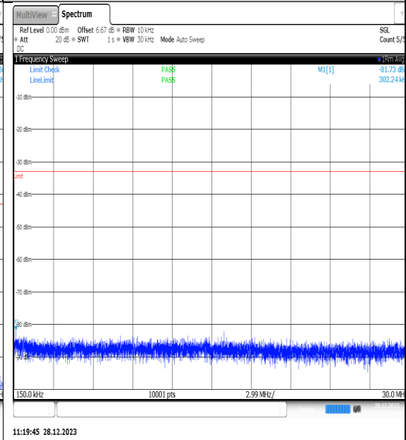
NTNV_N77-3450- 3550_PC2_30_60_M_TID10_NS_01_0.15_30_#1
