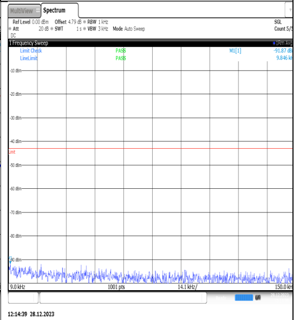
NTNV_N77-3450- 3550_PC2_30_60_H_TID2_NS_01_0.009_0.15_# 1
