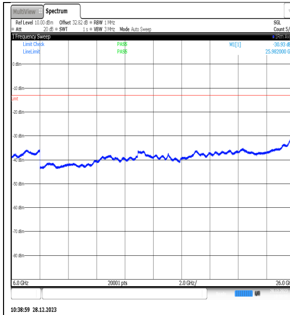
NTNV_N77-3450- 3550_PC2_30_60_M_TID1_NS_01_6000_26000_#1
