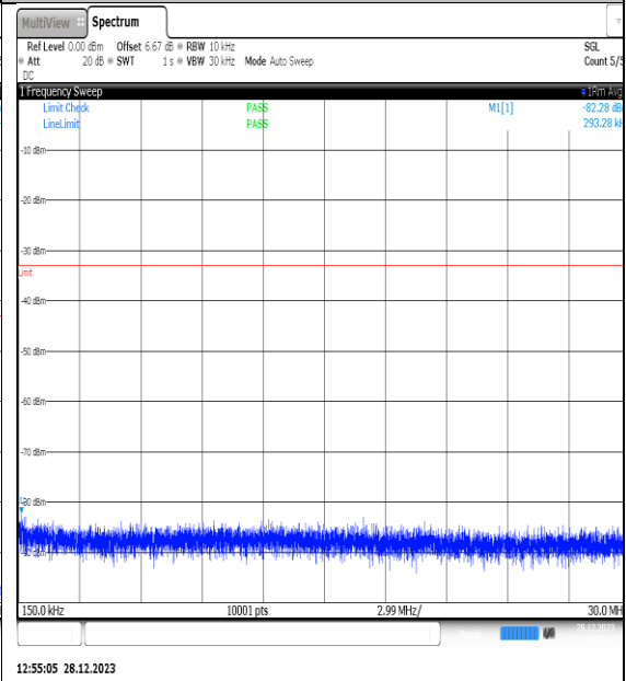
NTNV_N77-3450- 3550_PC2_30_60_H_TID7_NS_01_0.15_30_#1
