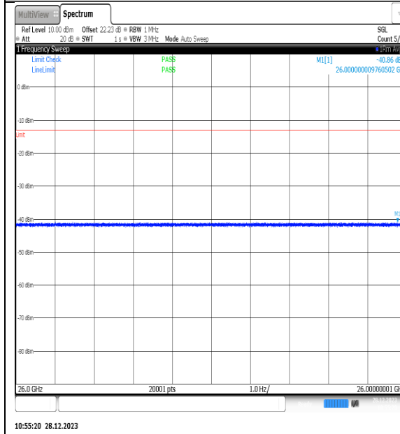
NTNV_N77-3450- 3550_PC2_30_60_M_TID4_NS_01_26000_40000_# #1
