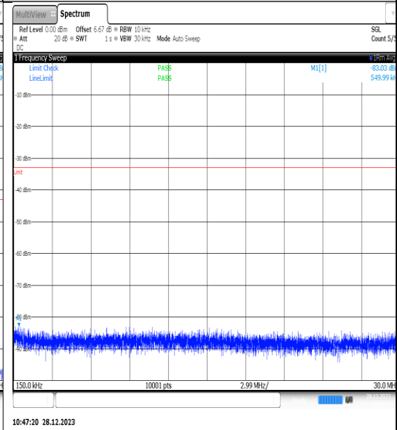
NTNV_N77-3450- 3550_PC2_30_60_M_TID2_NS_01_0.15_30_#1
