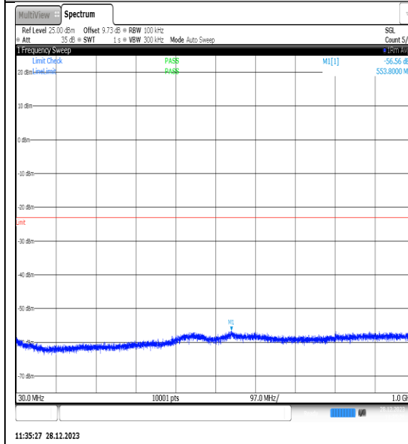
NTNV_N77-3450- 3550_PC2_30_60_M_TID12_NS_01_30_1000_#1
