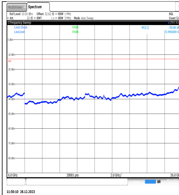
NTNV_N77-3450- 3550_PC2_30_60_M_TID13_NS_01_6000_26000 _#1
