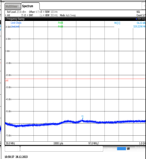
NTNV_N77-3450- 3550_PC2_30_60_M_TID3_NS_01_30_1000_#1
