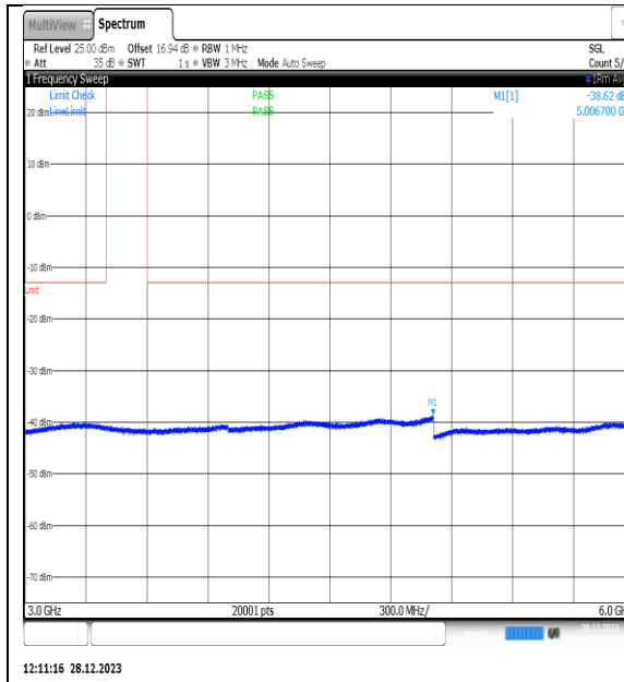
NTNV_N77-3450- 3550_PC2_30_60_H_TID1_NS_01_3000_6000_# 1
