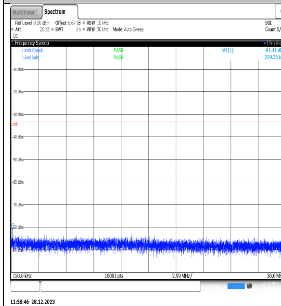
NTNV_N77-3450- 3550_PC2_30_60_M_TID15_NS_01_0.15_30_#1
