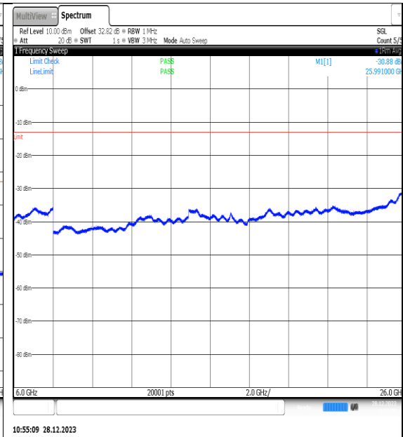
NTNV_N77-3450- 3550_PC2_30_60_M_TID4_NS_01_6000_26000_# #1
