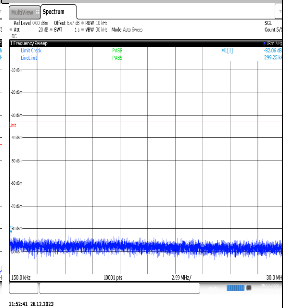
NTNV_N77-3450- 3550_PC2_30_60_M_TID14_NS_01_0.15_30_#1
