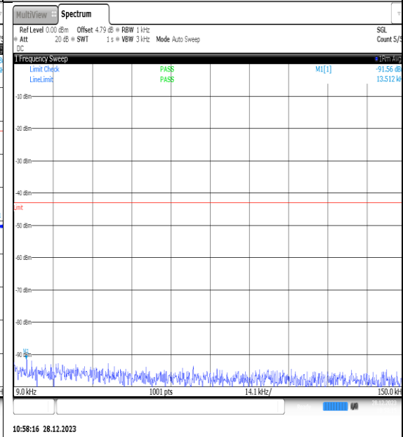
NTNV_N77-3450- 3550_PC2_30_60_M_TID5_NS_01_0.009_0.15_# 1
