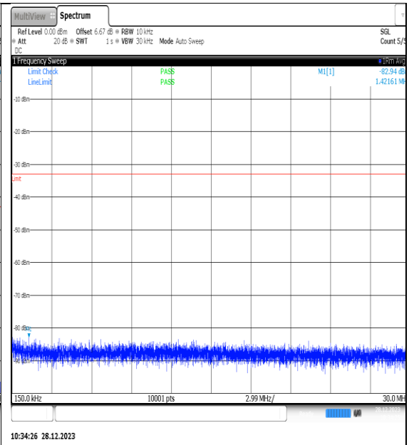
NTNV_N77-3450- 3550_PC2_30_60_L_TID15_NS_01_0.15_30_#1
