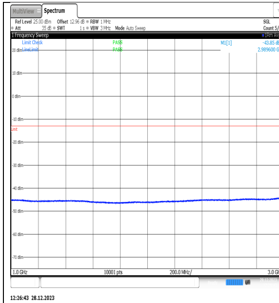
NTNV_N77-3450- 3550_PC2_30_60_H_TID4_NS_01_1000_3000_# 1
