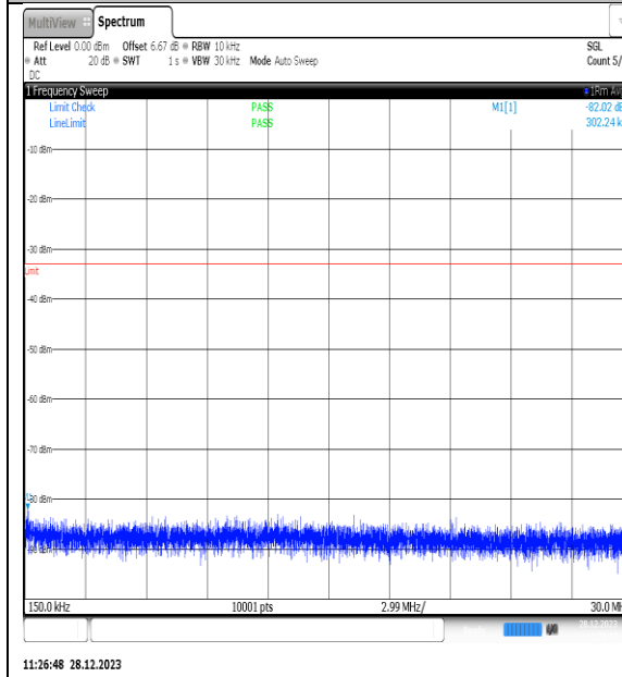
NTNV_N77-3450- 3550_PC2_30_60_M_TID11_NS_01_0.15_30_#1
