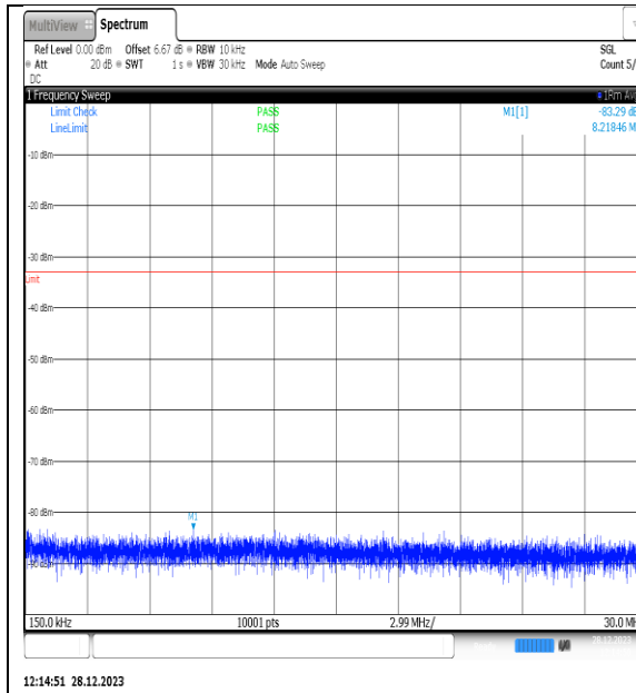
NTNV_N77-3450- 3550_PC2_30_60_H_TID2_NS_01_0.15_30_#1
