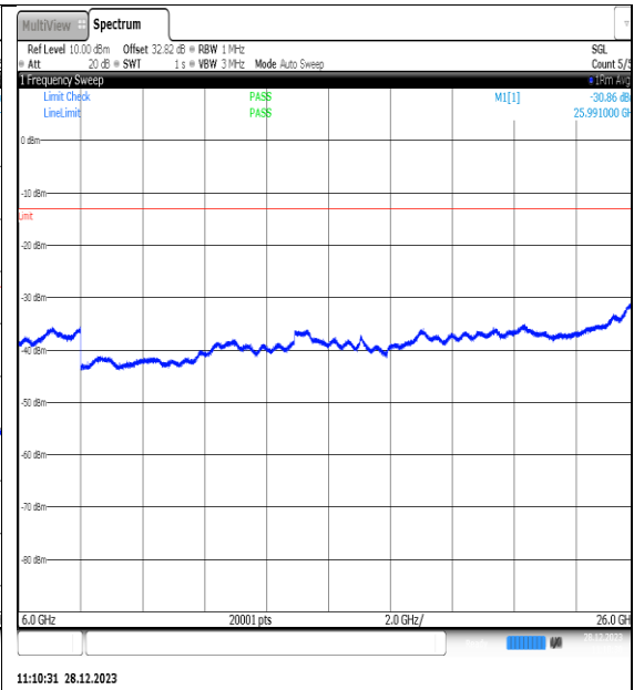
NTNV_N77-3450- 3550_PC2_30_60_M_TID8_NS_01_6000_26000_# 1
