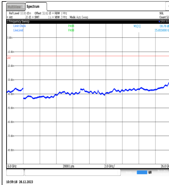
NTNV_N77-3450- 3550_PC2_30_60_M_TID5_NS_01_6000_26000_#1
