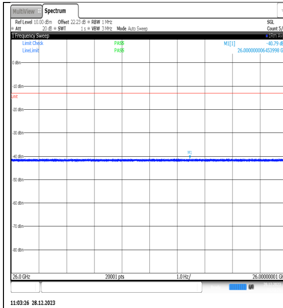
NTNV_N77-3450- 3550_PC2_30_60_M_TID6_NS_01_26000_40000 #1
