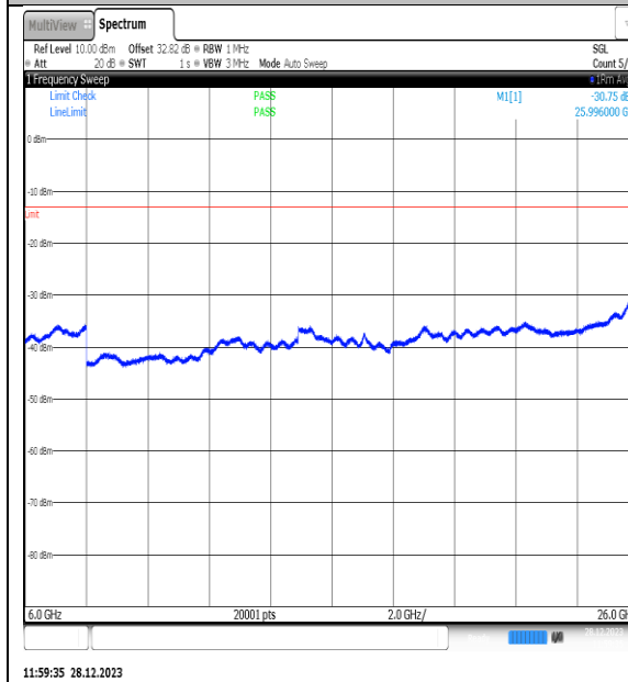
NTNV_N77-3450- 3550_PC2_30_60_M_TID15_NS_01_6000_26000_#1
