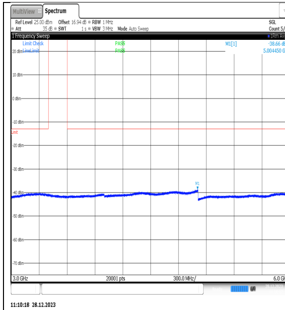
NTNV_N77-3450- 3550_PC2_30_60_M_TID8_NS_01_3000_6000_# 1
