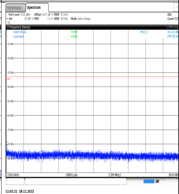
NTNV_N77-3450- 3550_PC2_30_60_M_TID6_NS_01_0.15_30_#1
