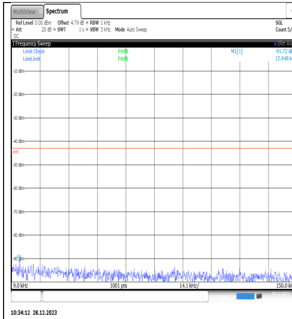
NTNV_N77-3450- 3550_PC2_30_60_L_TID15_NS_01_0.009_0.15_#1
