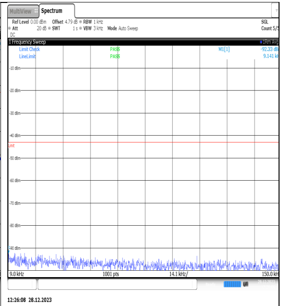
NTNV_N77-3450- 3550_PC2_30_60_H_TID4_NS_01_0.009_0.15_# 1
