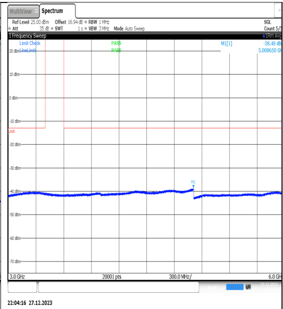
NTNV_N77-3450- 3550_PC2_30_50_H_TID13_NS_01_3000_6000_ #1
