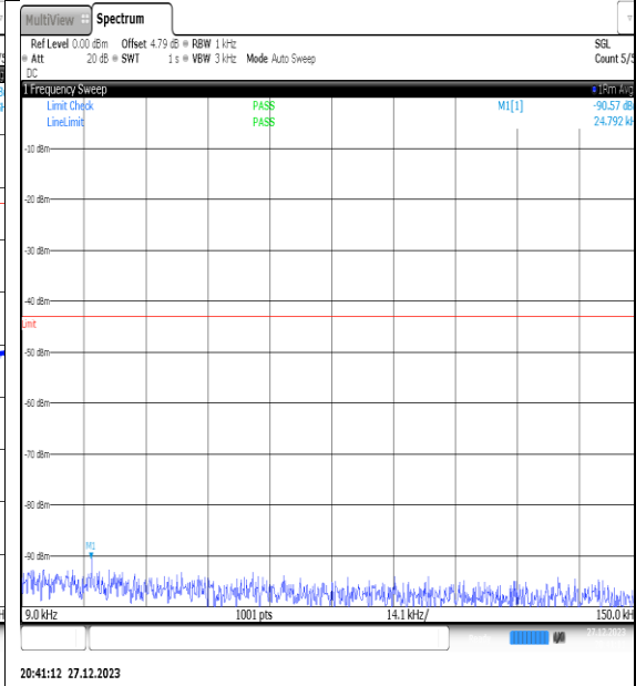
NTNV_N77-3450- 3550_PC2_30_50_H_TID7_NS_01_0.009_0.15_# 1
