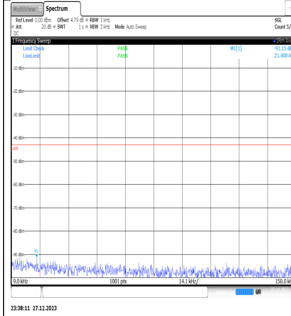
NTNV_N77-3450- 3550_PC2_30_60_L_TID6_NS_01_0.009_0.15_# 1
