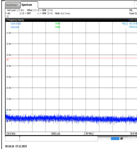
NTNV_N77-3450- 3550_PC2_30_50_H_TID5_NS_01_0.15_30_#1
