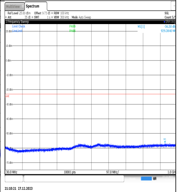
NTNV_N77-3450- 3550_PC2_30_50_H_TID9_NS_01_30_1000_#1
