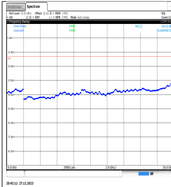
NTNV_N77-3450- 3550_PC2_30_50_H_TID7_NS_01_6000_26000_#1
