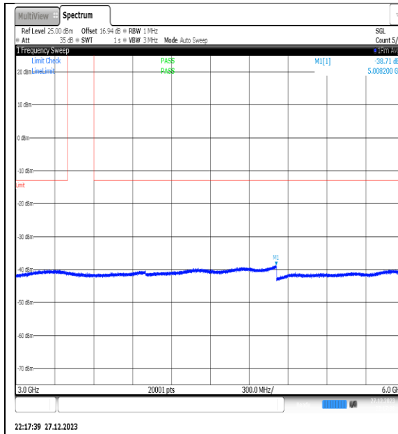
NTNV_N77-3450- 3550_PC2_30_50_H_TID14_NS_01_3000_6000_ #1
