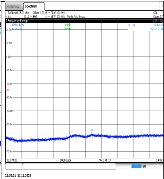
NTNV_N77-3450-3550_PC2_30_50_H_TID15_NS_01_30_1000_#1
