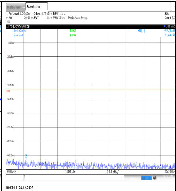
NTNV_N77-3450- 3550_PC2_30_60_L_TID10_NS_01_0.009_0.15_ #1
