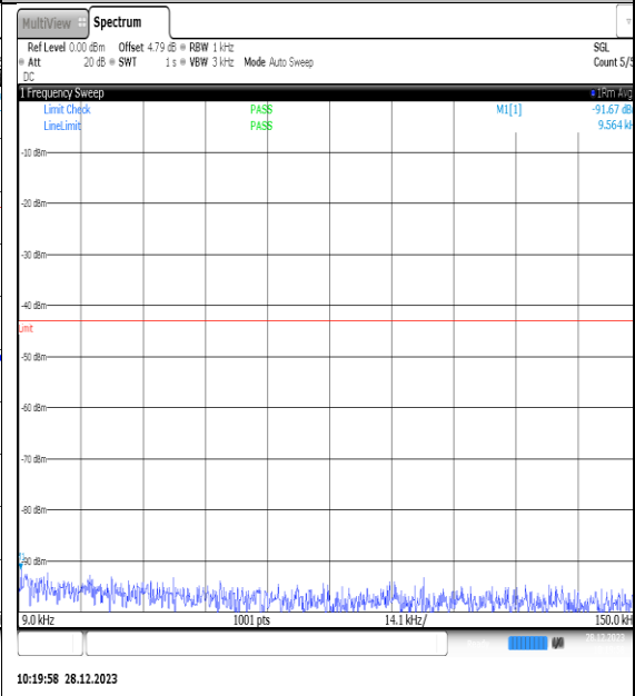
NTNV_N77-3450- 3550_PC2_30_60_L_TID12_NS_01_0.009_0.15_#1
