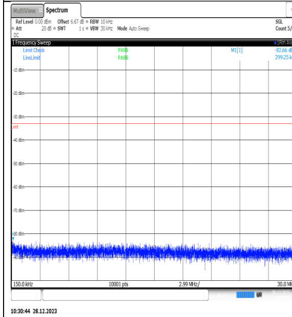
NTNV_N77-3450- 3550_PC2_30_60_L_TID14_NS_01_0.15_30_#1
