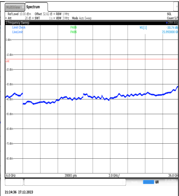
NTNV_N77-3450- 3550_PC2_30_50_H_TID10_NS_01_6000_26000_#1
