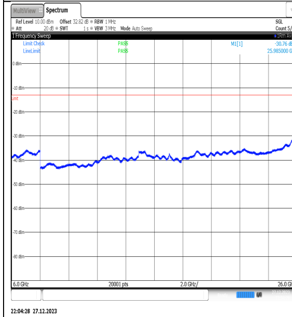
NTNV_N77-3450- 3550_PC2_30_50_H_TID13_NS_01_6000_26000_ #1
