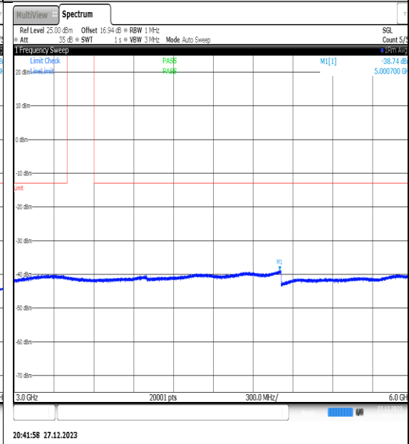
NTNV_N77-3450- 3550_PC2_30_50_H_TID7_NS_01_3000_6000_#1
