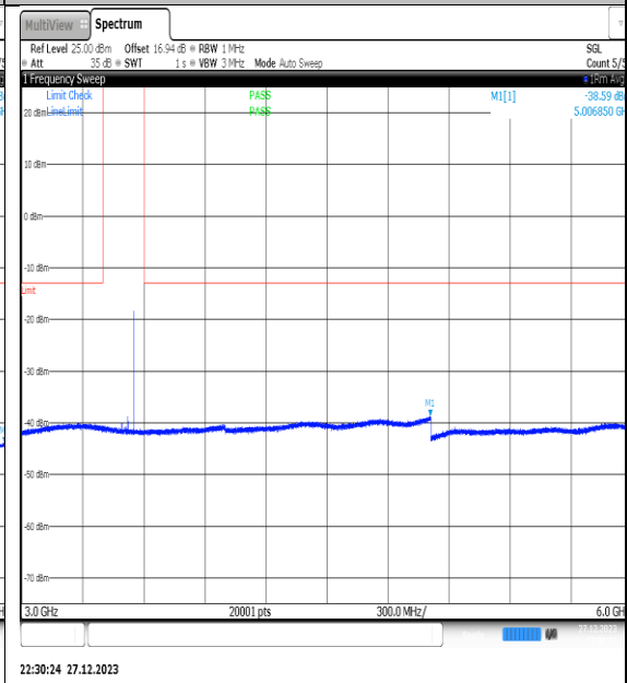
NTNV_N77-3450-3550_PC2_30_50_H_TID15_NS_01_3000_6000_#1
