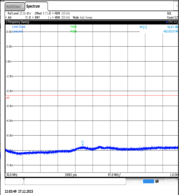
NTNV_N77-3450- 3550_PC2_30_50_H_TID13_NS_01_30_1000_#1
