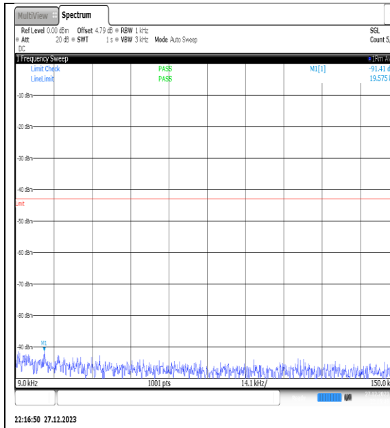
NTNV_N77-3450- 3550_PC2_30_50_H_TID14_NS_01_0.009_0.15_ #1
