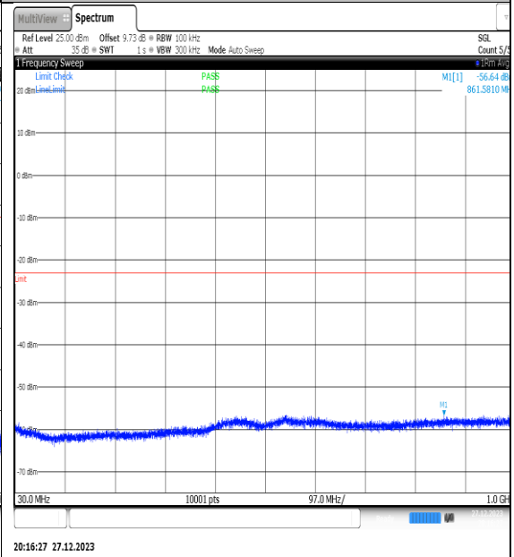
NTNV_N77-3450- 3550_PC2_30_50_H_TID5_NS_01_30_1000_#1
