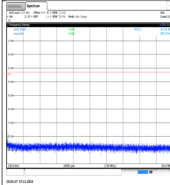
NTNV_N77-3450- 3550_PC2_30_60_L_TID7_NS_01_0.15_30_#1
