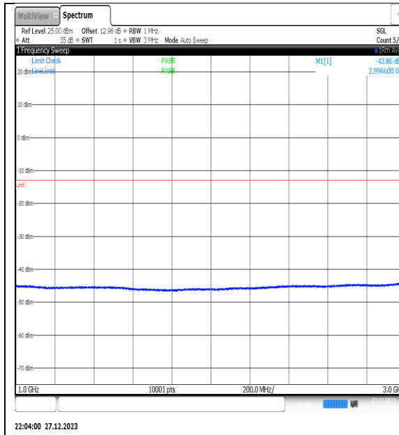
NTNV_N77-3450- 3550_PC2_30_50_H_TID13_NS_01_1000_3000_ #1
