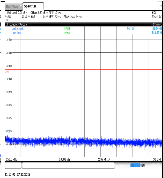
NTNV_N77-3450- 3550_PC2_30_50_H_TID14_NS_01_0.15_30_#1
