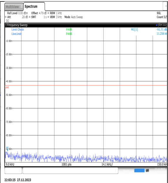
NTNV_N77-3450- 3550_PC2_30_50_H_TID13_NS_01_0.009_0.15_#1
