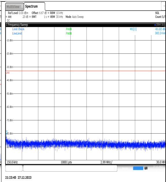
NTNV_N77-3450- 3550_PC2_30_50_H_TID10_NS_01_0.15_30_#1
