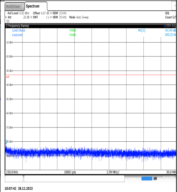
NTNV_N77-3450- 3550_PC2_30_60_L_TID9_NS_01_0.15_30_# 1
