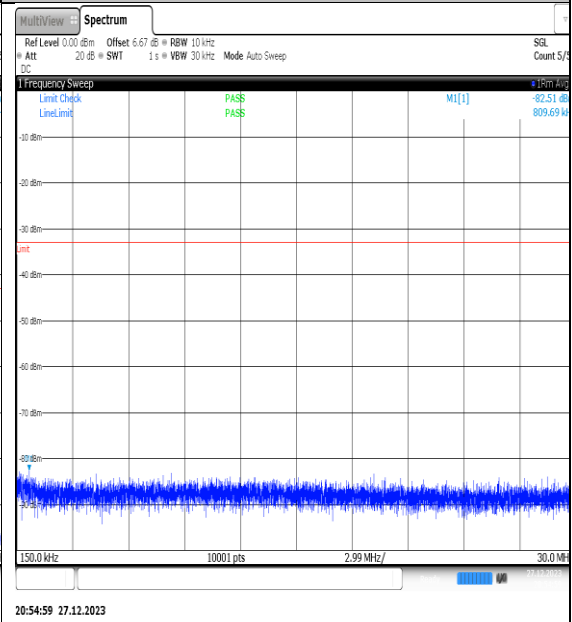
NTNV_N77-3450- 3550_PC2_30_50_H_TID8_NS_01_0.15_30_#1
