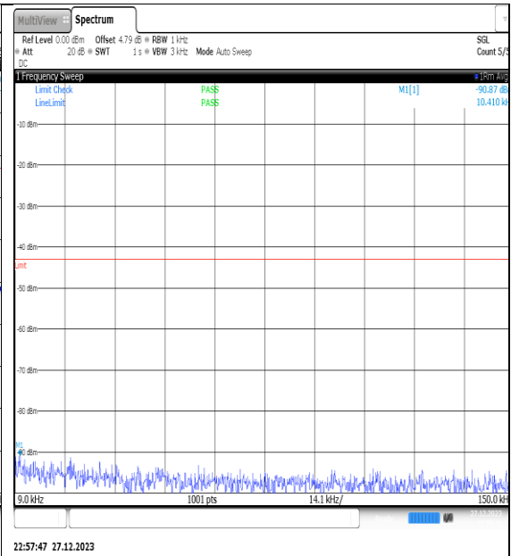
NTNV_N77-3450- 3550_PC2_30_60_L_TID3_NS_01_0.009_0.15_# 1
