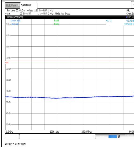
NTNV_N77-3450-3550_PC2_30_50_H_TID15_NS_01_1000_3000_#1
