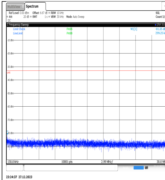
NTNV_N77-3450- 3550_PC2_30_60_L_TID5_NS_01_0.15_30_#1
