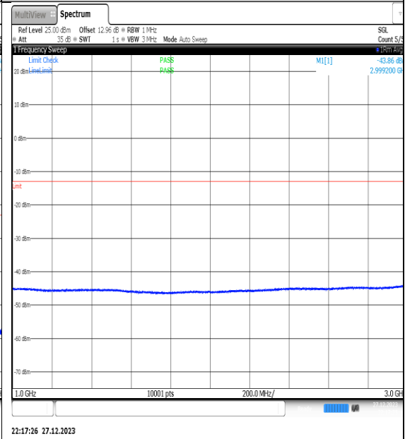
NTNV_N77-3450- 3550_PC2_30_50_H_TID14_NS_01_1000_3000_ #1
