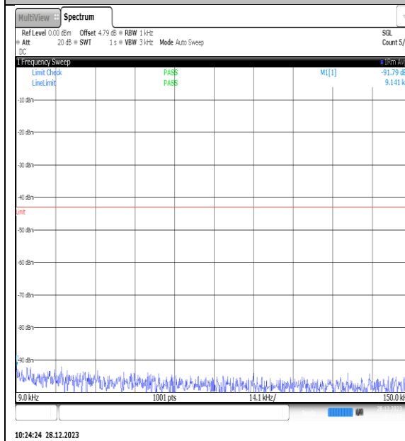
NTNV_N77-3450- 3550_PC2_30_60_L_TID13_NS_01_0.009_0.15_#1
