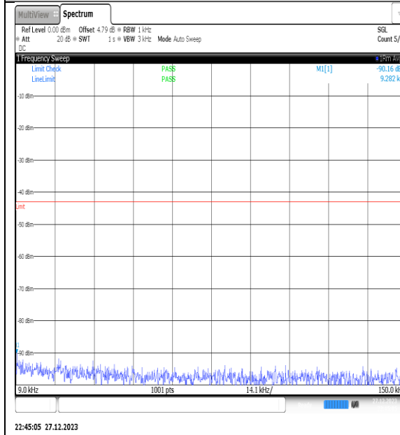
NTNV_N77-3450- 3550_PC2_30_60_L_TID2_NS_01_0.009_0.15_# 1
