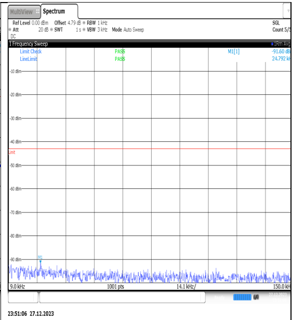
NTNV_N77-3450- 3550_PC2_30_60_L_TID7_NS_01_0.009_0.15_# 1
