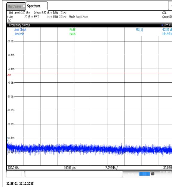
NTNV_N77-3450- 3550_PC2_30_60_L_TID3_NS_01_0.15_30_#1
