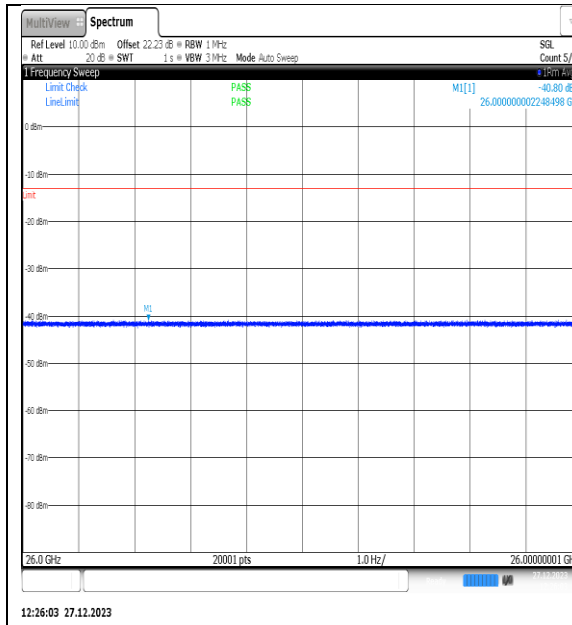
NTNV_N77-3450- 3550_PC2_30_50_H_TID4_NS_01_26000_40000 #1
