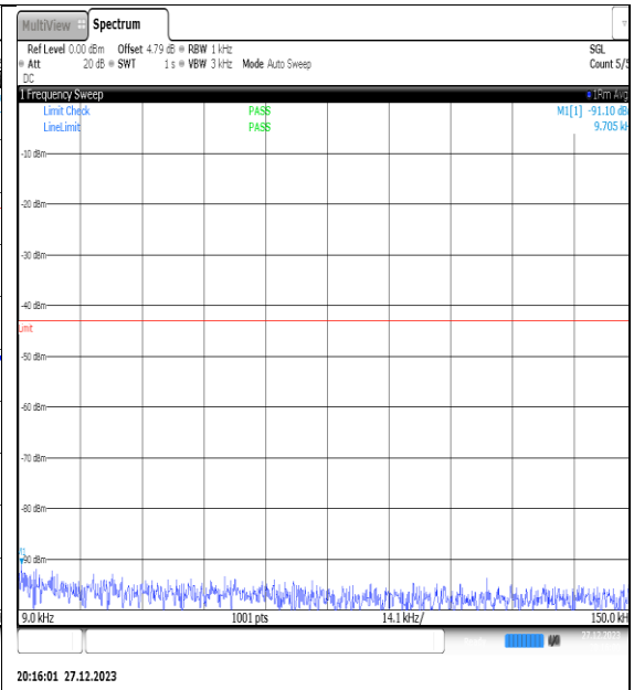
NTNV_N77-3450- 3550_PC2_30_50_H_TID5_NS_01_0.009_0.15_# 1
