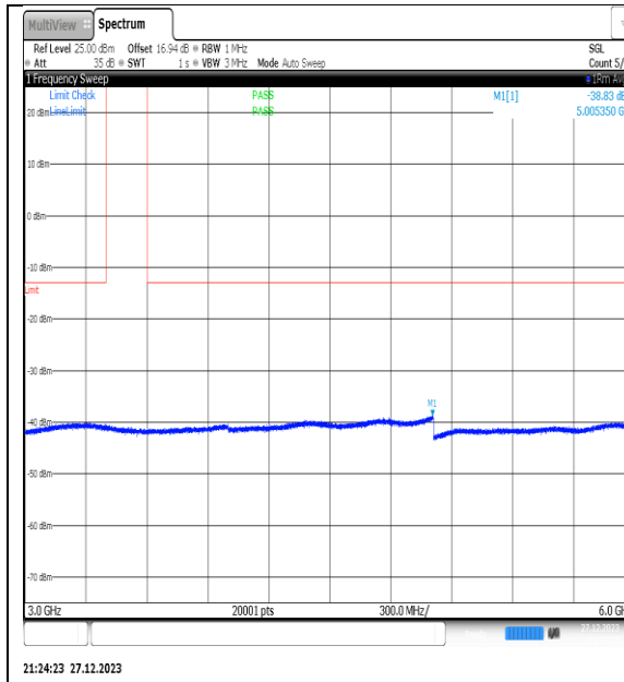
NTNV_N77-3450- 3550_PC2_30_50_H_TID10_NS_01_3000_6000_#1
