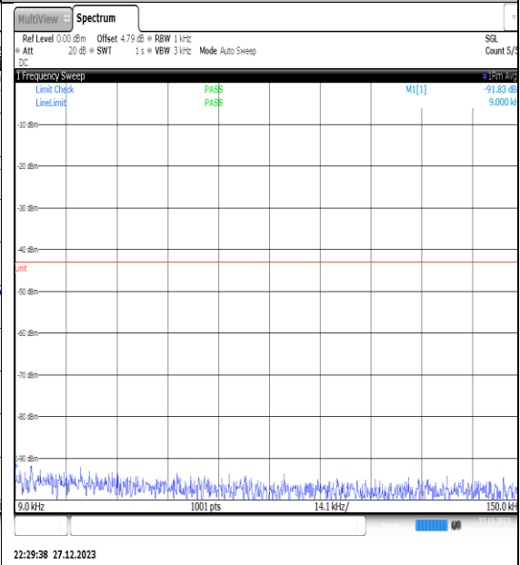
NTNV_N77-3450- 3550_PC2_30_50_H_TID15_NS_01_0.009_0.15_ #1
