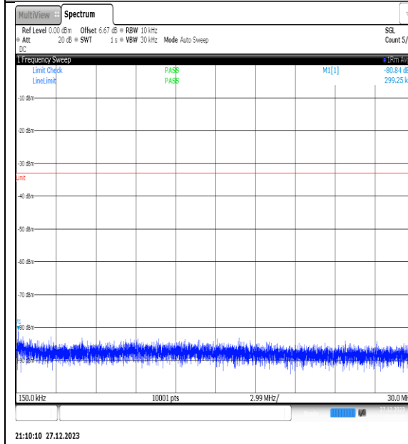
NTNV_N77-3450- 3550_PC2_30_50_H_TID9_NS_01_0.15_30_#1
