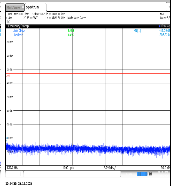
NTNV_N77-3450- 3550_PC2_30_60_L_TID13_NS_01_0.15_30_#1
