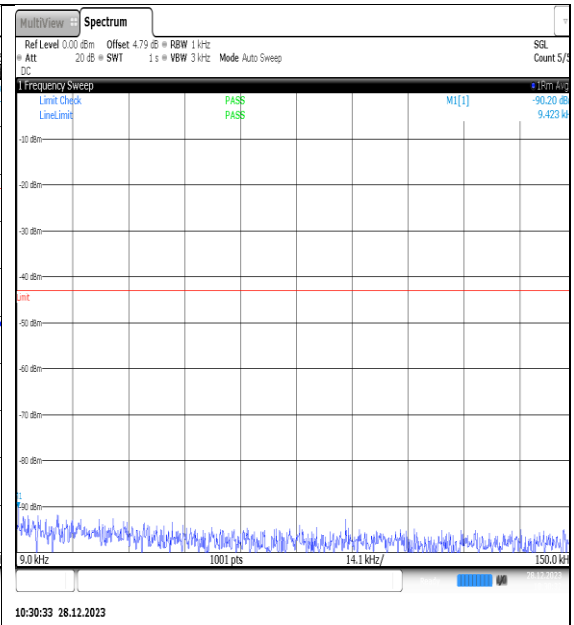
NTNV_N77-3450- 3550_PC2_30_60_L_TID14_NS_01_0.009_0.15_#1
