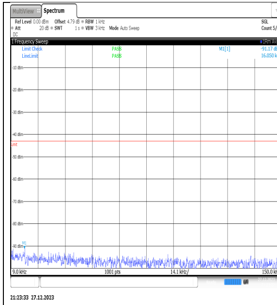
NTNV_N77-3450- 3550_PC2_30_50_H_TID10_NS_01_0.009_0.15_ #1
