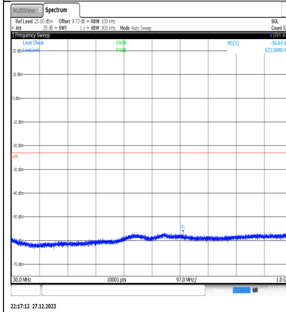
NTNV_N77-3450- 3550_PC2_30_50_H_TID14_NS_01_30_1000_#1
