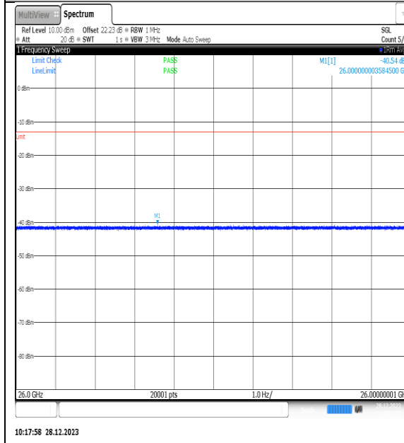
NTNV_N77-3450- 3550_PC2_30_60_L_TID11_NS_01_26000_4000_0_#1
