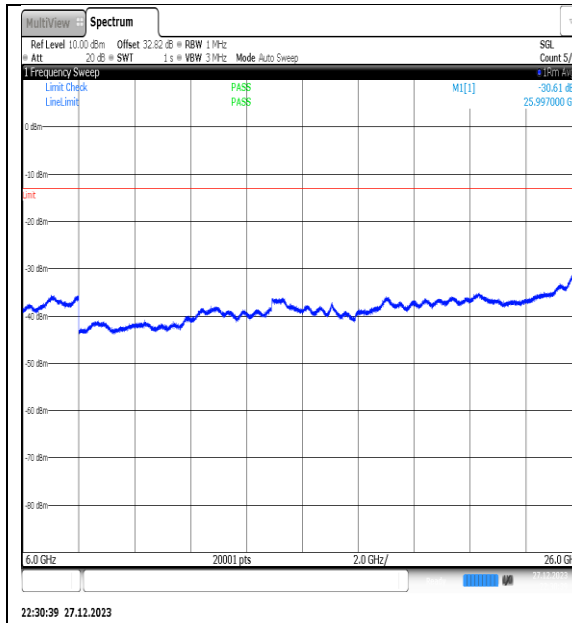
NTNV_N77-3450- 3550_PC2_30_50_H_TID15_NS_01_6000_26000 _#1
