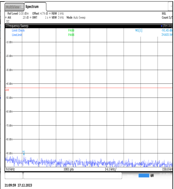
NTNV_N77-3450- 3550_PC2_30_50_H_TID9_NS_01_0.009_0.15_# 1
