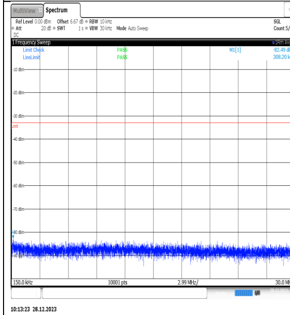
NTNV_N77-3450- 3550_PC2_30_60_L_TID10_NS_01_0.15_30_#1
