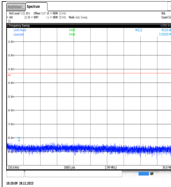
NTNV_N77-3450- 3550_PC2_30_60_L_TID12_NS_01_0.15_30_#1
