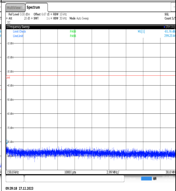
NTNV_N77-3450- 3550_PC2_30_50_L_TID8_NS_01_0.15_30_#1
