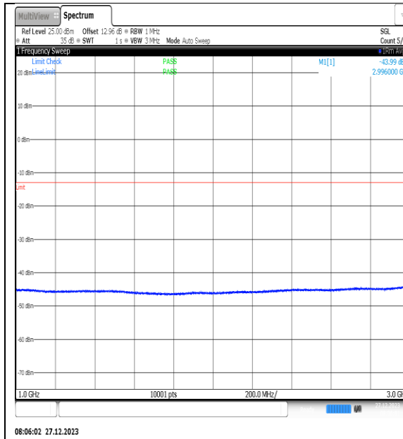
NTNV_N77-3450- 3550_PC2_30_40_H_TID8_NS_01_1000_3000_# 1
