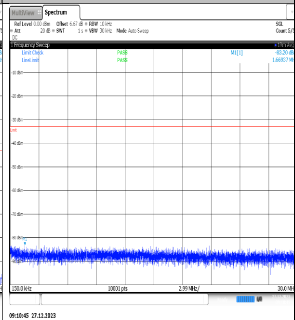
NTNV_N77-3450- 3550_PC2_30_50_L_TID4_NS_01_0.15_30_#1
