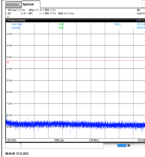
NTNV_N77-3450- 3550_PC2_30_40_H_TID8_NS_01_0.15_30_#1
