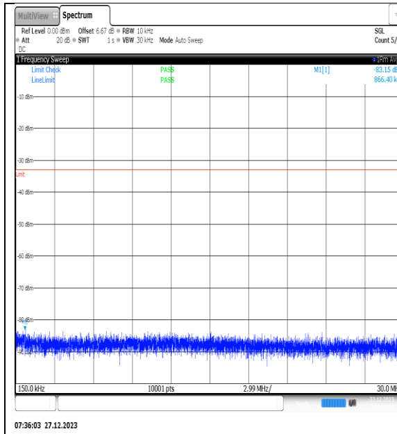
NTNV_N77-3450-3550_PC2_30_40_H_TID2_NS_01_0.15_30_#1
