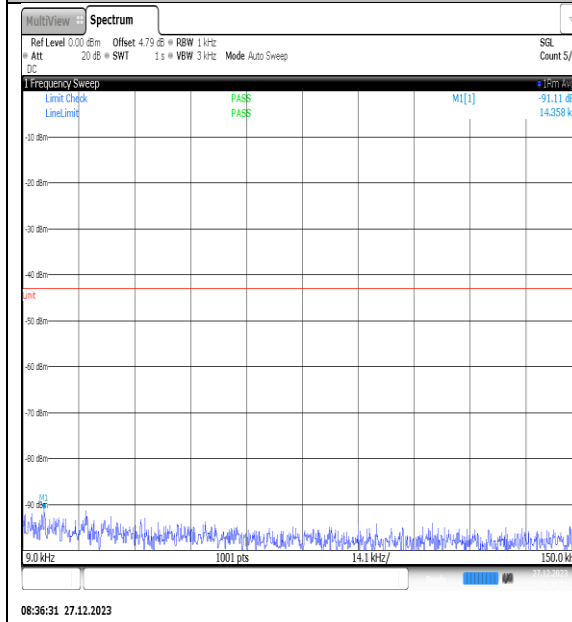
NTNV_N77-3450- 3550_PC2_30_40_H_TID15_NS_01_0.009_0.15_#1
