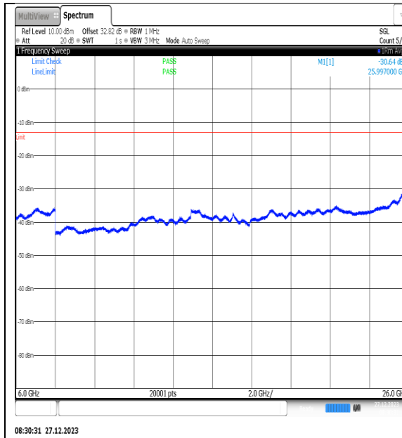
NTNV_N77-3450- 3550_PC2_30_40_H_TID14_NS_01_6000_26000 _#1
