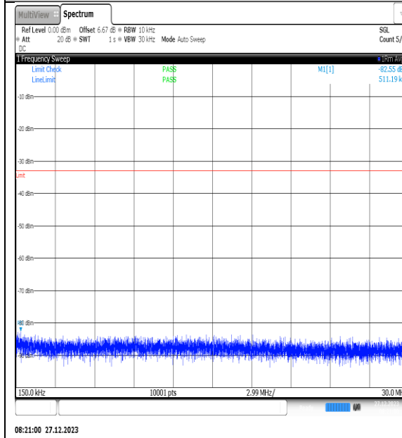
NTNV_N77-3450- 3550_PC2_30_40_H_TID12_NS_01_0.15_30_#1
