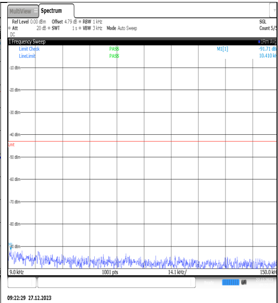
NTNV_N77-3450- 3550_PC2_30_50_L_TID5_NS_01_0.009_0.15_# 1
