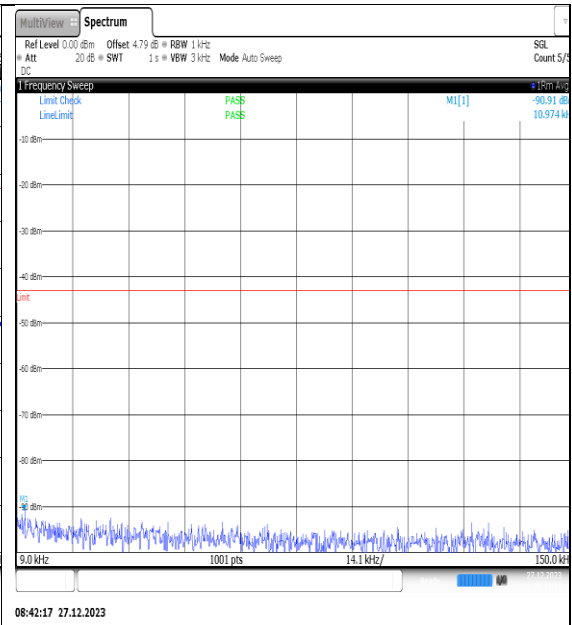
NTNV_N77-3450- 3550_PC2_30_50_L_TID1_NS_01_0.009_0.15_# 1
