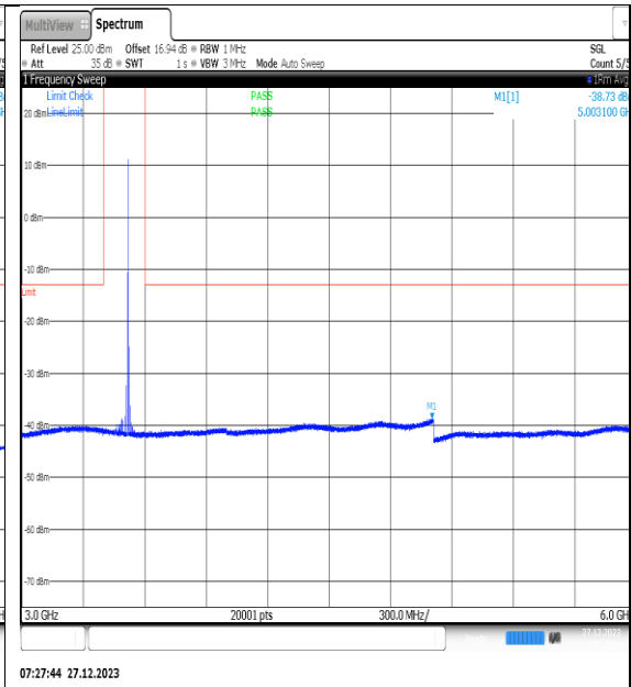
NTNV_N77-3450- 3550_PC2_30_40_M_TID15_NS_01_3000_6000_ #1
