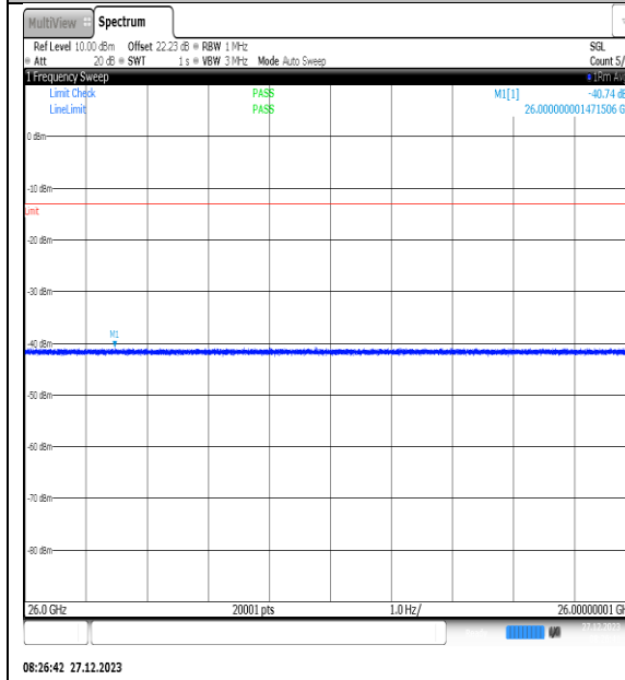
NTNV_N77-3450- 3550_PC2_30_40_H_TID13_NS_01_26000_4000_ 0_#1
