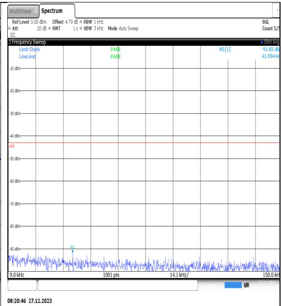
NTNV_N77-3450- 3550_PC2_30_40_H_TID12_NS_01_0.009_0.15_ #1
