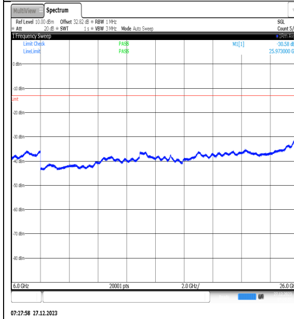
NTNV_N77-3450- 3550_PC2_30_40_M_TID15_NS_01_6000_26000_ #1
