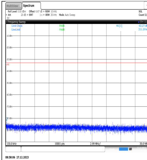
NTNV_N77-3450- 3550_PC2_30_50_L_TID3_NS_01_0.15_30_#1
