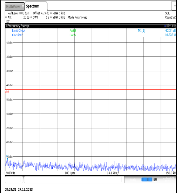
NTNV_N77-3450- 3550_PC2_30_40_H_TID14_NS_01_0.009_0.15_ #1
