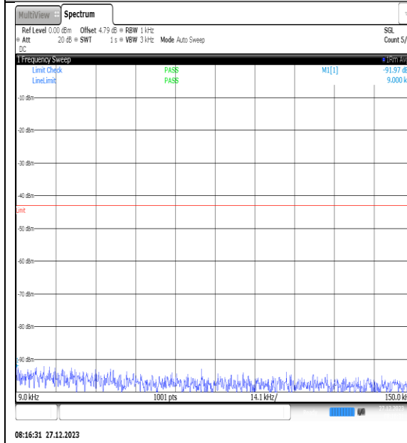
NTNV_N77-3450- 3550_PC2_30_40_H_TID11_NS_01_0.009_0.15_#1
