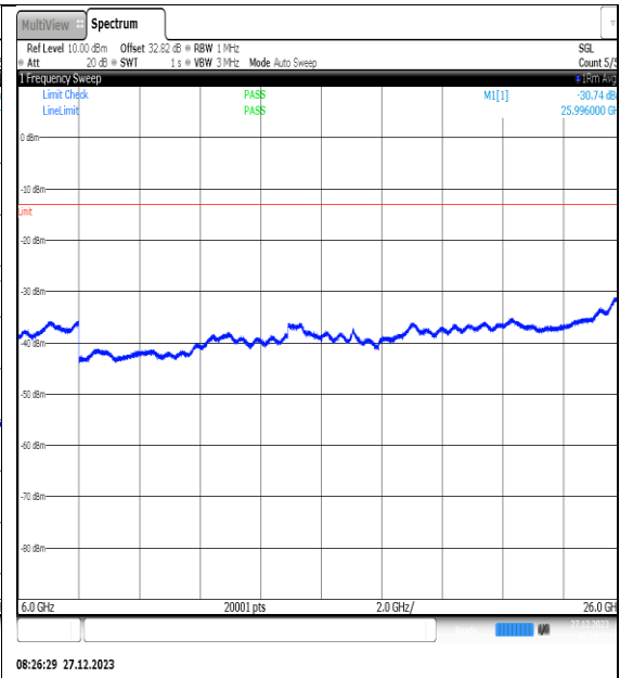
NTNV_N77-3450- 3550_PC2_30_40_H_TID13_NS_01_6000_26000_ #1
