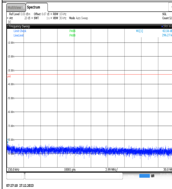
NTNV_N77-3450- 3550_PC2_30_40_M_TID15_NS_01_0.15_30_#1
