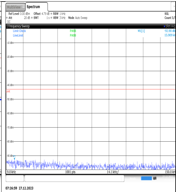
NTNV_N77-3450- 3550_PC2_30_40_M_TID15_NS_01_0.009_0.15_ #1
