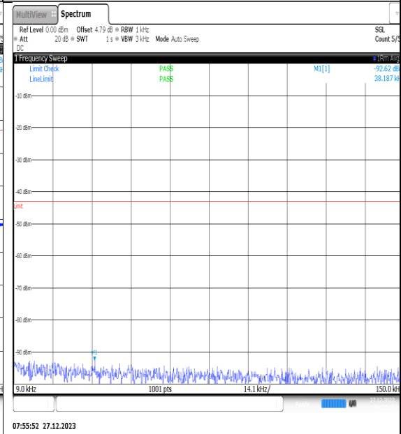
NTNV_N77-3450- 3550_PC2_30_40_H_TID6_NS_01_0.009_0.15_# 1
