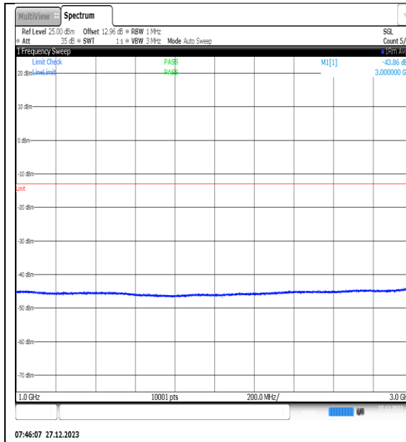
NTNV_N77-3450- 3550_PC2_30_40_H_TID4_NS_01_1000_3000_# 1
