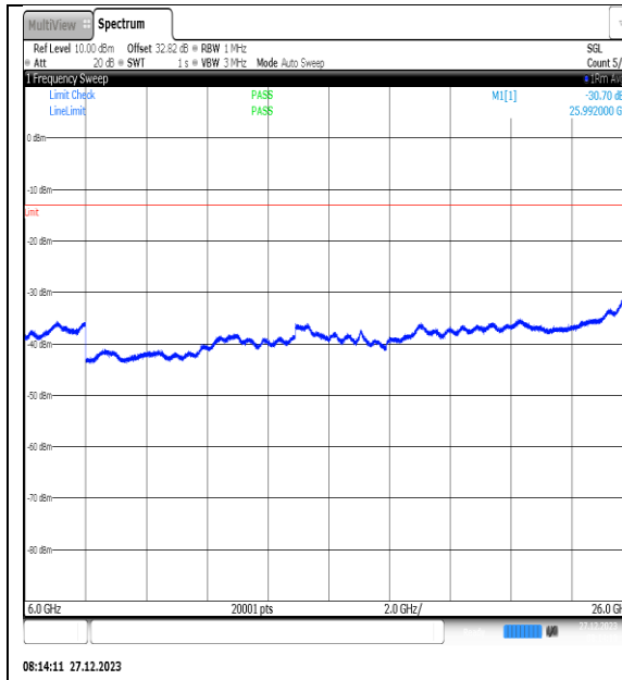
NTNV_N77-3450- 3550_PC2_30_40_H_TID10_NS_01_6000_26000 _#1
