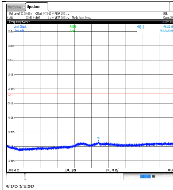
NTNV_N77-3450- 3550_PC2_30_40_M_TID14_NS_01_30_1000_#1
