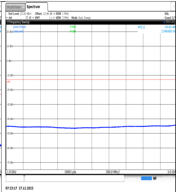
NTNV_N77-3450- 3550_PC2_30_40_M_TID14_NS_01_1000_3000_#1
