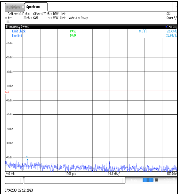
NTNV_N77-3450- 3550_PC2_30_40_H_TID4_NS_01_0.009_0.15_# 1
