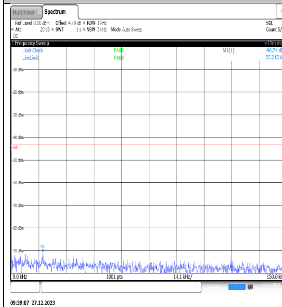
NTNV_N77-3450- 3550_PC2_30_50_L_TID8_NS_01_0.009_0.15_# 1
