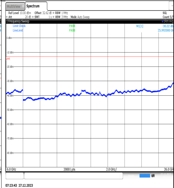
NTNV_N77-3450- 3550_PC2_30_40_M_TID14_NS_01_6000_26000_#1
