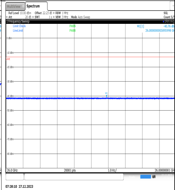
NTNV_N77-3450- 3550_PC2_30_40_M_TID15_NS_01_26000_4000 0_#1
