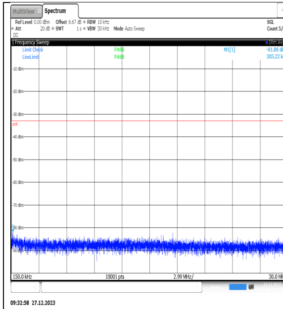
NTNV_N77-3450-3550_PC2_30_50_L_TID7_NS_01_0.15_30_#1
