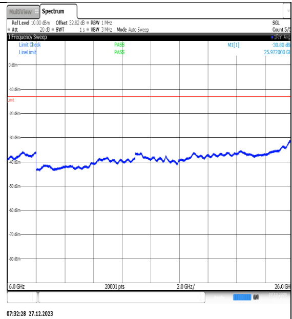
NTNV_N77-3450- 3550_PC2_30_40_H_TID1_NS_01_6000_26000_# 1
