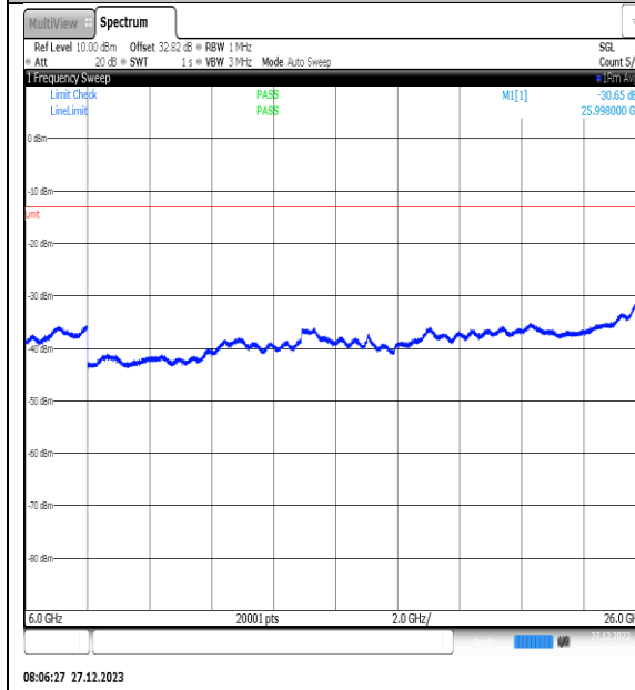
NTNV_N77-3450- 3550_PC2_30_40_H_TID8_NS_01_6000_26000_# 1
