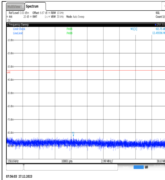
NTNV_N77-3450- 3550_PC2_30_40_H_TID6_NS_01_0.15_30_#1
