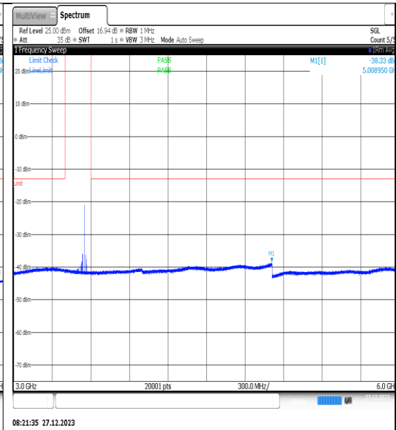
NTNV_N77-3450- 3550_PC2_30_40_H_TID12_NS_01_3000_6000_ #1
