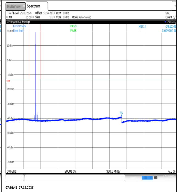
NTNV_N77-3450-3550_PC2_30_40_H_TID2_NS_01_3000_6000_#1
