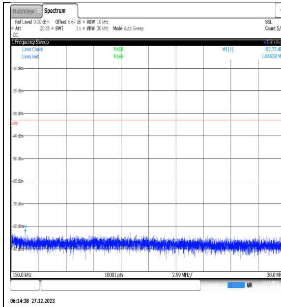
NTNV_N77-3450- 3550_PC2_30_40_M_TID1_NS_01_0.15_30_#1
