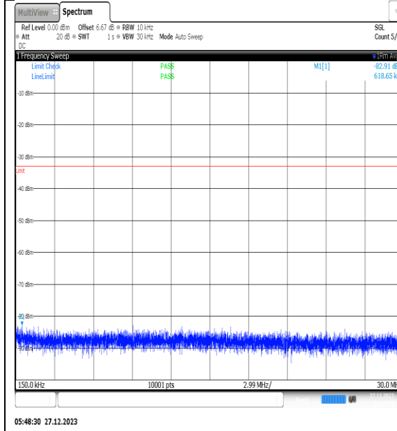
NTNV_N77-3450- 3550_PC2_30_40_L_TID10_NS_01_0.15_30_#1
