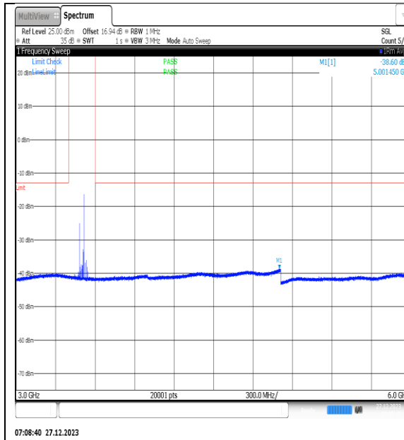
NTNV_N77-3450- 3550_PC2_30_40_M_TID12_NS_01_3000_6000_ #1
