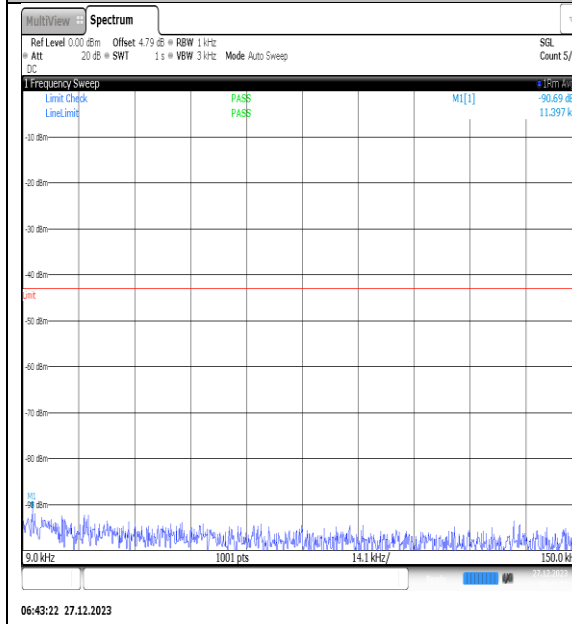
NTNV_N77-3450- 3550_PC2_30_40_M_TID6_NS_01_0.009_0.15_#1
