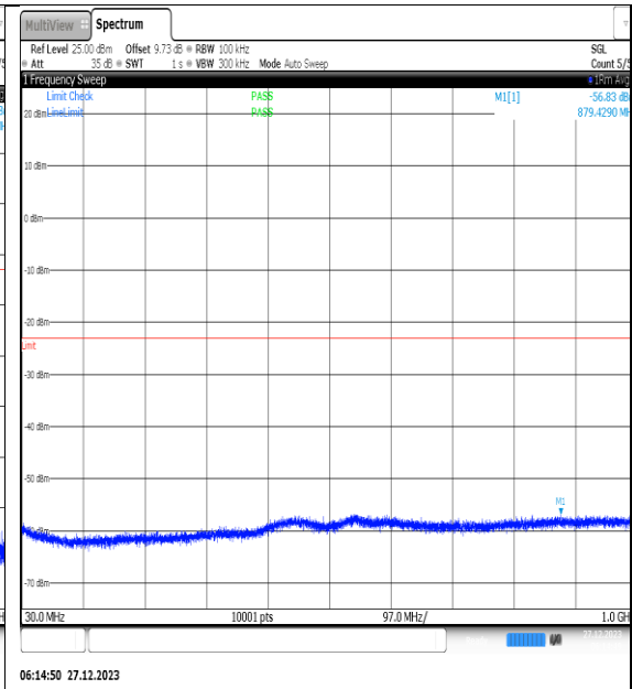
NTNV_N77-3450- 3550_PC2_30_40_M_TID1_NS_01_30_1000_#1
