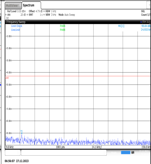
NTNV_N77-3450- 3550_PC2_30_40_M_TID9_NS_01_0.009_0.15_# 1
