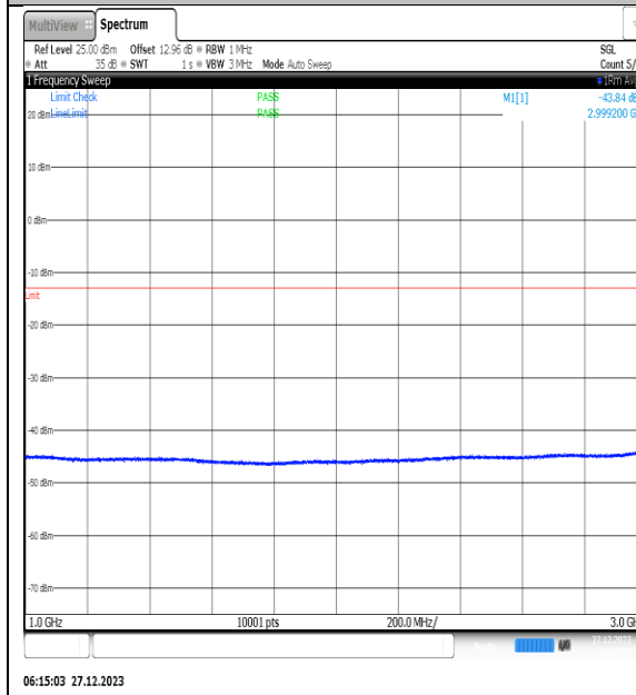
NTNV_N77-3450- 3550_PC2_30_40_M_TID1_NS_01_1000_3000_# 1
