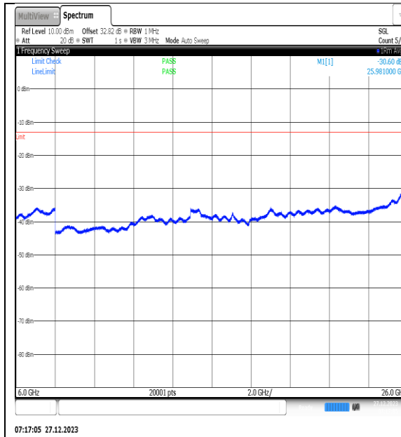
NTNV_N77-3450- 3550_PC2_30_40_M_TID13_NS_01_6000_26000 _#1
