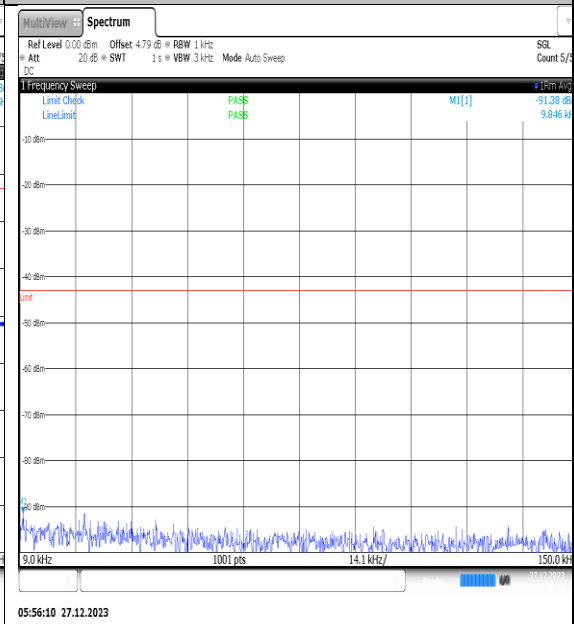
NTNV_N77-3450- 3550_PC2_30_40_L_TID12_NS_01_0.009_0.15_ #1
