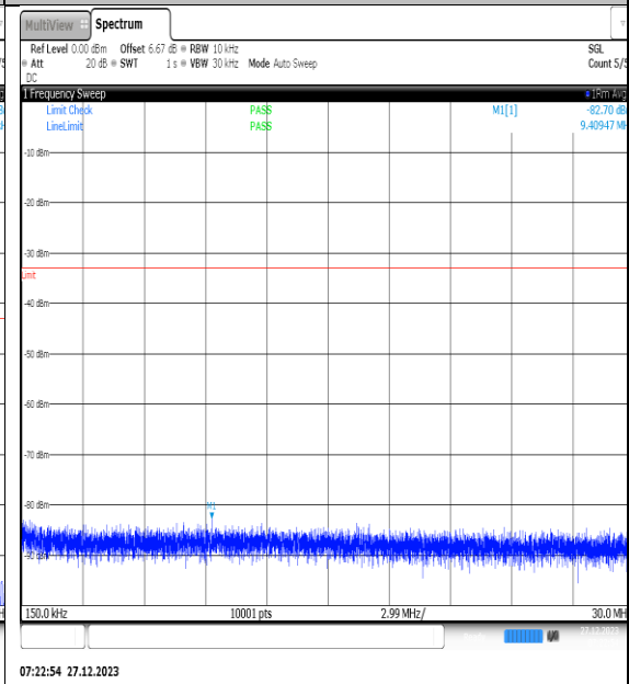
NTNV_N77-3450- 3550_PC2_30_40_M_TID14_NS_01_0.15_30_#1
