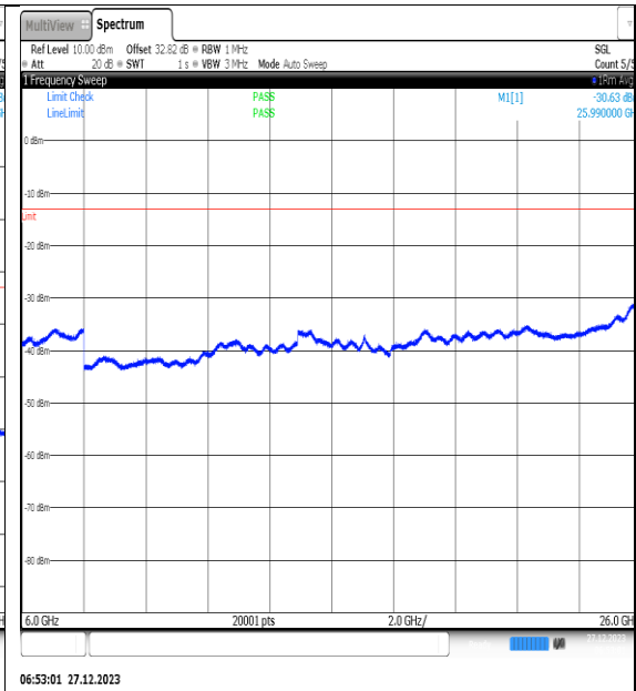
NTNV_N77-3450- 3550_PC2_30_40_M_TID8_NS_01_6000_26000_# 1
