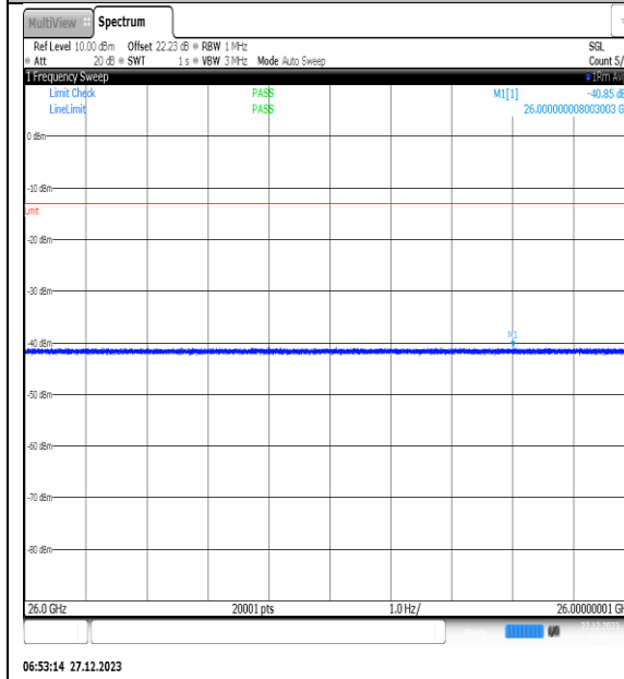
NTNV_N77-3450- 3550_PC2_30_40_M_TID8_NS_01_26000_40000_# 1
