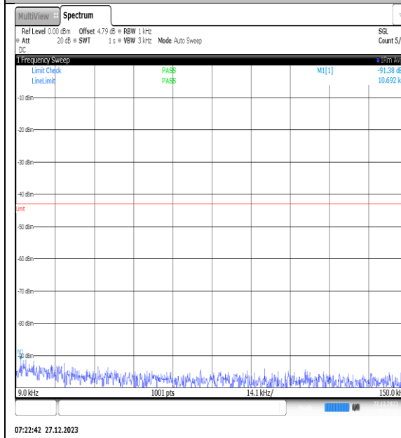
NTNV_N77-3450- 3550_PC2_30_40_M_TID14_NS_01_0.009_0.15_#1
