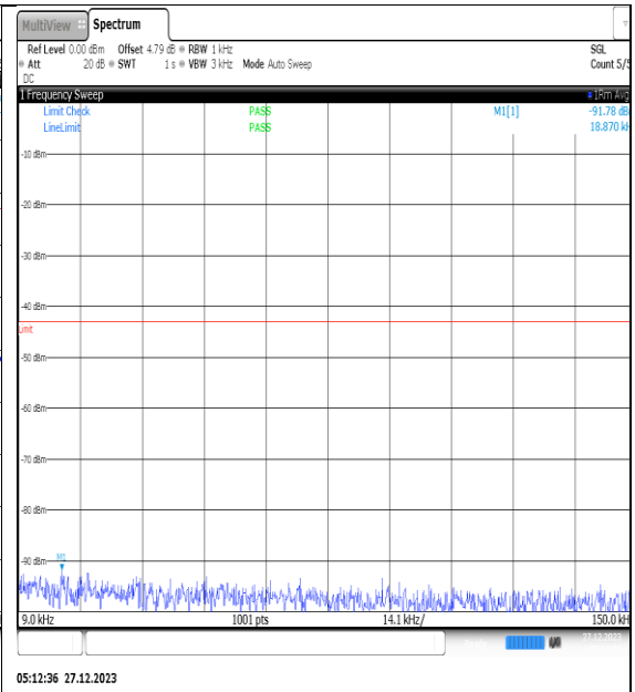
NTNV_N77-3450- 3550_PC2_30_40_L_TID6_NS_01_0.009_0.15_# 1
