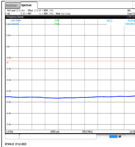
NTNV_N77-3450- 3550_PC2_30_40_M_TID11_NS_01_1000_3000_ #1
