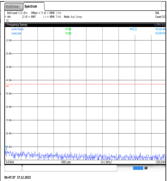
NTNV_N77-3450- 3550_PC2_30_40_M_TID7_NS_01_0.009_0.15_# 1
