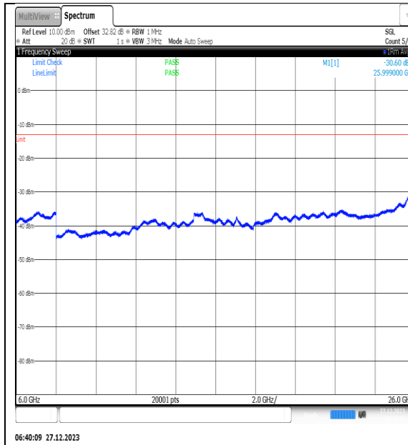
NTNV_N77-3450- 3550_PC2_30_40_M_TID5_NS_01_6000_26000_#1
