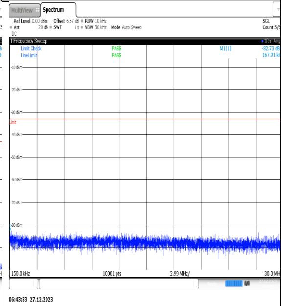
NTNV_N77-3450- 3550_PC2_30_40_M_TID6_NS_01_0.15_30_#1
