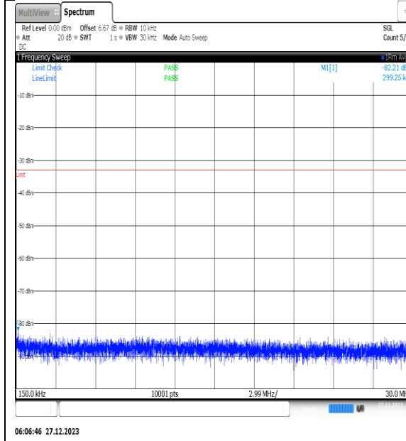
NTNV_N77-3450- 3550_PC2_30_40_L_TID14_NS_01_0.15_30_#1
