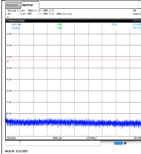
NTNV_N77-3450- 3550_PC2_30_40_M_TID3_NS_01_0.15_30_#1
