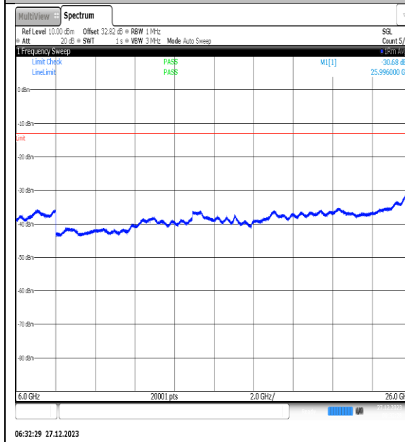
NTNV_N77-3450- 3550_PC2_30_40_M_TID3_NS_01_6000_26000_# 1
