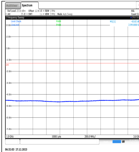
NTNV_N77-3450- 3550_PC2_30_40_M_TID3_NS_01_1000_3000_# 1
