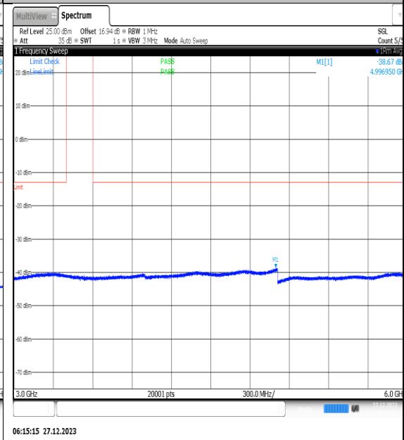
NTNV_N77-3450- 3550_PC2_30_40_M_TID1_NS_01_3000_6000_# 1
