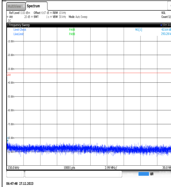
NTNV_N77-3450- 3550_PC2_30_40_M_TID7_NS_01_0.15_30_#1
