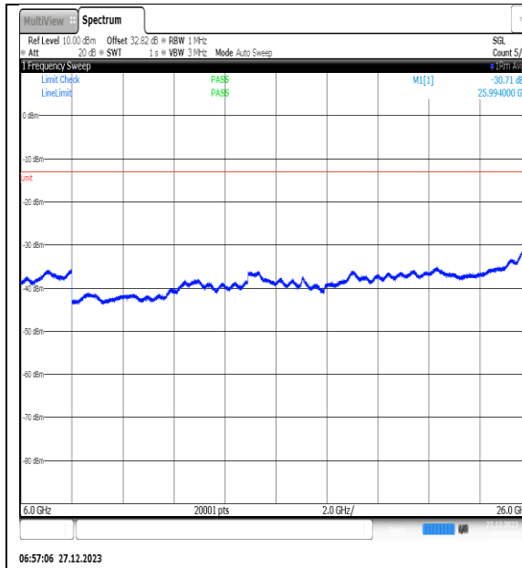
NTNV_N77-3450- 3550_PC2_30_40_M_TID9_NS_01_6000_26000_#1
