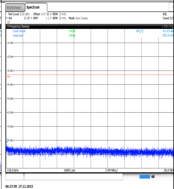
NTNV_N77-3450- 3550_PC2_30_40_M_TID2_NS_01_0.15_30_#1
