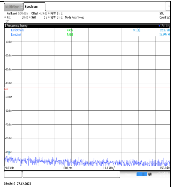
NTNV_N77-3450- 3550_PC2_30_40_L_TID10_NS_01_0.009_0.15_ #1
