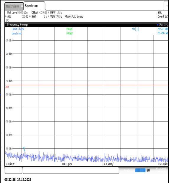
NTNV_N77-3450- 3550_PC2_30_40_L_TID8_NS_01_0.009_0.15_# 1
