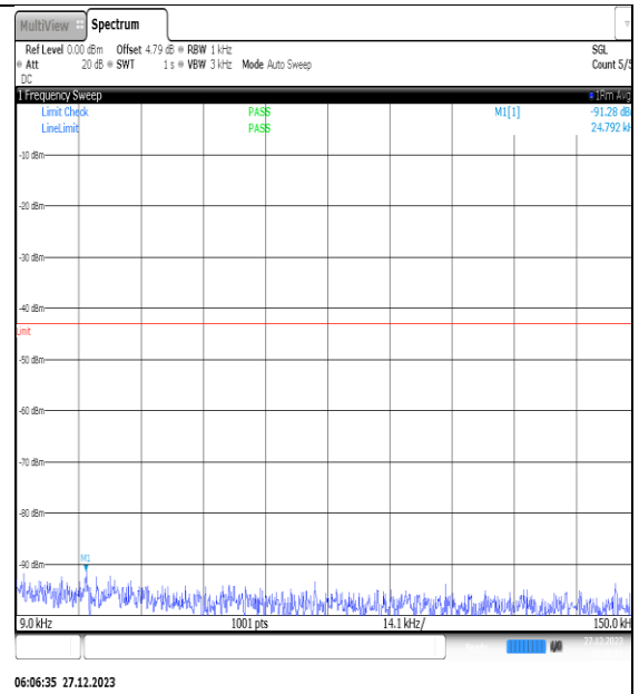
NTNV_N77-3450- 3550_PC2_30_40_L_TID14_NS_01_0.009_0.15_#1
