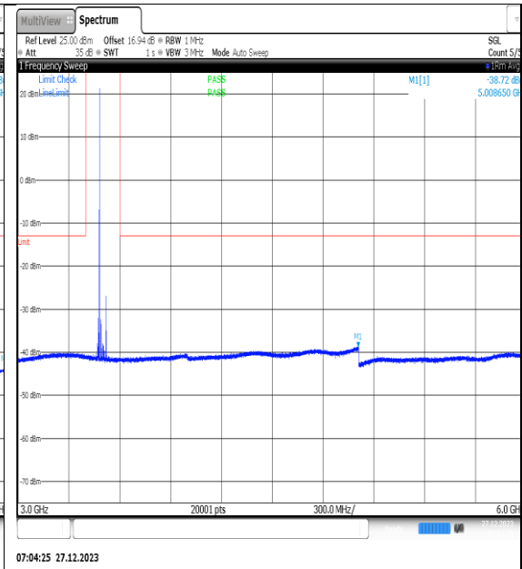
NTNV_N77-3450- 3550_PC2_30_40_M_TID11_NS_01_3000_6000_ #1
