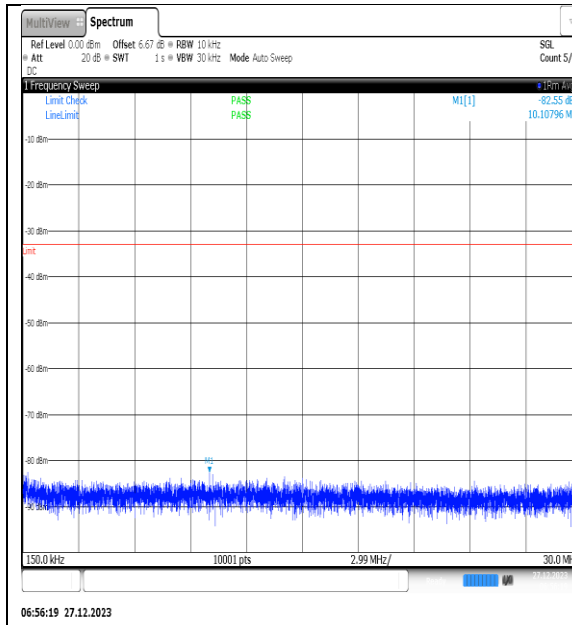
NTNV_N77-3450- 3550_PC2_30_40_M_TID9_NS_01_0.15_30_#1
