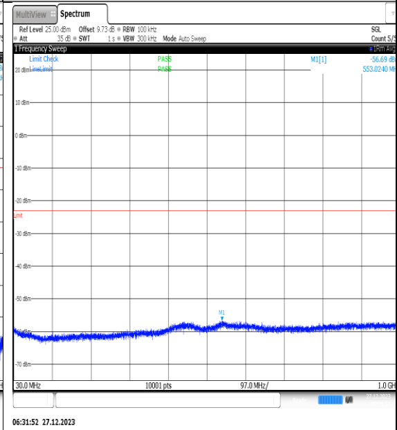
NTNV_N77-3450- 3550_PC2_30_40_M_TID3_NS_01_30_1000_#1
