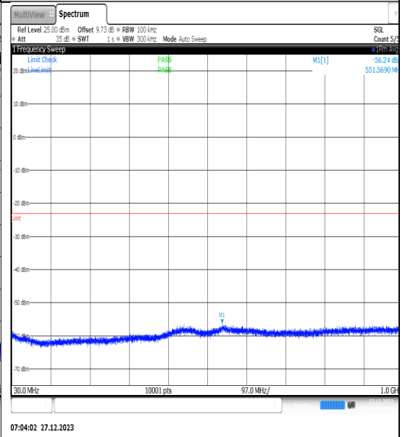
NTNV_N77-3450- 3550_PC2_30_40_M_TID11_NS_01_30_1000_#1
