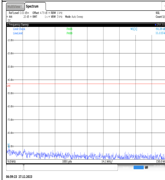
NTNV_N77-3450- 3550_PC2_30_40_M_TID10_NS_01_0.009_0.15_#1
