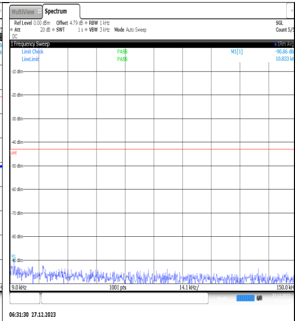
NTNV_N77-3450- 3550_PC2_30_40_M_TID3_NS_01_0.009_0.15_# 1
