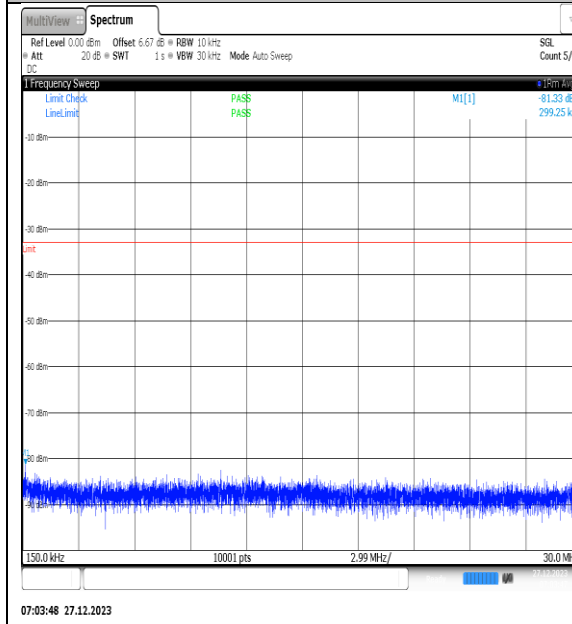
NTNV_N77-3450- 3550_PC2_30_40_M_TID11_NS_01_0.15_30_#1
