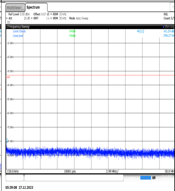
NTNV_N77-3450- 3550_PC2_30_40_L_TID9_NS_01_0.15_30_#1
