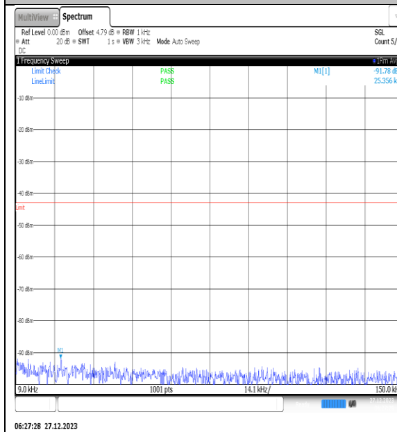
NTNV_N77-3450- 3550_PC2_30_40_M_TID2_NS_01_0.009_0.15_#1
