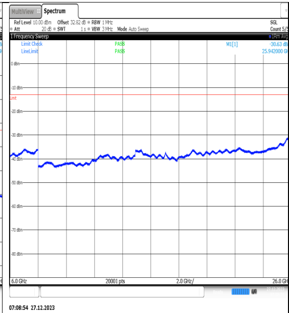
NTNV_N77-3450- 3550_PC2_30_40_M_TID12_NS_01_6000_26000 _#1
