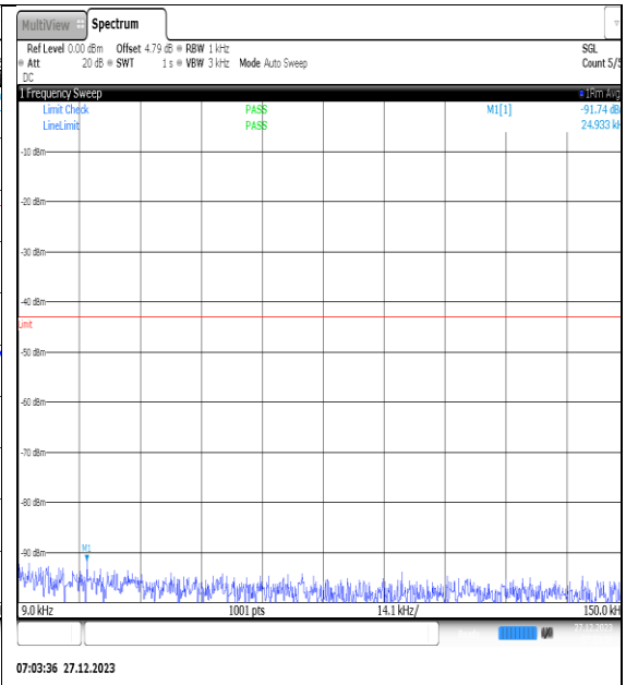
NTNV_N77-3450- 3550_PC2_30_40_M_TID11_NS_01_0.009_0.15_ #1
