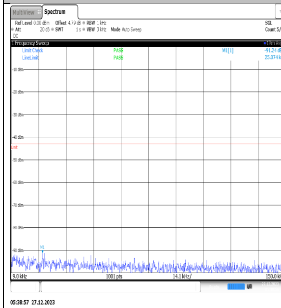
NTNV_N77-3450- 3550_PC2_30_40_L_TID9_NS_01_0.009_0.15_#1
