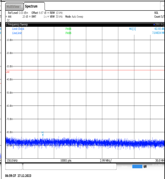
NTNV_N77-3450- 3550_PC2_30_40_M_TID10_NS_01_0.15_30_#1
