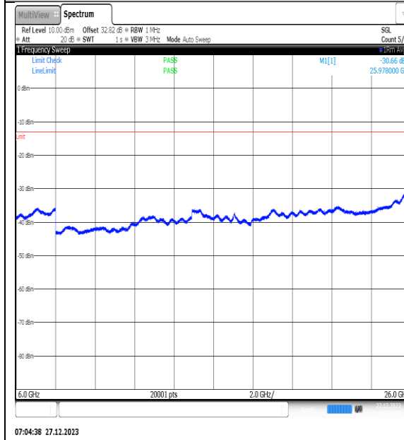
NTNV_N77-3450- 3550_PC2_30_40_M_TID11_NS_01_6000_26000 _#1
