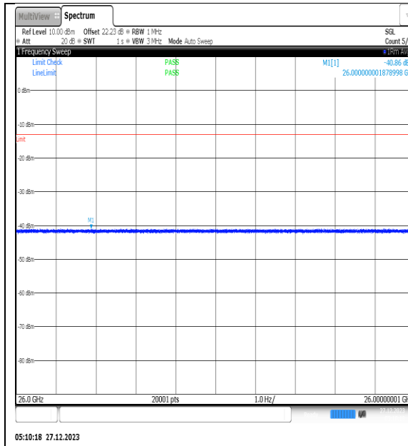
NTNV_N77-3450- 3550_PC2_30_40_L_TID5_NS_01_26000_40000 #1
