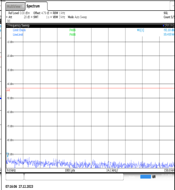
NTNV_N77-3450- 3550_PC2_30_40_M_TID13_NS_01_0.009_0.15_ #1
