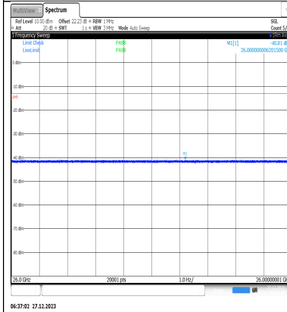
NTNV_N77-3450- 3550_PC2_30_40_M_TID4_NS_01_26000_40000_# 1
