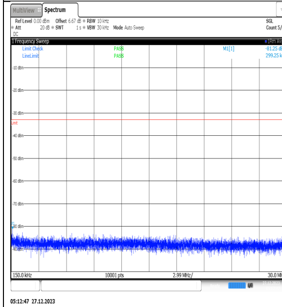
NTNV_N77-3450- 3550_PC2_30_40_L_TID6_NS_01_0.15_30_#1
