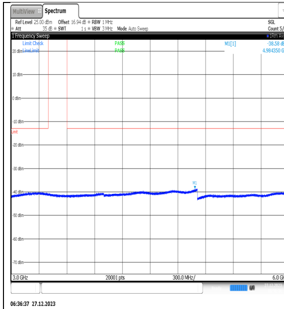
NTNV_N77-3450- 3550_PC2_30_40_M_TID4_NS_01_3000_6000_# 1
