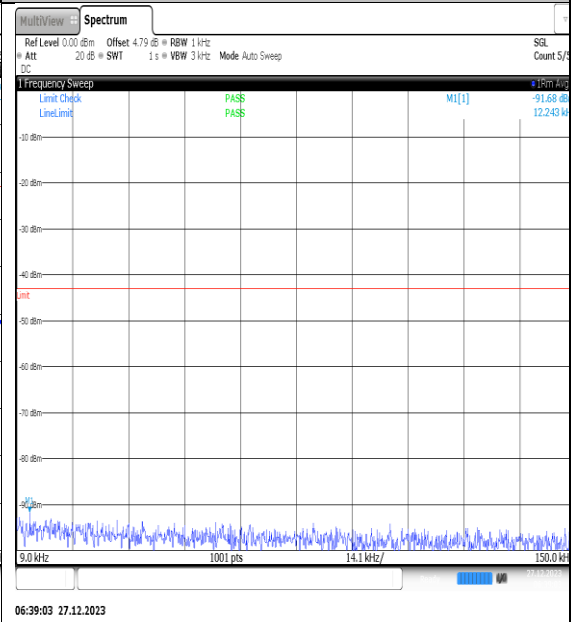
NTNV_N77-3450- 3550_PC2_30_40_M_TID5_NS_01_0.009_0.15_# 1
