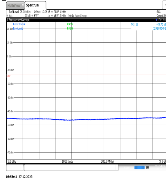
NTNV_N77-3450- 3550_PC2_30_40_M_TID9_NS_01_1000_3000_# 1
