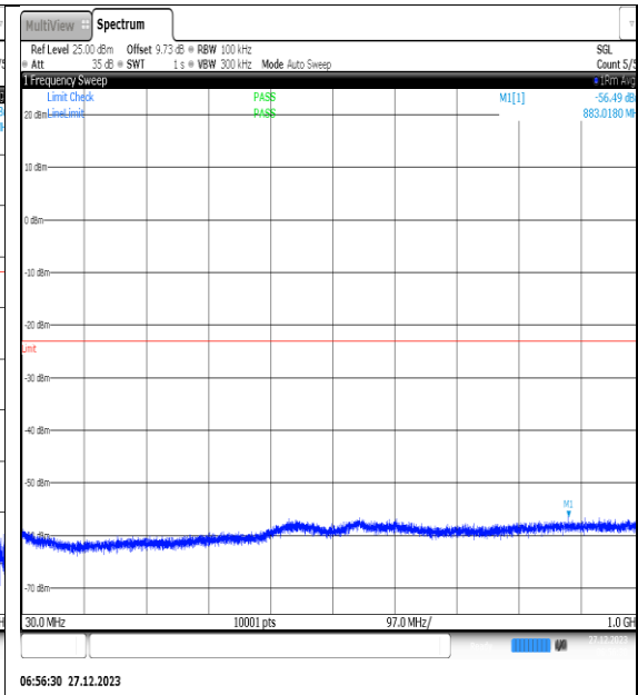
NTNV_N77-3450- 3550_PC2_30_40_M_TID9_NS_01_30_1000_#1
