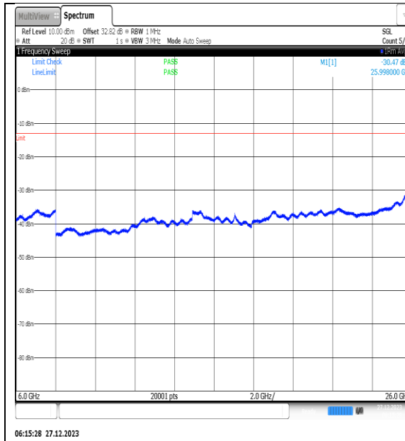
NTNV_N77-3450- 3550_PC2_30_40_M_TID1_NS_01_6000_26000_#1
