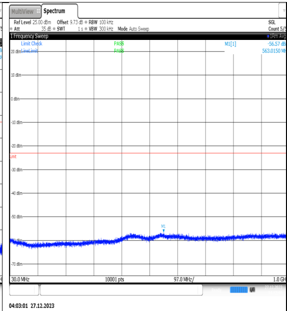
NTNV_N77-3450- 3550_PC2_30_30_H_TID7_NS_01_30_1000_#1
