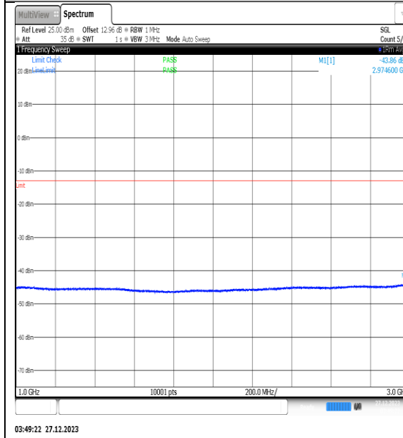
NTNV_N77-3450- 3550_PC2_30_30_H_TID3_NS_01_1000_3000_#1
