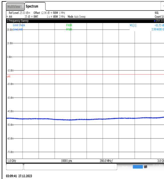
NTNV_N77-3450- 3550_PC2_30_30_M_TID12_NS_01_1000_3000_ #1
