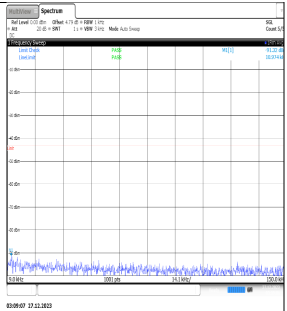
NTNV_N77-3450- 3550_PC2_30_30_M_TID12_NS_01_0.009_0.15_ #1
