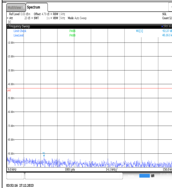
NTNV_N77-3450- 3550_PC2_30_30_H_TID4_NS_01_0.009_0.15_# 1
