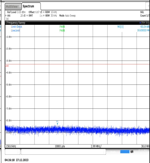
NTNV_N77-3450- 3550_PC2_30_30_H_TID12_NS_01_0.15_30_#1
