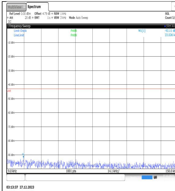
NTNV_N77-3450- 3550_PC2_30_30_M_TID13_NS_01_0.009_0.15_ #1
