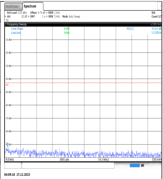
NTNV_N77-3450- 3550_PC2_30_30_H_TID9_NS_01_0.009_0.15_# 1
