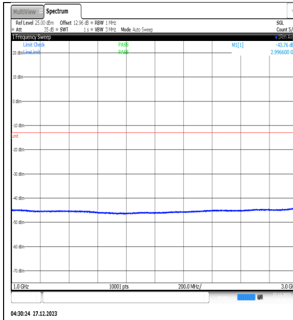
NTNV_N77-3450- 3550_PC2_30_30_H_TID13_NS_01_1000_3000_ #1
