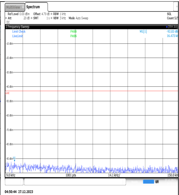
NTNV_N77-3450- 3550_PC2_30_40_L_TID2_NS_01_0.009_0.15_# 1
