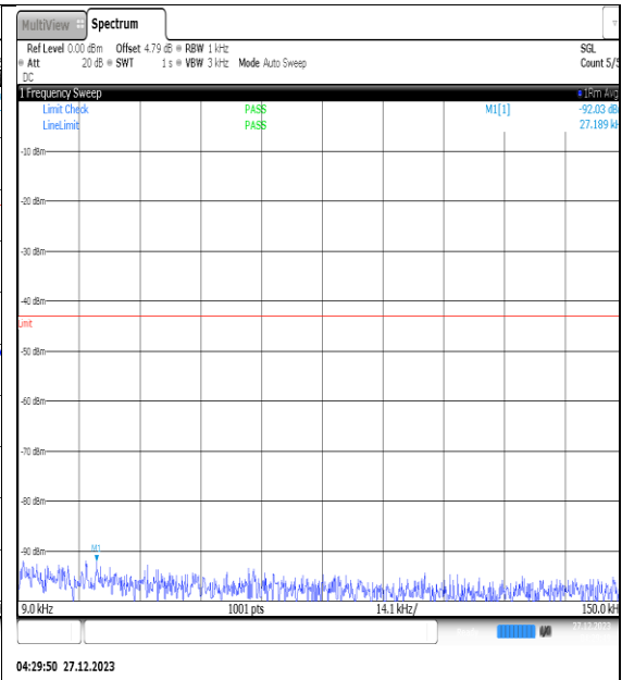
NTNV_N77-3450- 3550_PC2_30_30_H_TID13_NS_01_0.009_0.15_ #1
