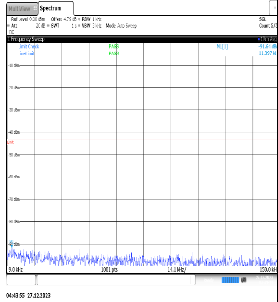
NTNV_N77-3450- 3550_PC2_30_30_H_TID15_NS_01_0.009_0.15_#1
