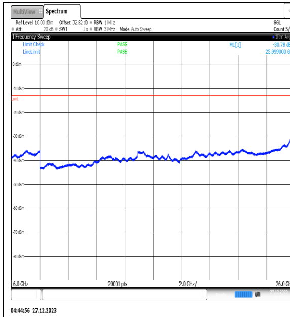
NTNV_N77-3450- 3550_PC2_30_30_H_TID15_NS_01_6000_26000 _#1
