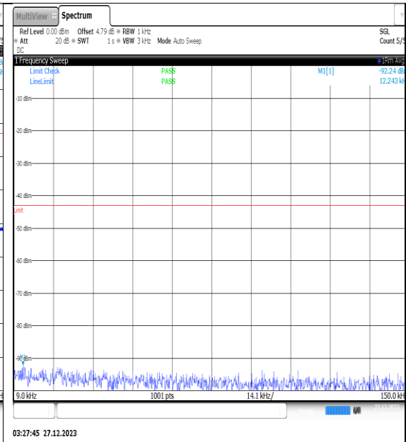
NTNV_N77-3450- 3550_PC2_30_30_H_TID1_NS_01_0.009_0.15_# 1
