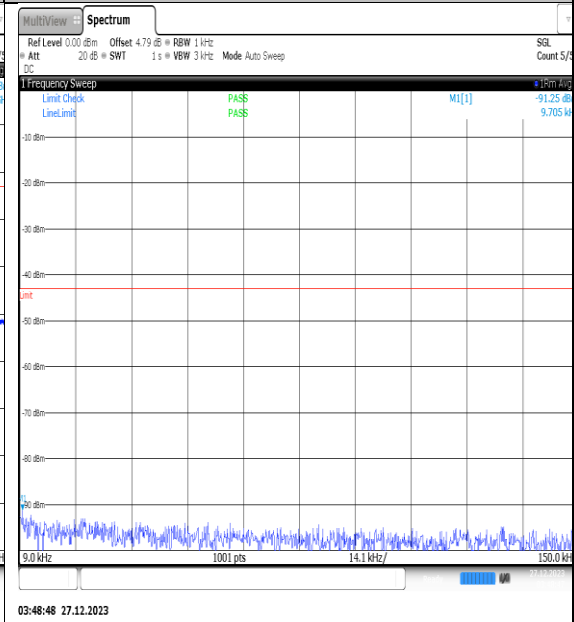
NTNV_N77-3450- 3550_PC2_30_30_H_TID3_NS_01_0.009_0.15_# 1
