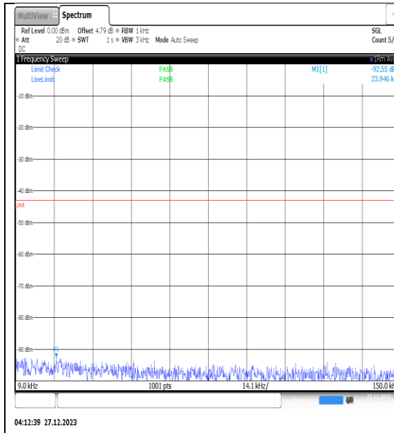
NTNV_N77-3450- 3550_PC2_30_30_H_TID10_NS_01_0.009_0.15_#1
