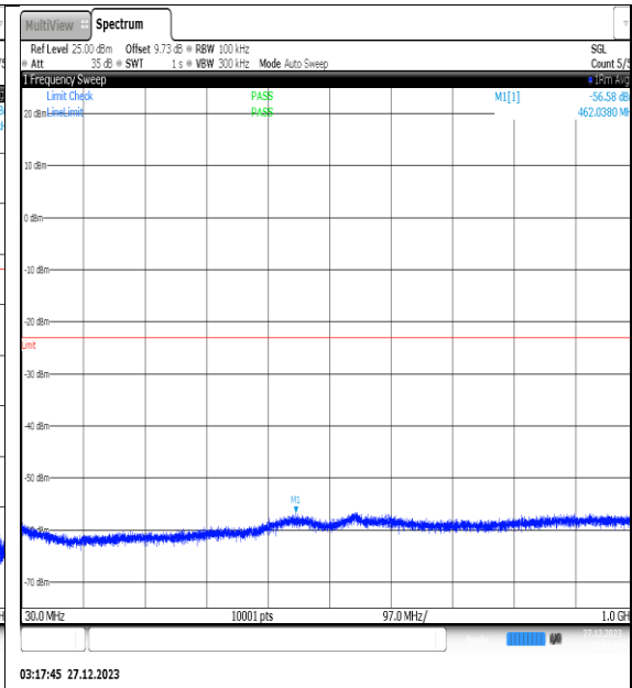
NTNV_N77-3450- 3550_PC2_30_30_M_TID14_NS_01_30_1000_#1
