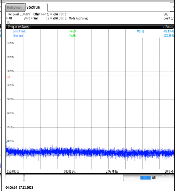
NTNV_N77-3450- 3550_PC2_30_30_H_TID8_NS_01_0.15_30_#1
