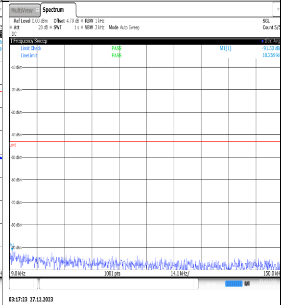
NTNV_N77-3450- 3550_PC2_30_30_M_TID14_NS_01_0.009_0.15_#1
