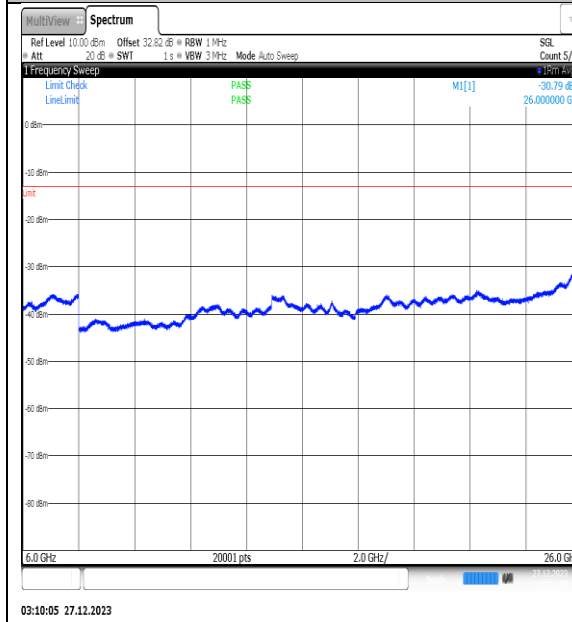
NTNV_N77-3450- 3550_PC2_30_30_M_TID12_NS_01_6000_26000_ #1
