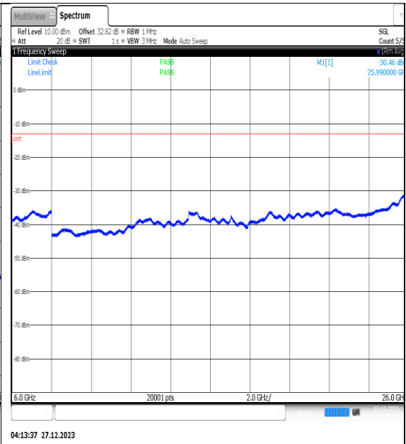
NTNV_N77-3450- 3550_PC2_30_30_H_TID10_NS_01_6000_26000_#1
