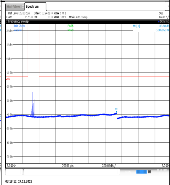
NTNV_N77-3450- 3550_PC2_30_30_M_TID14_NS_01_3000_6000_#1
