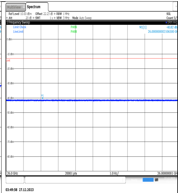
NTNV_N77-3450- 3550_PC2_30_30_H_TID3_NS_01_26000_40000 _#1
