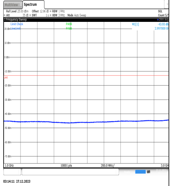
NTNV_N77-3450- 3550_PC2_30_30_M_TID13_NS_01_1000_3000_ #1
