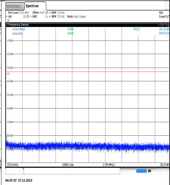
NTNV_N77-3450- 3550_PC2_30_40_L_TID1_NS_01_0.15_30_#1
