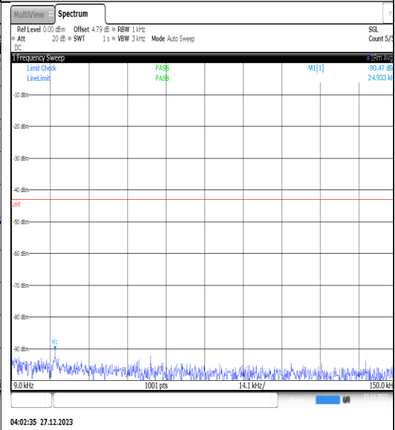
NTNV_N77-3450- 3550_PC2_30_30_H_TID7_NS_01_0.009_0.15_# 1
