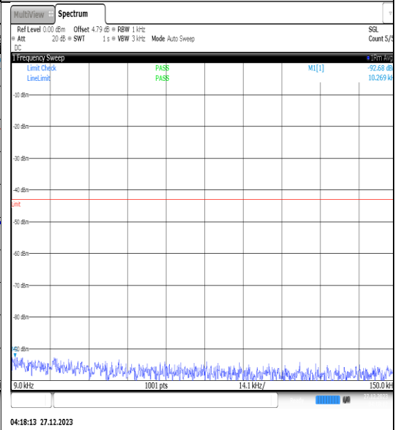
NTNV_N77-3450- 3550_PC2_30_30_H_TID11_NS_01_0.009_0.15_#1
