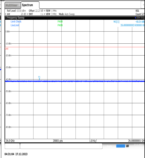
NTNV_N77-3450- 3550_PC2_30_30_H_TID13_NS_01_26000_4000_0_ #1
