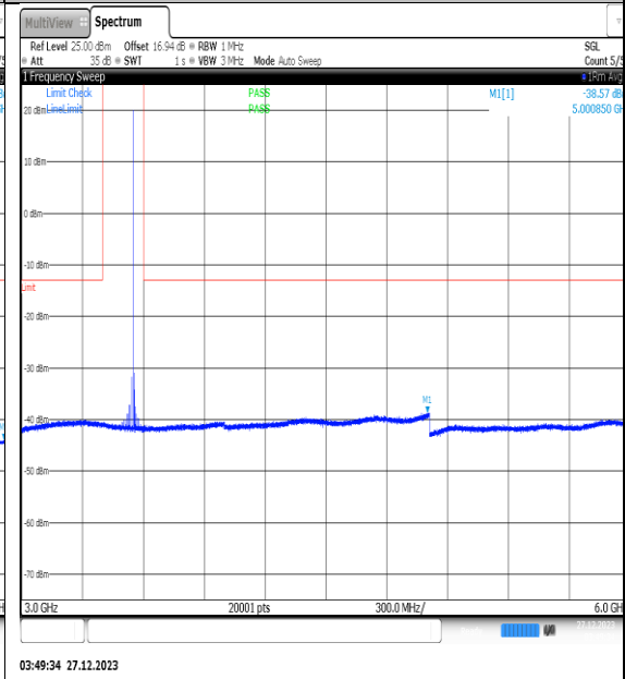
NTNV_N77-3450- 3550_PC2_30_30_H_TID3_NS_01_3000_6000_#1
