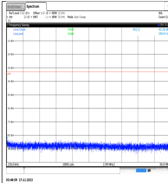
NTNV_N77-3450- 3550_PC2_30_30_H_TID3_NS_01_0.15_30_#1
