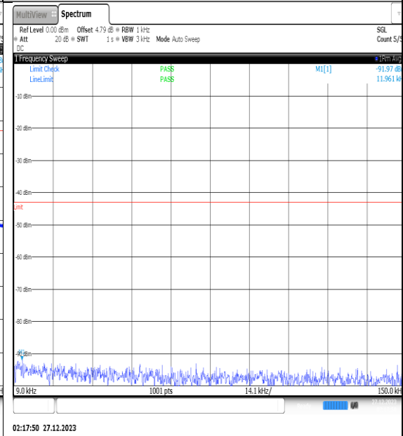
NTNV_N77-3450- 3550_PC2_30_30_M_TID2_NS_01_0.009_0.15_# 1
