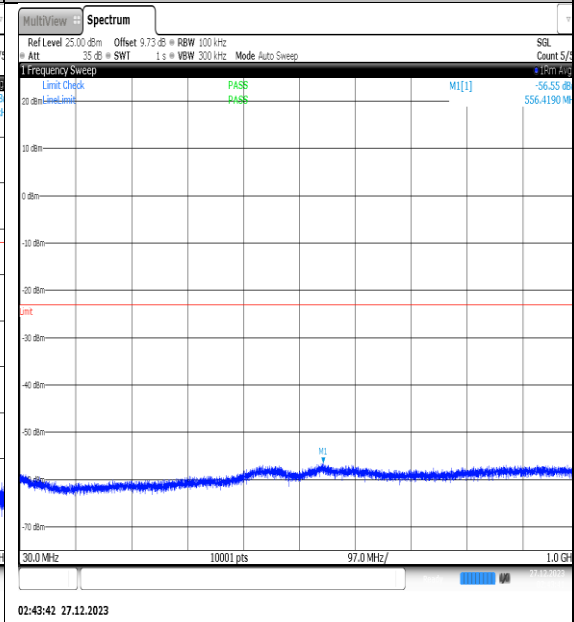
NTNV_N77-3450- 3550_PC2_30_30_M_TID8_NS_01_30_1000_#1
