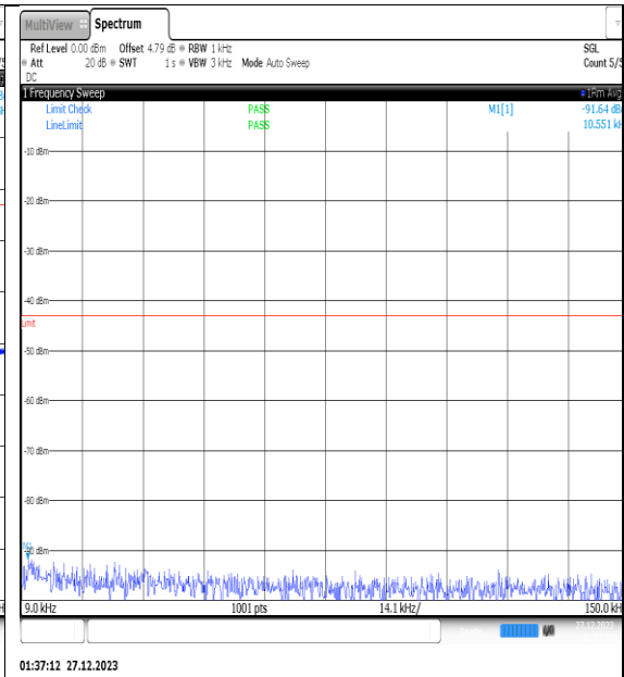
NTNV_N77-3450- 3550_PC2_30_30_L_TID7_NS_01_0.009_0.15_# 1
