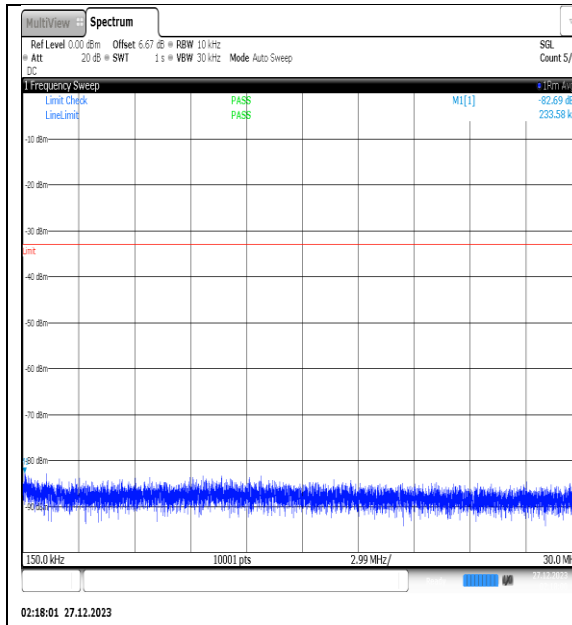
NTNV_N77-3450-3550_PC2_30_30_M_TID2_NS_01_0.15_30_#1
