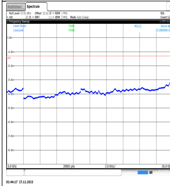
NTN_V_N77-3450- 3550_PC2_30_30_M_TID8_NS_01_6000_26000_# #1
