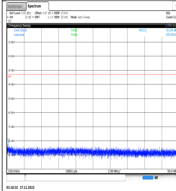
NTNV_N77-3450- 3550_PC2_30_30_L_TID15_NS_01_0.15_30_#1
