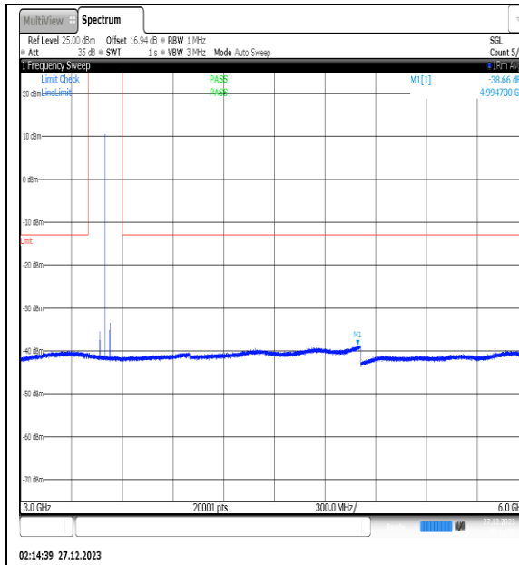
NTNV_N77-3450- 3550_PC2_30_30_M_TID1_NS_01_3000_6000_# 1
