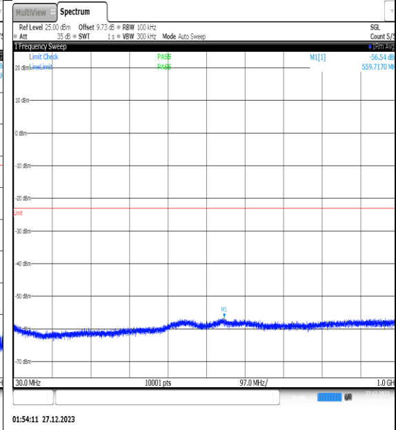
NTNV_N77-3450- 3550_PC2_30_30_L_TID11_NS_01_30_1000_#1
