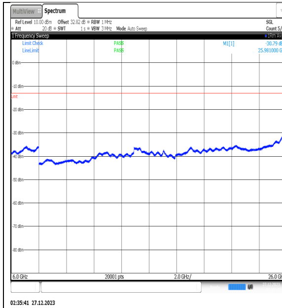
NTNV_N77-3450- 3550_PC2_30_30_M_TID6_NS_01_6000_26000_ #1
