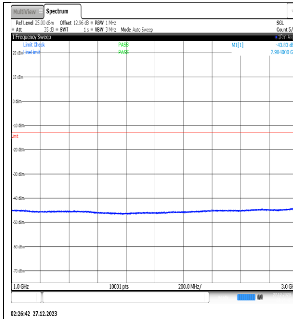
NTNV_N77-3450- 3550_PC2_30_30_M_TID4_NS_01_1000_3000_# 1
