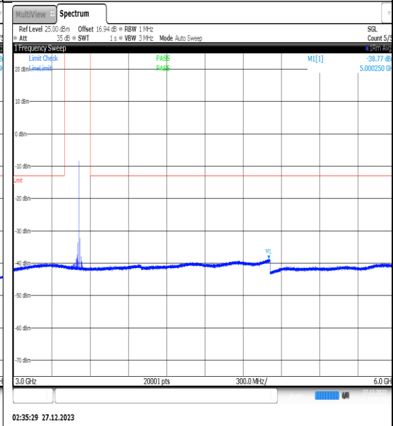
NTNV_N77-3450- 3550_PC2_30_30_M_TID6_NS_01_3000_6000_#1
