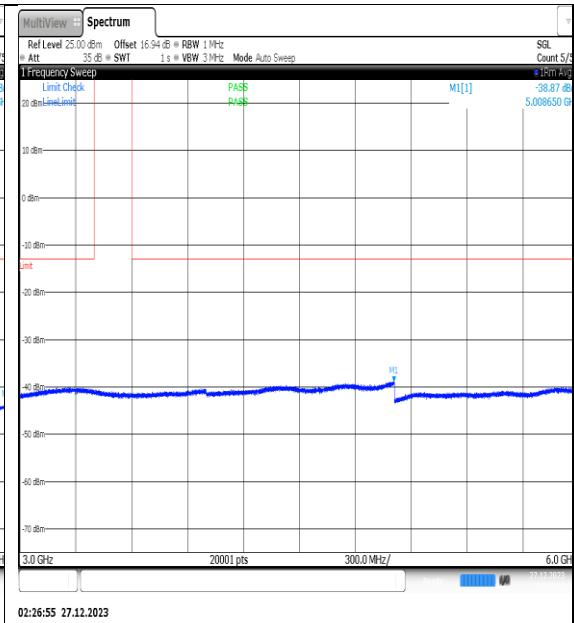
NTNV_N77-3450- 3550_PC2_30_30_M_TID4_NS_01_3000_6000_# 1
