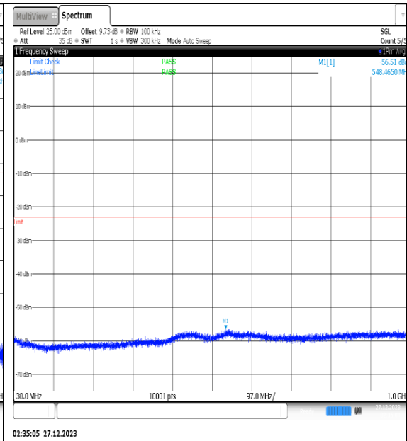
NTNV_N77-3450- 3550_PC2_30_30_M_TID6_NS_01_30_1000_#1
