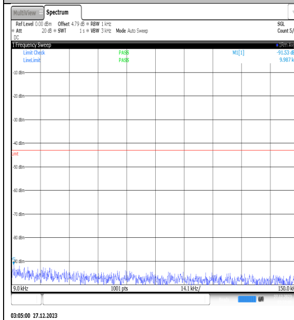
NTNV_N77-3450- 3550_PC2_30_30_M_TID11_NS_01_0.009_0.15_#1
