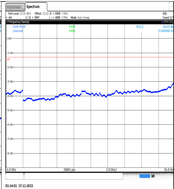
NTNV_N77-3450- 3550_PC2_30_30_M_TID1_NS_01_6000_26000_# #1
