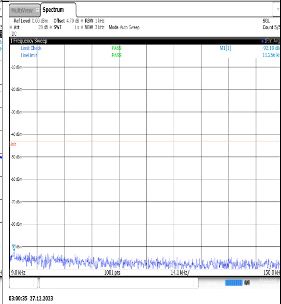
NTNV_N77-3450- 3550_PC2_30_30_M_TID10_NS_01_0.009_0.15_# 1
