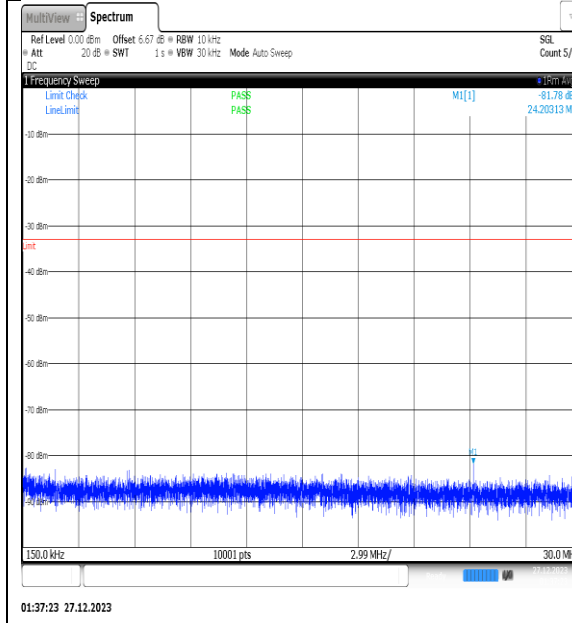
NTNV_N77-3450- 3550_PC2_30_30_L_TID7_NS_01_0.15_30_#1
