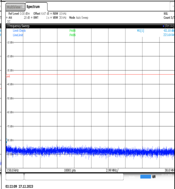
NTNV_N77-3450- 3550_PC2_30_30_M_TID3_NS_01_0.15_30_#1
