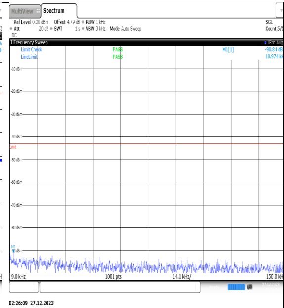
NTNV_N77-3450- 3550_PC2_30_30_M_TID4_NS_01_0.009_0.15_# 1
