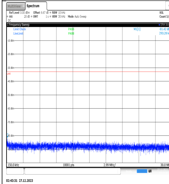
NTNV_N77-3450- 3550_PC2_30_30_M_TID8_NS_01_0.15_30_#1
