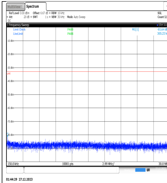
NTNV_N77-3450- 3550_PC2_30_30_L_TID9_NS_01_0.15_30_#1
