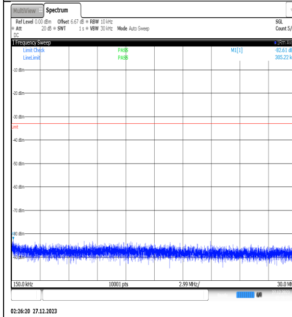
NTNV_N77-3450- 3550_PC2_30_30_M_TID4_NS_01_0.15_30_#1
