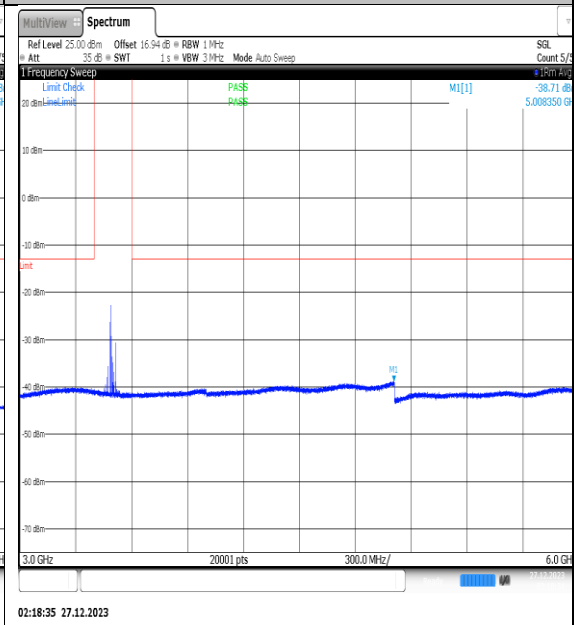
NTNV_N77-3450-3550_PC2_30_30_M_TID2_NS_01_3000_6000_#1
