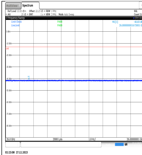
NTNV_N77-3450- 3550_PC2_30_30_M_TID3_NS_01_26000_40000 #1
