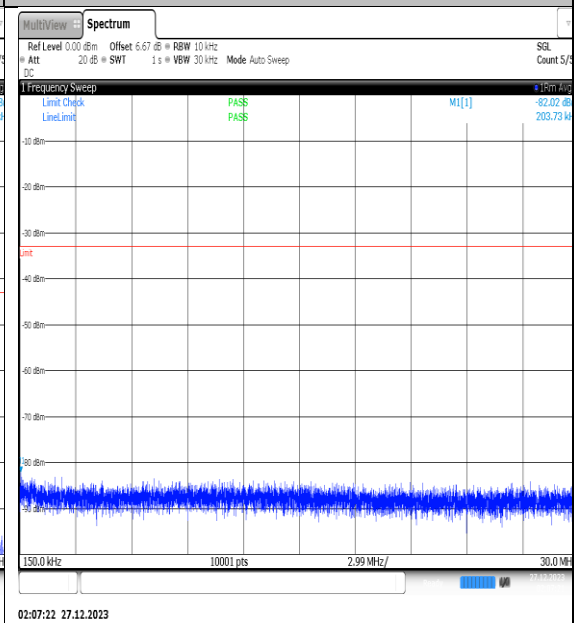
NTNV_N77-3450- 3550_PC2_30_30_L_TID14_NS_01_0.15_30_#1
