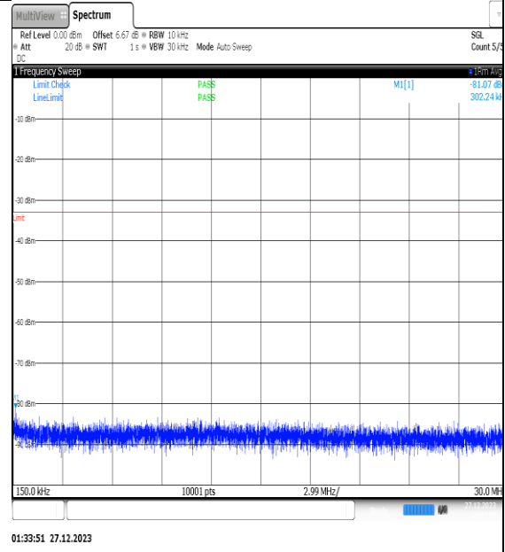
NTNV_N77-3450- 3550_PC2_30_30_L_TID6_NS_01_0.15_30_#1
