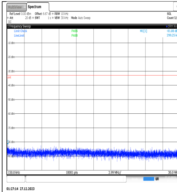
NTNV_N77-3450- 3550_PC2_30_30_L_TID5_NS_01_0.15_30_#1
