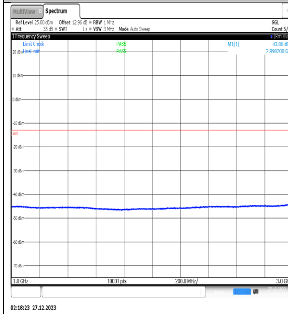
NTNV_N77-3450-3550_PC2_30_30_M_TID2_NS_01_1000_3000_#1
