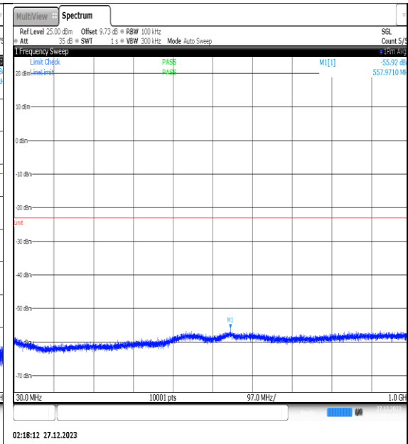
NTNV_N77-3450-3550_PC2_30_30_M_TID2_NS_01_30_1000_#1
