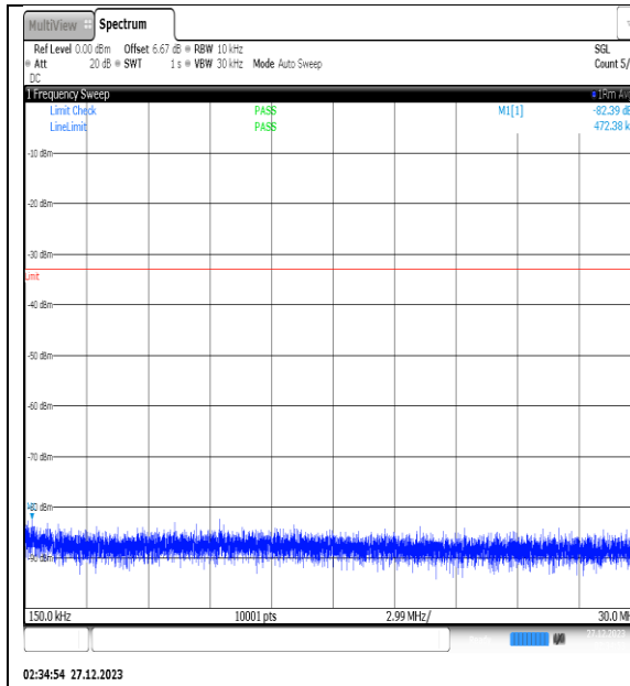
NTNV_N77-3450- 3550_PC2_30_30_M_TID6_NS_01_0.15_30_#1
