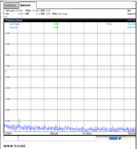
NTNV_N77-3450- 3550_PC2_30_25_H_TID10_NS_01_0.009_0.15_ #1
