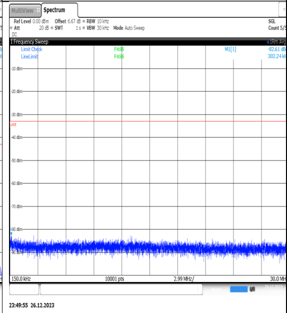
NTNV_N77-3450-3550_PC2_30_25_M_TID12_NS_01_0.15_30_#1
