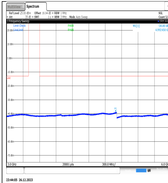
NTNV_N77-3450- 3550_PC2_30_25_M_TID10_NS_01_3000_6000_ #1
