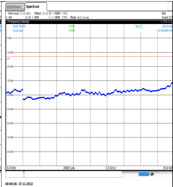
NTNV_N77-3450- 3550_PC2_30_25_M_TID14_NS_01_6000_26000 #1
