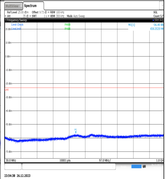
NTNV_N77-3450- 3550_PC2_30_25_M_TID13_NS_01_30_1000_#1
