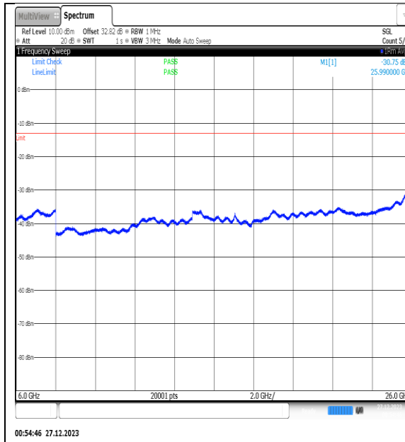
NTNV_N77-3450- 3550_PC2_30_25_H_TID12_NS_01_6000_26000 _#1
