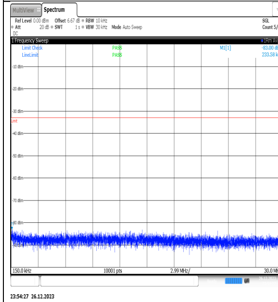
NTNV_N77-3450- 3550_PC2_30_25_M_TID13_NS_01_0.15_30_#1
