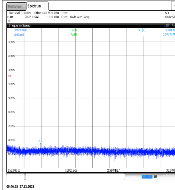
NTNV_N77-3450- 3550_PC2_30_25_H_TID10_NS_01_0.15_30_#1
