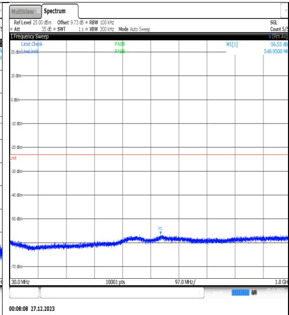
NTNV_N77-3450-3550_PC2_30_25_M_TID15_NS_01_30_1000_#1
