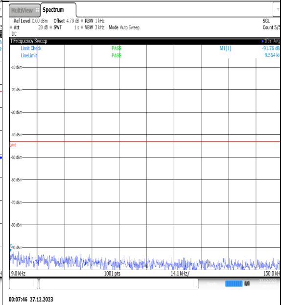
NTNV_N77-3450- 3550_PC2_30_25_M_TID15_NS_01_0.009_0.15_ #1
