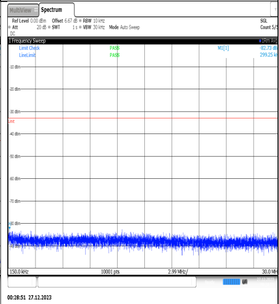
NTNV_N77-3450- 3550_PC2_30_25_H_TID5_NS_01_0.15_30_#1
