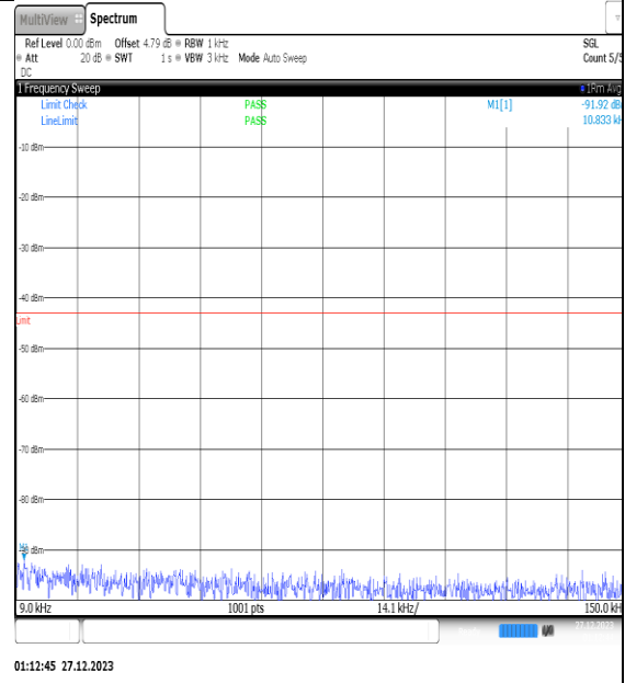
NTNV_N77-3450- 3550_PC2_30_30_L_TID1_NS_01_0.009_0.15_#1
