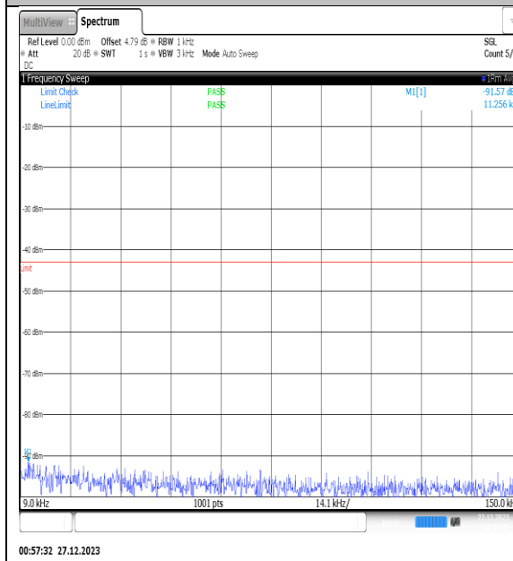
NTNV_N77-3450- 3550_PC2_30_25_H_TID13_NS_01_0.009_0.15_#1
