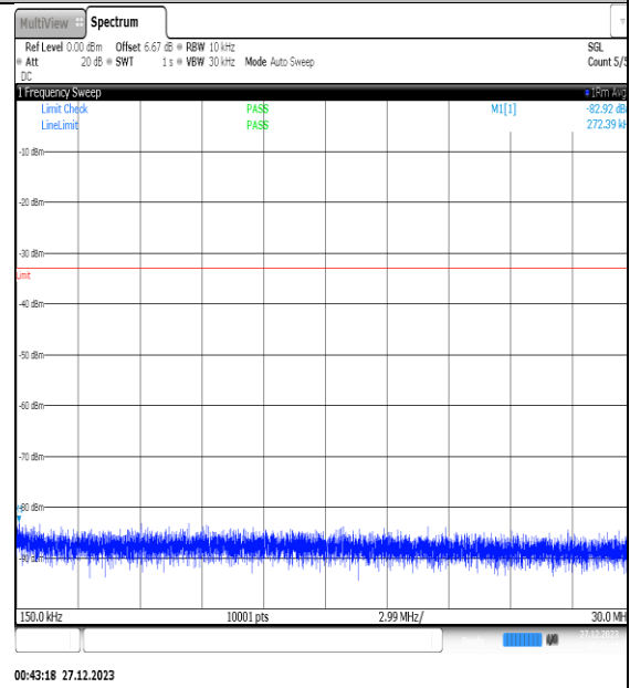
NTNV_N77-3450- 3550_PC2_30_25_H_TID9_NS_01_0.15_30_#1
