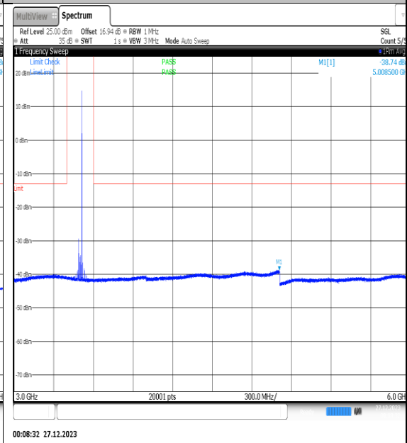
NTNV_N77-3450-3550_PC2_30_25_M_TID15_NS_01_3000_6000_#1
