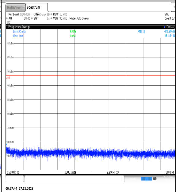
NTNV_N77-3450- 3550_PC2_30_25_H_TID13_NS_01_0.15_30_#1
