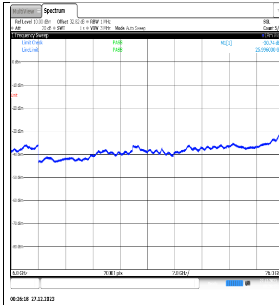
NTNV_N77-3450- 3550_PC2_30_25_H_TID4_NS_01_6000_26000_#1
