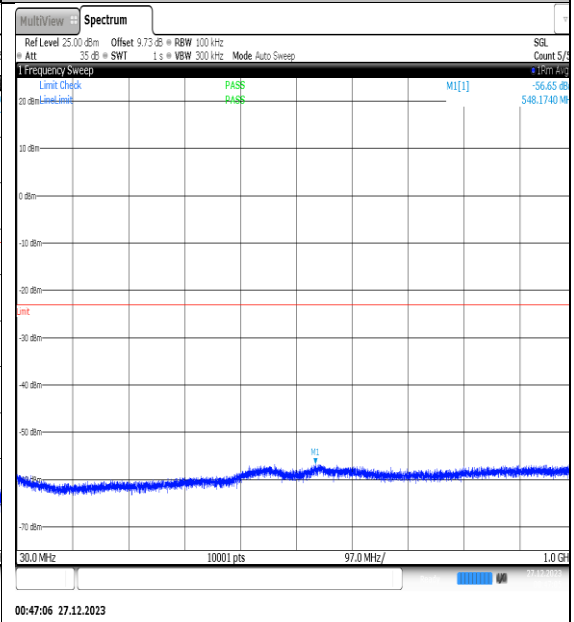
NTNV_N77-3450- 3550_PC2_30_25_H_TID10_NS_01_30_1000_#1
