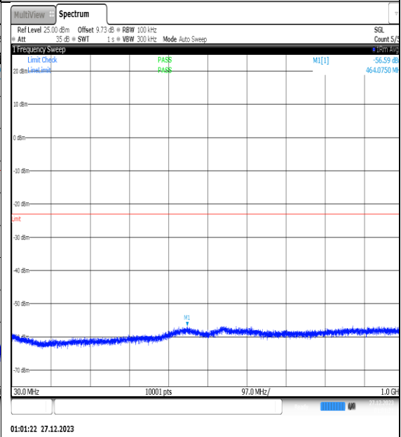
NTNV_N77-3450- 3550_PC2_30_25_H_TID14_NS_01_30_1000_#1
