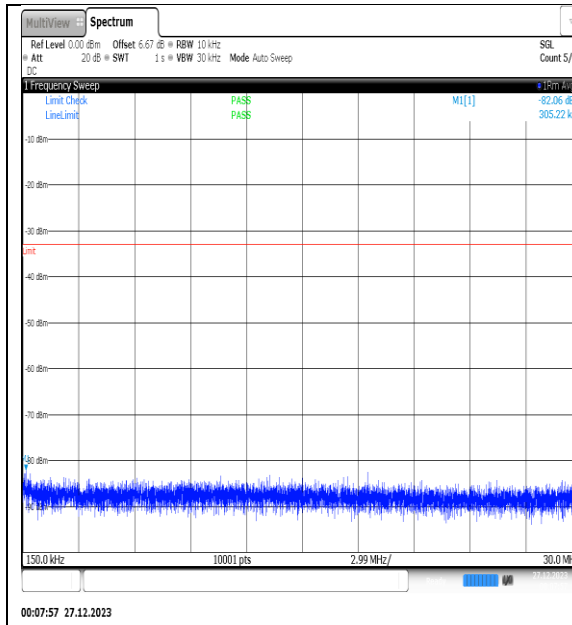
NTNV_N77-3450-3550_PC2_30_25_M_TID15_NS_01_0.15_30_#1
