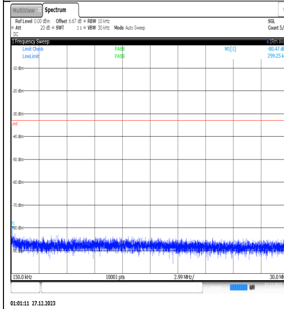
NTNV_N77-3450- 3550_PC2_30_25_H_TID14_NS_01_0.15_30_#1
