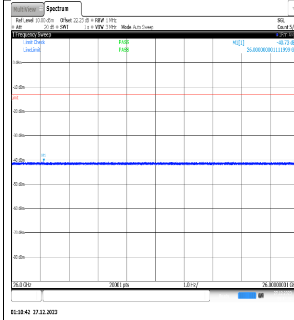
NTNV_N77-3450- 3550_PC2_30_25_H_TID15_NS_01_26000_4000_0_#1
