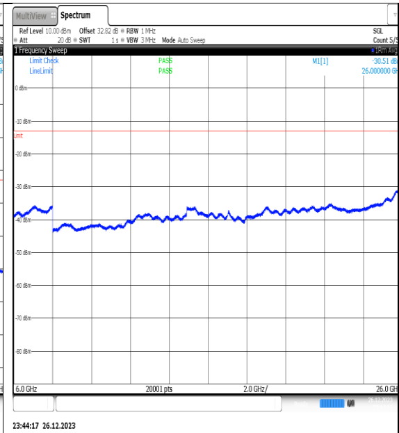
NTNV_N77-3450- 3550_PC2_30_25_M_TID10_NS_01_6000_26000 #1
