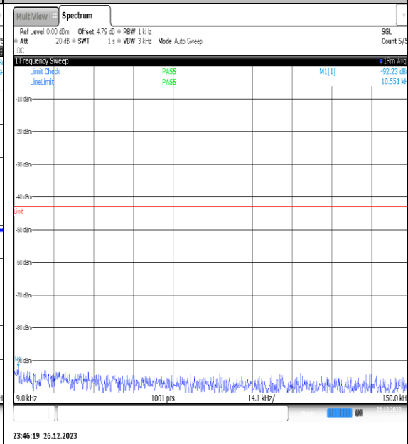
NTNV_N77-3450- 3550_PC2_30_25_M_TID11_NS_01_0.009_0.15_ #1
