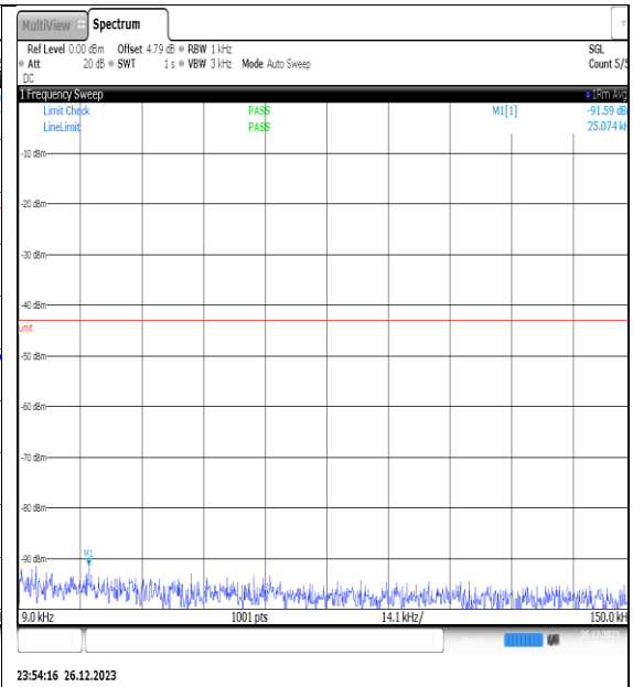
NTNV_N77-3450- 3550_PC2_30_25_M_TID13_NS_01_0.009_0.15_ #1
