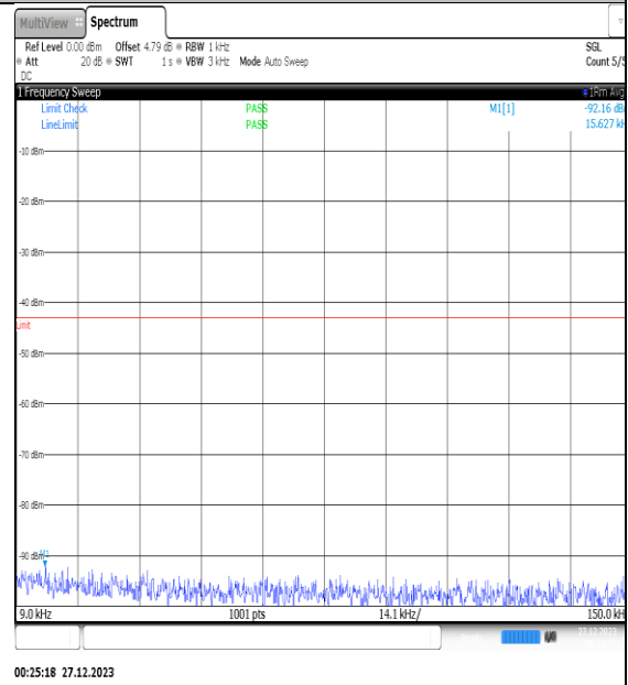
NTNV_N77-3450- 3550_PC2_30_25_H_TID4_NS_01_0.009_0.15_# 1
