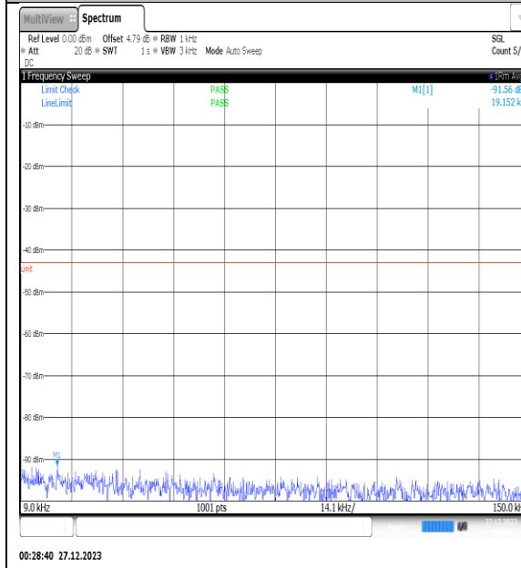
NTNV_N77-3450- 3550_PC2_30_25_H_TID5_NS_01_0.009_0.15_#1
