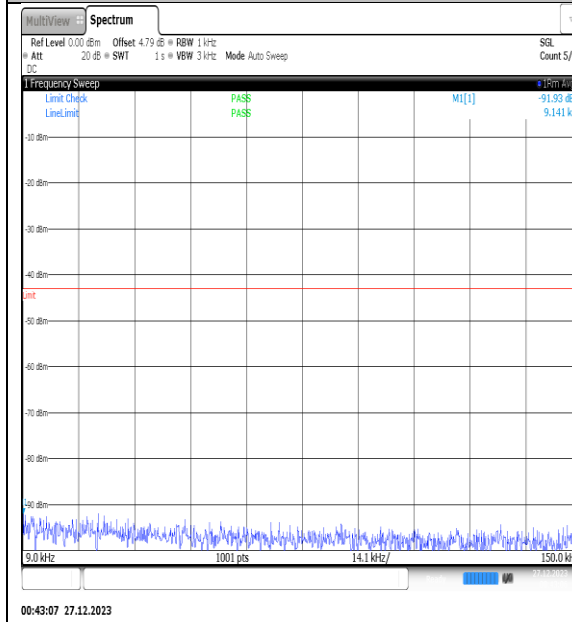
NTNV_N77-3450- 3550_PC2_30_25_H_TID9_NS_01_0.009_0.15_#1
