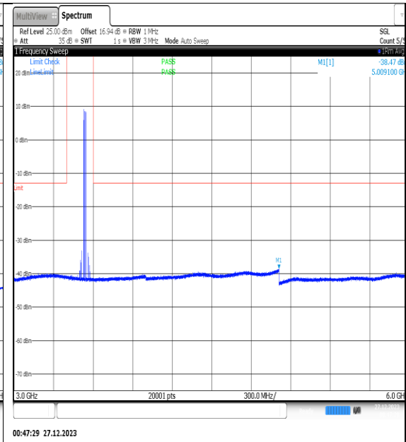
NTNV_N77-3450- 3550_PC2_30_25_H_TID10_NS_01_3000_6000_ #1
