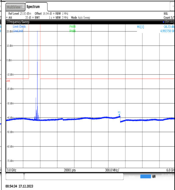
NTNV_N77-3450-3550_PC2_30_25_H_TID12_NS_01_3000_6000_#1
