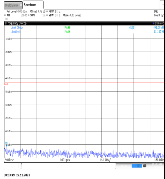
NTNV_N77-3450- 3550_PC2_30_25_H_TID12_NS_01_0.009_0.15_#1
