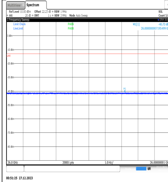
NTNV_N77-3450- 3550_PC2_30_25_H_TID11_NS_01_26000_4000_0_#1
