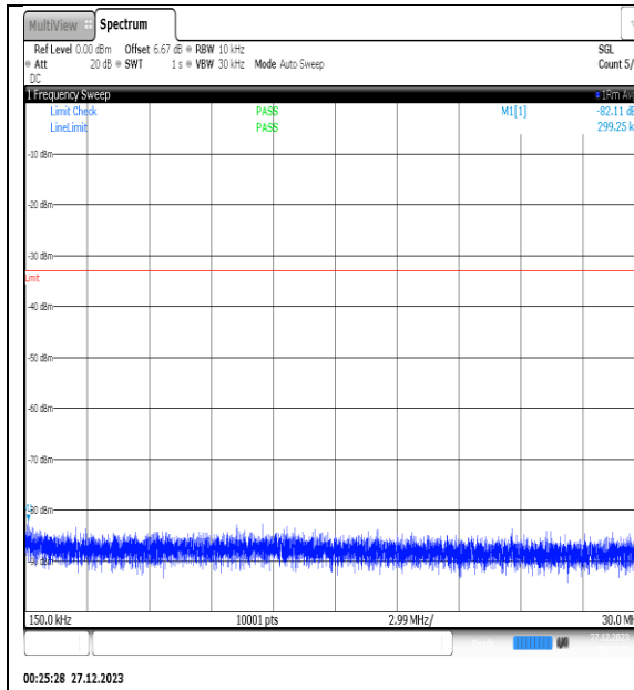
NTNV_N77-3450- 3550_PC2_30_25_H_TID4_NS_01_0.15_30_#1
