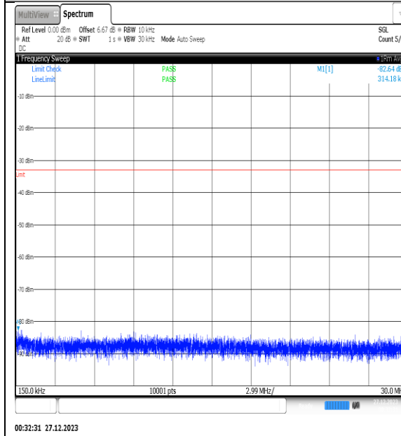
NTNV_N77-3450- 3550_PC2_30_25_H_TID6_NS_01_0.15_30_#1
