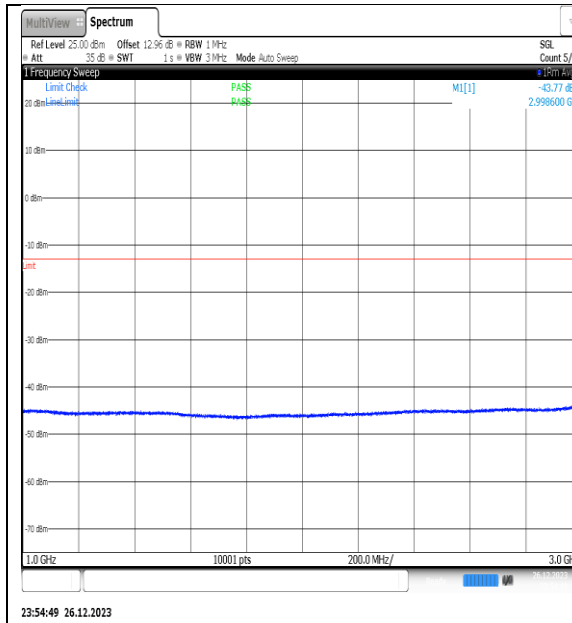
NTNV_N77-3450- 3550_PC2_30_25_M_TID13_NS_01_1000_3000_ #1
