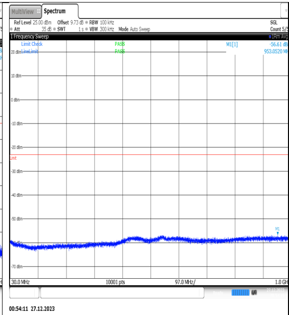
NTNV_N77-3450-3550_PC2_30_25_H_TID12_NS_01_30_1000_#1
