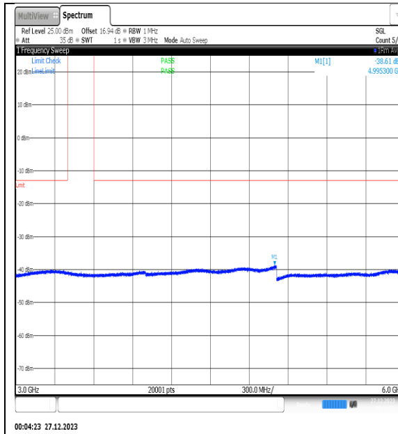
NTNV_N77-3450- 3550_PC2_30_25_M_TID14_NS_01_3000_6000_ #1
