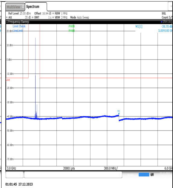
NTNV_N77-3450- 3550_PC2_30_25_H_TID14_NS_01_3000_6000_ #1
