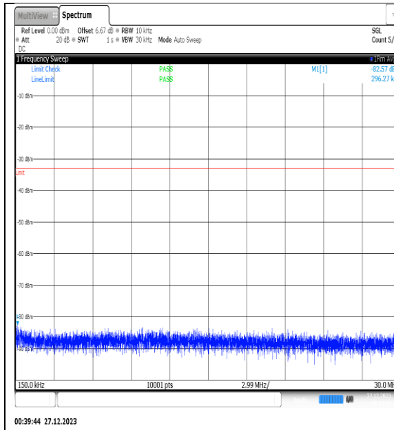
NTNV_N77-3450- 3550_PC2_30_25_H_TID8_NS_01_0.15_30_#1
