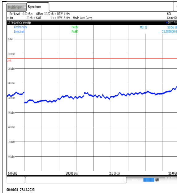
NTNV_N77-3450- 3550_PC2_30_25_H_TID8_NS_01_6000_26000_#1
