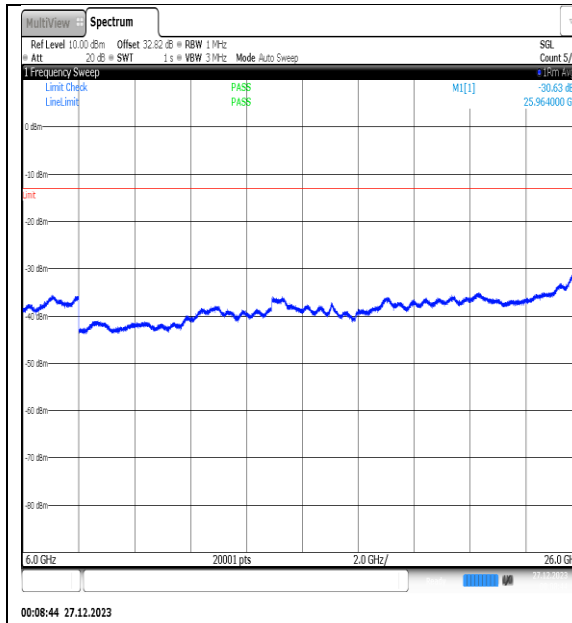
NTNV_N77-3450- 3550_PC2_30_25_M_TID15_NS_01_6000_26000 _#1
