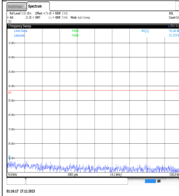
NTNV_N77-3450- 3550_PC2_30_30_L_TID2_NS_01_0.009_0.15_# 1
