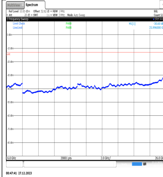
NTNV_N77-3450- 3550_PC2_30_25_H_TID10_NS_01_6000_26000 #1
