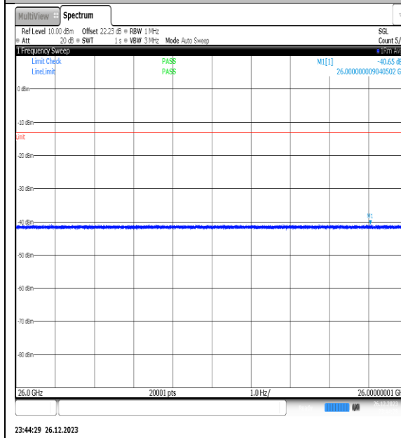
NTNV_N77-3450- 3550_PC2_30_25_M_TID10_NS_01_26000_4000 0_#1
