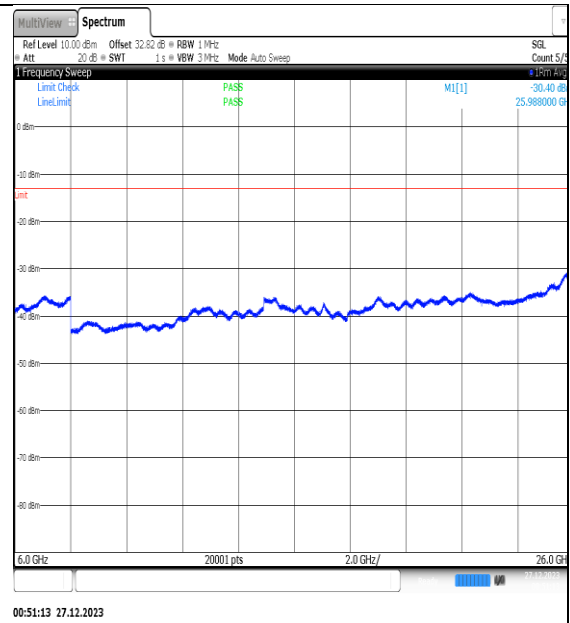
NTNV_N77-3450- 3550_PC2_30_25_H_TID11_NS_01_6000_26000_#1
