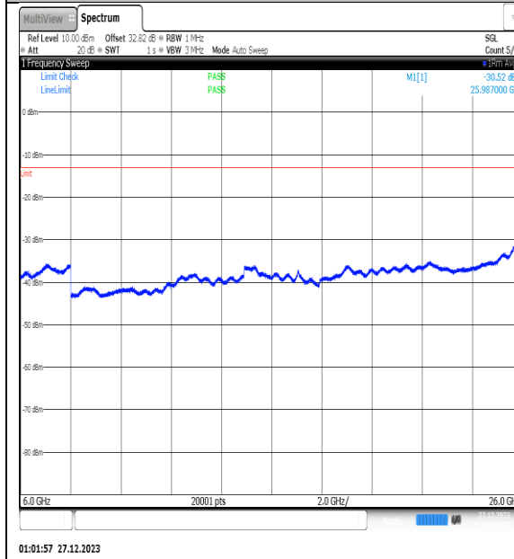
NTNV_N77-3450- 3550_PC2_30_25_H_TID14_NS_01_6000_26000_ #1
