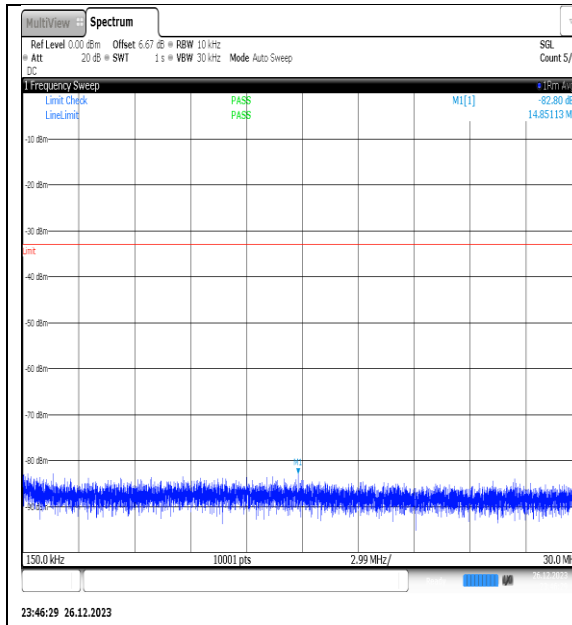
NTNV_N77-3450- 3550_PC2_30_25_M_TID11_NS_01_0.15_30_#1
