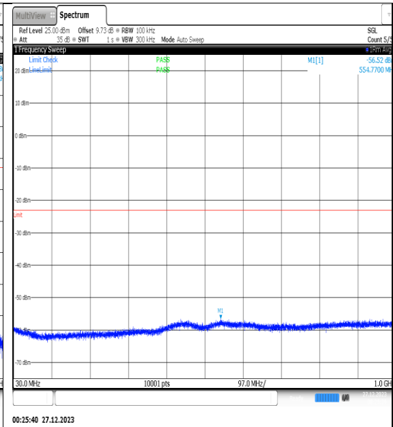
NTNV_N77-3450- 3550_PC2_30_25_H_TID4_NS_01_30_1000_#1
