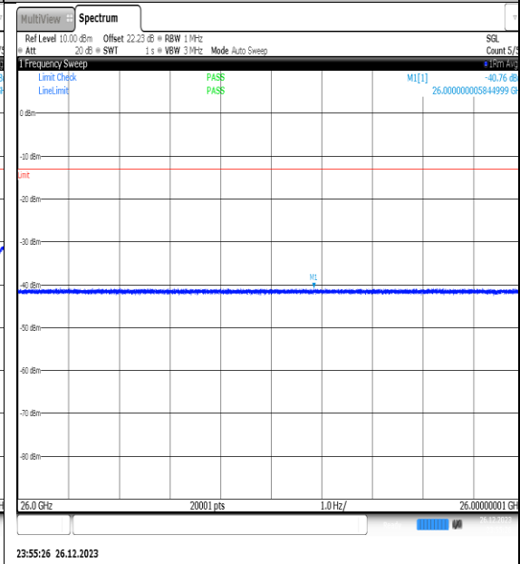
NTNV_N77-3450- 3550_PC2_30_25_M_TID13_NS_01_26000_4000_0_ #1
