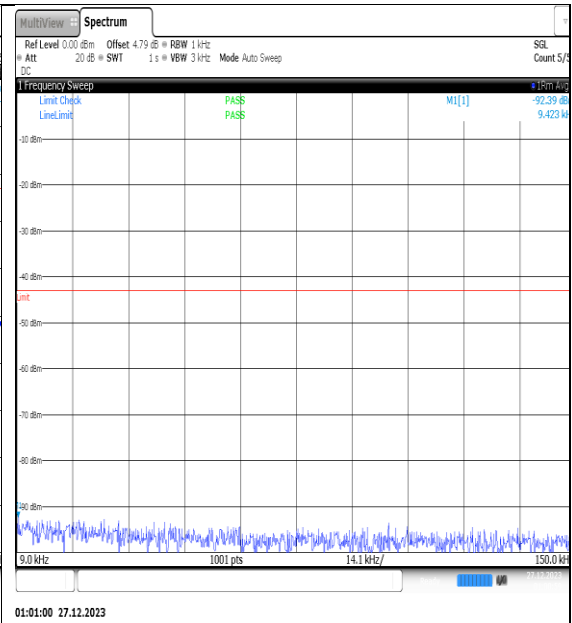
NTNV_N77-3450- 3550_PC2_30_25_H_TID14_NS_01_0.009_0.15_ #1
