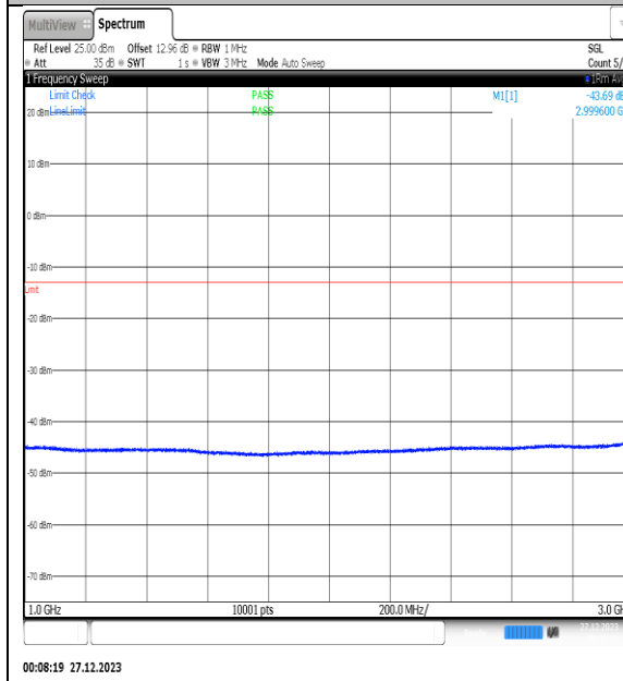
NTNV_N77-3450-3550_PC2_30_25_M_TID15_NS_01_1000_3000_#1
