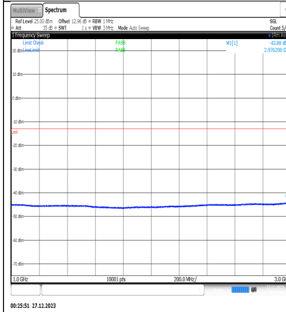
NTNV_N77-3450- 3550_PC2_30_25_H_TID4_NS_01_1000_3000_#1
