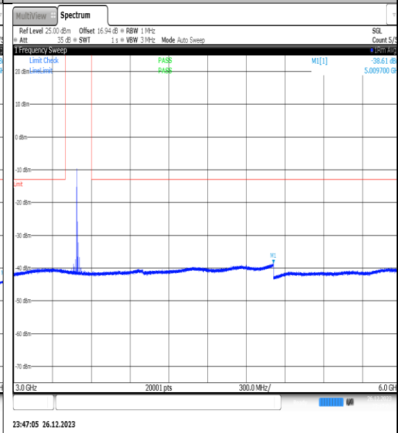
NTNV_N77-3450- 3550_PC2_30_25_M_TID11_NS_01_3000_6000_#1
