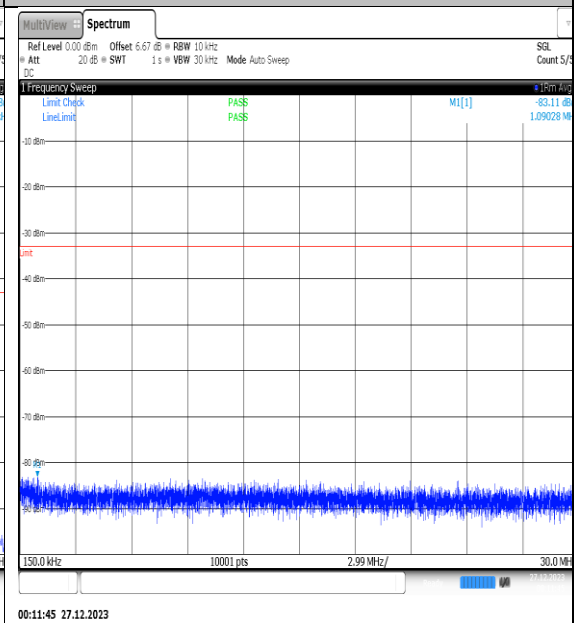
NTNV_N77-3450- 3550_PC2_30_25_H_TID1_NS_01_0.15_30_#1
