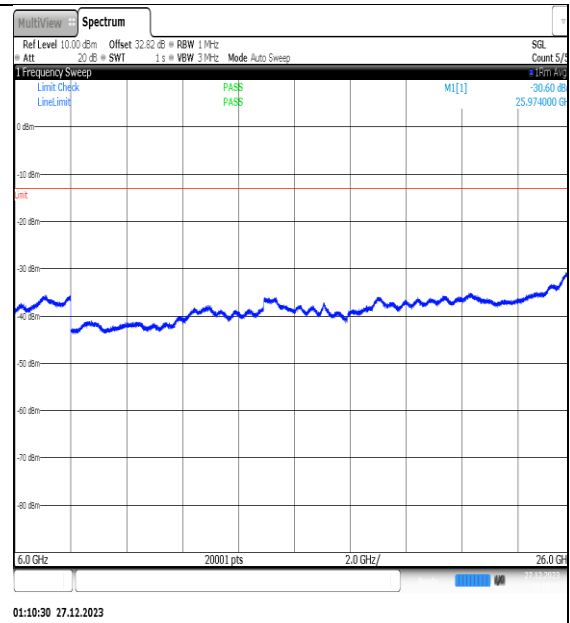
NTNV_N77-3450- 3550_PC2_30_25_H_TID15_NS_01_6000_26000_#1
