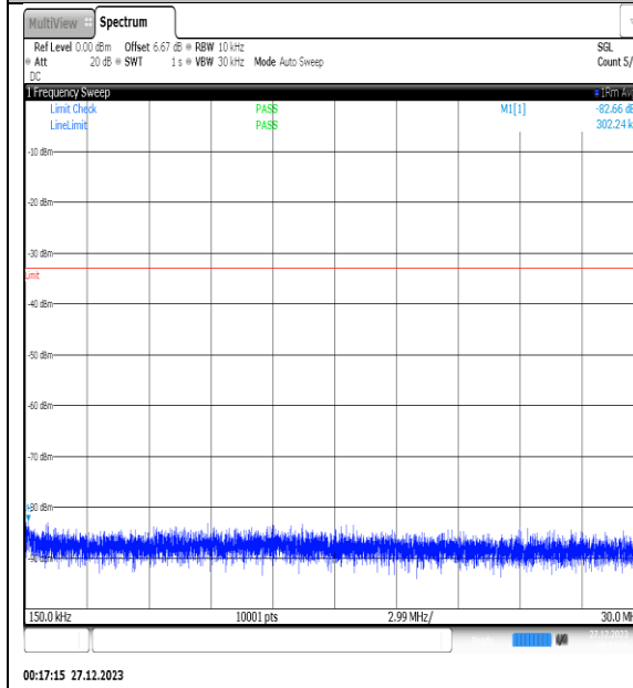
NTNV_N77-3450- 3550_PC2_30_25_H_TID2_NS_01_0.15_30_#1
