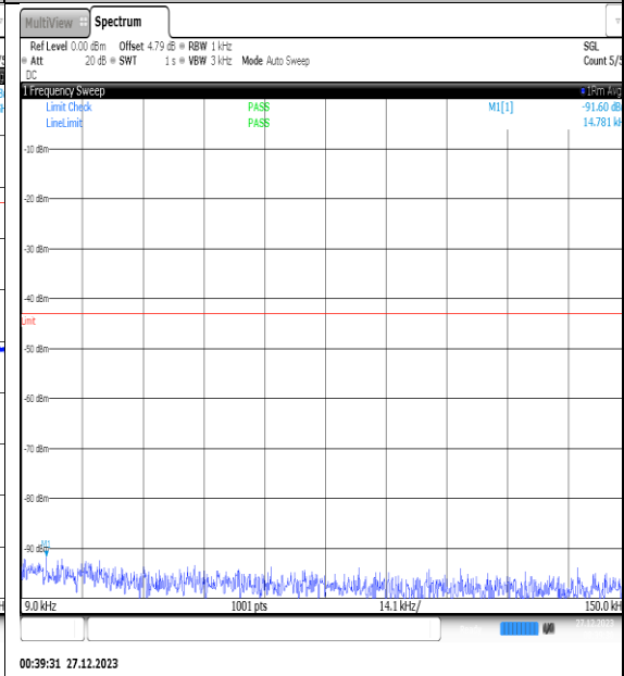
NTN_V_N77-3450- 3550_PC2_30_25_H_TID8_NS_01_0.009_0.15_# 1
