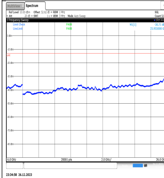
NTNV_N77-3450- 3550_PC2_30_25_M_TID9_NS_01_6000_26000_# #1
