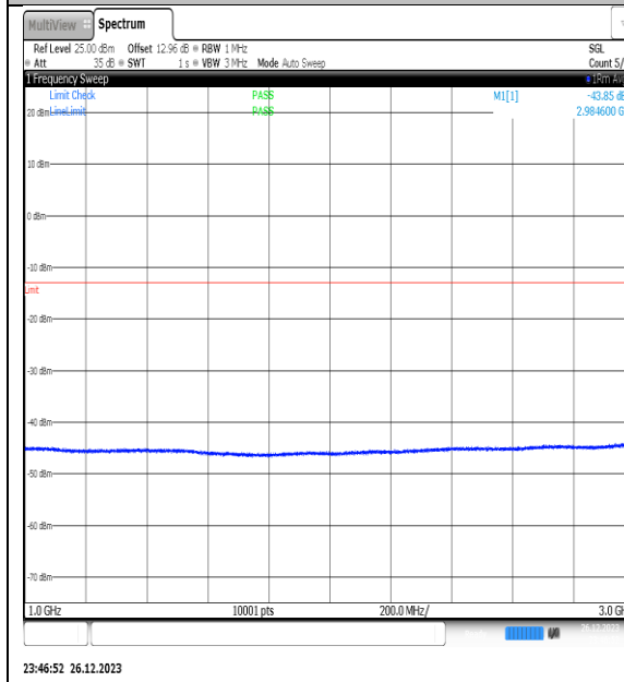
NTNV_N77-3450- 3550_PC2_30_25_M_TID11_NS_01_1000_3000_#1
