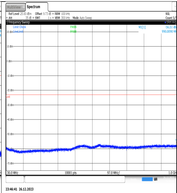
NTNV_N77-3450- 3550_PC2_30_25_M_TID11_NS_01_30_1000_#1
