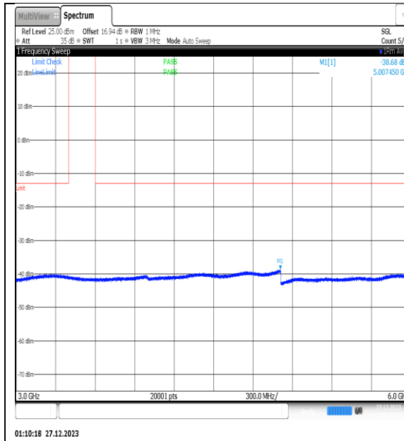
NTNV_N77-3450- 3550_PC2_30_25_H_TID15_NS_01_3000_6000_#1
