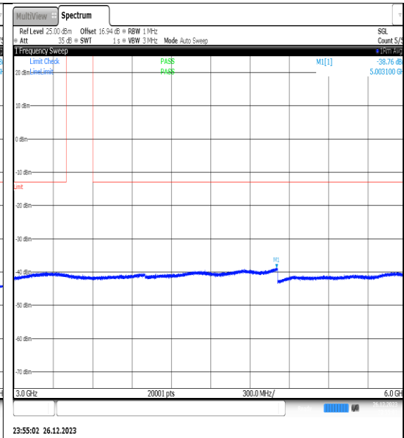
NTNV_N77-3450- 3550_PC2_30_25_M_TID13_NS_01_3000_6000_ #1
