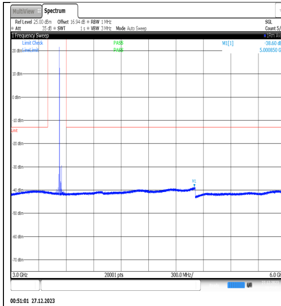
NTNV_N77-3450- 3550_PC2_30_25_H_TID11_NS_01_3000_6000_#1
