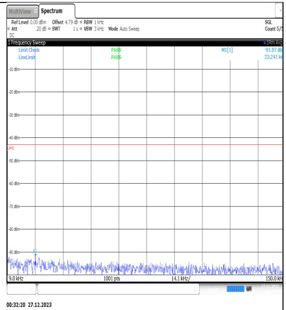
NTNV_N77-3450- 3550_PC2_30_25_H_TID6_NS_01_0.009_0.15_# 1
