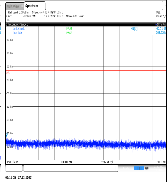
NTNV_N77-3450- 3550_PC2_30_30_L_TID2_NS_01_0.15_30_#1
