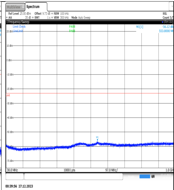
NTNV_N77-3450- 3550_PC2_30_25_H_TID8_NS_01_30_1000_#1
