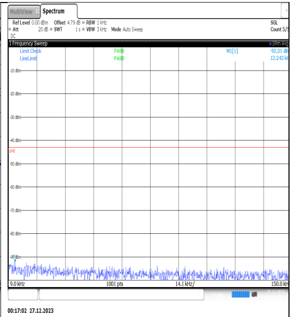
NTNV_N77-3450- 3550_PC2_30_25_H_TID2_NS_01_0.009_0.15_# 1
