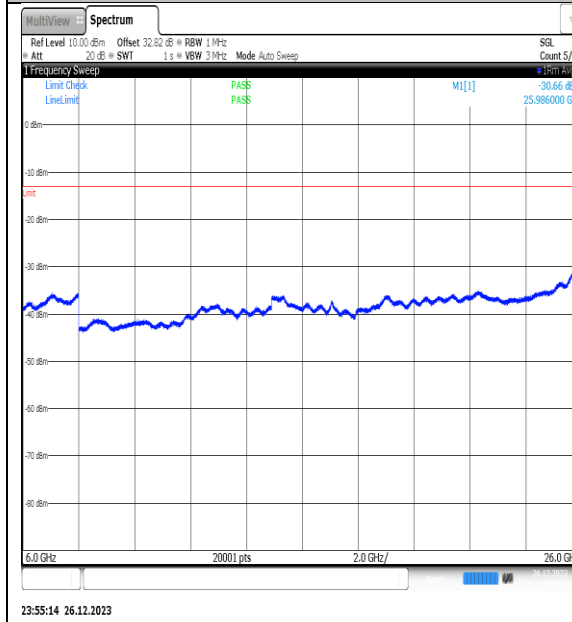
NTNV_N77-3450- 3550_PC2_30_25_M_TID13_NS_01_6000_26000_ #1
