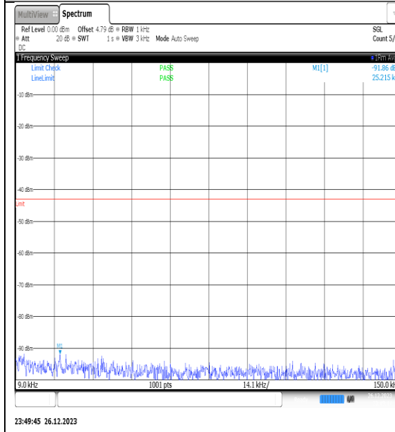
NTNV_N77-3450-3550_PC2_30_25_M_TID12_NS_01_0.009_0.15_#1
