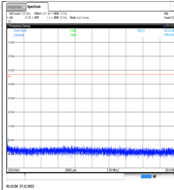
NTNV_N77-3450- 3550_PC2_30_30_L_TID1_NS_01_0.15_30_#1
