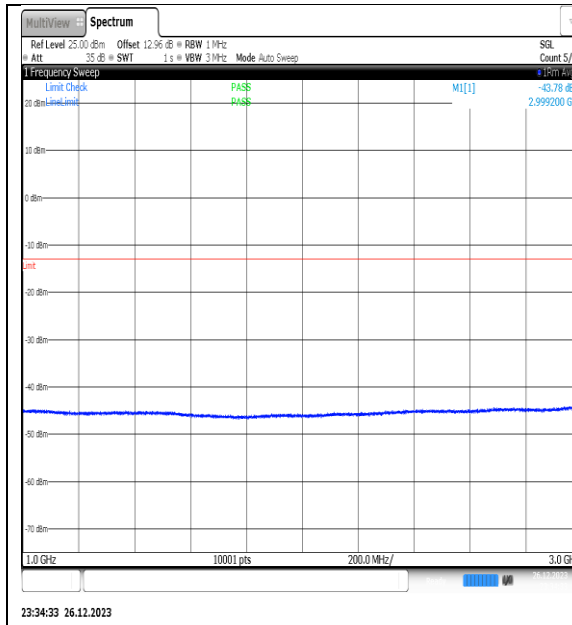
NTNV_N77-3450- 3550_PC2_30_25_M_TID9_NS_01_1000_3000_# 1
