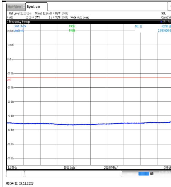
NTNV_N77-3450-3550_PC2_30_25_H_TID12_NS_01_1000_3000_#1
