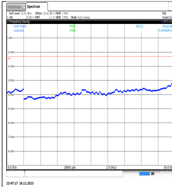
NTNV_N77-3450-3550_PC2_30_25_M_TID11_NS_01_6000_26000_#1
