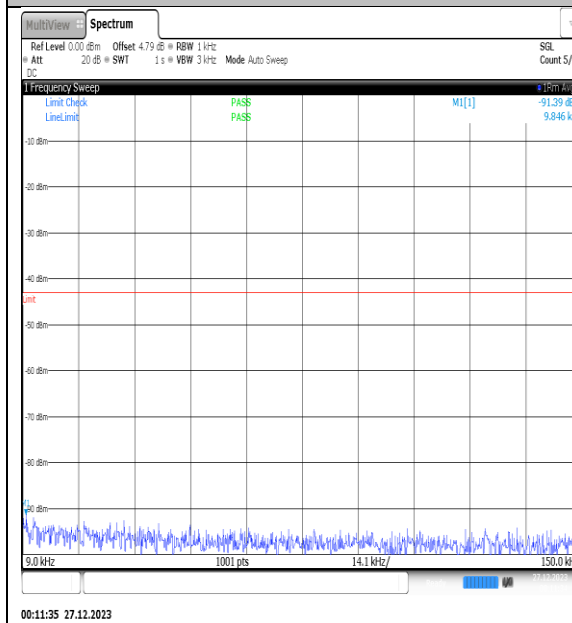
NTNV_N77-3450- 3550_PC2_30_25_H_TID1_NS_01_0.009_0.15_# 1
