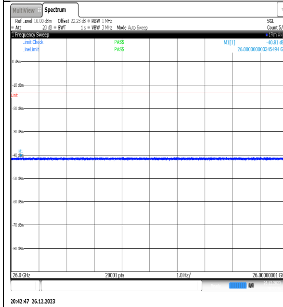
NTNV_N77-3450- 3550_PC2_30_20_M_TID15_NS_01_26000_4000 0_#1
