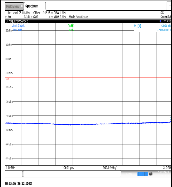
NTNV_N77-3450- 3550_PC2_30_20_M_TID11_NS_01_1000_3000_ #1
