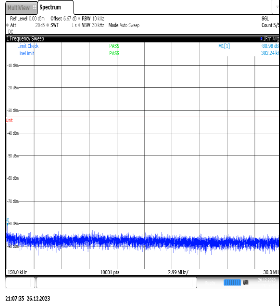
NTNV_N77-3450- 3550_PC2_30_20_H_TID6_NS_01_0.15_30_#1
