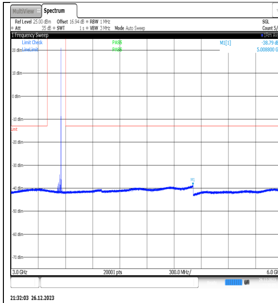
NTNV_N77-3450- 3550_PC2_30_20_H_TID12_NS_01_3000_6000_#1
