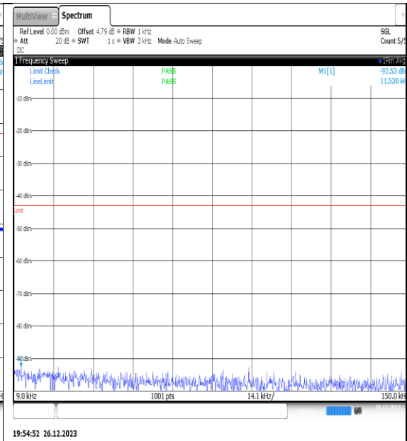
NTNV_N77-3450- 3550_PC2_30_20_M_TID6_NS_01_0.009_0.15_# 1
