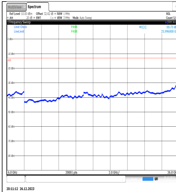
NTNV_N77-3450- 3550_PC2_30_20_M_TID8_NS_01_6000_26000_ #1
