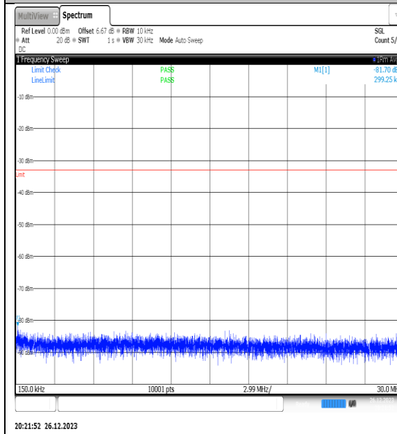
NTNV_N77-3450- 3550_PC2_30_20_M_TID10_NS_01_0.15_30_#1
