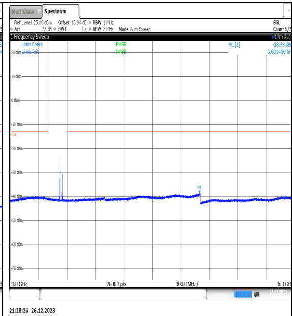
NTNV_N77-3450- 3550_PC2_30_20_H_TID11_NS_01_3000_6000_ #1
