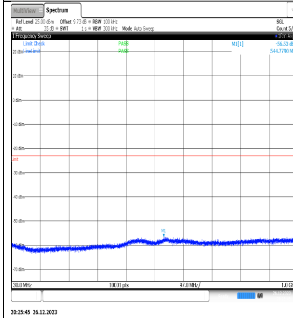
NTNV_N77-3450- 3550_PC2_30_20_M_TID11_NS_01_30_1000_#1
