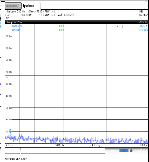
NTNV_N77-3450- 3550_PC2_30_20_M_TID12_NS_01_0.009_0.15_ #1
