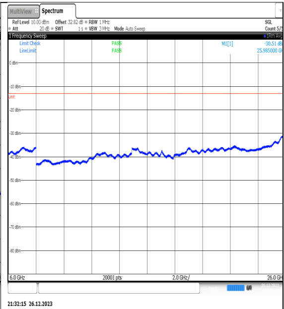
NTNV_N77-3450- 3550_PC2_30_20_H_TID12_NS_01_6000_26000_#1
