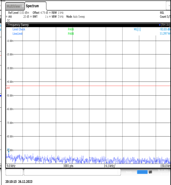
NTN_V_N77-3450- 3550_PC2_30_20_M_TID8_NS_01_0.009_0.15_# 1
