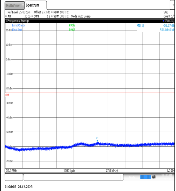
NTNV_N77-3450- 3550_PC2_30_20_H_TID11_NS_01_30_1000_#1
