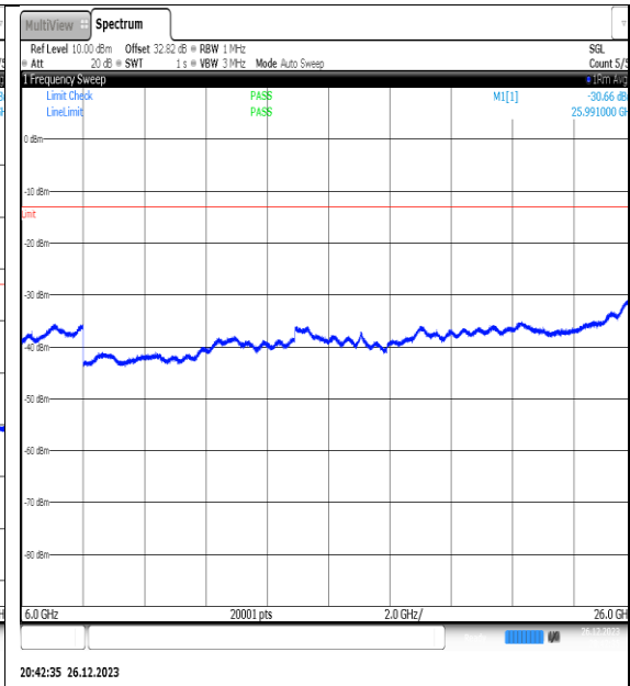
NTNV_N77-3450- 3550_PC2_30_20_M_TID15_NS_01_6000_26000 _#1
