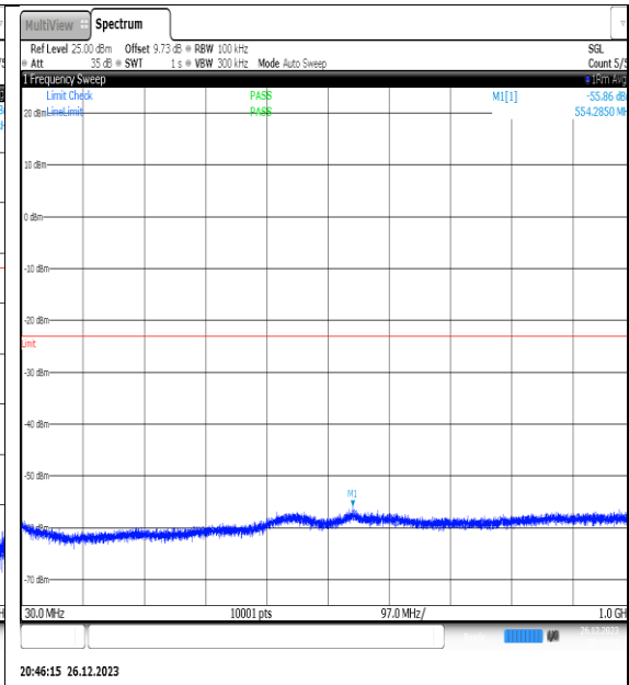
NTNV_N77-3450- 3550_PC2_30_20_H_TID1_NS_01_30_1000_#1
