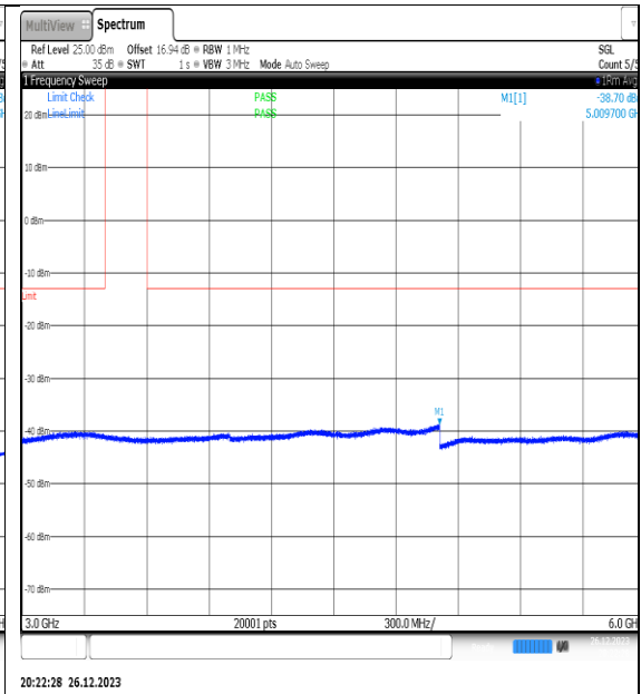
NTNV_N77-3450- 3550_PC2_30_20_M_TID10_NS_01_3000_6000_ #1
