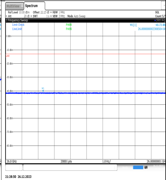
NTNV_N77-3450- 3550_PC2_30_20_H_TID11_NS_01_26000_4000_ 0_#1
