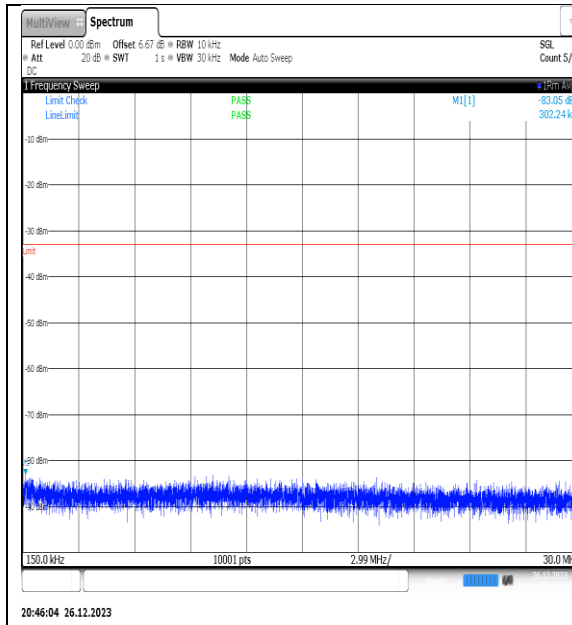
NTNV_N77-3450- 3550_PC2_30_20_H_TID1_NS_01_0.15_30_#1
