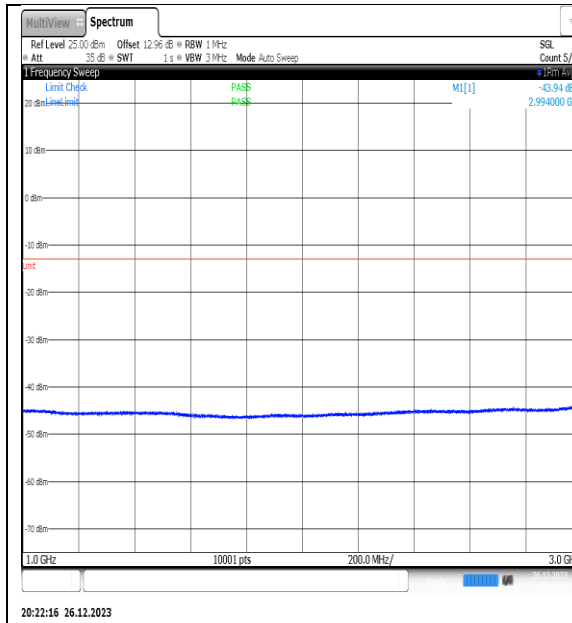
NTNV_N77-3450- 3550_PC2_30_20_M_TID10_NS_01_1000_3000_ #1
