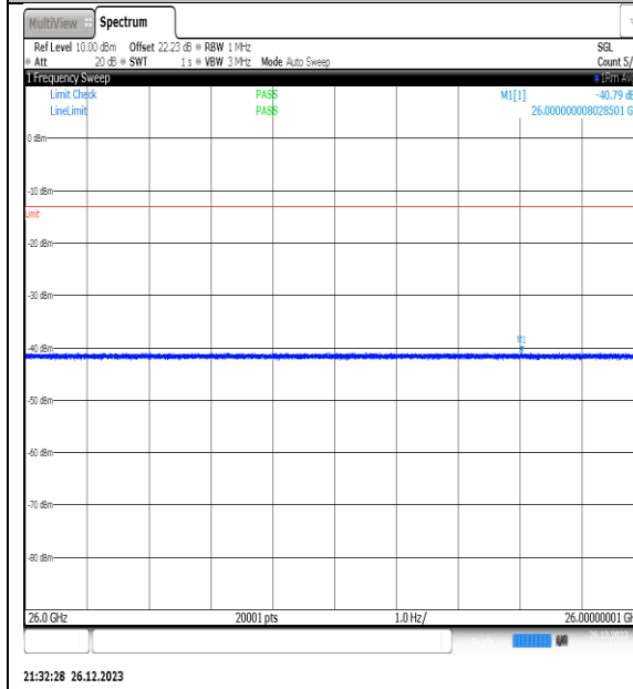
NTNV_N77-3450- 3550_PC2_30_20_H_TID12_NS_01_26000_4000_0_#1
