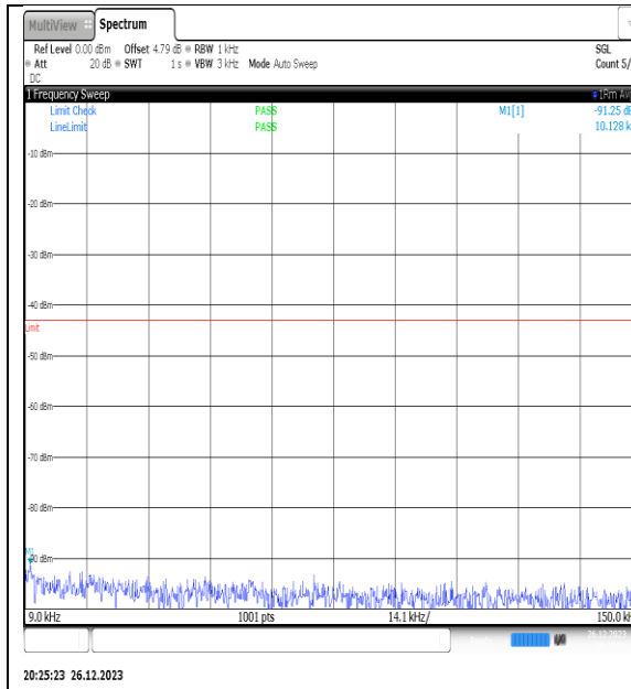
NTNV_N77-3450- 3550_PC2_30_20_M_TID11_NS_01_0.009_0.15_ #1
