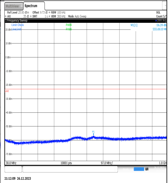
NTNV_N77-3450- 3550_PC2_30_20_H_TID7_NS_01_30_1000_#1
