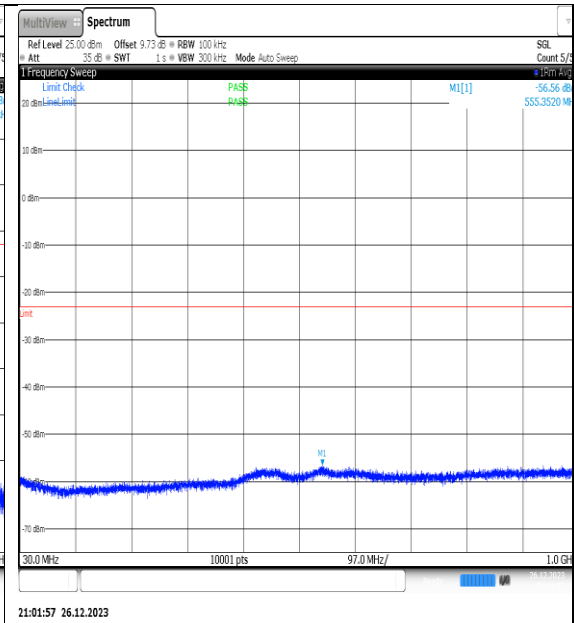
NTNV_N77-3450- 3550_PC2_30_20_H_TID5_NS_01_30_1000_#1
