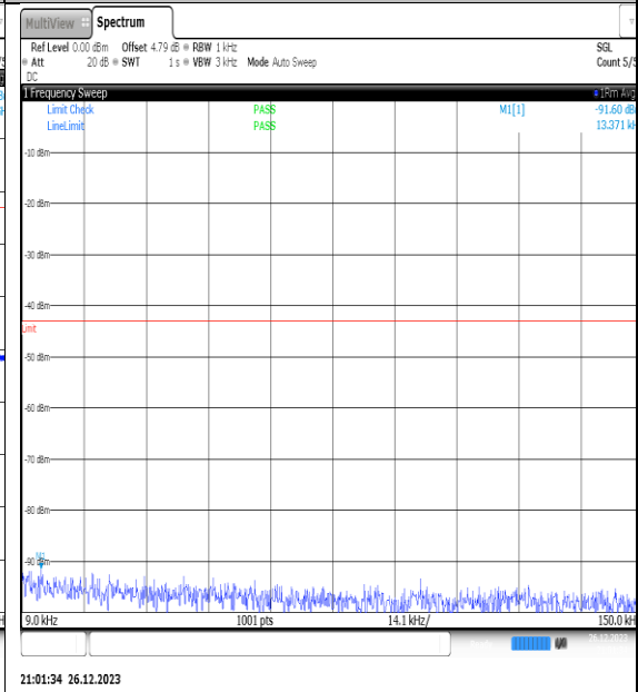
NTNV_N77-3450- 3550_PC2_30_20_H_TID5_NS_01_0.009_0.15_# 1
