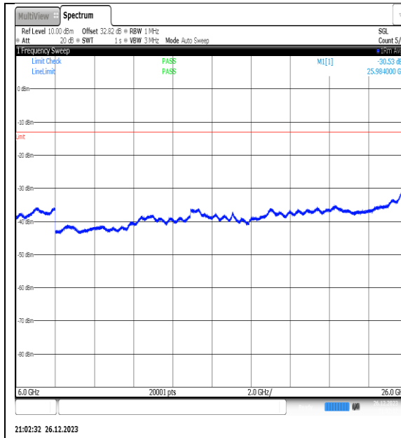
NTNV_N77-3450- 3550_PC2_30_20_H_TID5_NS_01_6000_26000_#1
