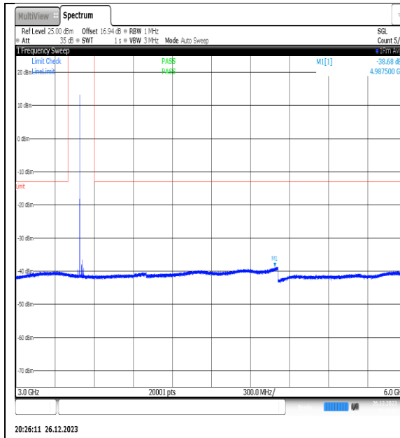
NTNV_N77-3450- 3550_PC2_30_20_M_TID11_NS_01_3000_6000_ #1
