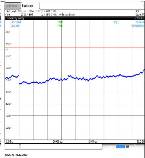
NTNV_N77-3450- 3550_PC2_30_20_M_TID11_NS_01_6000_26000 #1
