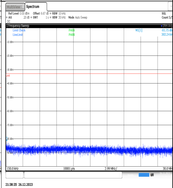
NTNV_N77-3450- 3550_PC2_30_20_H_TID14_NS_01_0.15_30_#1
