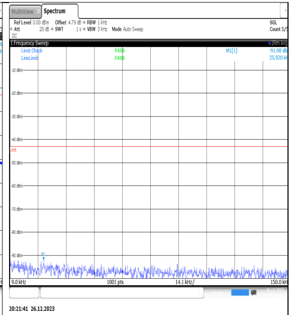
NTNV_N77-3450- 3550_PC2_30_20_M_TID10_NS_01_0.009_0.15_ #1
