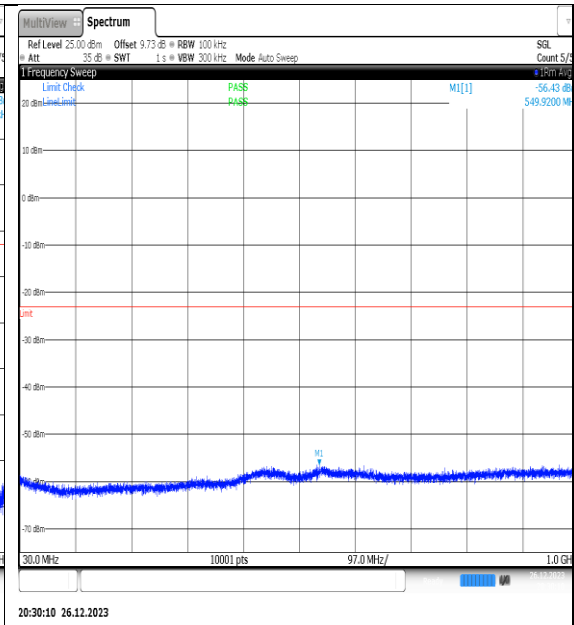
NTNV_N77-3450-3550_PC2_30_20_M_TID12_NS_01_30_1000_#1
