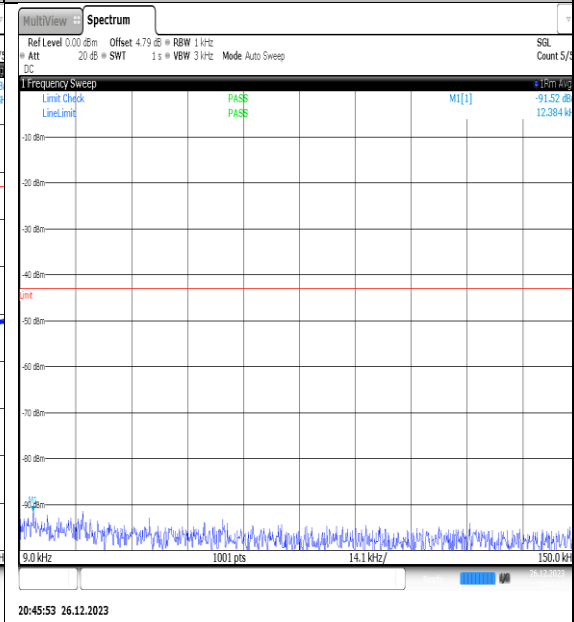
NTNV_N77-3450- 3550_PC2_30_20_H_TID1_NS_01_0.009_0.15_# 1
