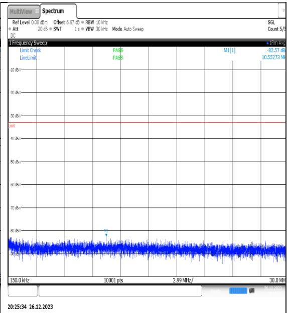
NTNV_N77-3450- 3550_PC2_30_20_M_TID11_NS_01_0.15_30_#1
