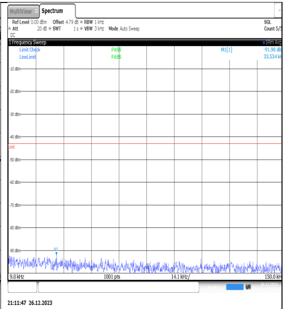
NTNV_N77-3450- 3550_PC2_30_20_H_TID7_NS_01_0.009_0.15_# 1
