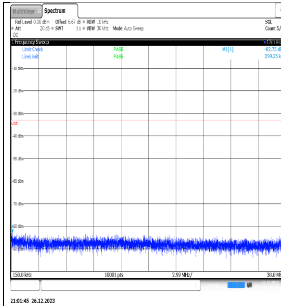
NTNV_N77-3450- 3550_PC2_30_20_H_TID5_NS_01_0.15_30_#1
