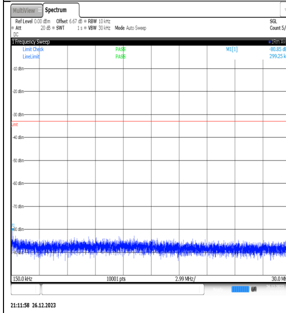
NTNV_N77-3450- 3550_PC2_30_20_H_TID7_NS_01_0.15_30_#1
