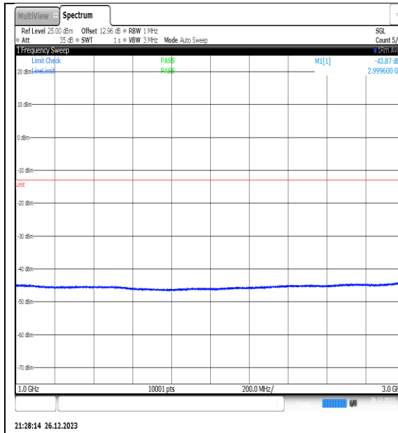
NTNV_N77-3450- 3550_PC2_30_20_H_TID11_NS_01_1000_3000_ #1
