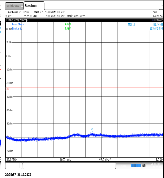
NTNV_N77-3450- 3550_PC2_30_20_M_TID14_NS_01_30_1000_#1
