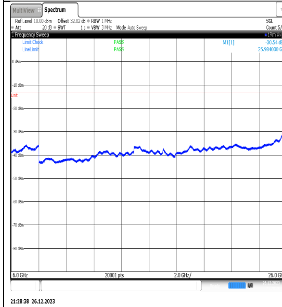
NTNV_N77-3450- 3550_PC2_30_20_H_TID11_NS_01_6000_26000_ #1
