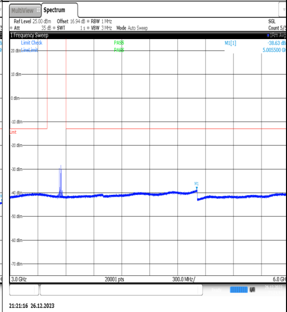
NTNV_N77-3450- 3550_PC2_30_20_H_TID9_NS_01_3000_6000_#1
