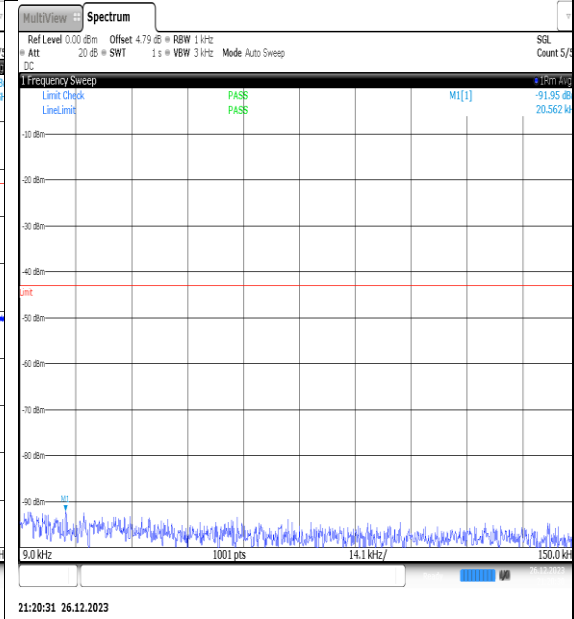
NTNV_N77-3450- 3550_PC2_30_20_H_TID9_NS_01_0.009_0.15_# 1
