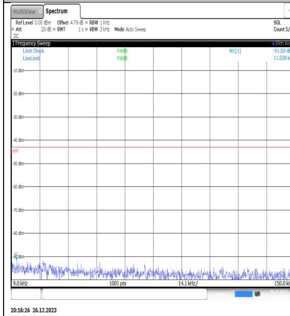
NTNV_N77-3450- 3550_PC2_30_20_M_TID9_NS_01_0.009_0.15_# 1
