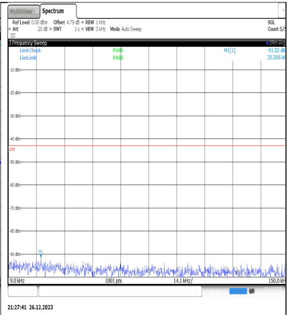
NTNV_N77-3450- 3550_PC2_30_20_H_TID11_NS_01_0.009_0.15_#1
