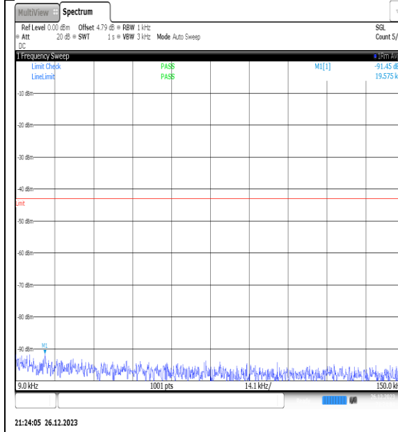
NTNV_N77-3450- 3550_PC2_30_20_H_TID10_NS_01_0.009_0.15_#1
