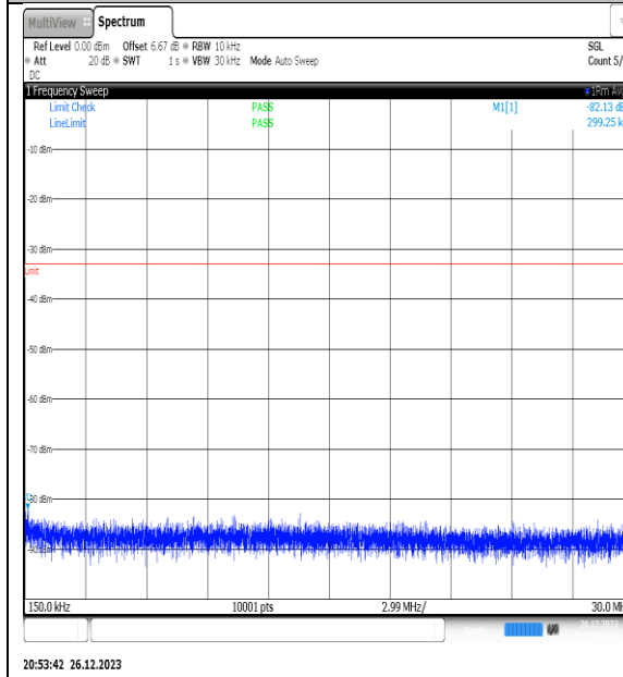
NTNV_N77-3450- 3550_PC2_30_20_H_TID3_NS_01_0.15_30_#1
