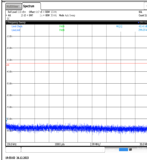
NTNV_N77-3450- 3550_PC2_30_20_M_TID6_NS_01_0.15_30_#1
