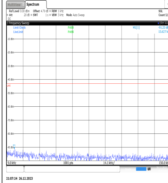
NTNV_N77-3450- 3550_PC2_30_20_H_TID6_NS_01_0.009_0.15_#1
