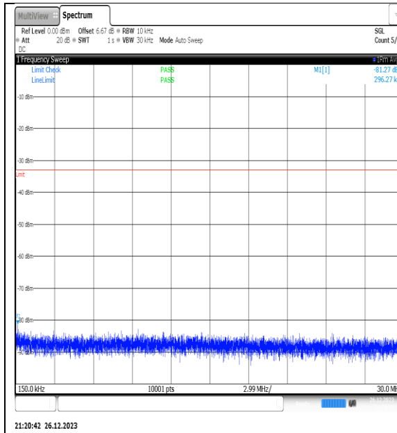
NTNV_N77-3450- 3550_PC2_30_20_H_TID9_NS_01_0.15_30_#1
