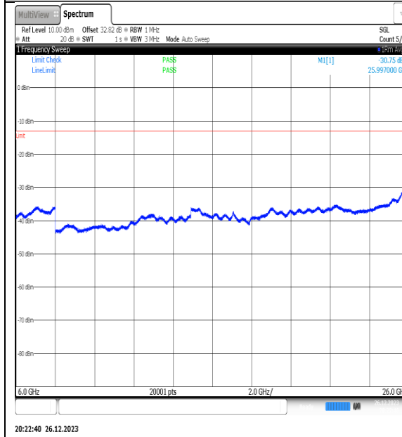
NTNV_N77-3450- 3550_PC2_30_20_M_TID10_NS_01_6000_26000_ #1
