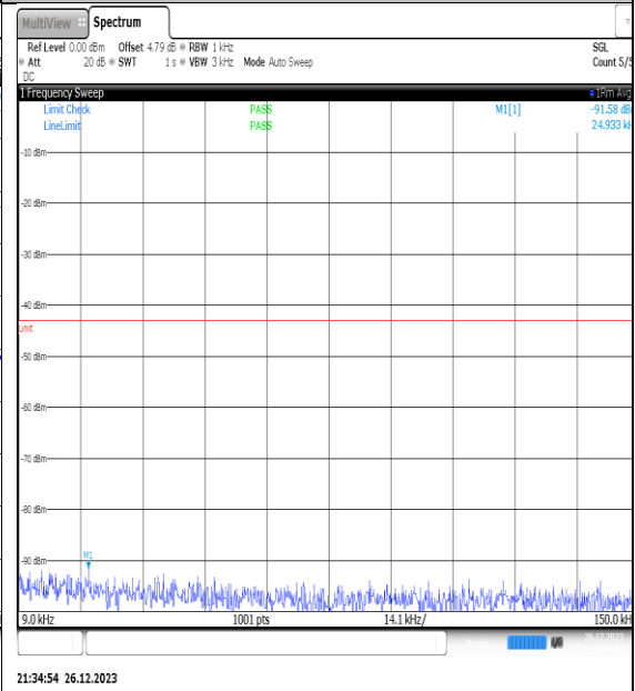
NTNV_N77-3450- 3550_PC2_30_20_H_TID13_NS_01_0.009_0.15_#1
