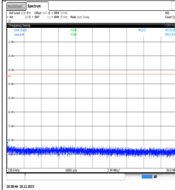
NTNV_N77-3450- 3550_PC2_30_20_M_TID14_NS_01_0.15_30_#1
