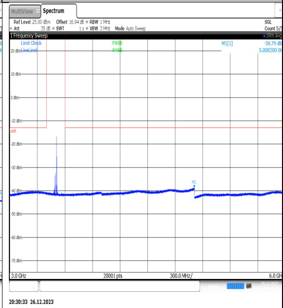
NTNV_N77-3450-3550_PC2_30_20_M_TID12_NS_01_3000_6000_#1
