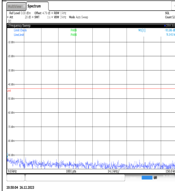
NTNV_N77-3450- 3550_PC2_30_20_H_TID2_NS_01_0.009_0.15_#1
