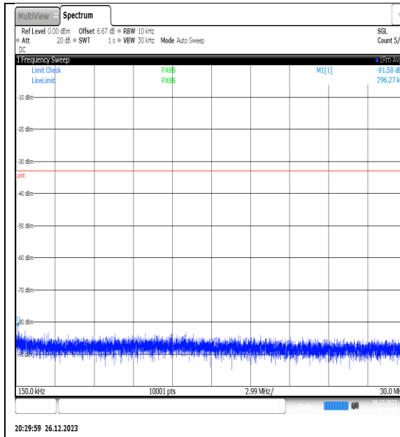
NTNV_N77-3450-3550_PC2_30_20_M_TID12_NS_01_0.15_30_#1
