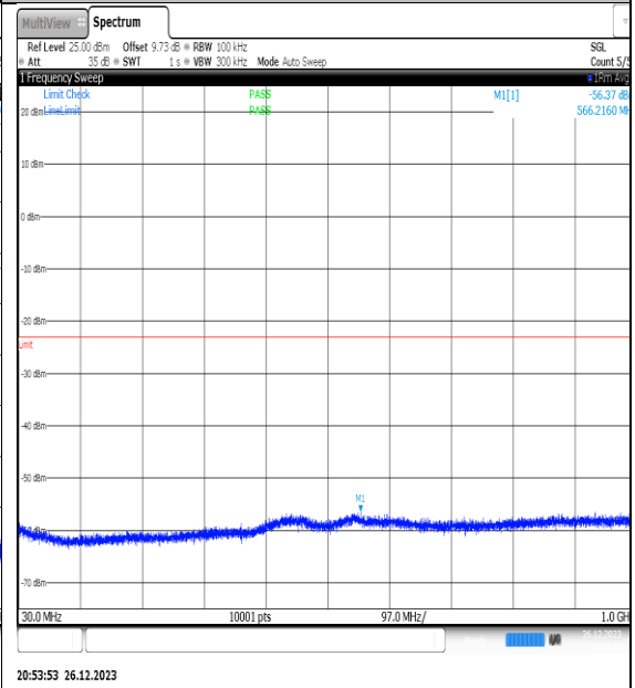
NTNV_N77-3450- 3550_PC2_30_20_H_TID3_NS_01_30_1000_#1
