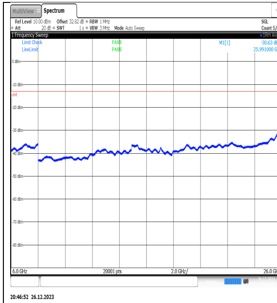
NTNV_N77-3450- 3550_PC2_30_20_H_TID1_NS_01_6000_26000_#1
