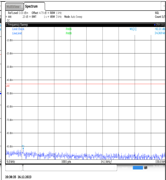
NTNV_N77-3450- 3550_PC2_30_20_M_TID14_NS_01_0.009_0.15_ #1
