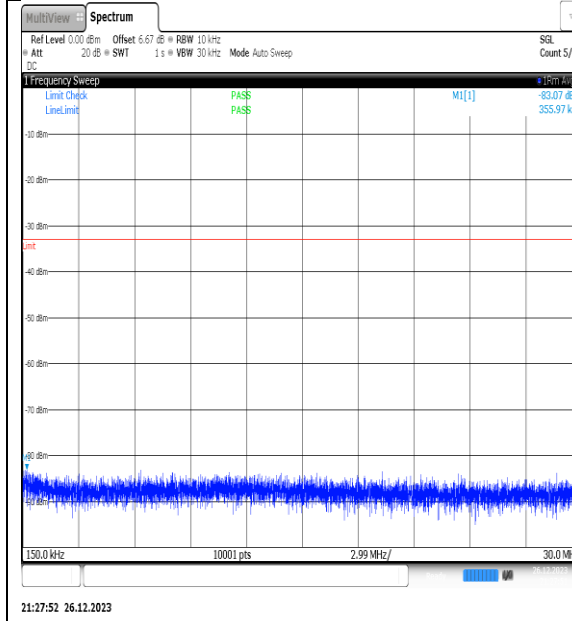
NTNV_N77-3450- 3550_PC2_30_20_H_TID11_NS_01_0.15_30_#1
