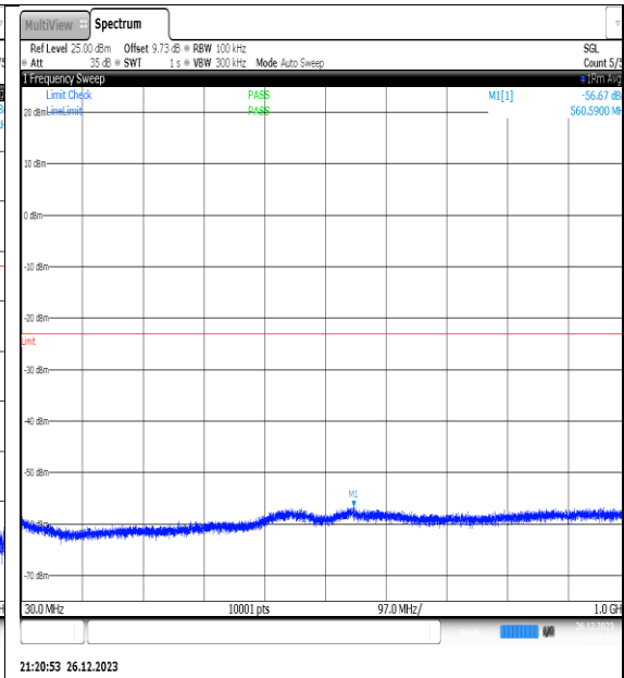
NTNV_N77-3450- 3550_PC2_30_20_H_TID9_NS_01_30_1000_#1
