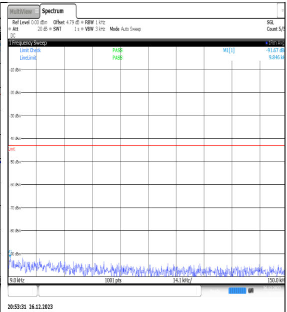
NTNV_N77-3450- 3550_PC2_30_20_H_TID3_NS_01_0.009_0.15_# 1
