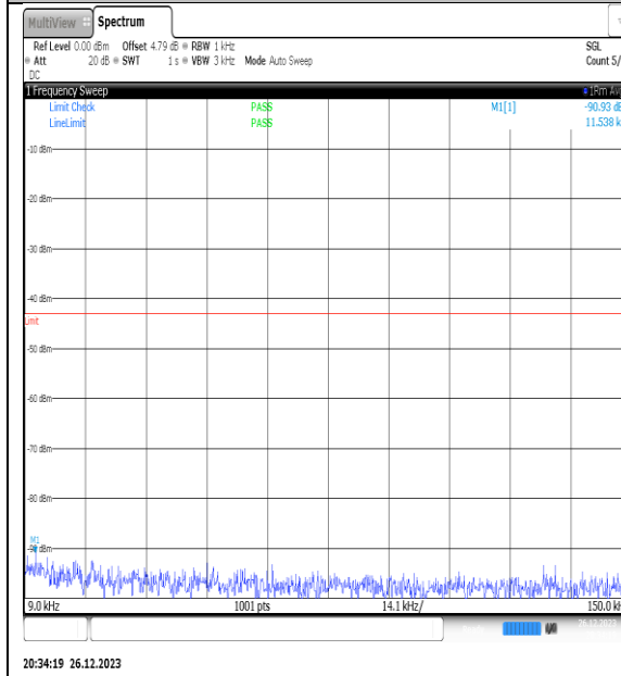
NTNV_N77-3450- 3550_PC2_30_20_M_TID13_NS_01_0.009_0.15_ _#1
