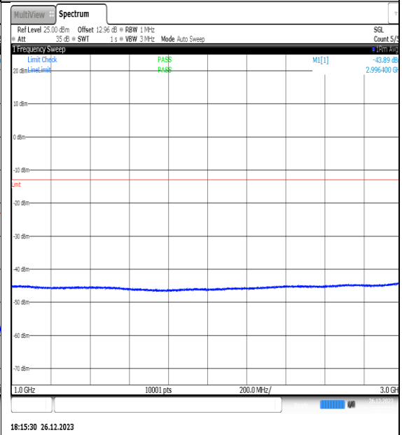
NTN_V_N77-3450- 3550_PC2_30_15_H_TID13_NS_01_1000_3000_ #1
