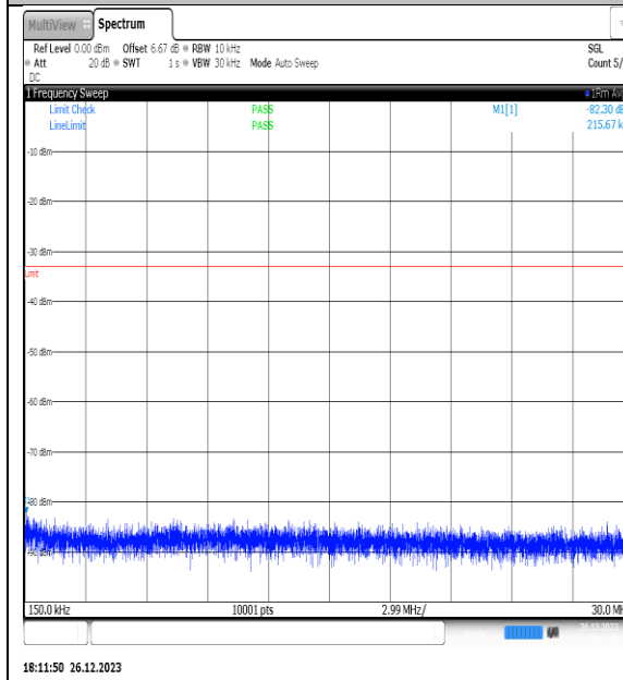
NTNV_N77-3450- 3550_PC2_30_15_H_TID12_NS_01_0.15_30_#1
