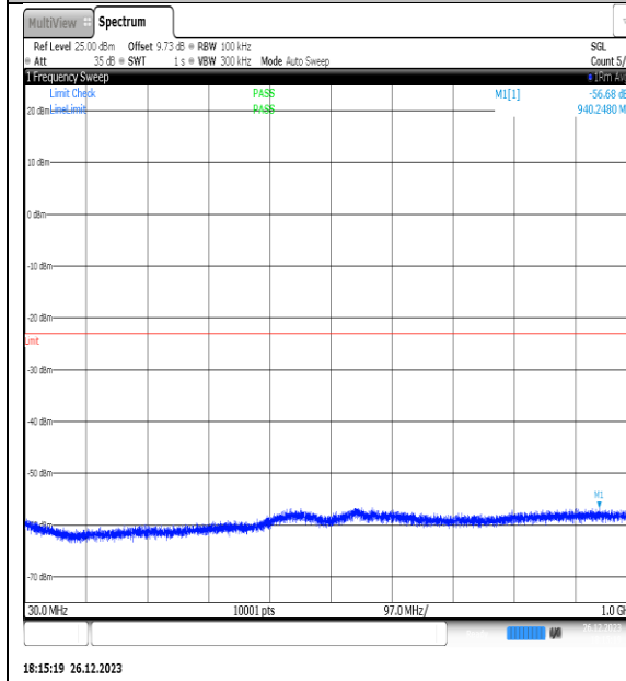
NTN_V_N77-3450- 3550_PC2_30_15_H_TID13_NS_01_30_1000_#1
