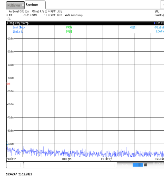
NTNV_N77-3450- 3550_PC2_30_20_L_TID4_NS_01_0.009_0.15_# 1
