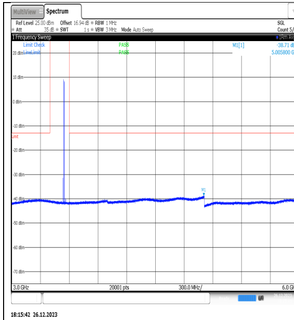
NTNV_N77-3450- 3550_PC2_30_15_H_TID13_NS_01_3000_6000_#1
