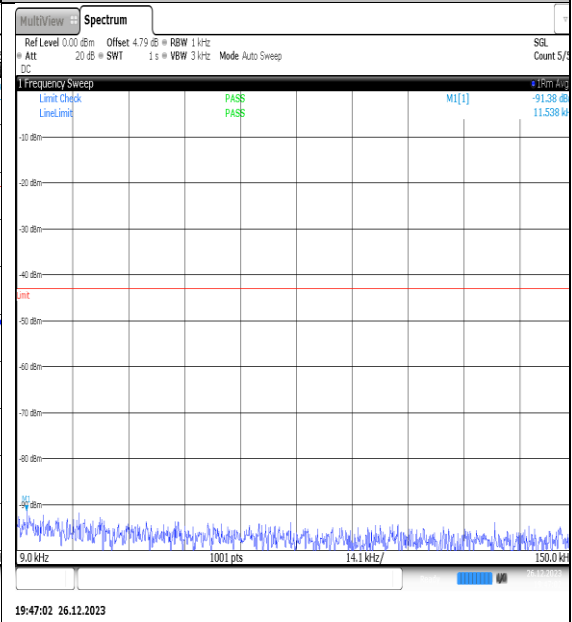
NTNV_N77-3450- 3550_PC2_30_20_M_TID4_NS_01_0.009_0.15_# 1
