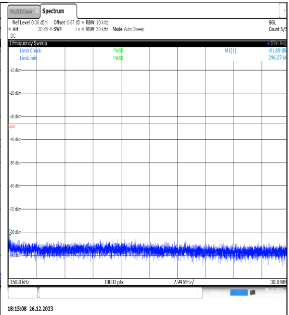
NTN_V_N77-3450- 3550_PC2_30_15_H_TID13_NS_01_0.15_30_#1
