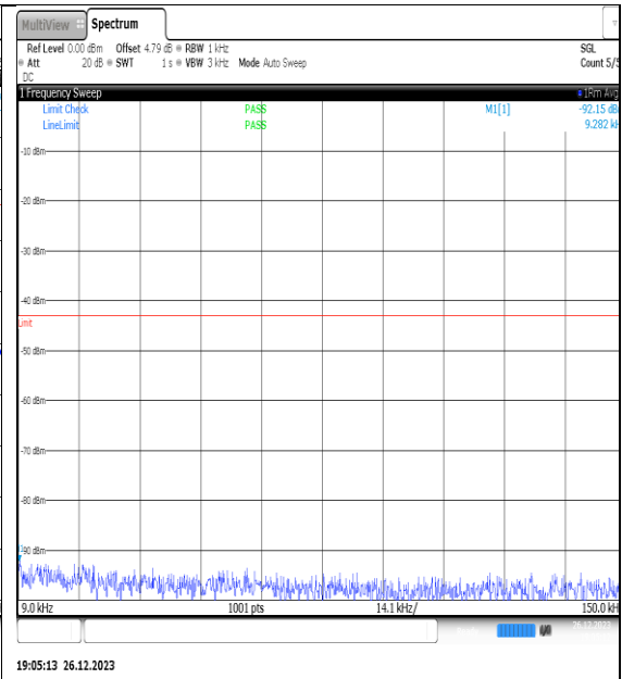
NTNV_N77-3450- 3550_PC2_30_20_L_TID9_NS_01_0.009_0.15_# 1
