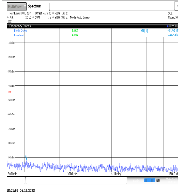
NTNV_N77-3450- 3550_PC2_30_15_H_TID15_NS_01_0.009_0.15_#1
