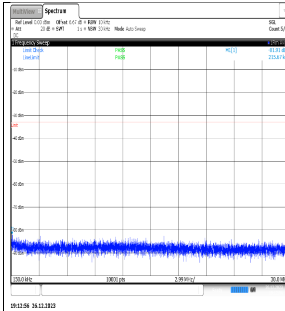
NTNV_N77-3450- 3550_PC2_30_20_L_TID11_NS_01_0.15_30_#1
