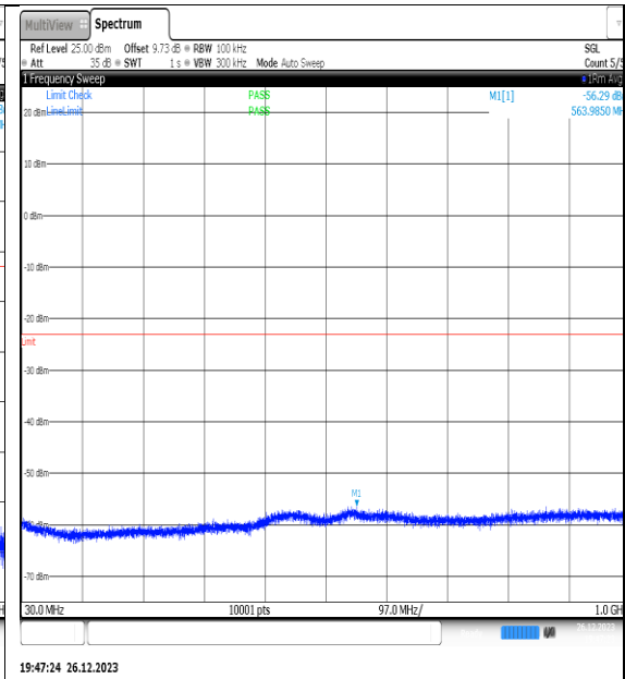
NTNV_N77-3450- 3550_PC2_30_20_M_TID4_NS_01_30_1000_#1
