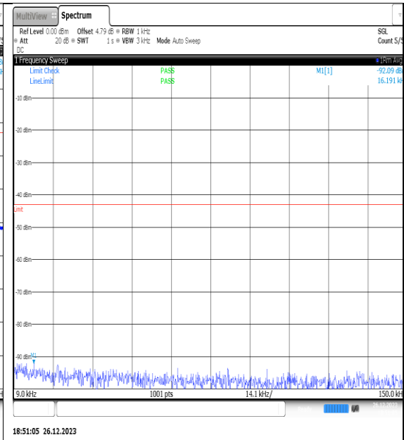
NTNV_N77-3450- 3550_PC2_30_20_L_TID5_NS_01_0.009_0.15_# 1
