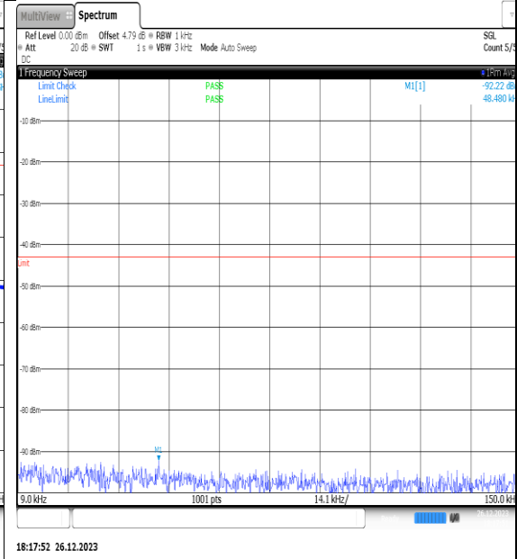
NTNV_N77-3450- 3550_PC2_30_15_H_TID14_NS_01_0.009_0.15_#1
