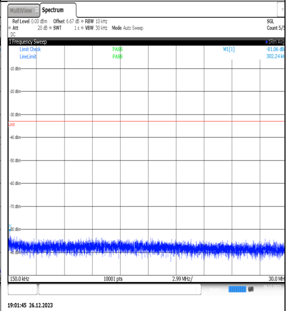
NTNV_N77-3450- 3550_PC2_30_20_L_TID8_NS_01_0.15_30_#1
