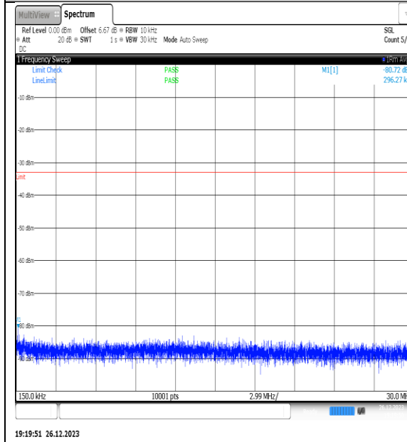
NTNV_N77-3450- 3550_PC2_30_20_L_TID13_NS_01_0.15_30_#1
