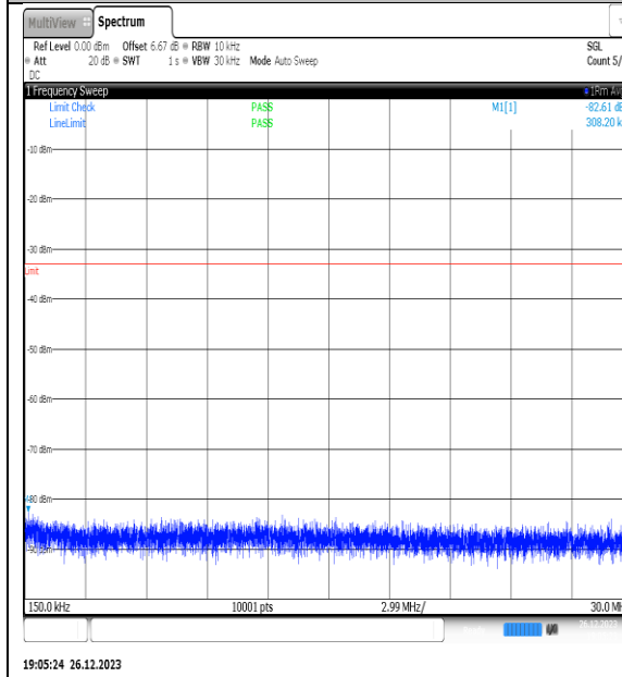
NTNV_N77-3450- 3550_PC2_30_20_L_TID9_NS_01_0.15_30_#1
