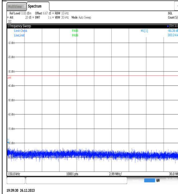
NTNV_N77-3450- 3550_PC2_30_20_M_TID2_NS_01_0.15_30_#1
