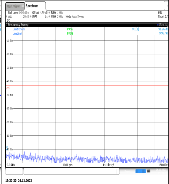
NTNV_N77-3450- 3550_PC2_30_20_L_TID15_NS_01_0.009_0.15_ #1
