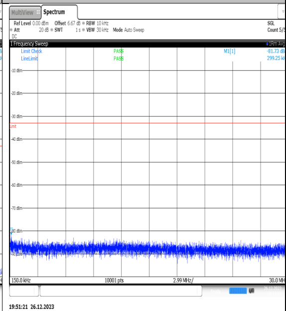
NTNV_N77-3450- 3550_PC2_30_20_M_TID5_NS_01_0.15_30_#1
