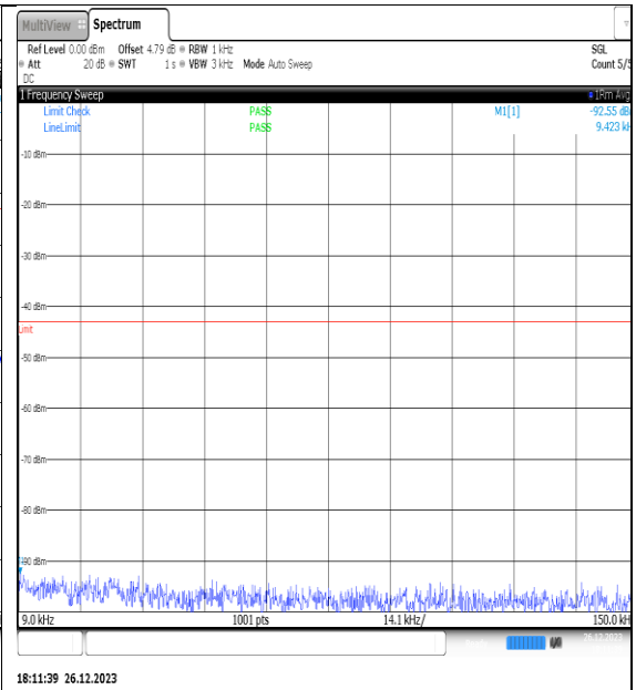
NTNV_N77-3450- 3550_PC2_30_15_H_TID12_NS_01_0.009_0.15_ #1
