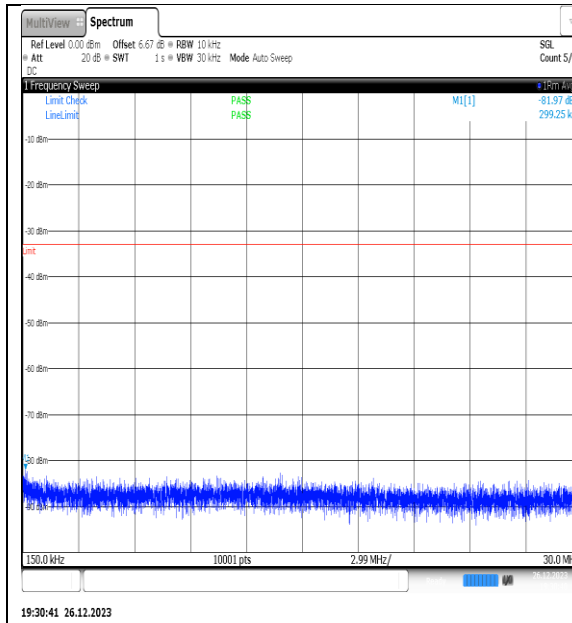
NTNV_N77-3450-3550_PC2_30_20_L_TID15_NS_01_0.15_30_#1
