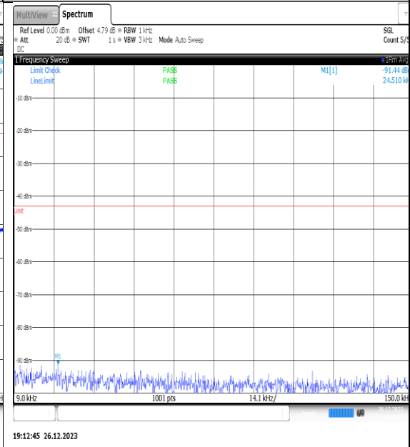
NTNV_N77-3450- 3550_PC2_30_20_L_TID11_NS_01_0.009_0.15_ #1
