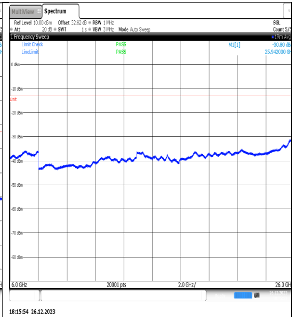
NTNV_N77-3450- 3550_PC2_30_15_H_TID13_NS_01_6000_26000_#1
