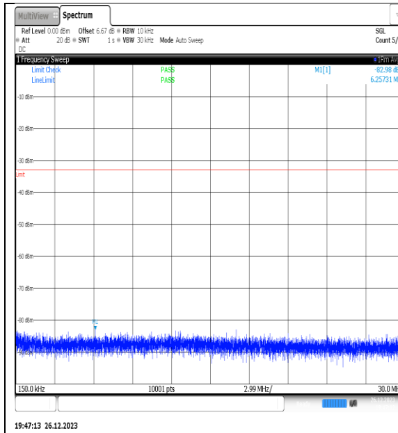
NTNV_N77-3450- 3550_PC2_30_20_M_TID4_NS_01_0.15_30_#1
