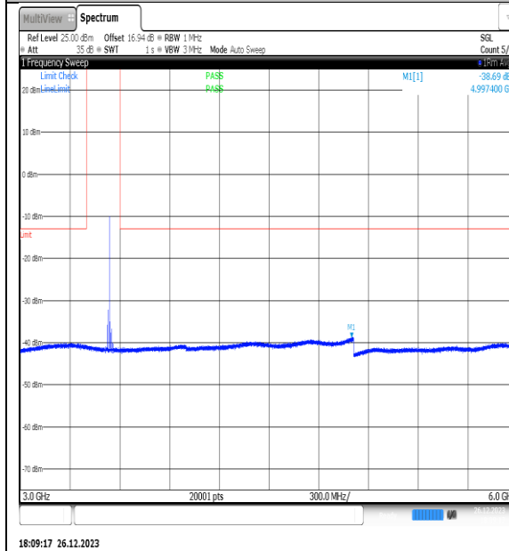
NTNV_N77-3450- 3550_PC2_30_15_H_TID11_NS_01_3000_6000_#1
