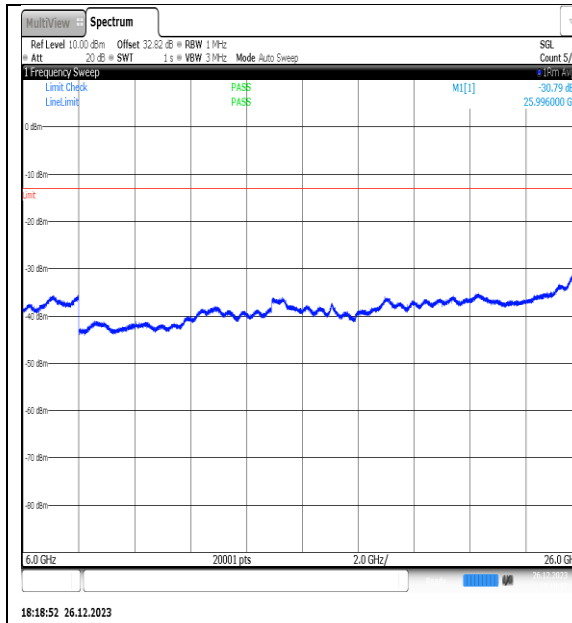
NTNV_N77-3450- 3550_PC2_30_15_H_TID14_NS_01_6000_26000 #1
