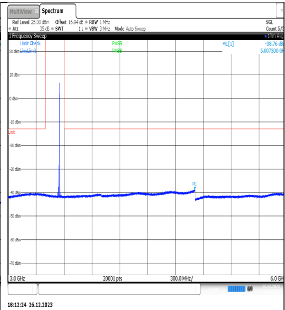
NTNV_N77-3450- 3550_PC2_30_15_H_TID12_NS_01_3000_6000_ #1
