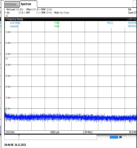
NTNV_N77-3450- 3550_PC2_30_20_L_TID4_NS_01_0.15_30_#1
