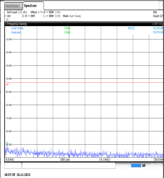
NTNV_N77-3450- 3550_PC2_30_20_L_TID7_NS_01_0.009_0.15_#1
