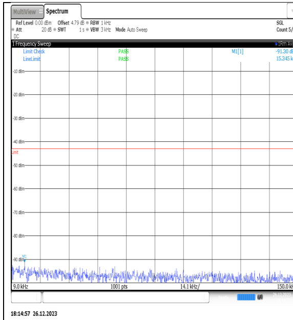
NTN_V_N77-3450- 3550_PC2_30_15_H_TID13_NS_01_0.009_0.15_ #1
