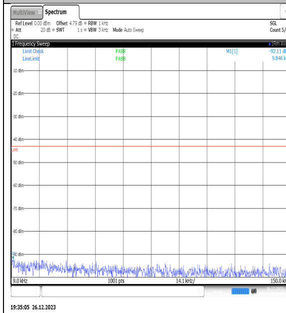
NTNV_N77-3450- 3550_PC2_30_20_M_TID1_NS_01_0.009_0.15_# 1
