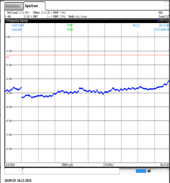
NTNV_N77-3450- 3550_PC2_30_15_H_TID11_NS_01_6000_26000_#1
