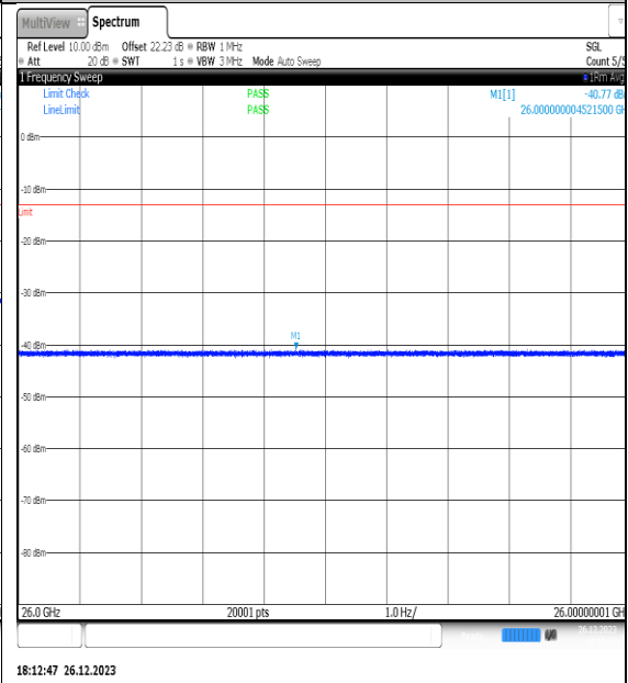
NTNV_N77-3450- 3550_PC2_30_15_H_TID12_NS_01_26000_4000_0_ #1
