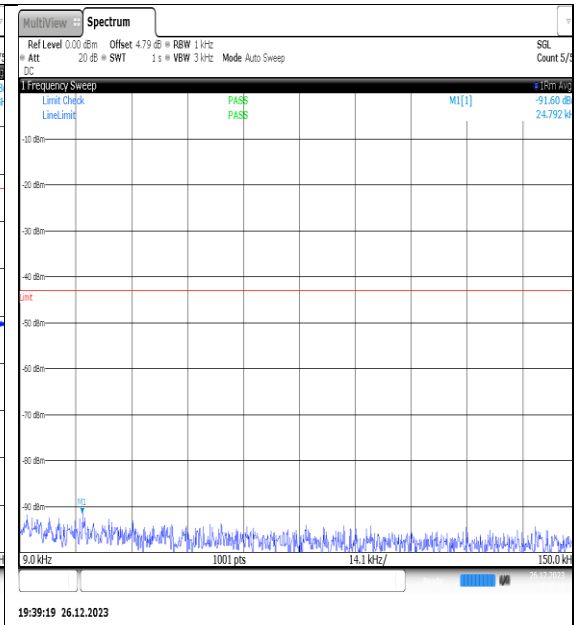
NTNV_N77-3450- 3550_PC2_30_20_M_TID2_NS_01_0.009_0.15_# 1
