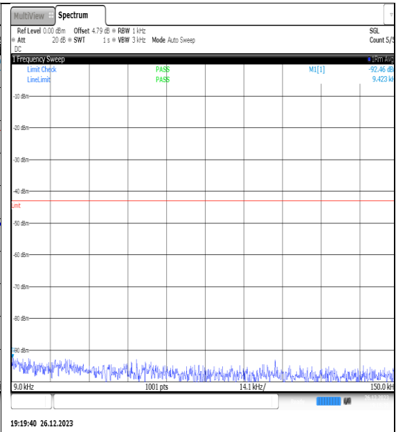
NTNV_N77-3450- 3550_PC2_30_20_L_TID13_NS_01_0.009_0.15_ #1
