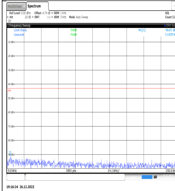
NTNV_N77-3450- 3550_PC2_30_20_L_TID12_NS_01_0.009_0.15_#1
