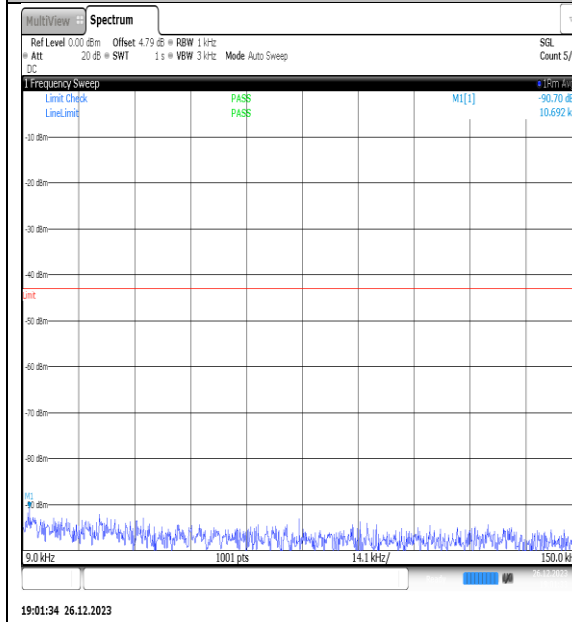
NTNV_N77-3450- 3550_PC2_30_20_L_TID8_NS_01_0.009_0.15_# 1
