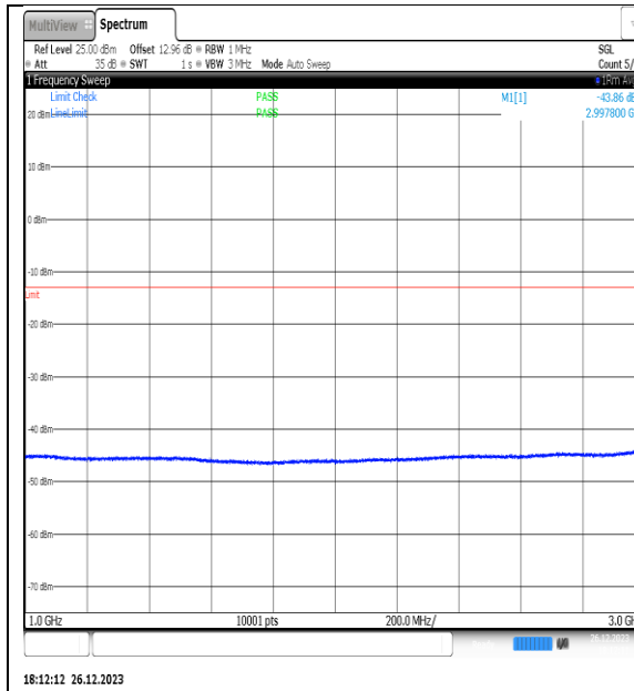
NTNV_N77-3450- 3550_PC2_30_15_H_TID12_NS_01_1000_3000_ #1
