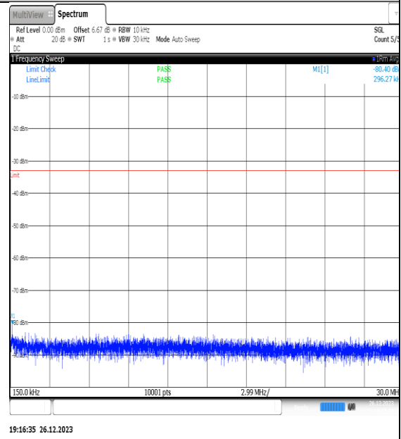
NTNV_N77-3450- 3550_PC2_30_20_L_TID12_NS_01_0.15_30_#1
