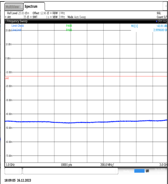
NTNV_N77-3450- 3550_PC2_30_15_H_TID11_NS_01_1000_3000_#1
