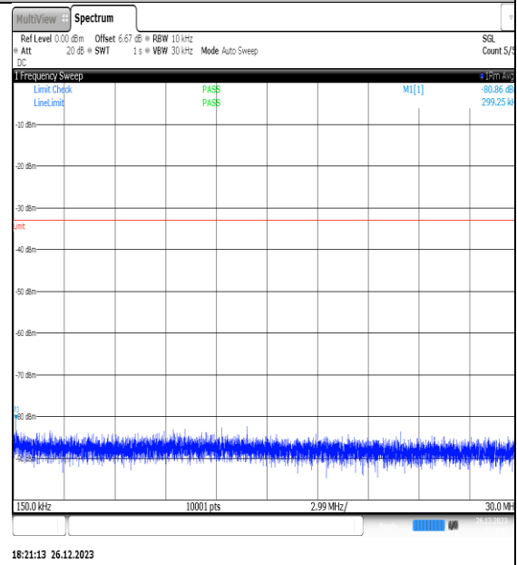
NTNV_N77-3450- 3550_PC2_30_15_H_TID15_NS_01_0.15_30_#1
