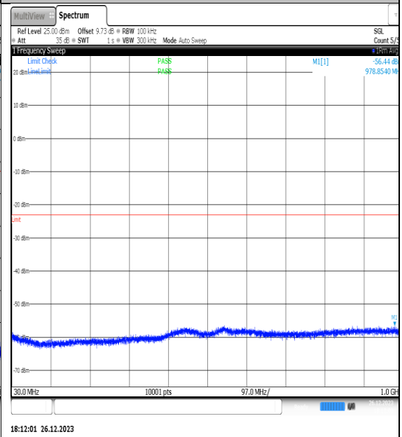
NTNV_N77-3450- 3550_PC2_30_15_H_TID12_NS_01_30_1000_#1
