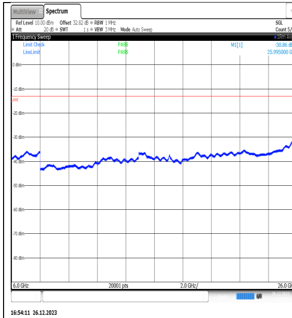
NTNV_N77-3450- 3550_PC2_30_15_M_TID9_NS_01_6000_26000_#1
