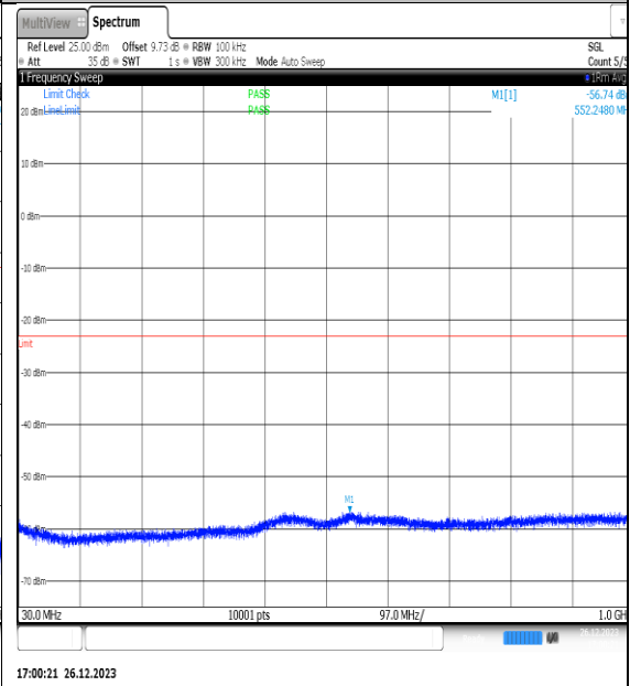
NTNV_N77-3450- 3550_PC2_30_15_M_TID11_NS_01_30_1000_#1
