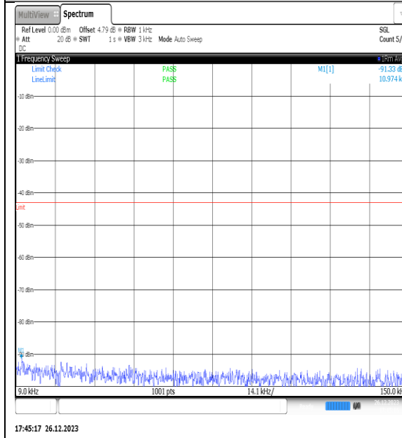
NTNV_N77-3450- 3550_PC2_30_15_H_TID7_NS_01_0.009_0.15_#1
