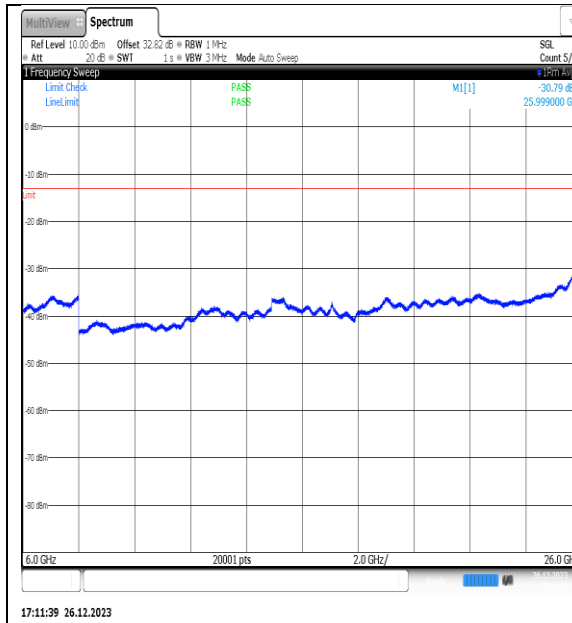
NTNV_N77-3450- 3550_PC2_30_15_M_TID13_NS_01_6000_26000 #1
