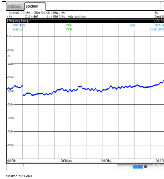
NTNV_N77-3450- 3550_PC2_30_15_M_TID5_NS_01_6000_26000_#1
