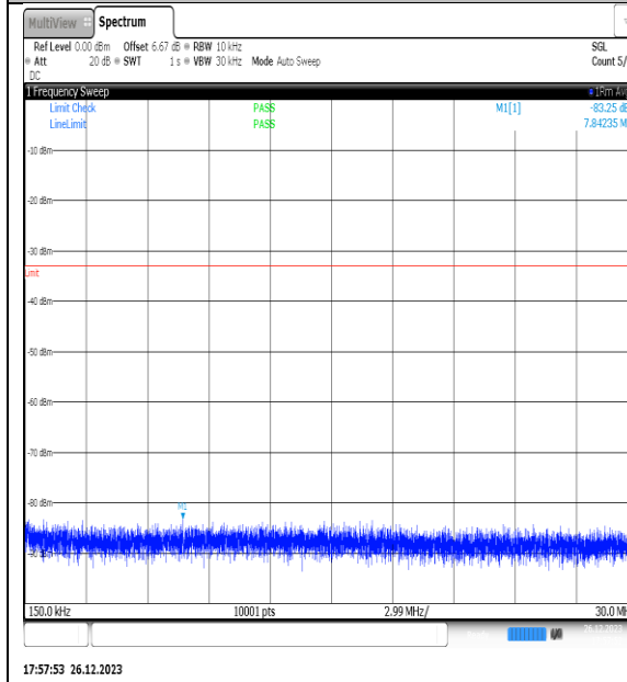
NTNV_N77-3450- 3550_PC2_30_15_H_TID8_NS_01_0.15_30_#1
