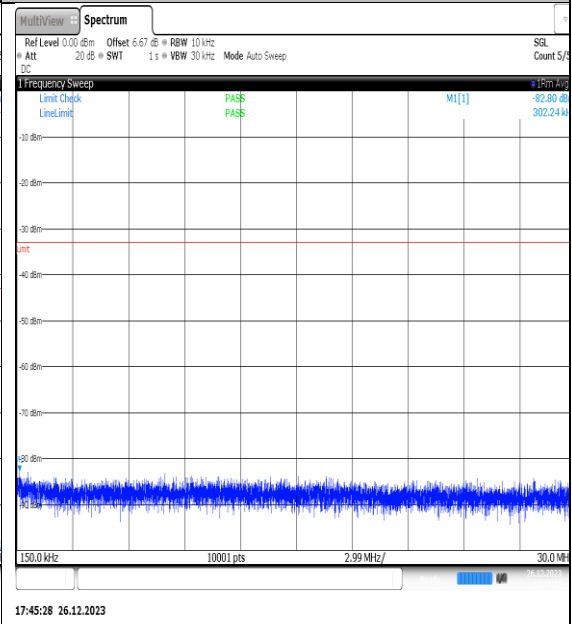
NTNV_N77-3450- 3550_PC2_30_15_H_TID7_NS_01_0.15_30_#1
