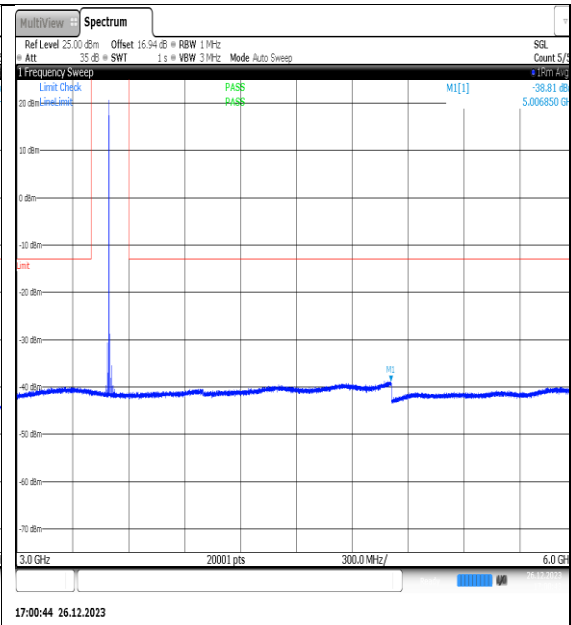
NTNV_N77-3450- 3550_PC2_30_15_M_TID11_NS_01_3000_6000_#1
