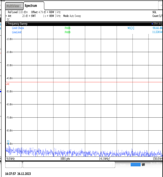
NTNV_N77-3450- 3550_PC2_30_15_M_TID5_NS_01_0.009_0.15_# 1
