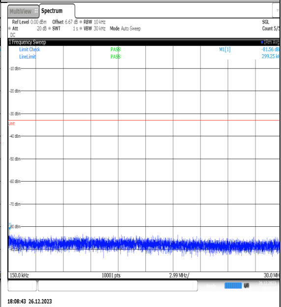
NTNV_N77-3450- 3550_PC2_30_15_H_TID11_NS_01_0.15_30_#1
