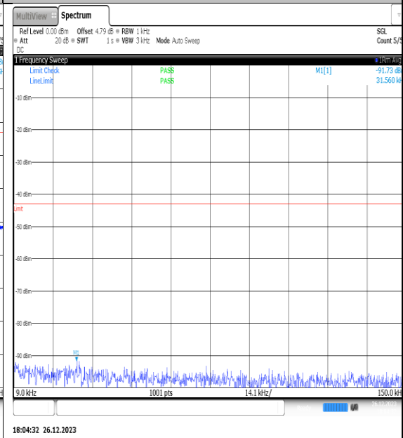
NTNV_N77-3450- 3550_PC2_30_15_H_TID10_NS_01_0.009_0.15_# 1
