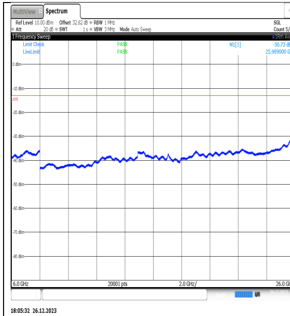
NTNV_N77-3450- 3550_PC2_30_15_H_TID10_NS_01_6000_26000 #1
