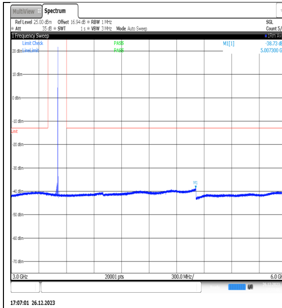
NTN_V_N77-3450- 3550_PC2_30_15_M_TID12_NS_01_3000_6000_ #1
