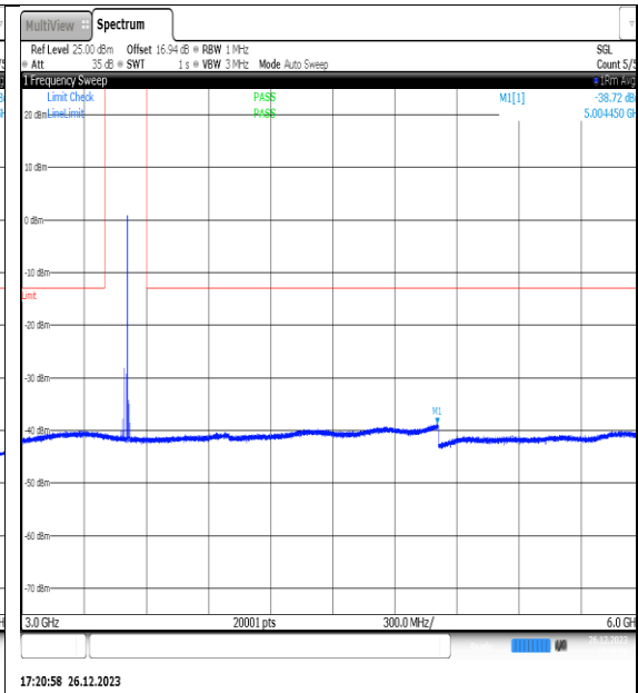
NTN_V_N77-3450- 3550_PC2_30_15_M_TID15_NS_01_3000_6000_ #1
