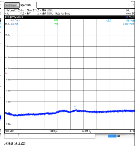
NTNV_N77-3450- 3550_PC2_30_15_M_TID5_NS_01_30_1000_#1
