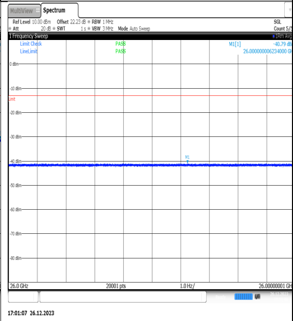
NTNV_N77-3450- 3550_PC2_30_15_M_TID11_NS_01_26000_4000_0_#1
