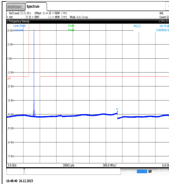
NTNV_N77-3450- 3550_PC2_30_15_M_TID8_NS_01_3000_6000_# 1
