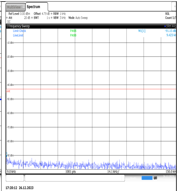
NTNV_N77-3450- 3550_PC2_30_15_M_TID15_NS_01_0.009_0.15_#1
