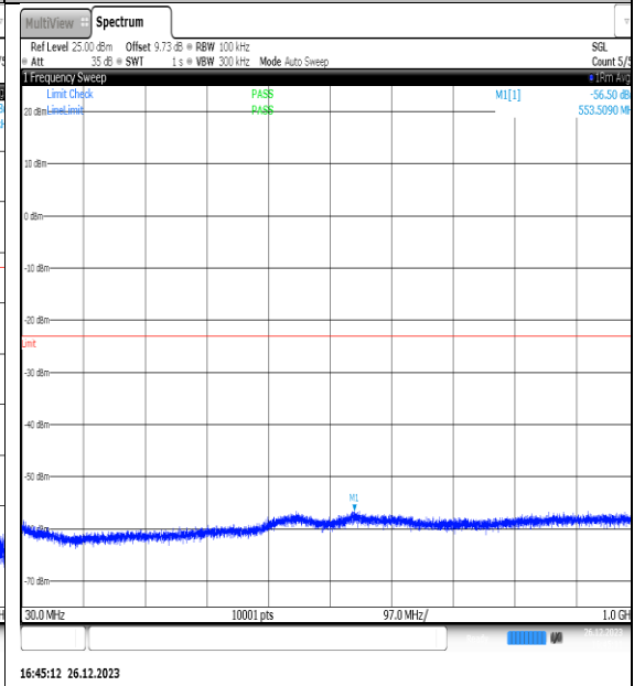
NTNV_N77-3450- 3550_PC2_30_15_M_TID7_NS_01_30_1000_#1
