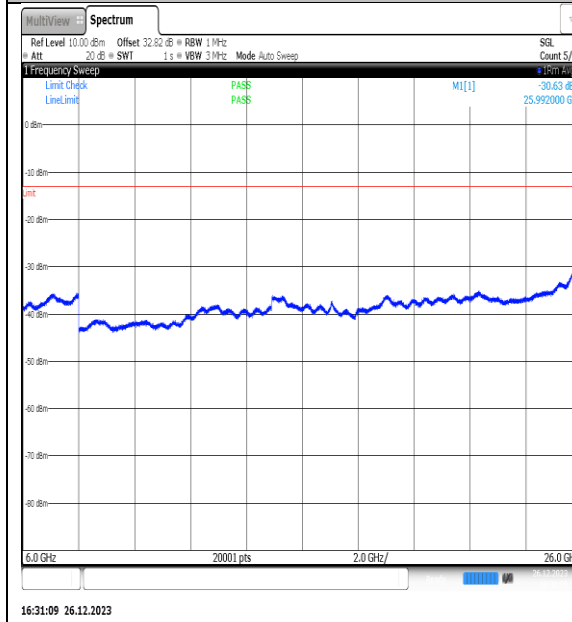
NTNV_N77-3450- 3550_PC2_30_15_M_TID3_NS_01_6000_26000_#1
