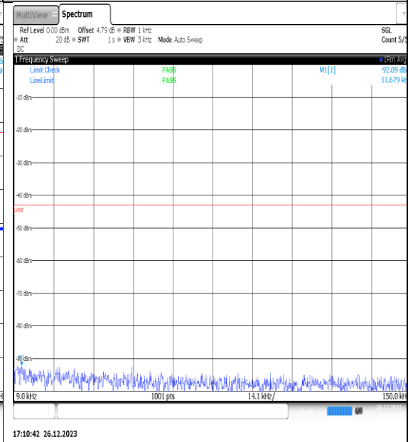
NTN_V_N77-3450- 3550_PC2_30_15_M_TID13_NS_01_0.009_0.15_ #1
