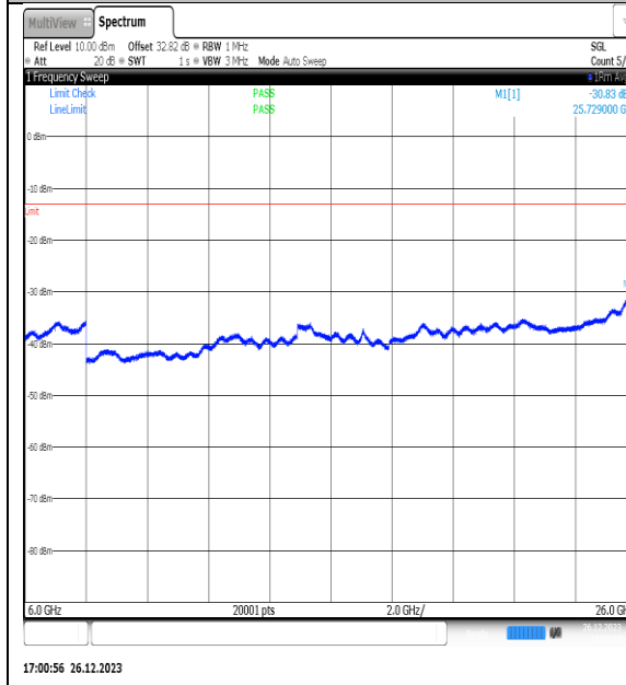
NTNV_N77-3450- 3550_PC2_30_15_M_TID11_NS_01_6000_26000_#1
