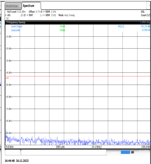
NTNV_N77-3450- 3550_PC2_30_15_M_TID7_NS_01_0.009_0.15_# 1
