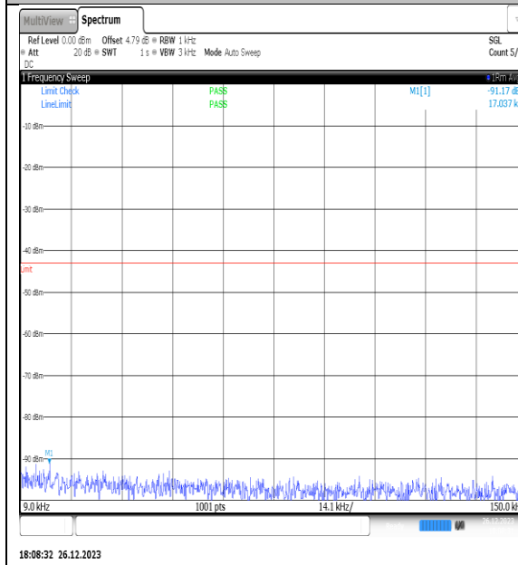
NTNV_N77-3450- 3550_PC2_30_15_H_TID11_NS_01_0.009_0.15_#1
