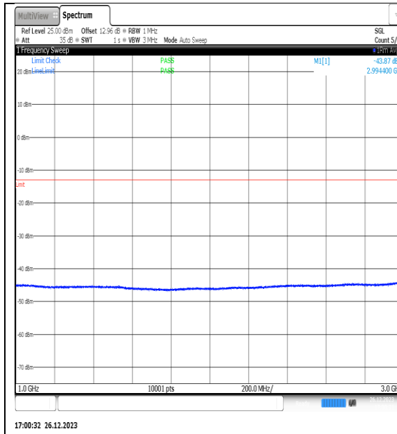
NTNV_N77-3450- 3550_PC2_30_15_M_TID11_NS_01_1000_3000_#1
