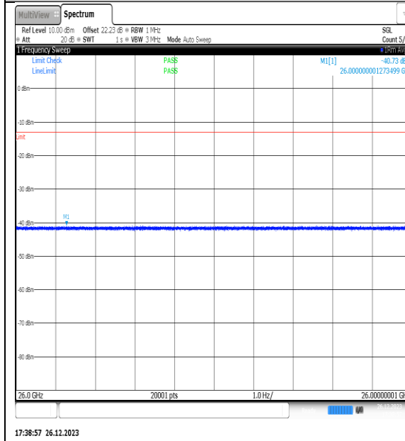
NTNV_N77-3450- 3550_PC2_30_15_H_TID5_NS_01_26000_40000_# 1
