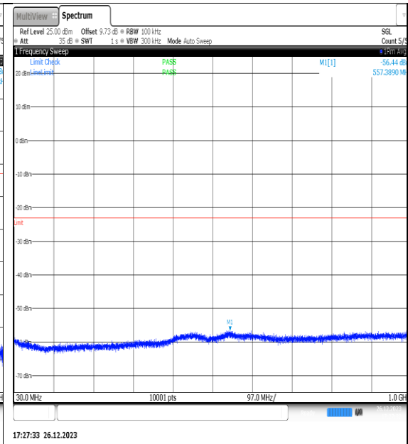
NTNV_N77-3450- 3550_PC2_30_15_H_TID2_NS_01_30_1000_#1
