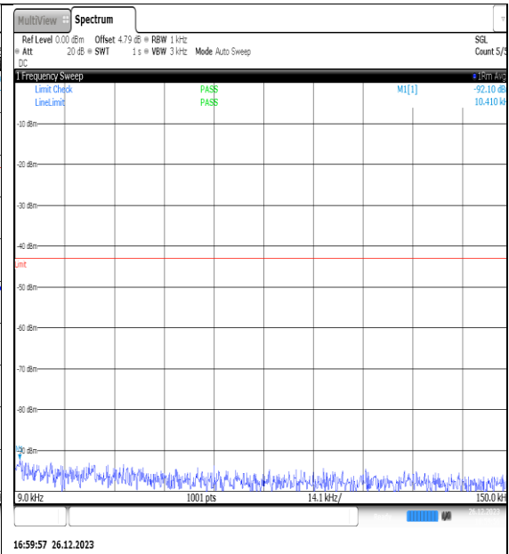
NTNV_N77-3450- 3550_PC2_30_15_M_TID11_NS_01_0.009_0.15_ #1
