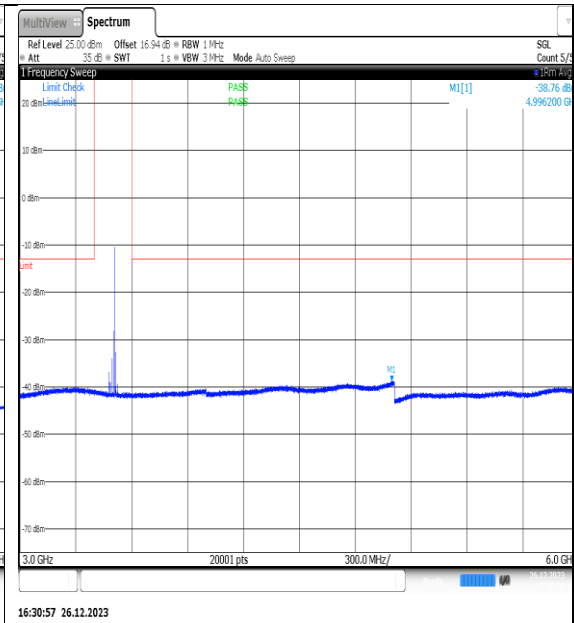
NTNV_N77-3450- 3550_PC2_30_15_M_TID3_NS_01_3000_6000_# 1
