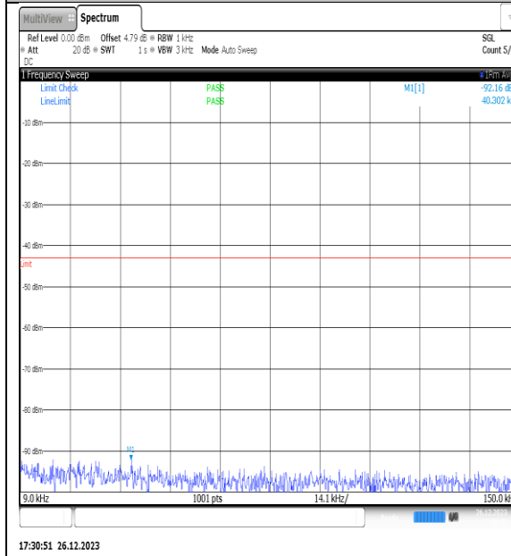
NTNV_N77-3450- 3550_PC2_30_15_H_TID3_NS_01_0.009_0.15_#1
