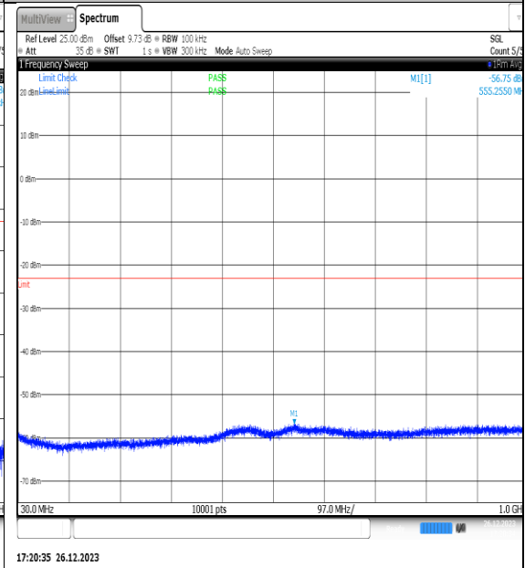
NTNV_N77-3450- 3550_PC2_30_15_M_TID15_NS_01_30_1000_#1
