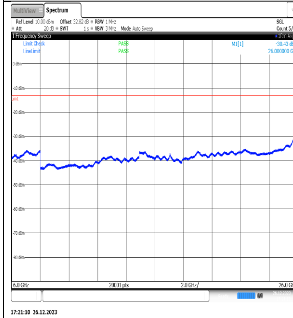
NTN_V_N77-3450- 3550_PC2_30_15_M_TID15_NS_01_6000_26000_ #1
