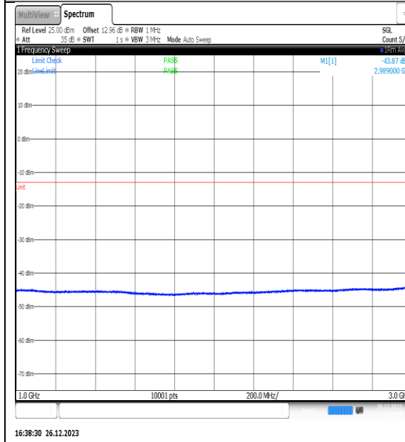
NTNV_N77-3450- 3550_PC2_30_15_M_TID5_NS_01_1000_3000_# 1
