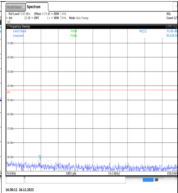
NTNV_N77-3450- 3550_PC2_30_15_M_TID3_NS_01_0.009_0.15_# 1
