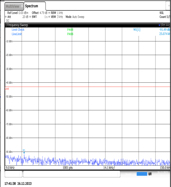
NTNV_N77-3450- 3550_PC2_30_15_H_TID6_NS_01_0.009_0.15_# 1
