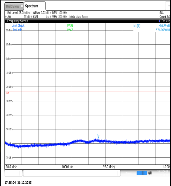
NTNV_N77-3450- 3550_PC2_30_15_H_TID8_NS_01_30_1000_#1
