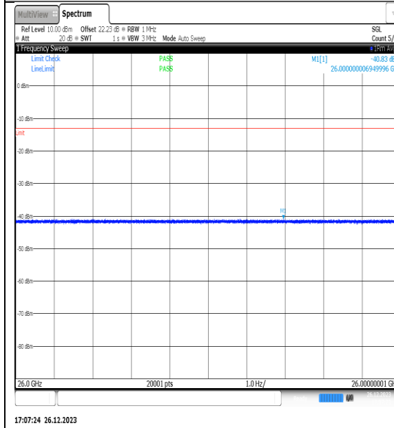
NTN_V_N77-3450- 3550_PC2_30_15_M_TID12_NS_01_26000_4000_ 0_#1
