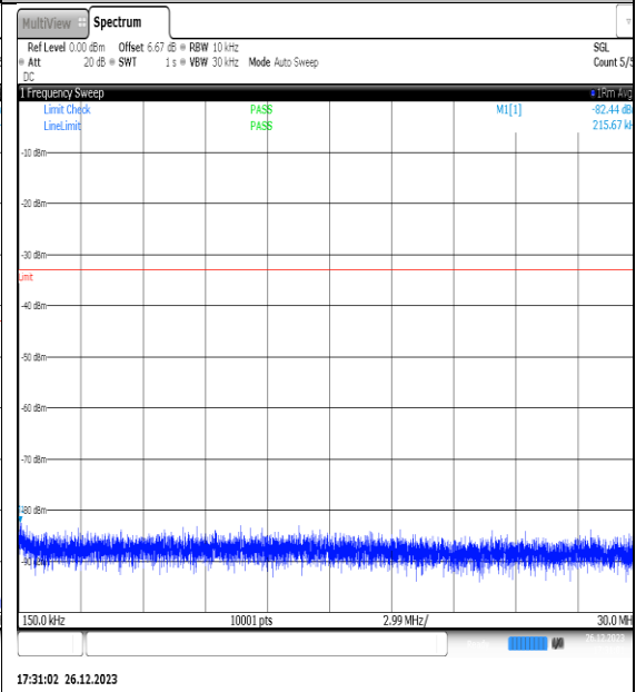
NTNV_N77-3450- 3550_PC2_30_15_H_TID3_NS_01_0.15_30_#1
