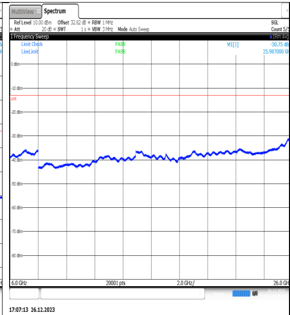
NTN_V_N77-3450- 3550_PC2_30_15_M_TID12_NS_01_6000_26000_ #1
