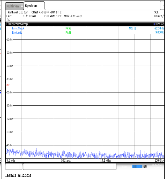
NTNV_N77-3450- 3550_PC2_30_15_M_TID9_NS_01_0.009_0.15_# 1
