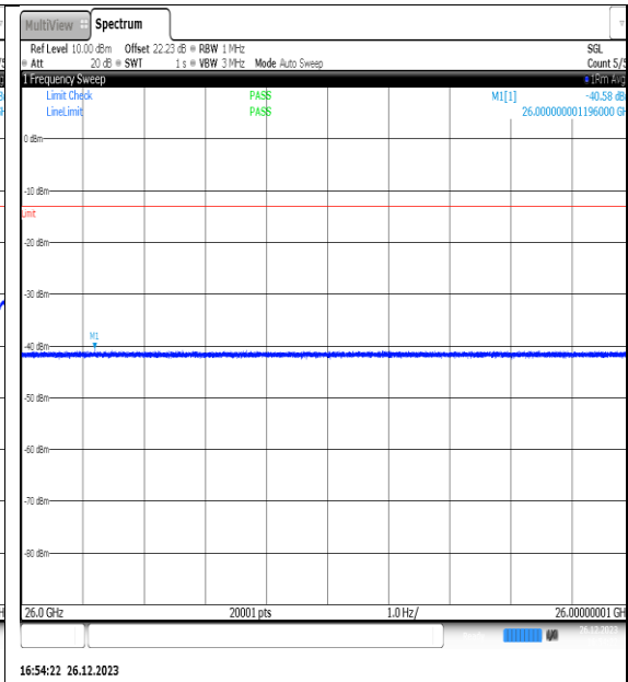
NTNV_N77-3450- 3550_PC2_30_15_M_TID9_NS_01_26000_40000_#1
