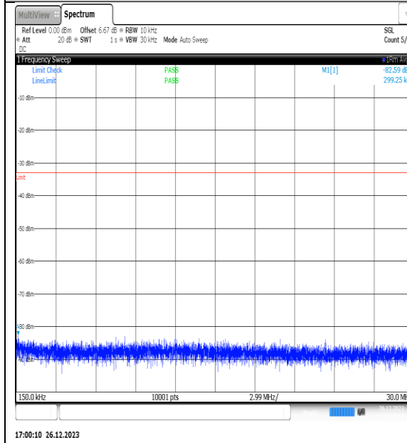
NTNV_N77-3450- 3550_PC2_30_15_M_TID11_NS_01_0.15_30_#1
