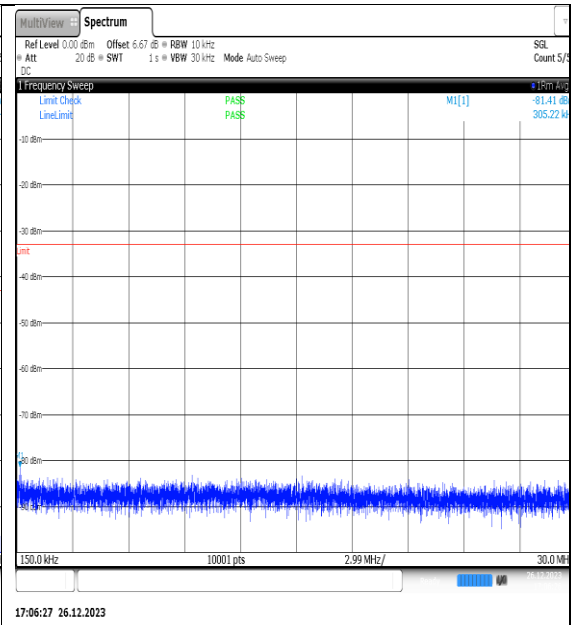
NTNV_N77-3450- 3550_PC2_30_15_M_TID12_NS_01_0.15_30_#1
