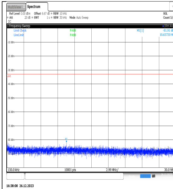
NTNV_N77-3450- 3550_PC2_30_15_M_TID5_NS_01_0.15_30_#1
