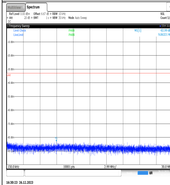
NTNV_N77-3450- 3550_PC2_30_15_M_TID3_NS_01_0.15_30_#1
