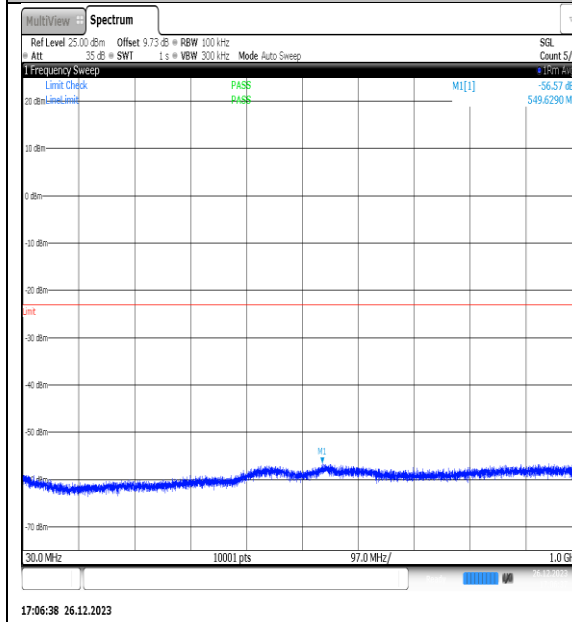
NTNV_N77-3450- 3550_PC2_30_15_M_TID12_NS_01_30_1000_#1
