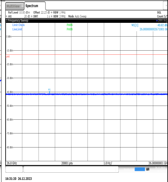
NTNV_N77-3450- 3550_PC2_30_15_M_TID3_NS_01_26000_40000_#1
