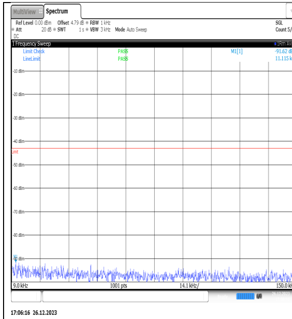
NTNV_N77-3450- 3550_PC2_30_15_M_TID12_NS_01_0.009_0.15_ #1
