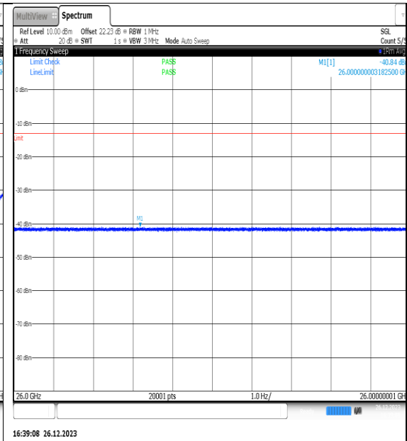
NTNV_N77-3450- 3550_PC2_30_15_M_TID5_NS_01_26000_40000_#1
