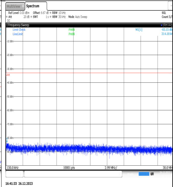
NTNV_N77-3450- 3550_PC2_30_15_M_TID6_NS_01_0.15_30_#1
