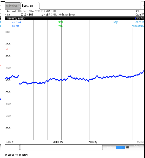
NTNV_N77-3450- 3550_PC2_30_15_M_TID8_NS_01_6000_26000_# 1
