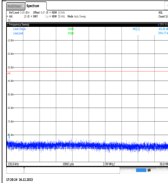
NTNV_N77-3450- 3550_PC2_30_15_M_TID15_NS_01_0.15_30_#1
