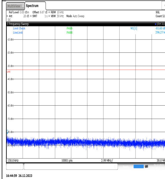
NTNV_N77-3450- 3550_PC2_30_15_M_TID7_NS_01_0.15_30_#1
