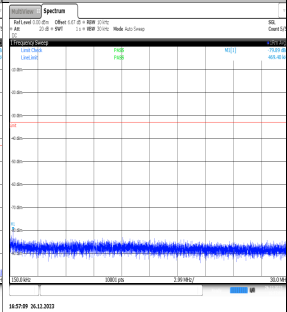
NTNV_N77-3450- 3550_PC2_30_15_M_TID10_NS_01_0.15_30_#1
