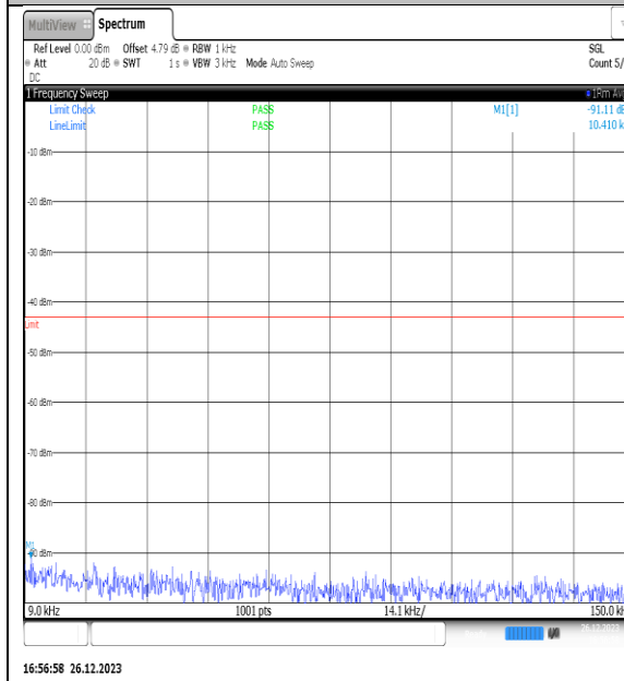
NTNV_N77-3450- 3550_PC2_30_15_M_TID10_NS_01_0.009_0.15_#1
