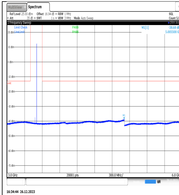
NTNV_N77-3450- 3550_PC2_30_15_M_TID4_NS_01_3000_6000_# 1
