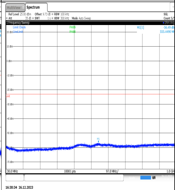
NTNV_N77-3450- 3550_PC2_30_15_M_TID3_NS_01_30_1000_#1
