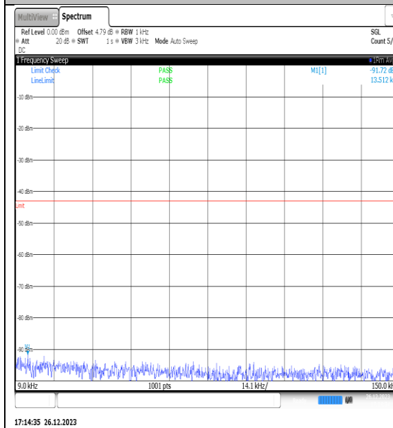
NTNV_N77-3450- 3550_PC2_30_15_M_TID14_NS_01_0.009_0.15_#1
