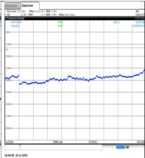
NTNV_N77-3450- 3550_PC2_30_15_M_TID4_NS_01_6000_26000_# 1
