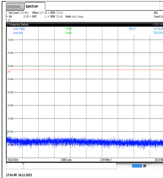
NTNV_N77-3450- 3550_PC2_30_15_H_TID6_NS_01_0.15_30_#1
