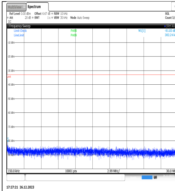
NTNV_N77-3450- 3550_PC2_30_15_H_TID2_NS_01_0.15_30_#1
