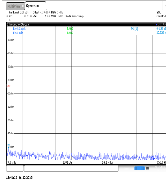
NTNV_N77-3450- 3550_PC2_30_15_M_TID6_NS_01_0.009_0.15_#1
