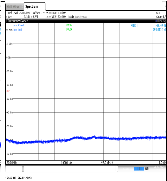
NTNV_N77-3450- 3550_PC2_30_15_H_TID6_NS_01_30_1000_#1
