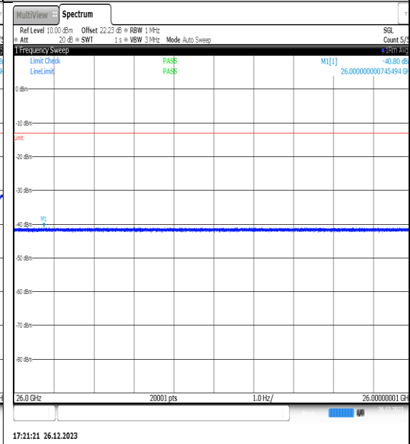
NTN_V_N77-3450- 3550_PC2_30_15_M_TID15_NS_01_26000_4000 0_#1
