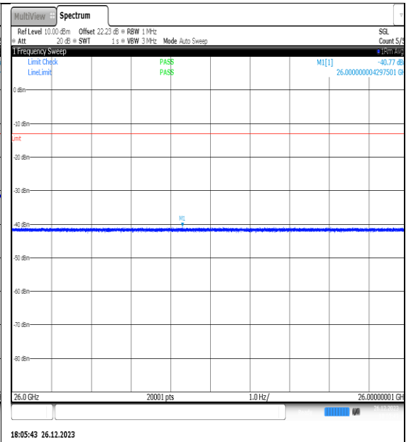
NTNV_N77-3450- 3550_PC2_30_15_H_TID10_NS_01_26000_4000 0_#1
