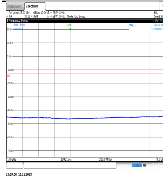
NTNV_N77-3450- 3550_PC2_30_10_H_TID15_NS_01_1000_3000_#1
