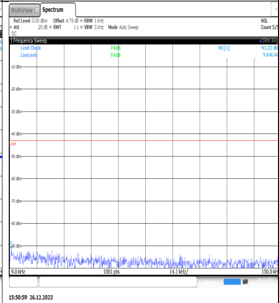
NTNV_N77-3450- 3550_PC2_30_15_L_TID8_NS_01_0.009_0.15_# 1
