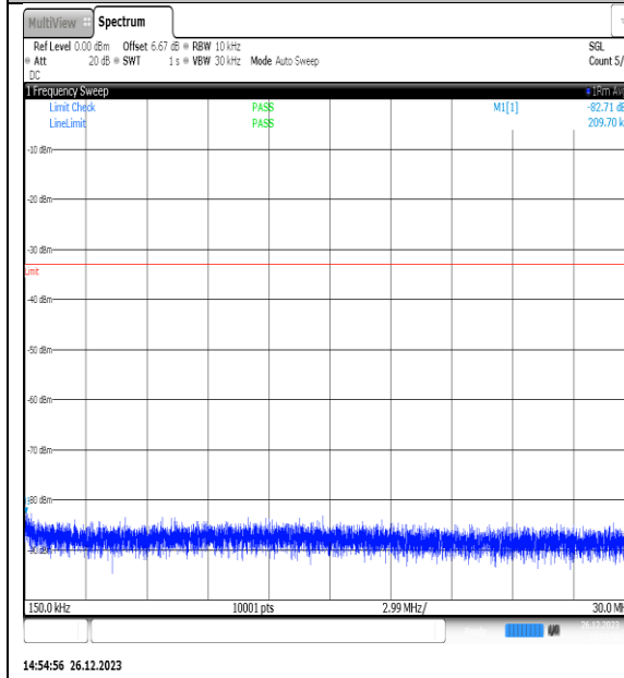
NTNV_N77-3450- 3550_PC2_30_10_H_TID9_NS_01_0.15_30_#1
