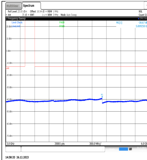
NTNV_N77-3450- 3550_PC2_30_10_H_TID10_NS_01_3000_6000_ #1
