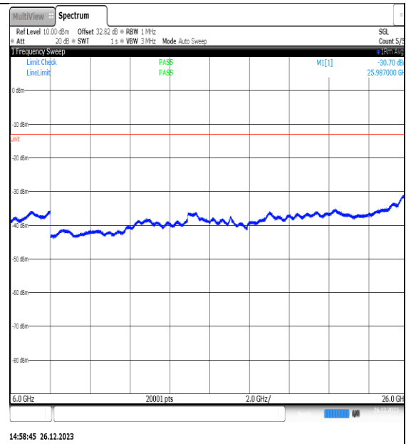
NTNV_N77-3450- 3550_PC2_30_10_H_TID10_NS_01_6000_26000 #1
