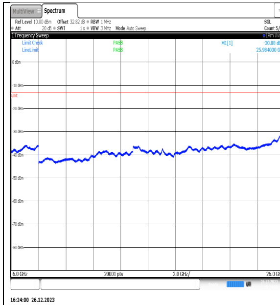
NTNV_N77-3450- 3550_PC2_30_15_M_TID1_NS_01_6000_26000_#1
