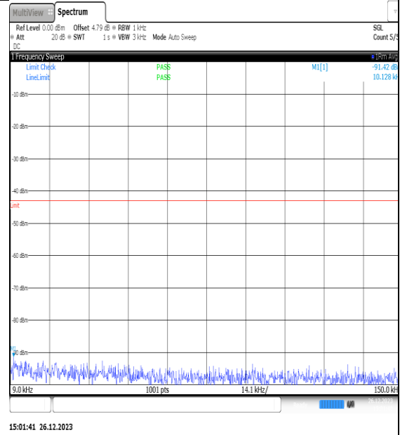
NTNV_N77-3450- 3550_PC2_30_10_H_TID11_NS_01_0.009_0.15_ #1
