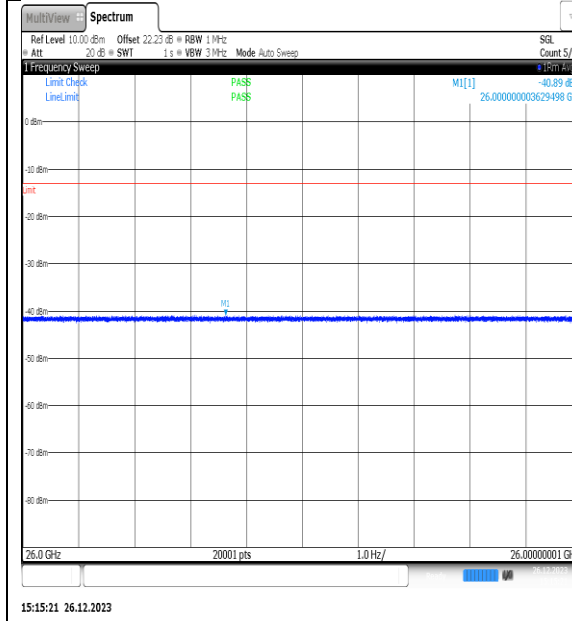
NTN_V_N77-3450- 3550_PC2_30_10_H_TID14_NS_01_26000_4000_ 0_#1
