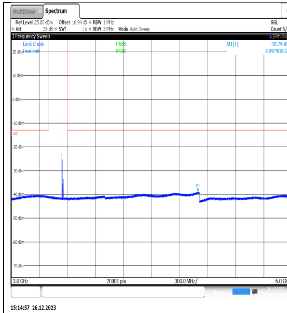
NTN_V_N77-3450- 3550_PC2_30_10_H_TID14_NS_01_3000_6000_ #1
