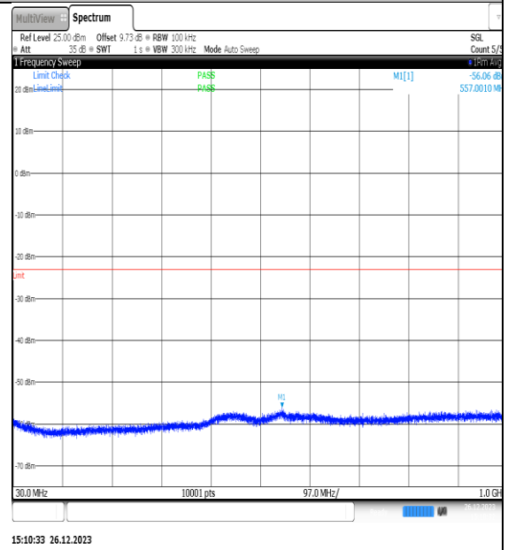
NTNV_N77-3450- 3550_PC2_30_10_H_TID13_NS_01_30_1000_#1
