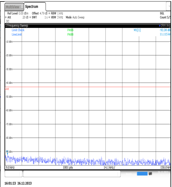
NTNV_N77-3450- 3550_PC2_30_15_L_TID10_NS_01_0.009_0.15_#1
