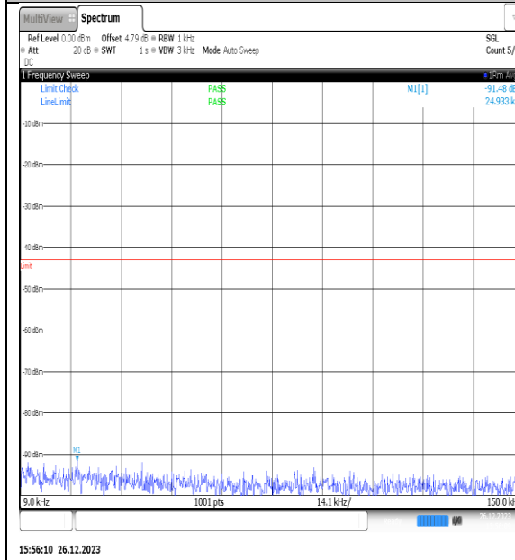
NTNV_N77-3450- 3550_PC2_30_15_L_TID9_NS_01_0.009_0.15_# 1
