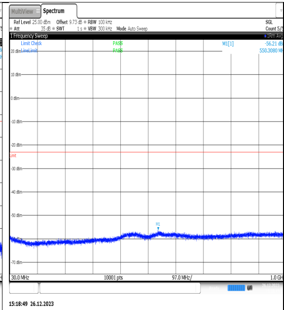
NTNV_N77-3450- 3550_PC2_30_10_H_TID15_NS_01_30_1000_#1
