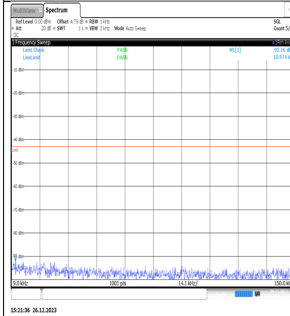
NTNV_N77-3450- 3550_PC2_30_15_L_TID1_NS_01_0.009_0.15_# 1
