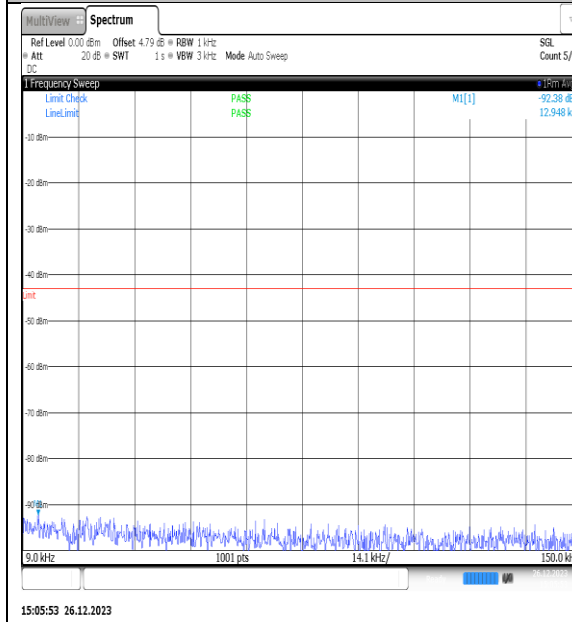
NTNV_N77-3450- 3550_PC2_30_10_H_TID12_NS_01_0.009_0.15_#1
