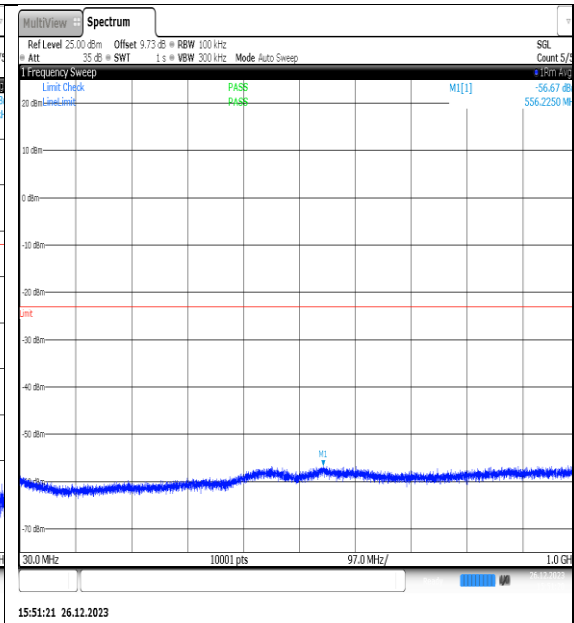
NTNV_N77-3450- 3550_PC2_30_15_L_TID8_NS_01_30_1000_#1
