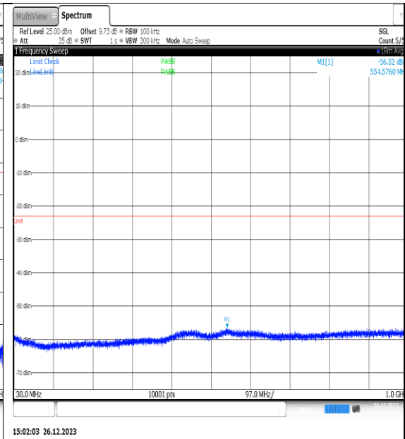
NTNV_N77-3450-3550_PC2_30_10_H_TID11_NS_01_30_1000_#1
