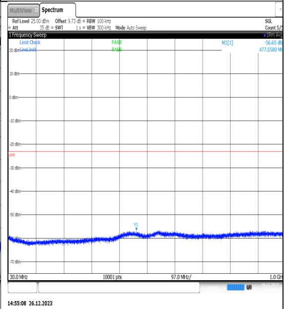
NTNV_N77-3450- 3550_PC2_30_10_H_TID9_NS_01_30_1000_#1
