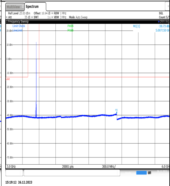
NTNV_N77-3450- 3550_PC2_30_10_H_TID15_NS_01_3000_6000_#1
