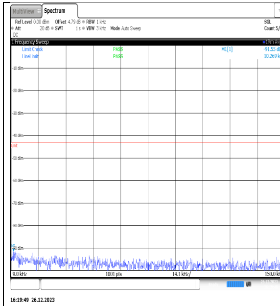
NTNV_N77-3450- 3550_PC2_30_15_L_TID15_NS_01_0.009_0.15_#1
