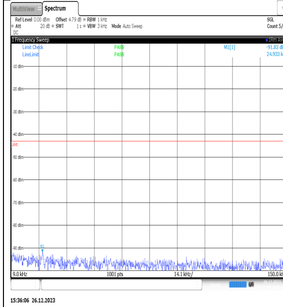
NTNV_N77-3450- 3550_PC2_30_15_L_TID5_NS_01_0.009_0.15_# 1
