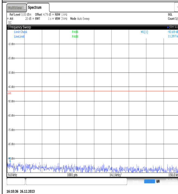
NTNV_N77-3450- 3550_PC2_30_15_L_TID13_NS_01_0.009_0.15_#1
