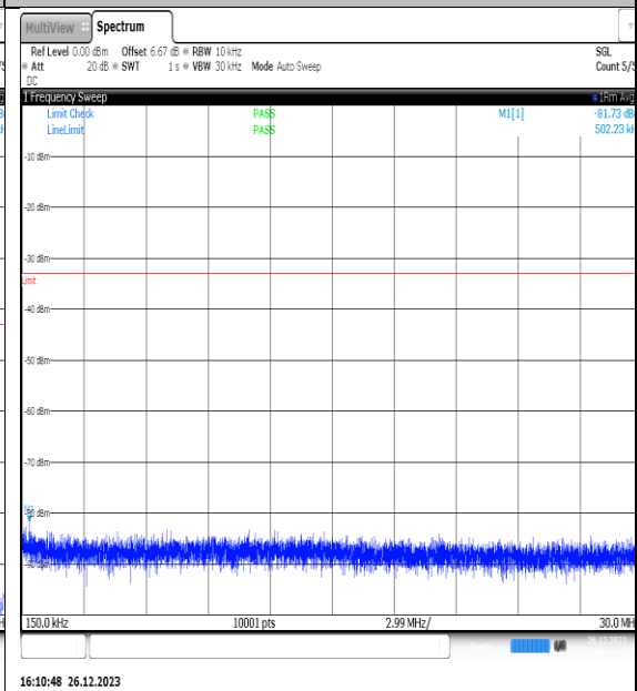
NTNV_N77-3450- 3550_PC2_30_15_L_TID13_NS_01_0.15_30_#1
