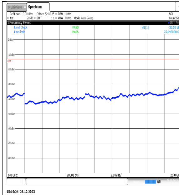
NTNV_N77-3450- 3550_PC2_30_10_H_TID15_NS_01_6000_26000 #1
