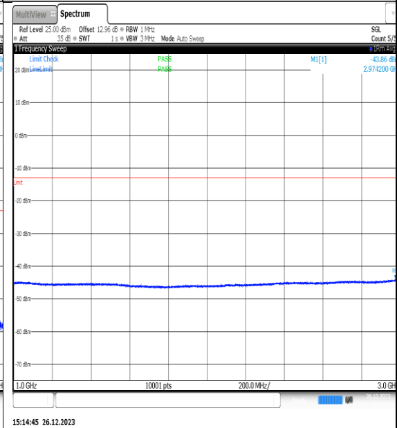
NTNV_N77-3450- 3550_PC2_30_10_H_TID14_NS_01_1000_3000_ #1
