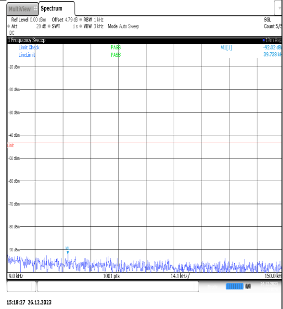
NTN_V_N77-3450- 3550_PC2_30_10_H_TID15_NS_01_0.009_0.15_ #1
