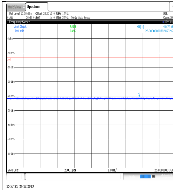
NTNV_N77-3450- 3550_PC2_30_15_L_TID9_NS_01_26000_40000 #1
