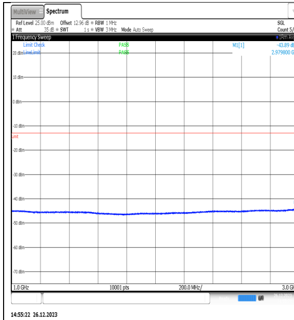
NTNV_N77-3450- 3550_PC2_30_10_H_TID9_NS_01_1000_3000_# 1
