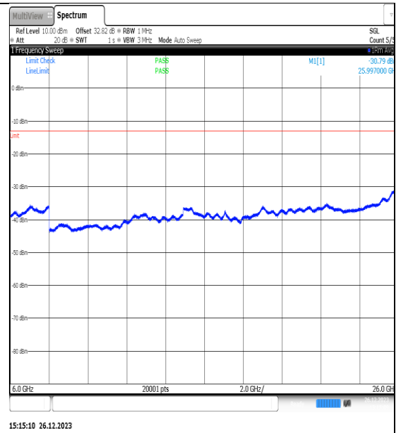
NTN_V_N77-3450- 3550_PC2_30_10_H_TID14_NS_01_6000_26000_ #1
