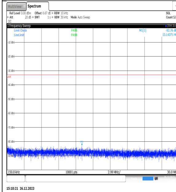
NTNV_N77-3450- 3550_PC2_30_10_H_TID13_NS_01_0.15_30_#1
