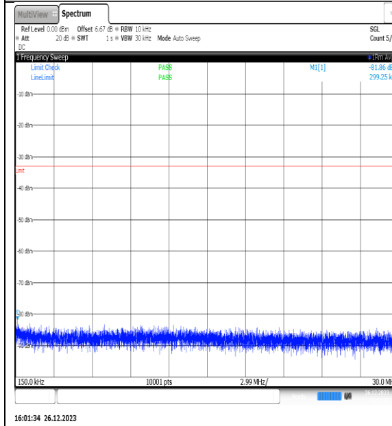
NTNV_N77-3450- 3550_PC2_30_15_L_TID10_NS_01_0.15_30_#1
