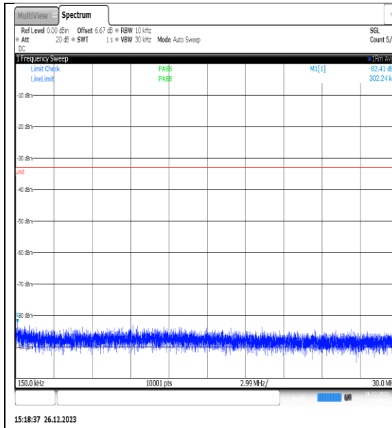
NTNV_N77-3450- 3550_PC2_30_10_H_TID15_NS_01_0.15_30_#1
