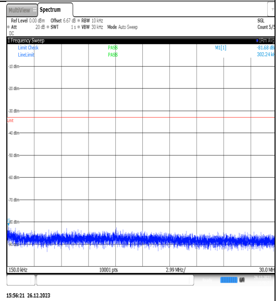
NTNV_N77-3450- 3550_PC2_30_15_L_TID9_NS_01_0.15_30_#1
