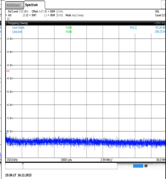
NTNV_N77-3450- 3550_PC2_30_15_L_TID5_NS_01_0.15_30_#1
