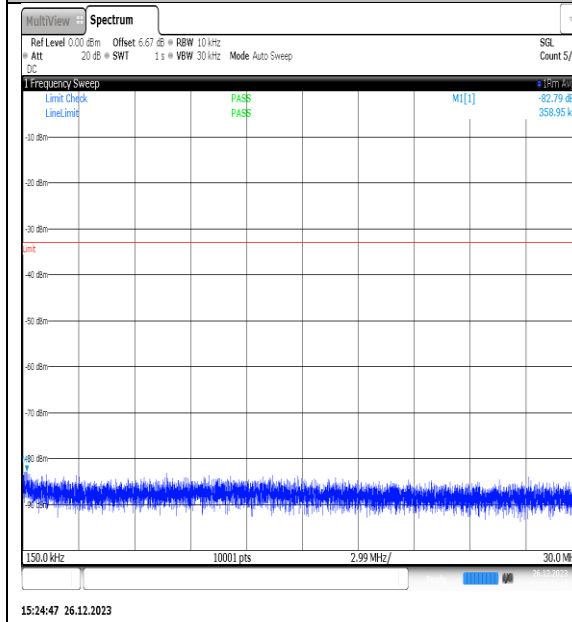
NTNV_N77-3450- 3550_PC2_30_15_L_TID2_NS_01_0.15_30_#1
