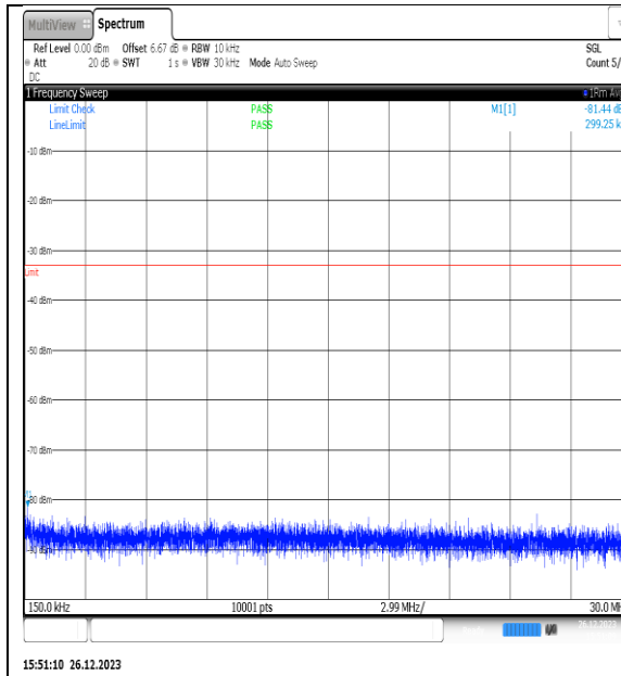
NTNV_N77-3450- 3550_PC2_30_15_L_TID8_NS_01_0.15_30_#1
