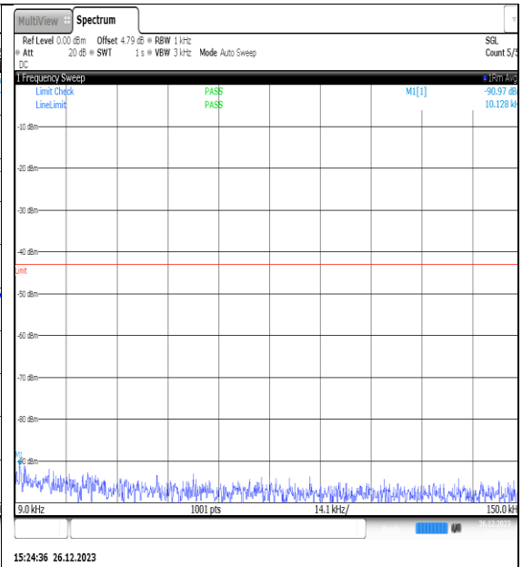
NTNV_N77-3450- 3550_PC2_30_15_L_TID2_NS_01_0.009_0.15_# 1
