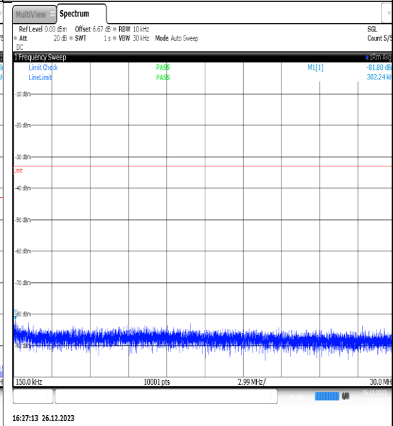
NTNV_N77-3450- 3550_PC2_30_15_M_TID2_NS_01_0.15_30_#1
