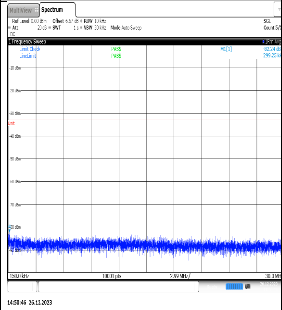
NTNV_N77-3450- 3550_PC2_30_10_H_TID8_NS_01_0.15_30_#1
