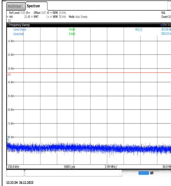
NTNV_N77-3450- 3550_PC2_30_10_M_TID8_NS_01_0.15_30_#1
