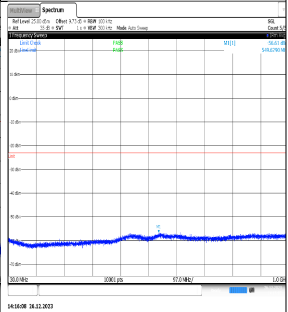
NTNV_N77-3450- 3550_PC2_30_10_H_TID5_NS_01_30_1000_#1
