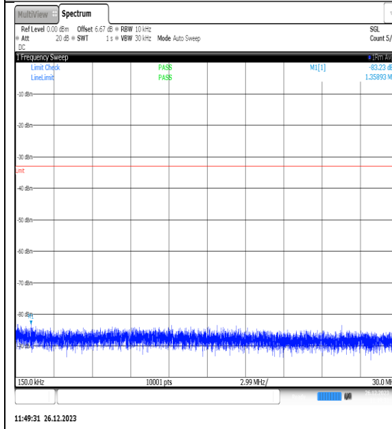
NTNV_N77-3450- 3550_PC2_30_10_L_TID15_NS_01_0.15_30_#1
