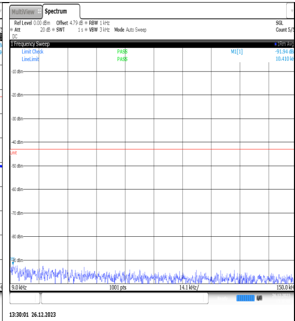
NTNV_N77-3450- 3550_PC2_30_10_H_TID1_NS_01_0.009_0.15_# 1
