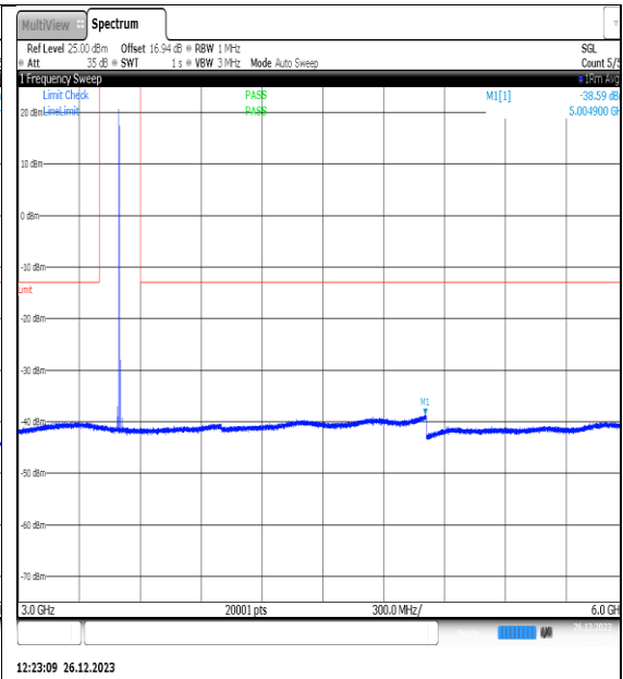
NTNV_N77-3450- 3550_PC2_30_10_M_TID8_NS_01_3000_6000_# 1
