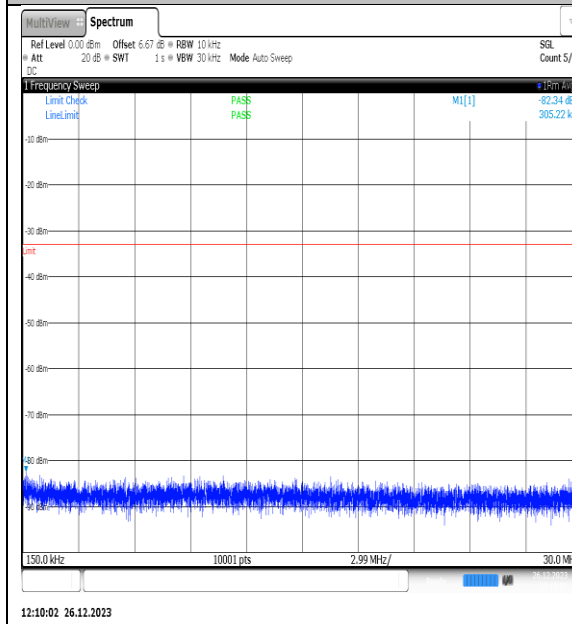
NTNV_N77-3450- 3550_PC2_30_10_M_TID4_NS_01_0.15_30_#1
