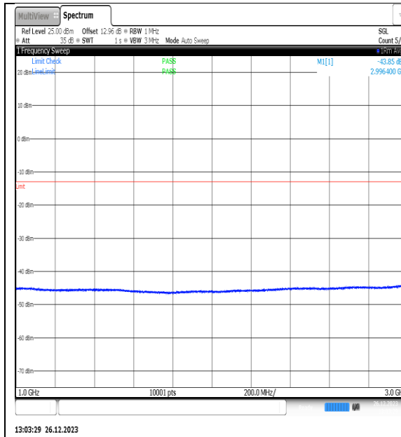
NTNV_N77-3450- 3550_PC2_30_10_M_TID12_NS_01_1000_3000_ #1
