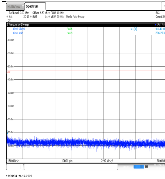
NTNV_N77-3450-3550_PC2_30_10_M_TID10_NS_01_0.15_30_#1
