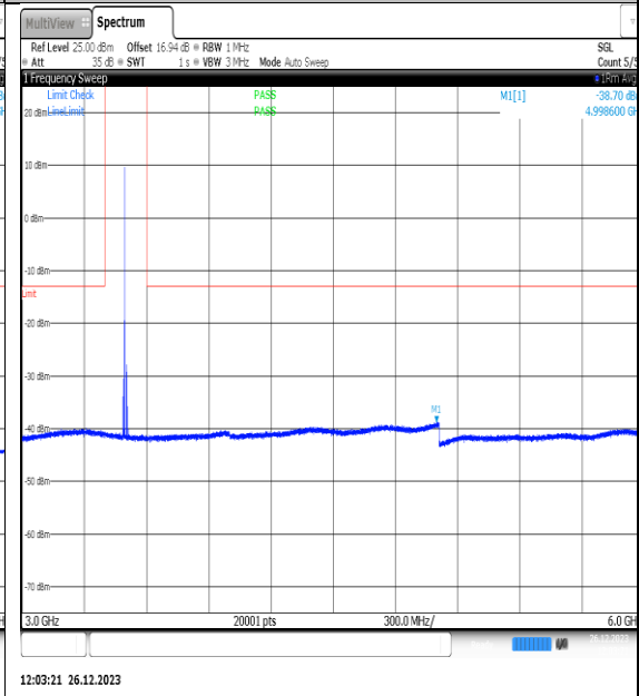
NTNV_N77-3450- 3550_PC2_30_10_M_TID2_NS_01_3000_6000_#1
