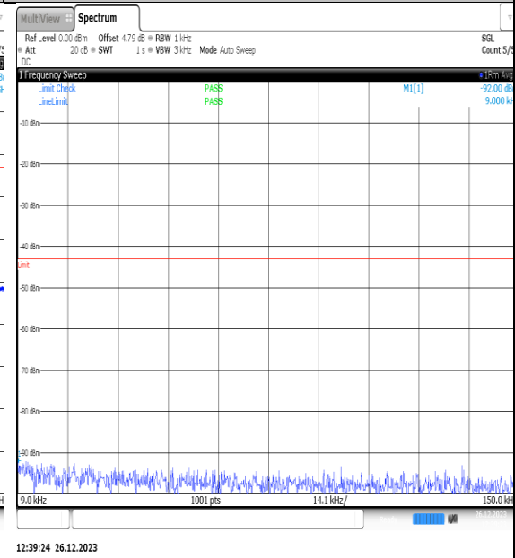
NTNV_N77-3450- 3550_PC2_30_10_M_TID10_NS_01_0.009_0.15_# 1
