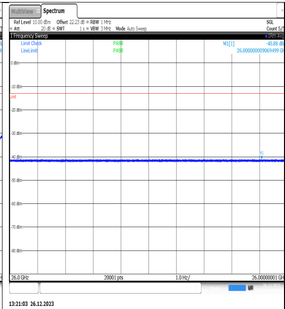
NTNV_N77-3450- 3550_PC2_30_10_M_TID14_NS_01_26000_4000 0_#1
