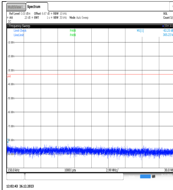
NTNV_N77-3450- 3550_PC2_30_10_M_TID2_NS_01_0.15_30_#1
