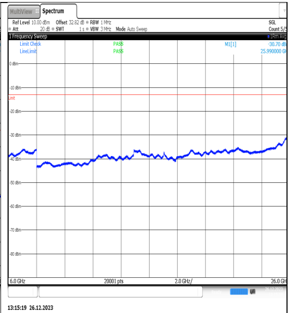
NTNV_N77-3450- 3550_PC2_30_10_M_TID13_NS_01_6000_26000 #1
