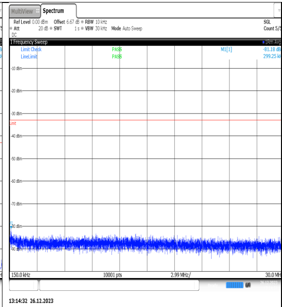
NTNV_N77-3450- 3550_PC2_30_10_M_TID13_NS_01_0.15_30_#1
