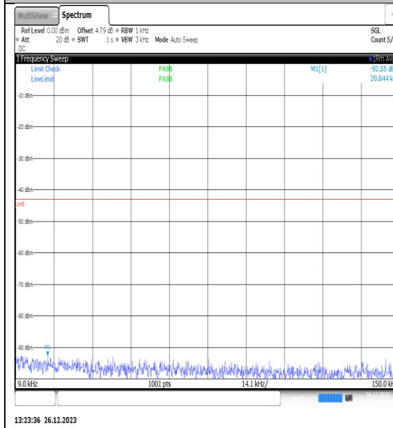
NTNV_N77-3450- 3550_PC2_30_10_M_TID15_NS_01_0.009_0.15_#1
