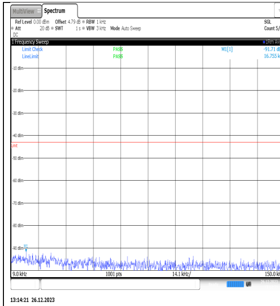
NTNV_N77-3450- 3550_PC2_30_10_M_TID13_NS_01_0.009_0.15_ #1
