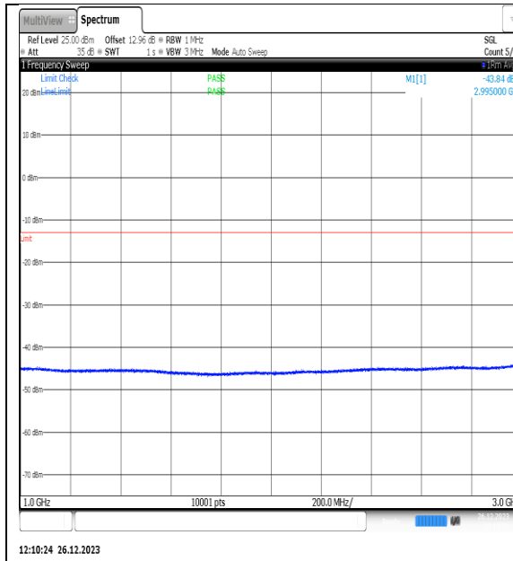
NTNV_N77-3450- 3550_PC2_30_10_M_TID4_NS_01_1000_3000_# 1
