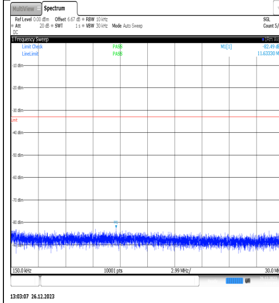
NTNV_N77-3450- 3550_PC2_30_10_M_TID12_NS_01_0.15_30_#1
