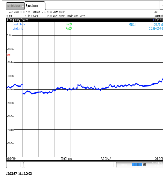
NTNV_N77-3450- 3550_PC2_30_10_M_TID12_NS_01_6000_26000_ #1
