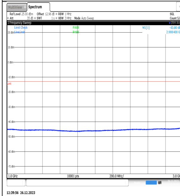
NTNV_N77-3450-3550_PC2_30_10_M_TID10_NS_01_1000_3000_#1
