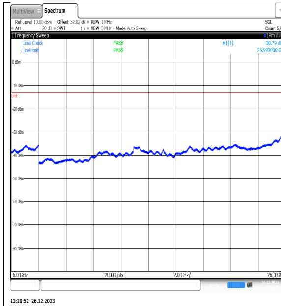
NTNV_N77-3450- 3550_PC2_30_10_M_TID14_NS_01_6000_26000 _#1
