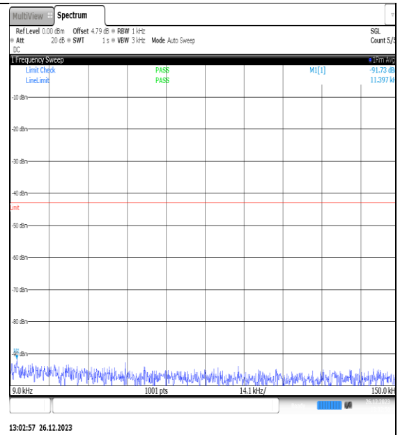
NTNV_N77-3450- 3550_PC2_30_10_M_TID12_NS_01_0.009_0.15_#1
