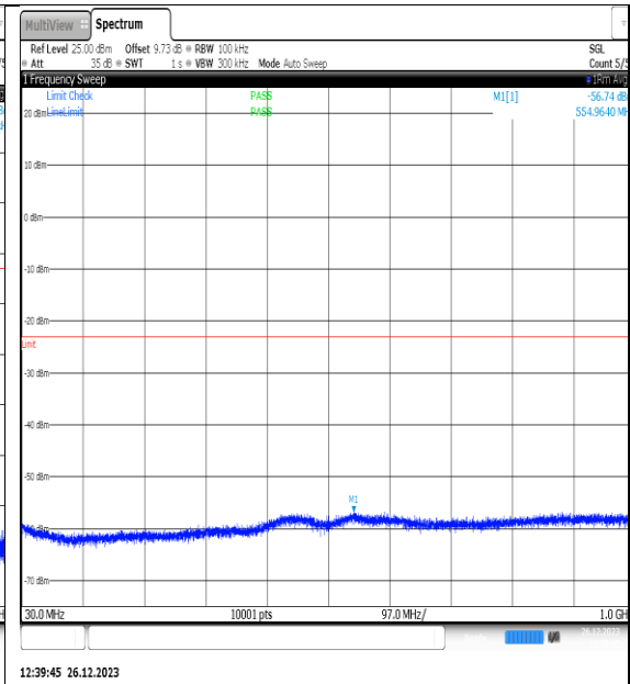
NTNV_N77-3450-3550_PC2_30_10_M_TID10_NS_01_30_1000_#1
