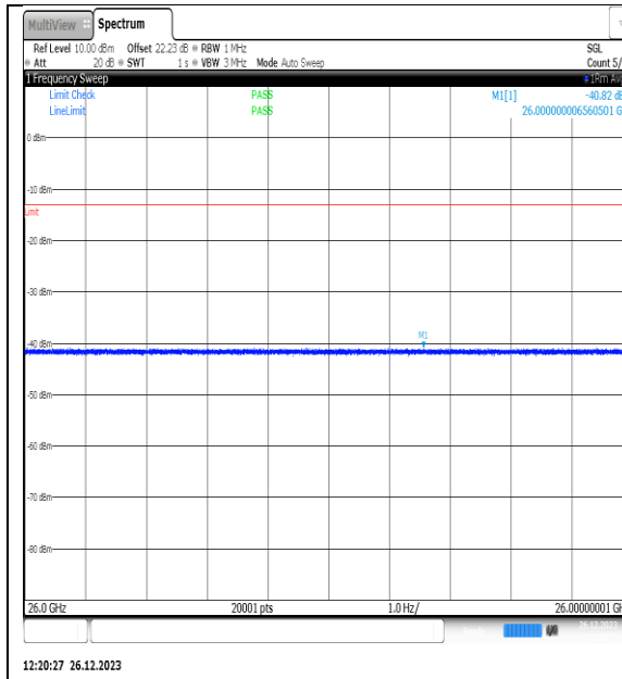
NTNV_N77-3450- 3550_PC2_30_10_M_TID7_NS_01_26000_40000 #1
