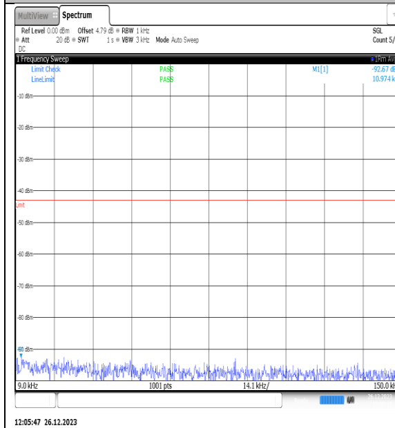
NTNV_N77-3450- 3550_PC2_30_10_M_TID3_NS_01_0.009_0.15_# 1
