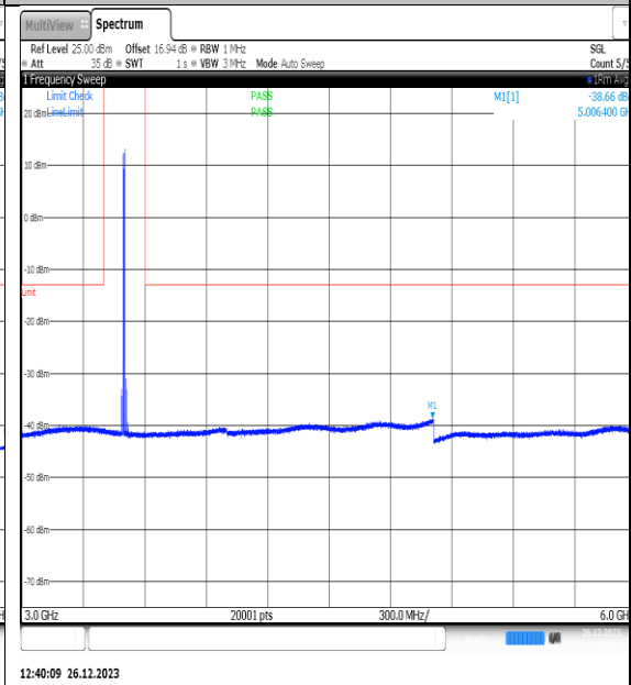
NTNV_N77-3450-3550_PC2_30_10_M_TID10_NS_01_3000_6000_#1
