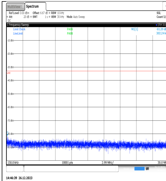
NTNV_N77-3450- 3550_PC2_30_10_H_TID7_NS_01_0.15_30_#1
