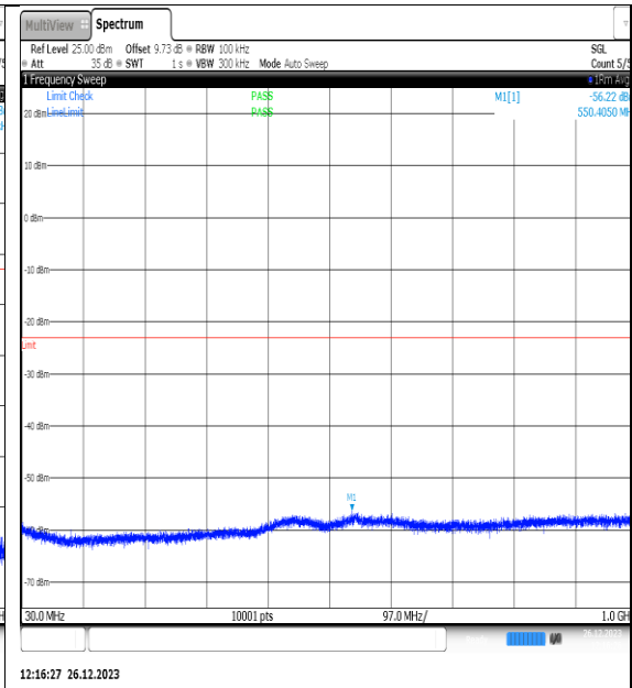
NTNV_N77-3450- 3550_PC2_30_10_M_TID6_NS_01_30_1000_#1
