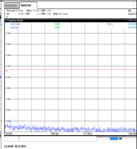
NTNV_N77-3450-3550_PC2_30_10_M_TID6_NS_01_0.009_0.15_#1
