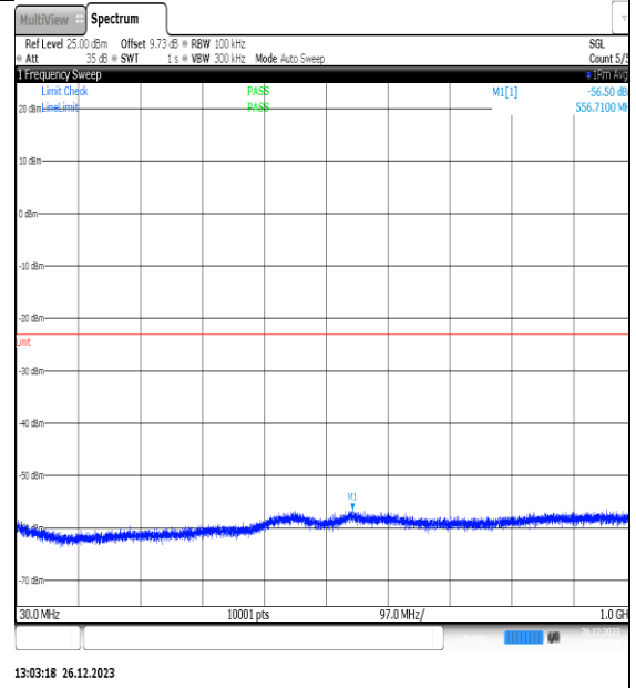
NTNV_N77-3450- 3550_PC2_30_10_M_TID12_NS_01_30_1000_#1
