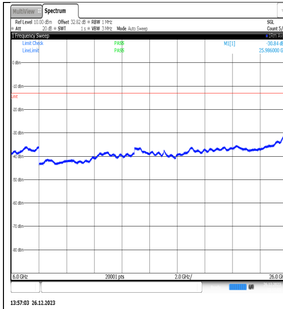
NTNV_N77-3450- 3550_PC2_30_10_H_TID3_NS_01_6000_26000_#1
