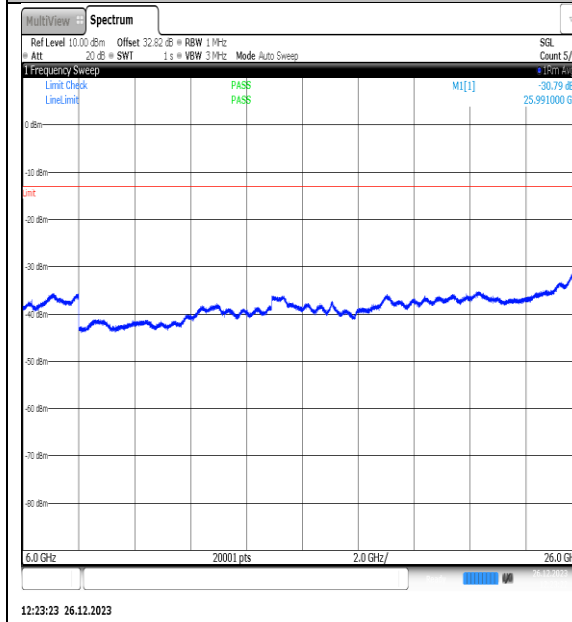
NTNV_N77-3450- 3550_PC2_30_10_M_TID8_NS_01_6000_26000_# #1
