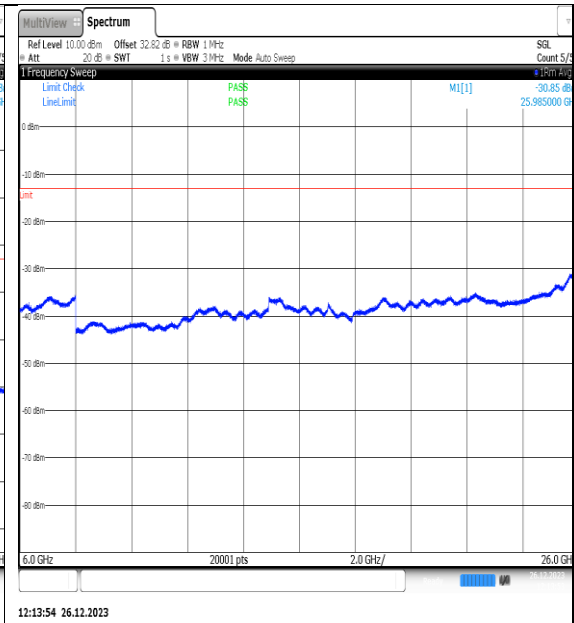
NTNV_N77-3450-3550_PC2_30_10_M_TID5_NS_01_6000_26000_#1
