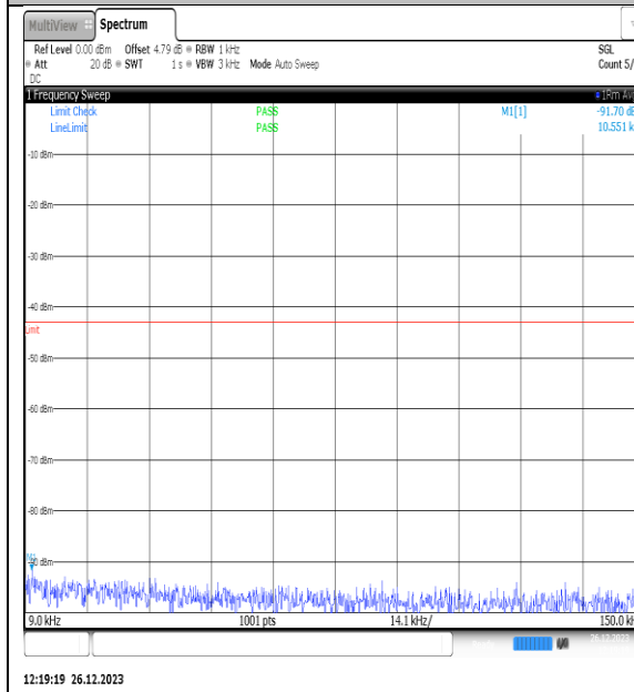
NTNV_N77-3450- 3550_PC2_30_10_M_TID7_NS_01_0.009_0.15_#1
