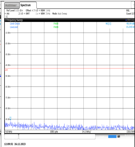
NTNV_N77-3450- 3550_PC2_30_10_M_TID4_NS_01_0.009_0.15_# 1
