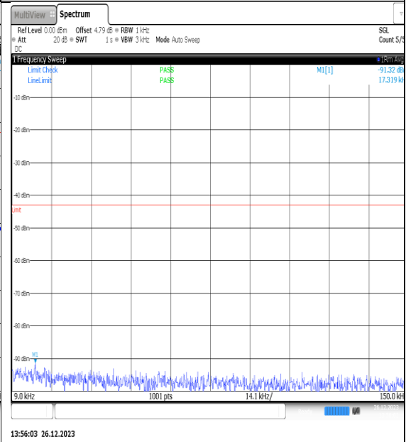
NTNV_N77-3450- 3550_PC2_30_10_H_TID3_NS_01_0.009_0.15_# 1
