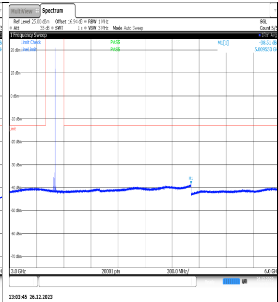
NTNV_N77-3450- 3550_PC2_30_10_M_TID12_NS_01_3000_6000_ #1
