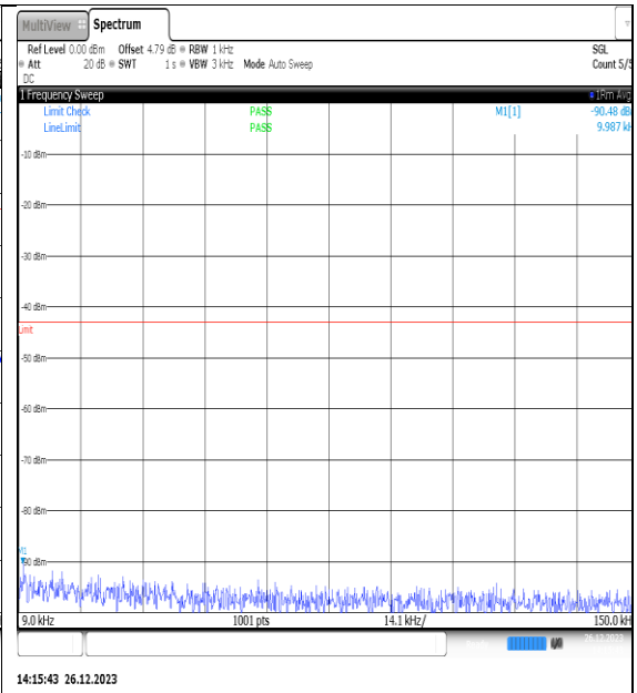
NTNV_N77-3450- 3550_PC2_30_10_H_TID5_NS_01_0.009_0.15_# 1
