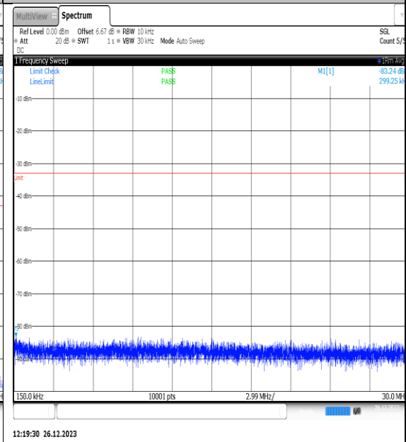
NTNV_N77-3450- 3550_PC2_30_10_M_TID7_NS_01_0.15_30_#1
