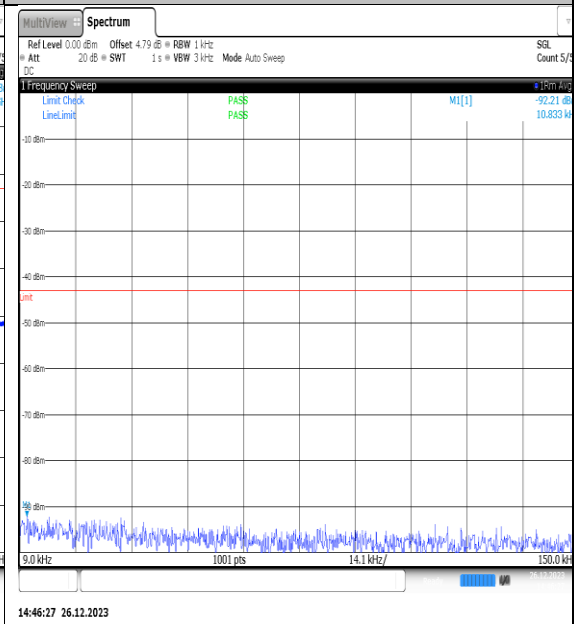
NTNV_N77-3450- 3550_PC2_30_10_H_TID7_NS_01_0.009_0.15_# 1
