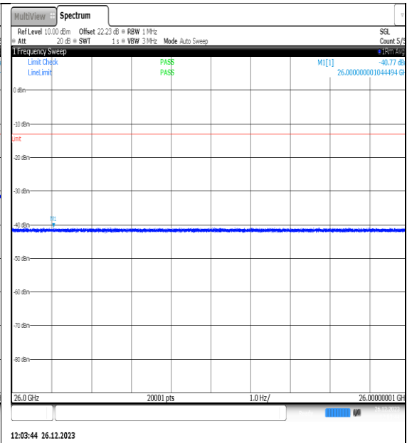
NTNV_N77-3450- 3550_PC2_30_10_M_TID2_NS_01_26000_40000 _#1
