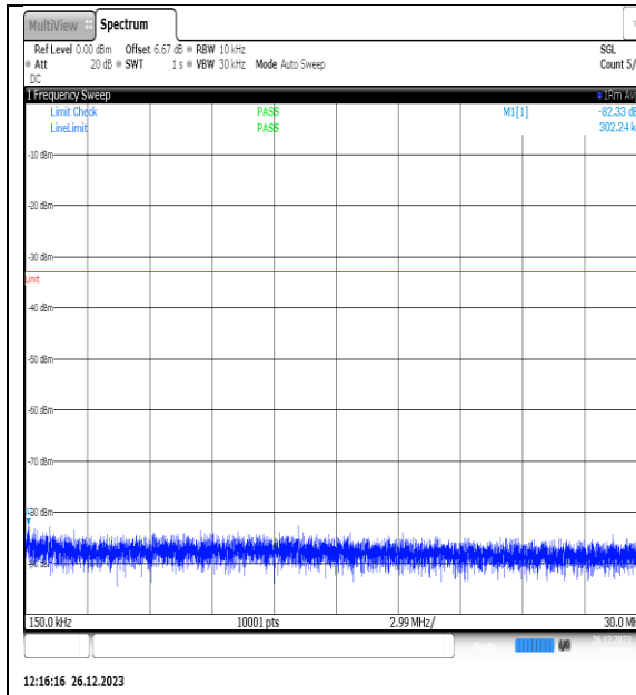
NTNV_N77-3450- 3550_PC2_30_10_M_TID6_NS_01_0.15_30_#1
