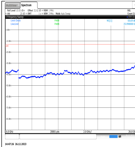
NTNV_N77-3450- 3550_PC2_30_10_H_TID7_NS_01_6000_26000_#1
