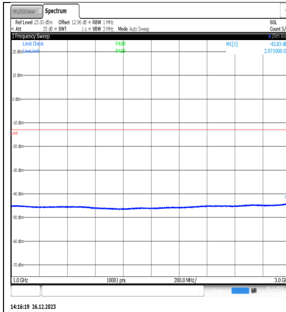
NTNV_N77-3450- 3550_PC2_30_10_H_TID5_NS_01_1000_3000_# 1
