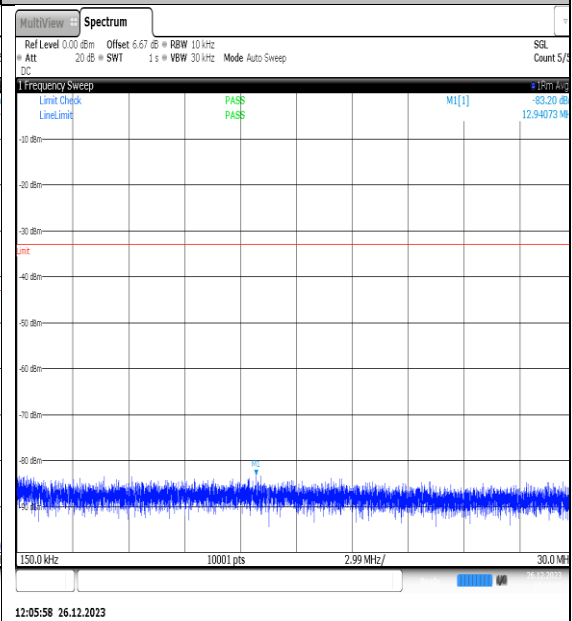
NTNV_N77-3450- 3550_PC2_30_10_M_TID3_NS_01_0.15_30_#1
