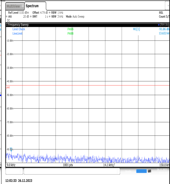
NTNV_N77-3450- 3550_PC2_30_10_M_TID2_NS_01_0.009_0.15_# 1
