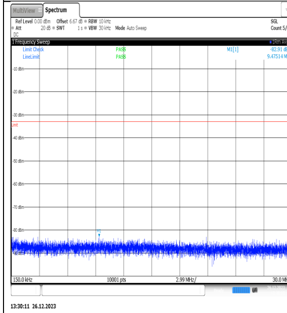
NTNV_N77-3450- 3550_PC2_30_10_H_TID1_NS_01_0.15_30_#1
