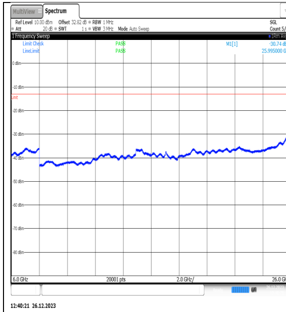
NTNV_N77-3450- 3550_PC2_30_10_M_TID10_NS_01_6000_26000 #1
