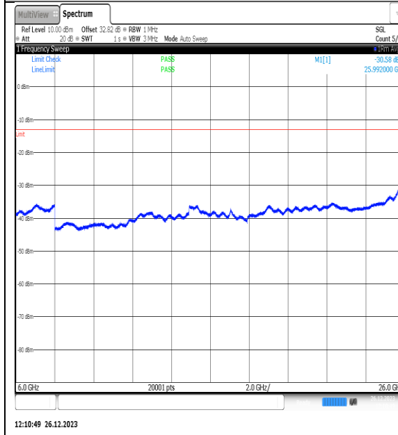
NTNV_N77-3450- 3550_PC2_30_10_M_TID4_NS_01_6000_26000_# 1
