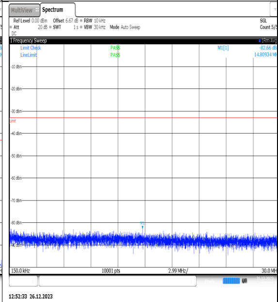
NTNV_N77-3450- 3550_PC2_30_10_M_TID11_NS_01_0.15_30_#1
