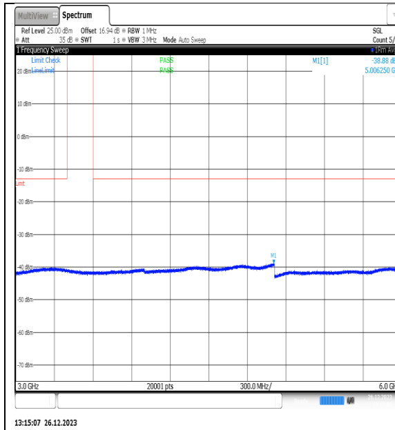
NTNV_N77-3450- 3550_PC2_30_10_M_TID13_NS_01_3000_6000_ #1
