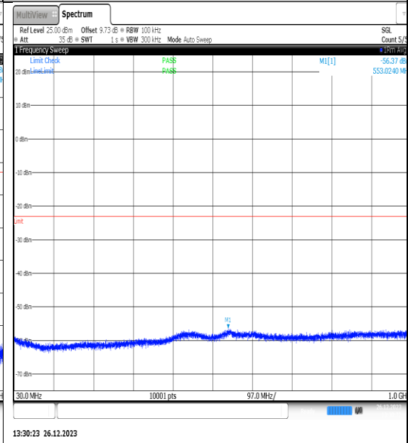
NTNV_N77-3450- 3550_PC2_30_10_H_TID1_NS_01_30_1000_#1
