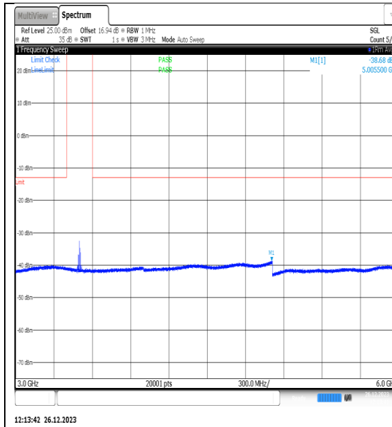
NTNV_N77-3450-3550_PC2_30_10_M_TID5_NS_01_3000_6000_#1
