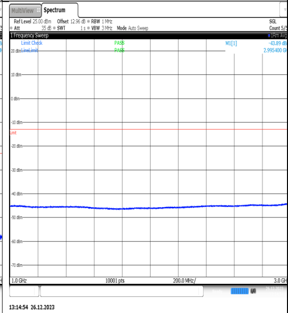
NTNV_N77-3450- 3550_PC2_30_10_M_TID13_NS_01_1000_3000_ #1
