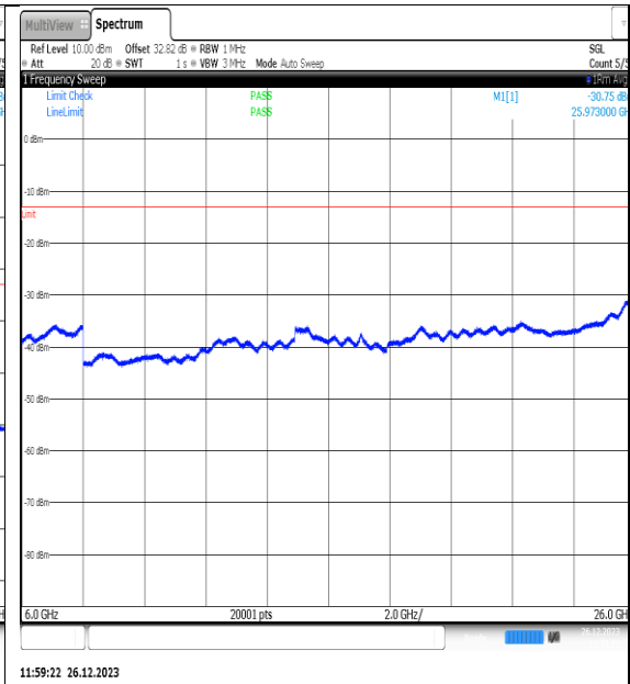
NTNV_N77-3450- 3550_PC2_30_10_M_TID1_NS_01_6000_26000_# #1
