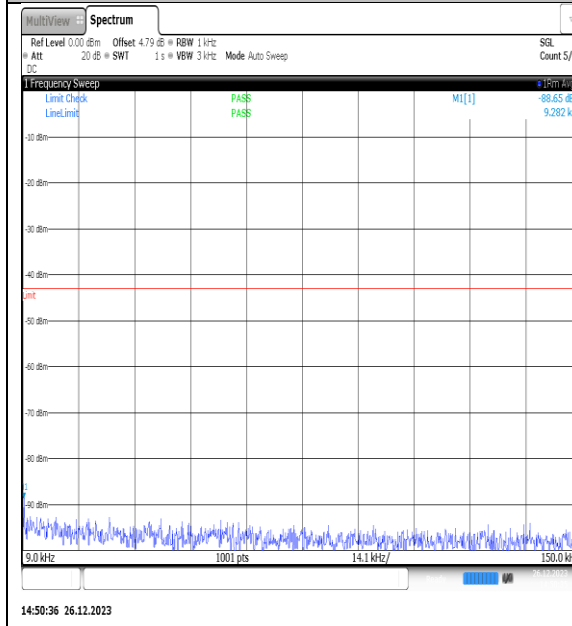
NTNV_N77-3450- 3550_PC2_30_10_H_TID8_NS_01_0.009_0.15_#1
