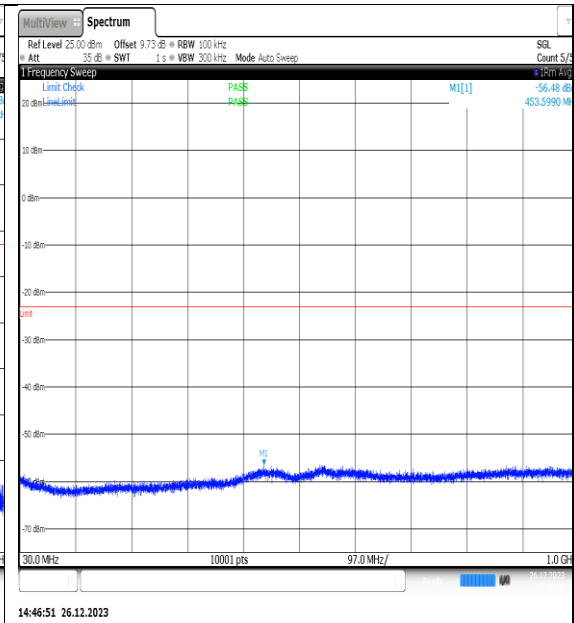
NTNV_N77-3450- 3550_PC2_30_10_H_TID7_NS_01_30_1000_#1
