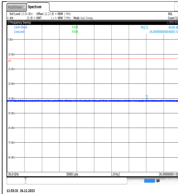
NTNV_N77-3450- 3550_PC2_30_10_M_TID11_NS_01_26000_4000 0_#1
