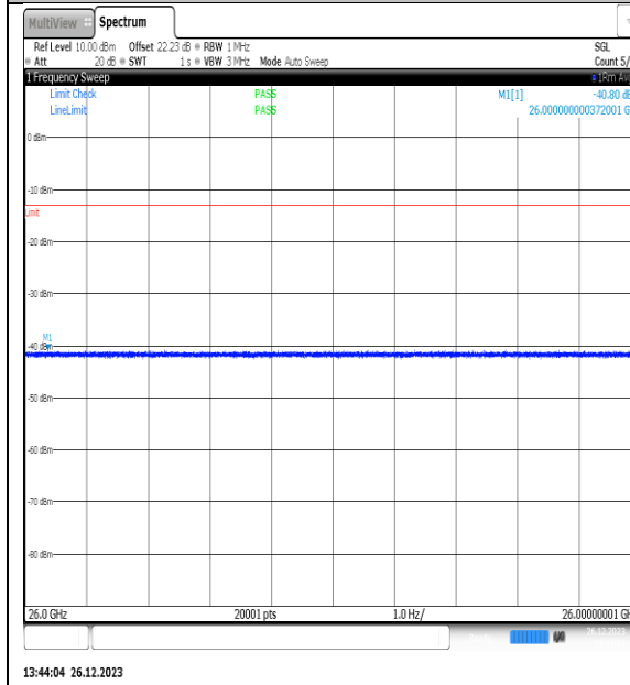
NTNV_N77-3450- 3550_PC2_30_10_H_TID2_NS_01_26000_40000_# 1
