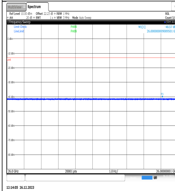
NTNV_N77-3450-3550_PC2_30_10_M_TID5_NS_01_26000_40000_#1
