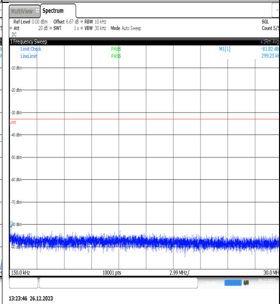
NTNV_N77-3450- 3550_PC2_30_10_M_TID15_NS_01_0.15_30_#1
