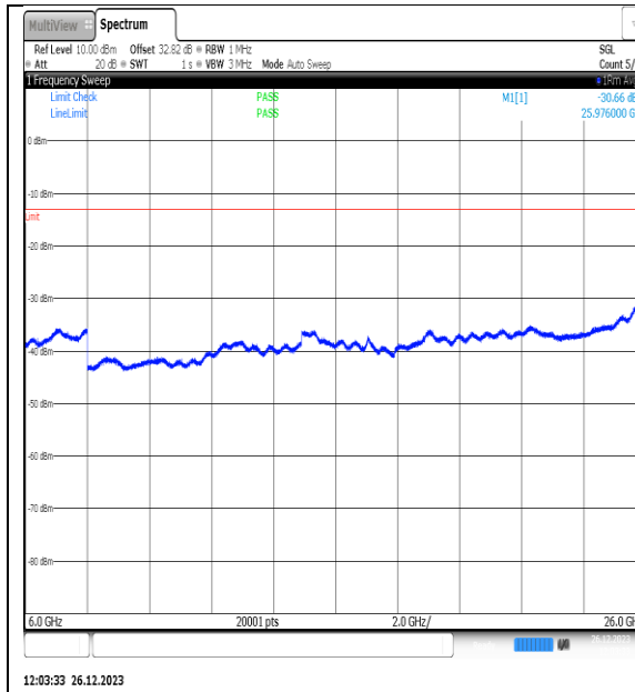
NTNV_N77-3450- 3550_PC2_30_10_M_TID2_NS_01_6000_26000_ #1
