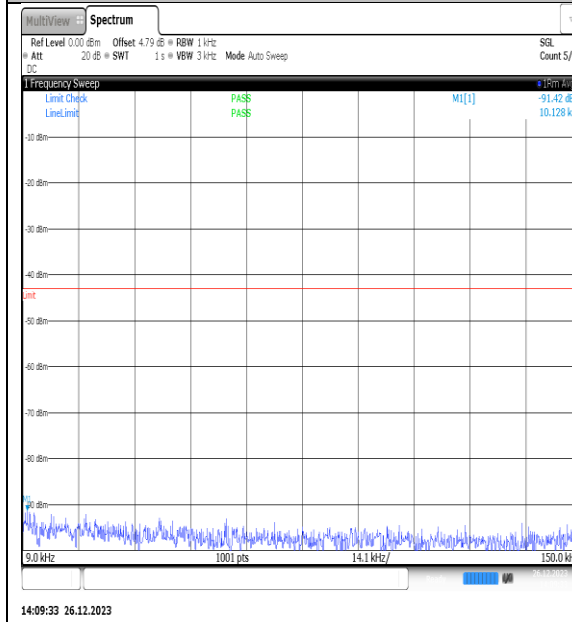
NTNV_N77-3450- 3550_PC2_30_10_H_TID4_NS_01_0.009_0.15_#1
