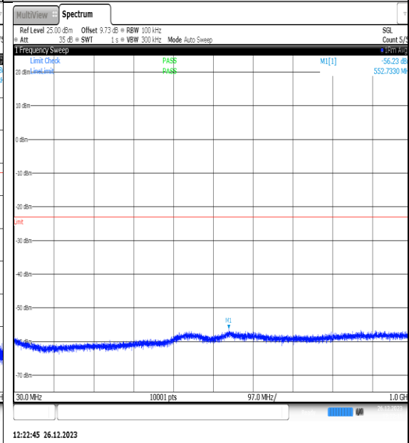
NTNV_N77-3450- 3550_PC2_30_10_M_TID8_NS_01_30_1000_#1
