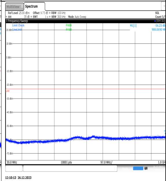
NTNV_N77-3450- 3550_PC2_30_10_M_TID4_NS_01_30_1000_#1
