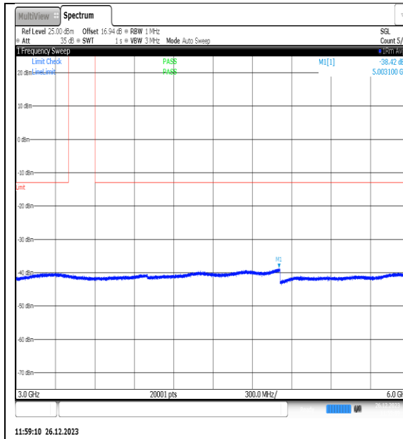
NTNV_N77-3450- 3550_PC2_30_10_M_TID1_NS_01_3000_6000_# 1
