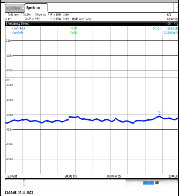
NTNV_N7_PC3_15_25_M_TID5_NS_01_12000_20000_#1
