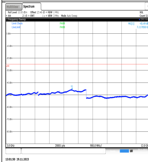
NTNV_N7_PC3_15_25_M_TID5_NS_01_3000_1 2000_#1
