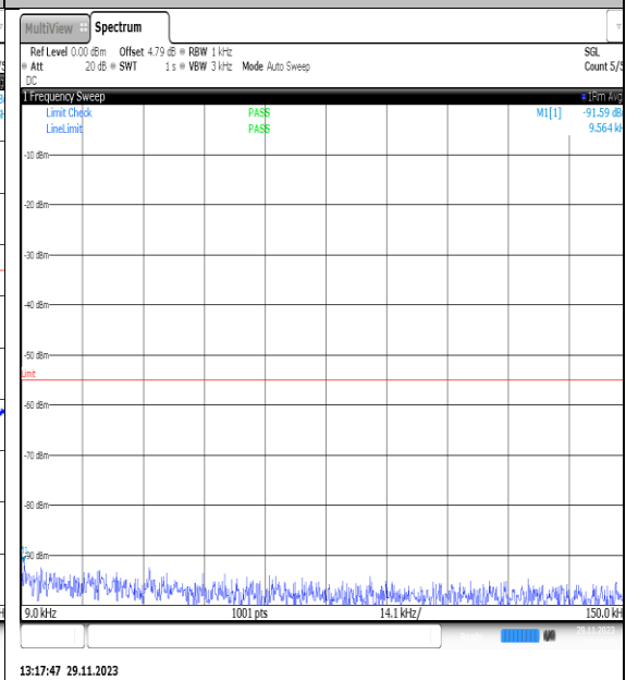
NTVN_N7_PC3_15_25_M_TID13_NS_01_0.009_0.15_#1
