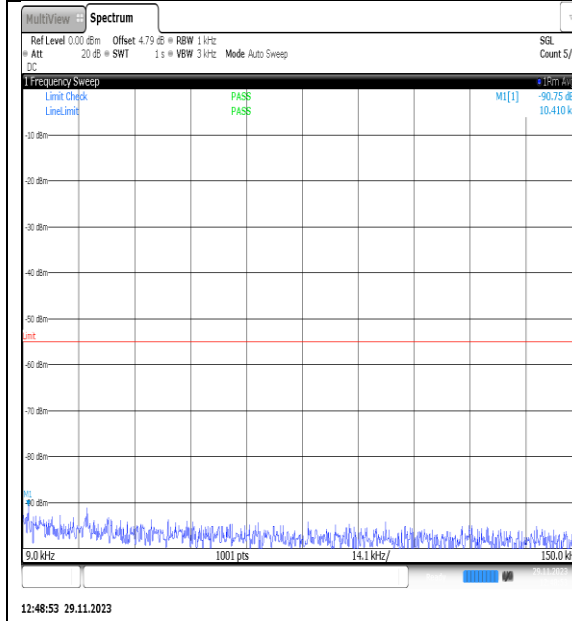
NTNV_N7_PC3_15_25_L_TID27_NS_01_0.009_0.15_#1
