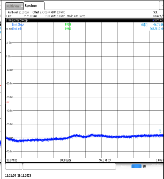
NTNV_N7_PC3_15_25_L_TID14_NS_01_30_100_0_#1
