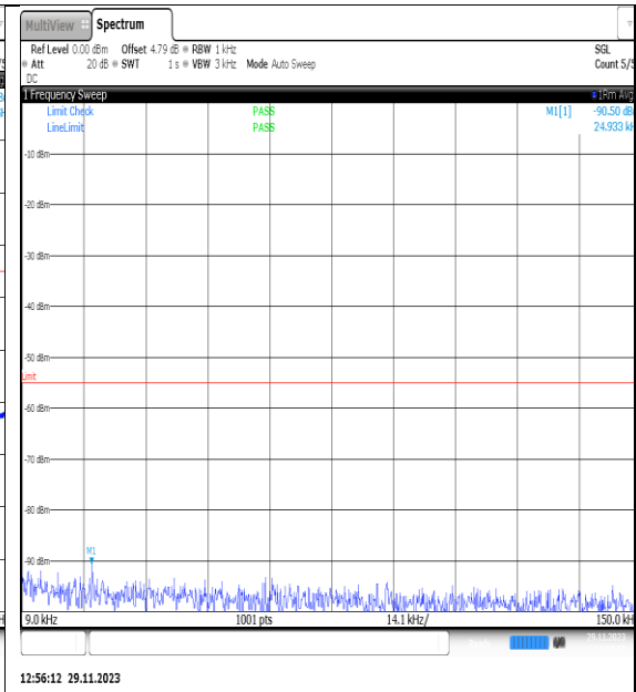
NTVN_N7_PC3_15_25_M_TID3_NS_01_0.009_0.15_#1
