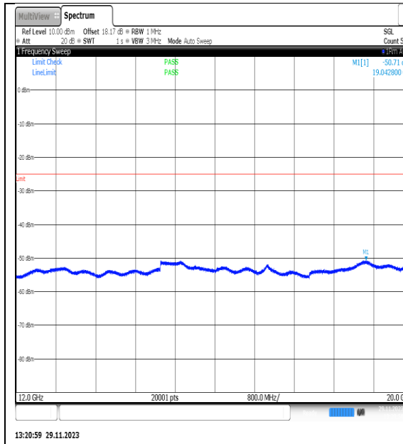
NTVN_N7_PC3_15_25_M_TID14_NS_01_12000_20000_#1
