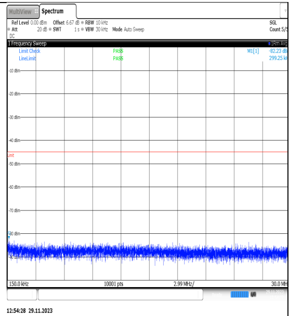
NTVN_N7_PC3_15_25_M_TID2_NS_01_0.15_30 _#1
