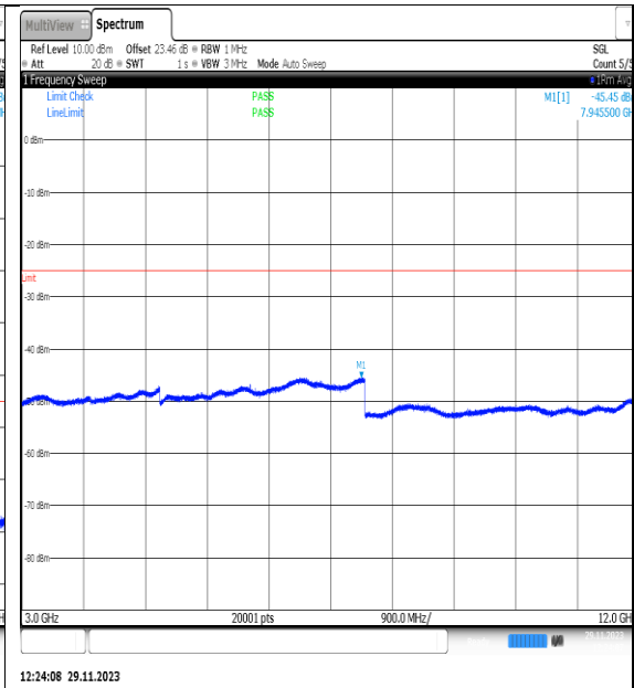
NTVN_N7_PC3_15_25_L_TID15_NS_01_3000_1_2000_#1
