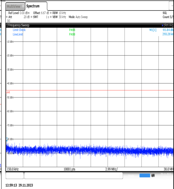
NTVN_N7_PC3_15_25_M_TID4_NS_01_0.15_30_#1
