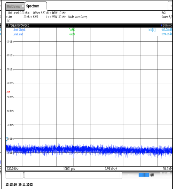
NTVN_N7_PC3_15_25_M_TID12_NS_01_0.15_30_#1
