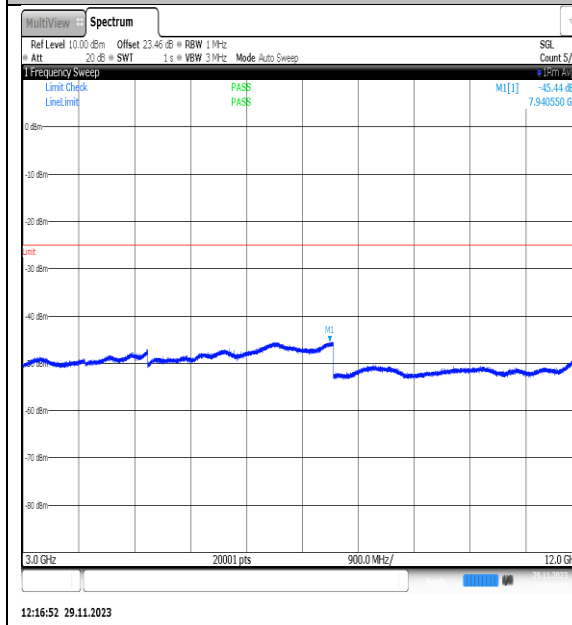
NTVN_N7_PC3_15_25_L_TID12_NS_01_3000_1_2000_#1
