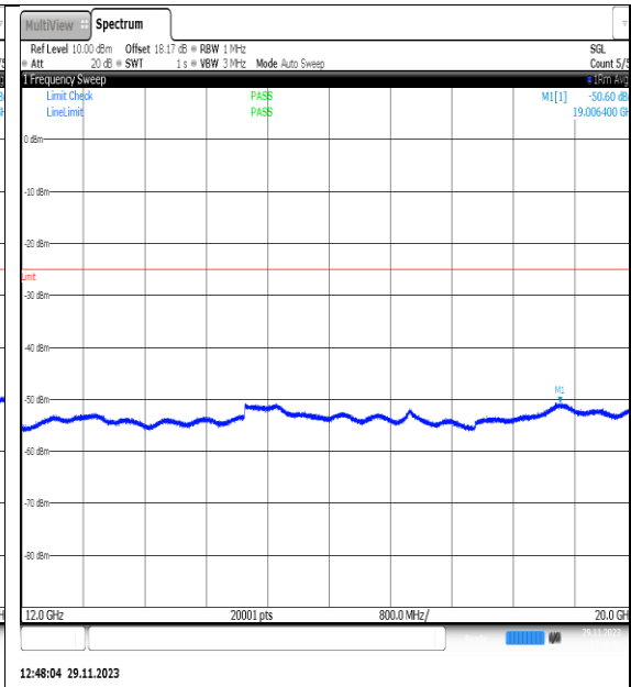
NTNV_N7_PC3_15_25_L_TID26_NS_01_12000_20000_#1
