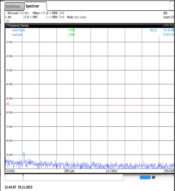
NTVN_N7_PC3_15_25_L_TID24_NS_01_0.009_0.15_#1
