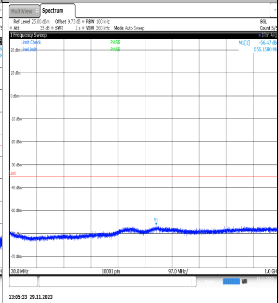
NTVN_N7_PC3_15_25_M_TID7_NS_01_30_100_0_#1
