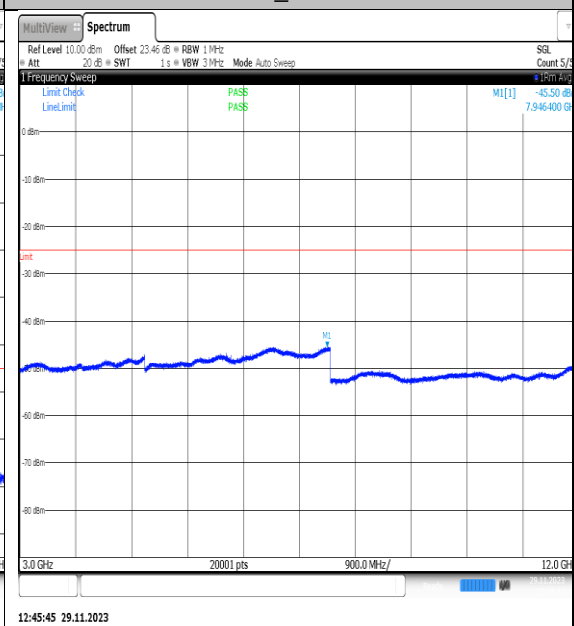
NTVN_N7_PC3_15_25_L_TID25_NS_01_3000_12000_#1
