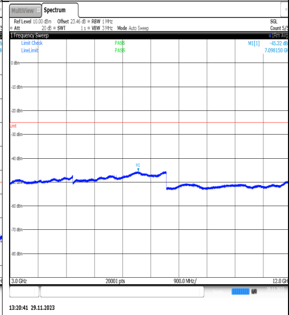
NTVN_N7_PC3_15_25_M_TID14_NS_01_3000_12000_#1
