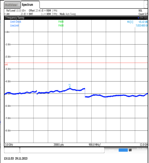
NTVN_N7_PC3_15_25_M_TID10_NS_01_3000_12000_#1
