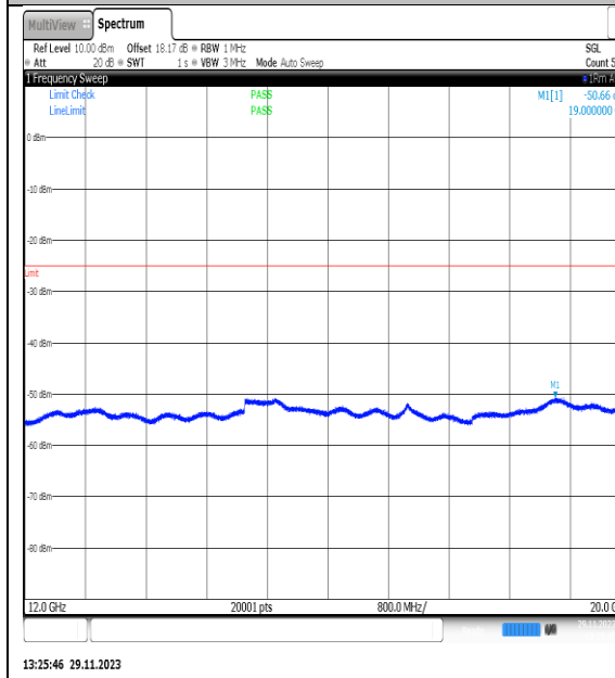
NTVN_N7_PC3_15_25_M_TID16_NS_01_12000_20000_#1
