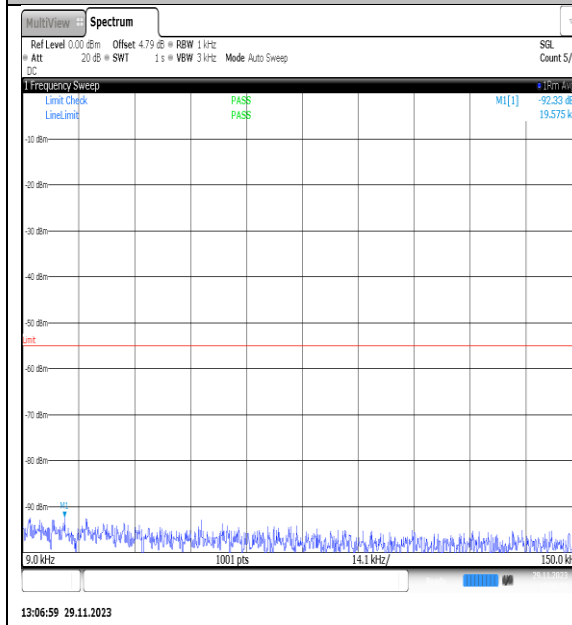
NTVN_N7_PC3_15_25_M_TID8_NS_01_0.009_0.15_#1
