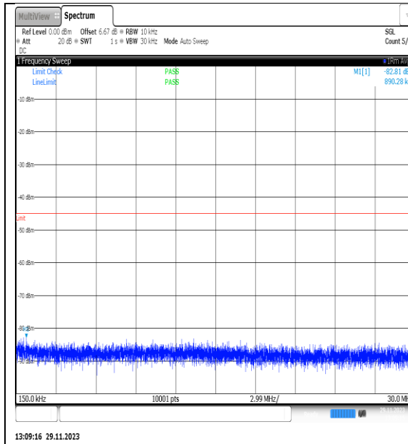
NTVN_N7_PC3_15_25_M_TID9_NS_01_0.15_30 #1
