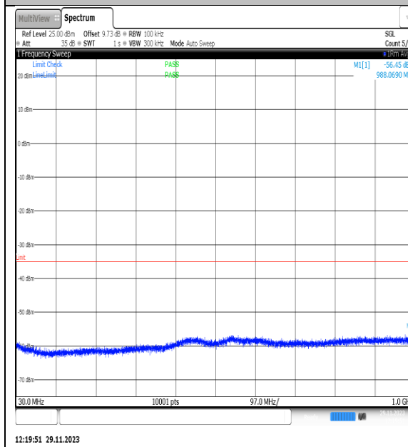
NTVN_N7_PC3_15_25_L_TID13_NS_01_30_100_0_#1
