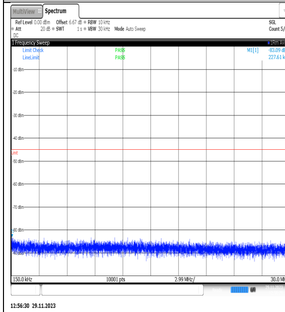
NTVN_N7_PC3_15_25_M_TID3_NS_01_0.15_30_#1
