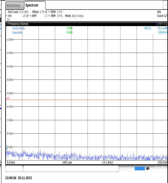
NTVN_N7_PC3_15_25_M_TID5_NS_01_0.009_0.15_#1
