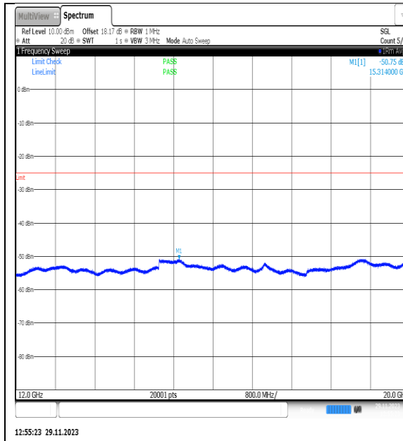
NTVN_N7_PC3_15_25_M_TID2_NS_01_12000_20000_#1
