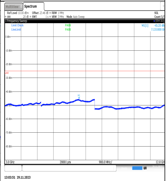
NTVN_N7_PC3_15_25_M_TID6_NS_01_3000_1_2000_#1
