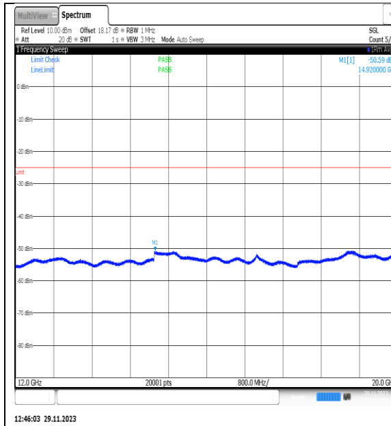
NTNV_N7_PC3_15_25_L_TID25_NS_01_12000_20000_#1
