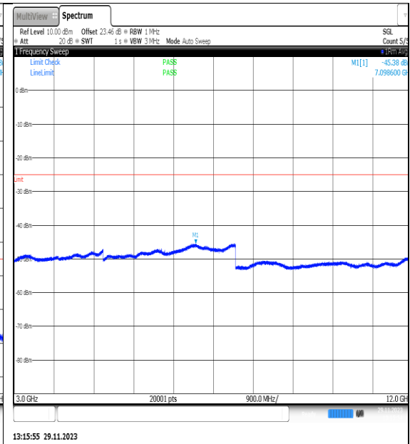
NTVN_N7_PC3_15_25_M_TID12_NS_01_3000_12000_#1
