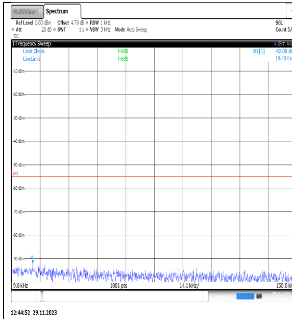
NTVN_N7_PC3_15_25_L_TID25_NS_01_0.009_0.15_#1
