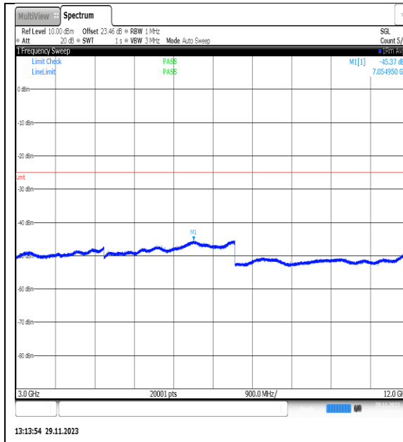
NTVN_N7_PC3_15_25_M_TID11_NS_01_3000_12000_#1
