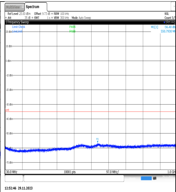
NTNV_N7_PC3_15_25_M_TID1_NS_01_30_100 0_#1
