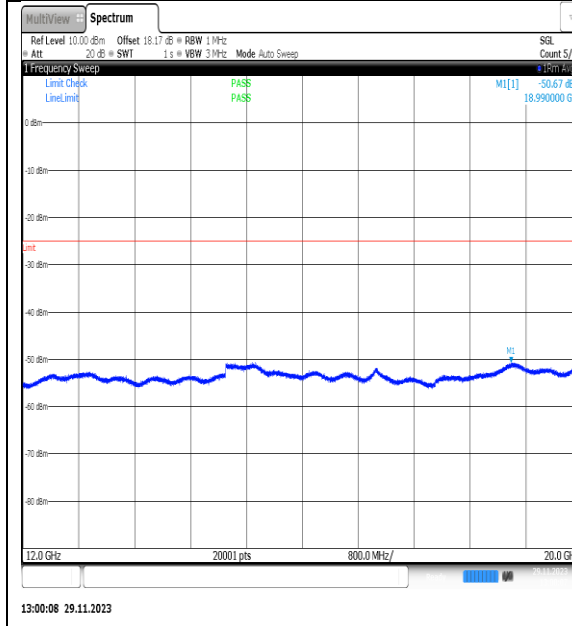
NTVN_N7_PC3_15_25_M_TID4_NS_01_12000_20000_#1
