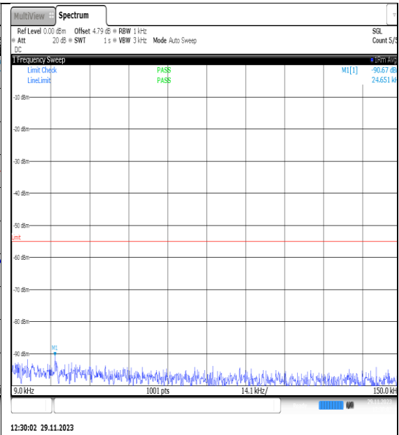
NTNV_N7_PC3_15_25_L_TID18_NS_01_0.009_0.15_#1
