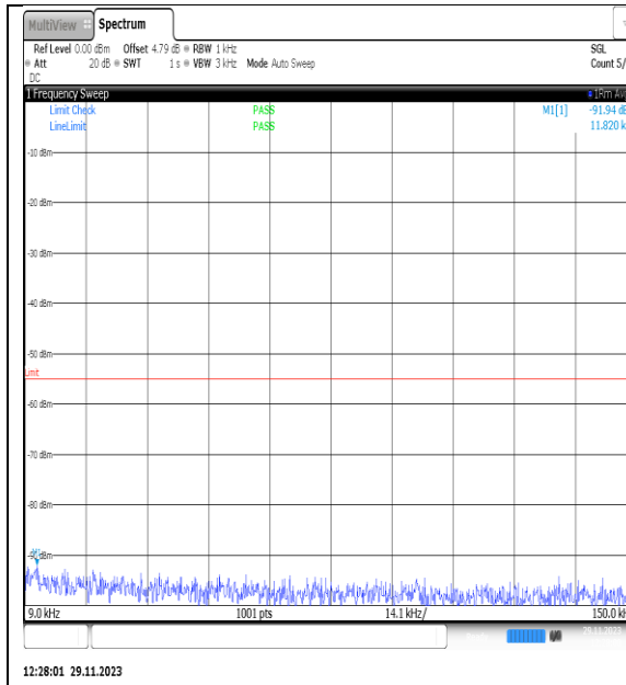
NTVN_N7_PC3_15_25_L_TID17_NS_01_0.009_0.15_#1
