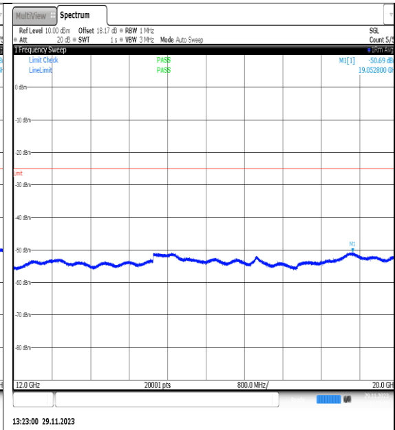
NTVN_N7_PC3_15_25_M_TID15_NS_01_12000_20000_#1
