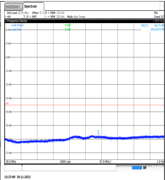
NTNV_N7_PC3_15_25_M_TID17_NS_01_30_10_00_#1
