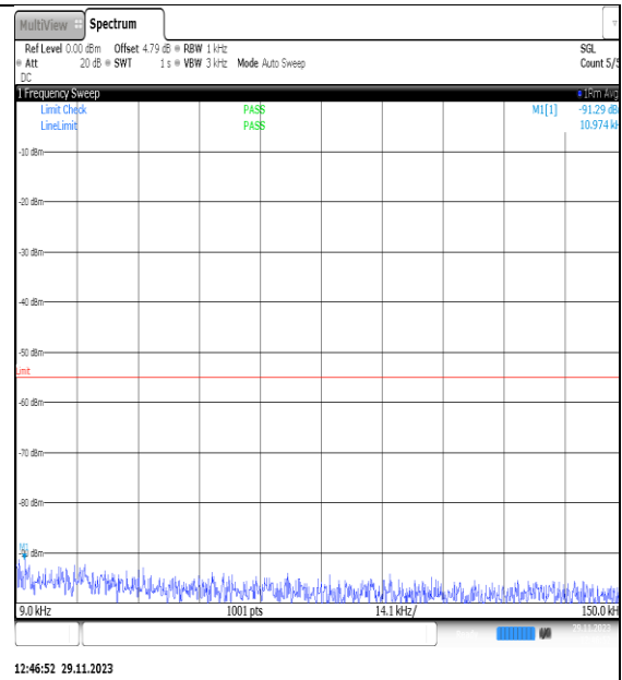
NTNV_N7_PC3_15_25_L_TID26_NS_01_0.009_0.15_#1
