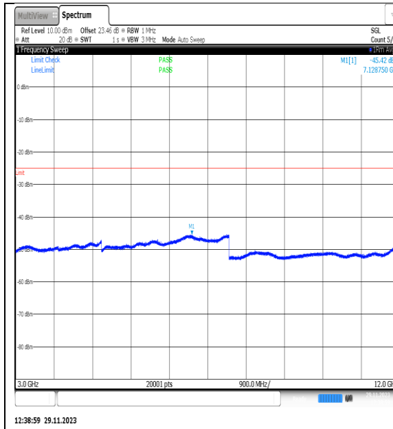
NTVN_N7_PC3_15_25_L_TID22_NS_01_3000_1 2000_#1
