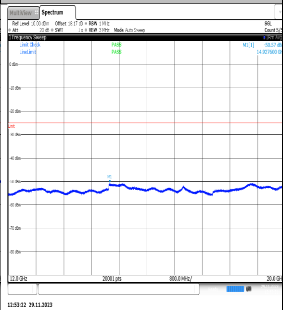
NTNV_N7_PC3_15_25_M_TID1_NS_01_12000_20000_#1
