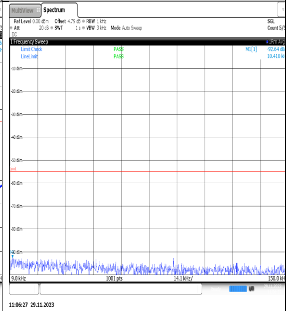
NTVN_N7_PC3_15_20_H_TID7_NS_01_0.009_0. 15_#1
