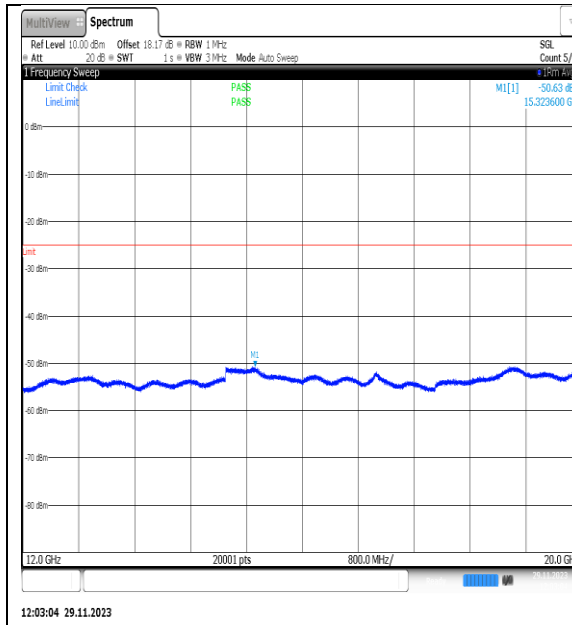
NTNV_N7_PC3_15_25_L_TID5_NS_01_12000_2_0000_#1
