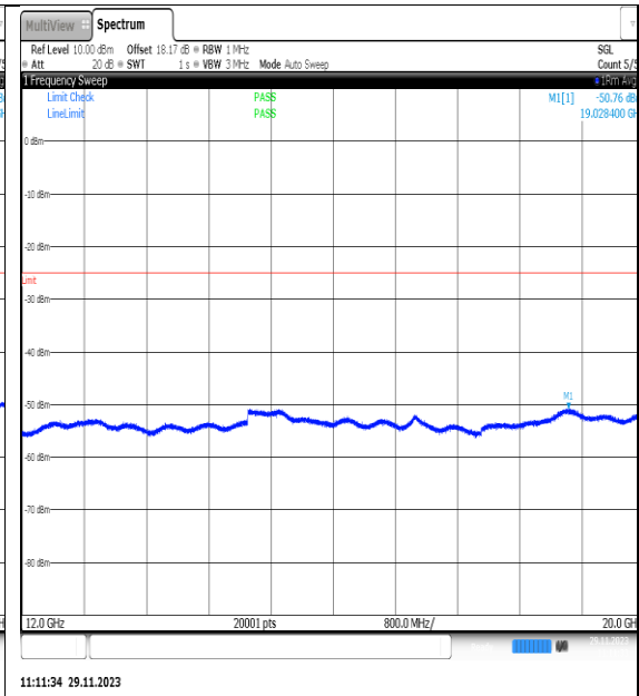
NTVN_N7_PC3_15_20_H_TID9_NS_01_12000_2_0000_#1
