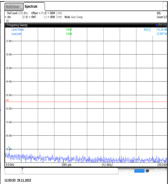
NTNV_N7_PC3_15_25_L_TID6_NS_01_0.009_0_15_#1
