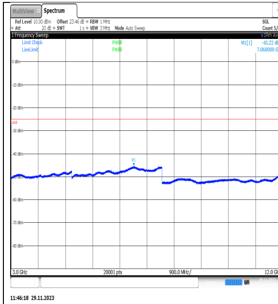
NTVN_N7_PC3_15_20_H_TID25_NS_01_3000_1_2000_#1
