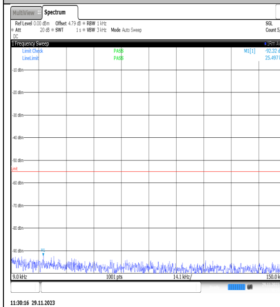
NTVN_N7_PC3_15_20_H_TID18_NS_01_0.009_0.15_#1
