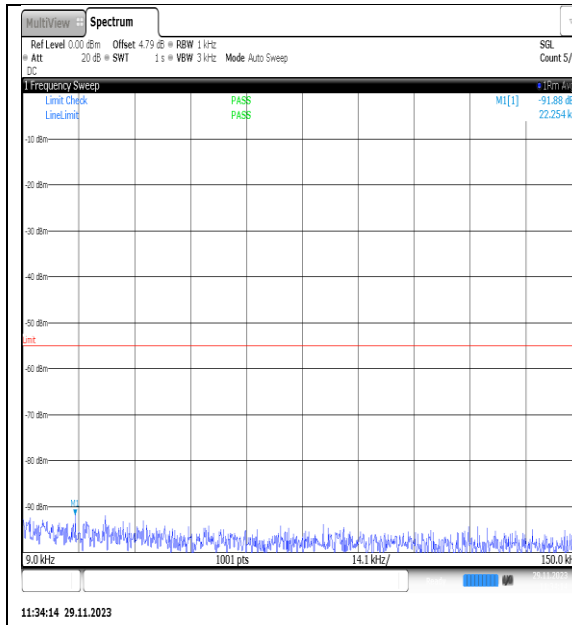
NTVN_N7_PC3_15_20_H_TID20_NS_01_0.009_0.15_#1
