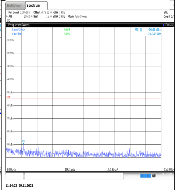
NTVN_N7_PC3_15_20_H_TID11_NS_01_0.009_0.15_#1
