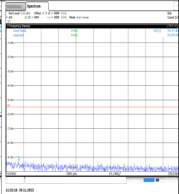
NTVN_N7_PC3_15_20_H_TID19_NS_01_0.009_0.15_#1
