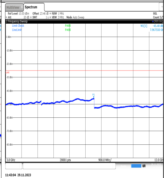
NTVN_N7_PC3_15_20_H_TID24_NS_01_3000_12000_#1
