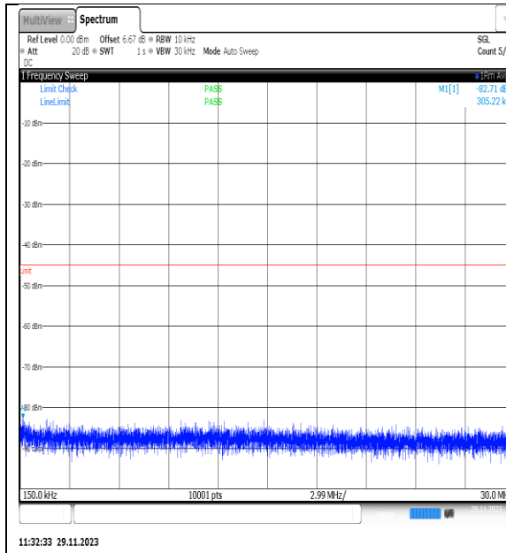
NTVN_N7_PC3_15_20_H_TID19_NS_01_0.15_3_0_#1
