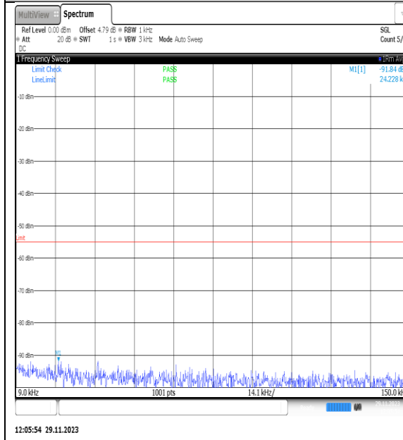
NTNV_N7_PC3_15_25_L_TID7_NS_01_0.009_0_15_#1
