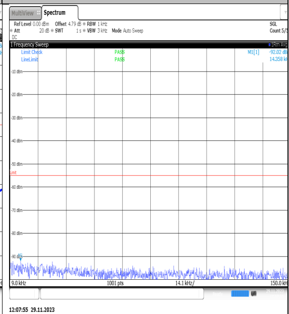
NTNV_N7_PC3_15_25_L_TID8_NS_01_0.009_0. 15_#1
