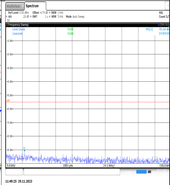
NTVN_N7_PC3_15_20_H_TID27_NS_01_0.009_0.15_#1
