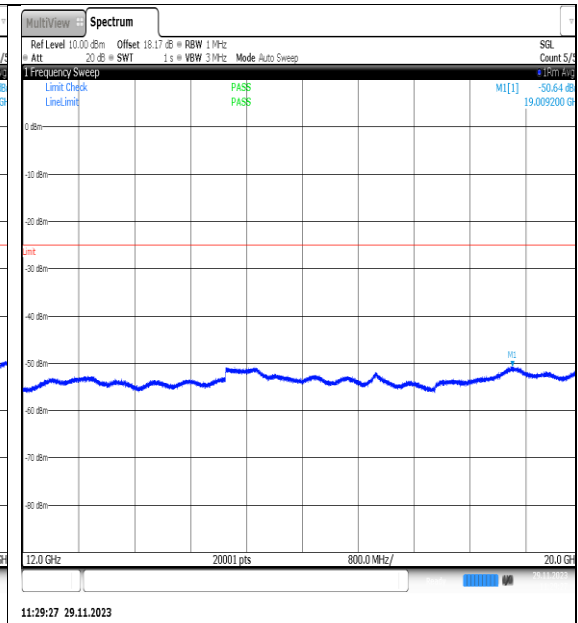
NTVN_N7_PC3_15_20_H_TID17_NS_01_12000_20000_#1
