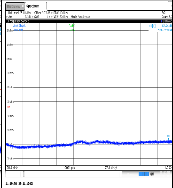
NTVN_N7_PC3_15_20_H_TID13_NS_01_30_100_0_#1
