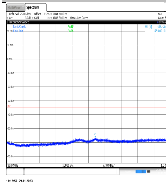
NTVN_N7_PC3_15_20_H_TID12_NS_01_30_100_0_#1
