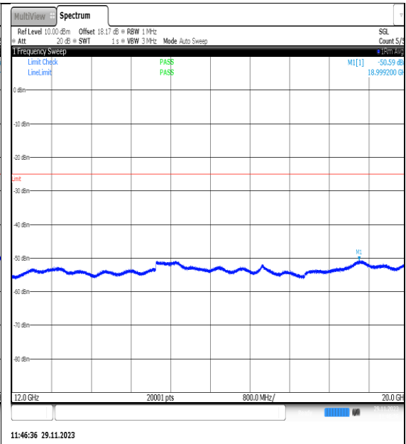
NTVN_N7_PC3_15_20_H_TID25_NS_01_12000_20000_#1
