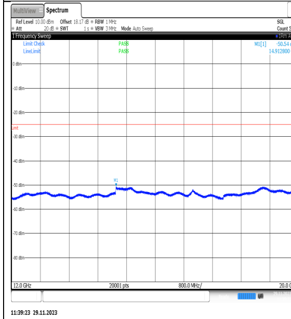
NTVN_N7_PC3_15_20_H_TID22_NS_01_12000_20000_#1
