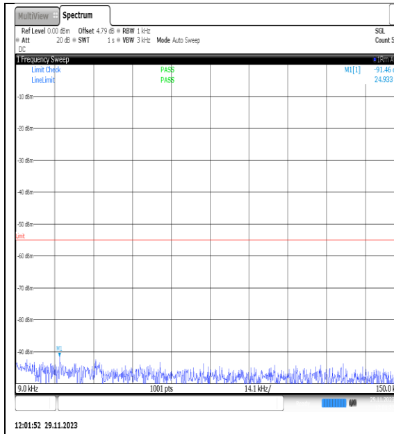
NTNV_N7_PC3_15_25_L_TID5_NS_01_0.009_0_15_#1
