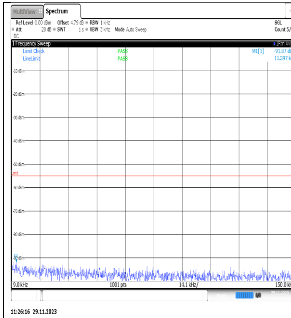
NTVN_N7_PC3_15_20_H_TID16_NS_01_0.009_0.15_#1
