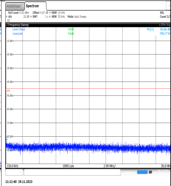
NTVN_N7_PC3_15_20_H_TID10_NS_01_0.15_3_0_#1
