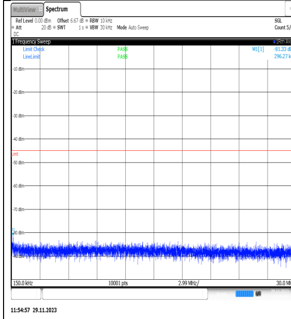
NTVN_N7_PC3_15_25_L_TID2_NS_01_0.15_30_#1
