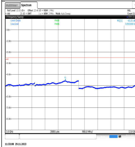
NTVN_N7_PC3_15_20_H_TID19_NS_01_3000_1_2000_#1
