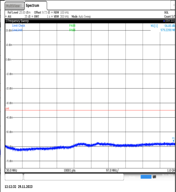
NTNV_N7_PC3_15_25_L_TID10_NS_01_30_100_0_#1
