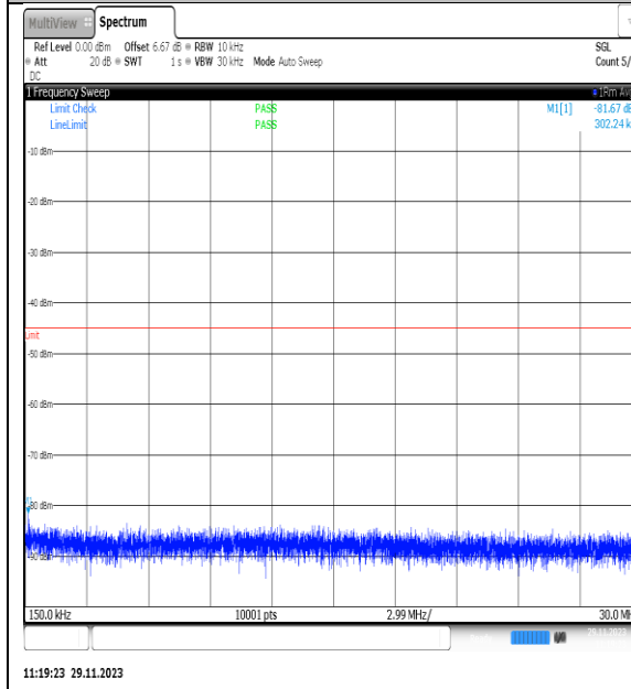
NTVN_N7_PC3_15_20_H_TID13_NS_01_0.15_30_#1
