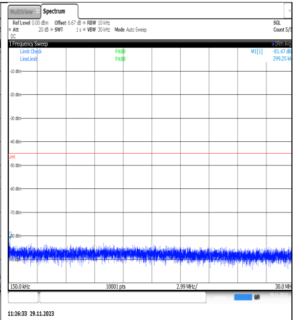
NTVN_N7_PC3_15_20_H_TID16_NS_01_0.15_3_0_#1
