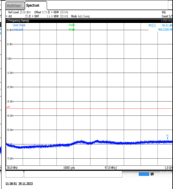
NTVN_N7_PC3_15_20_H_TID17_NS_01_30_100_0_#1
