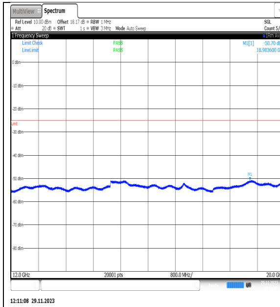
NTNV_N7_PC3_15_25_L_TID9_NS_01_12000_2_0000_#1
