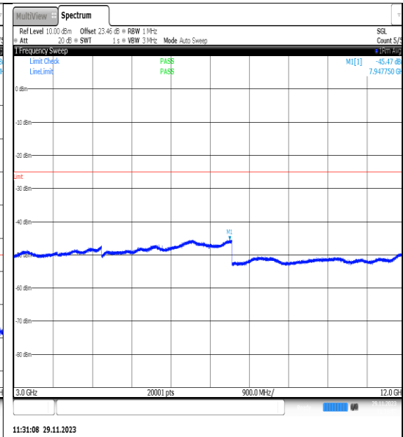
NTVN_N7_PC3_15_20_H_TID18_NS_01_3000_1_2000_#1
