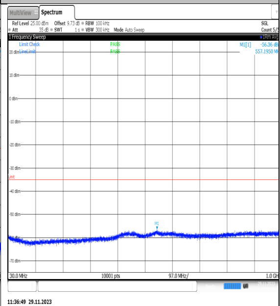
NTVN_N7_PC3_15_20_H_TID21_NS_01_30_100_0_#1
