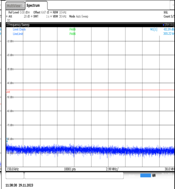
NTVN_N7_PC3_15_20_H_TID22_NS_01_0.15_30_#1
