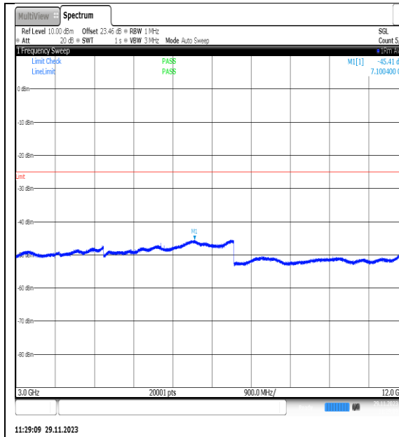
NTVN_N7_PC3_15_20_H_TID17_NS_01_3000_1_2000_#1
