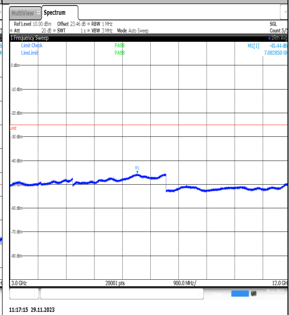
NTVN_N7_PC3_15_20_H_TID12_NS_01_3000_12000_#1
