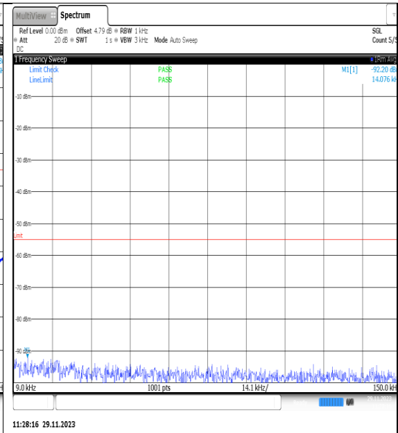
NTVN_N7_PC3_15_20_H_TID17_NS_01_0.009_0.15_#1
