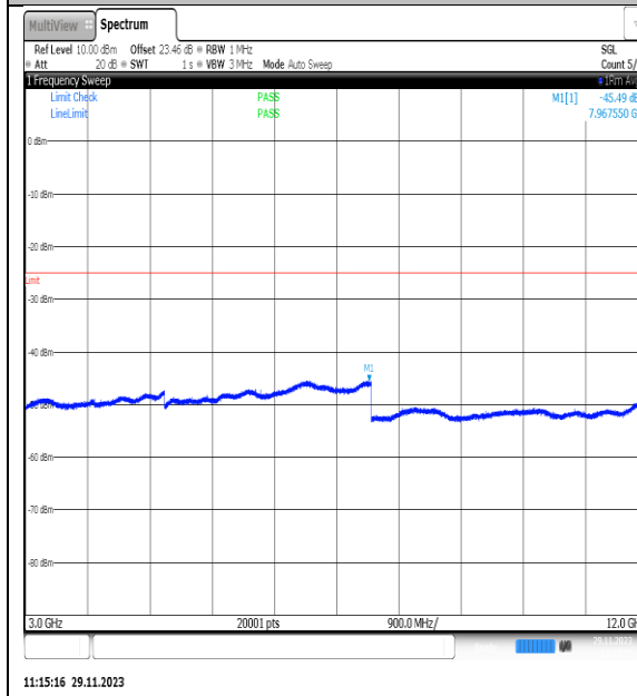
NTVN_N7_PC3_15_20_H_TID11_NS_01_3000_1_2000_#1
