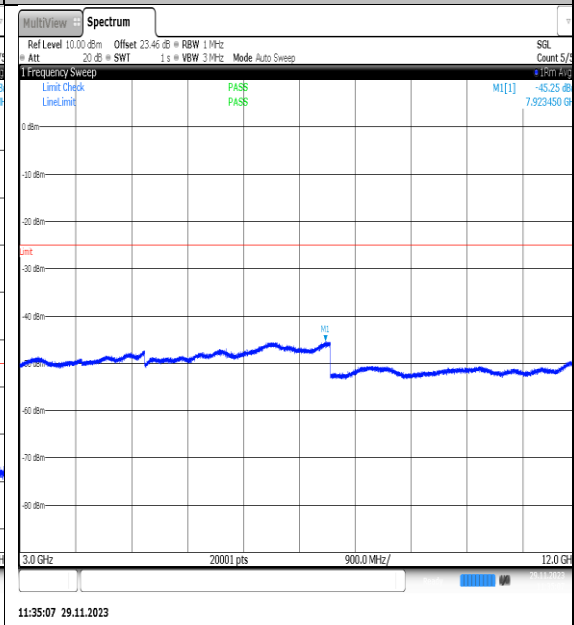
NTVN_N7_PC3_15_20_H_TID20_NS_01_3000_12000_#1
