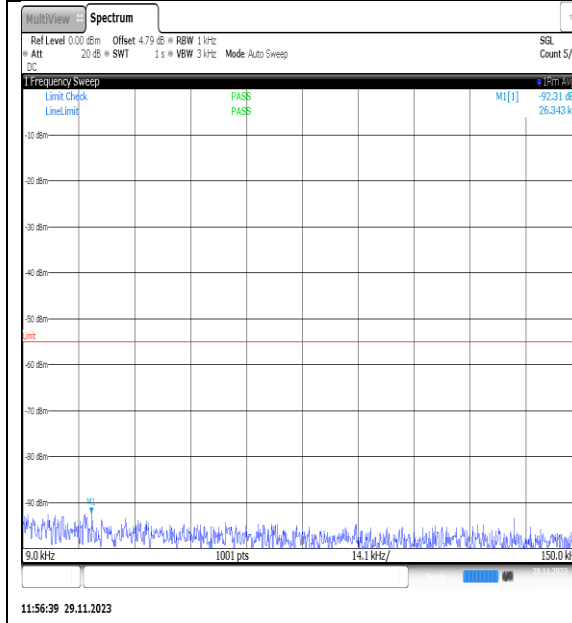
NTVN_N7_PC3_15_25_L_TID3_NS_01_0.009_0_15_#1
