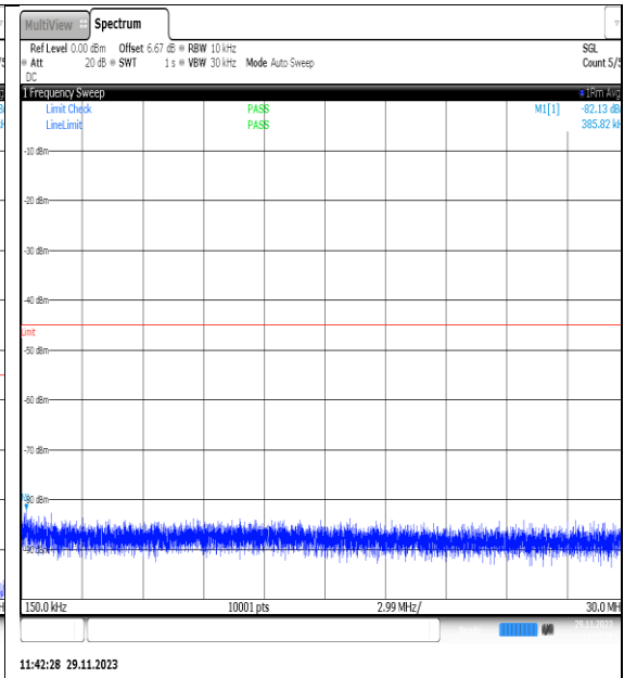
NTVN_N7_PC3_15_20_H_TID24_NS_01_0.15_3_0_#1
