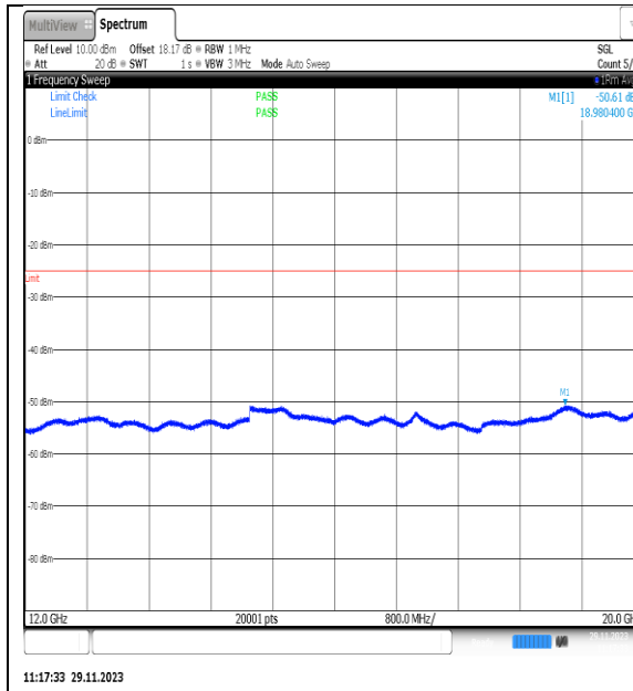
NTVN_N7_PC3_15_20_H_TID12_NS_01_12000_20000_#1
