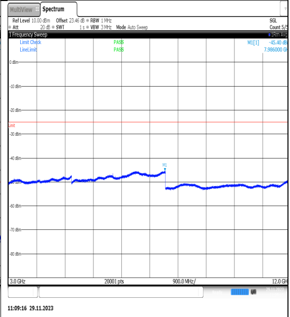
NTVN_N7_PC3_15_20_H_TID8_NS_01_3000_12000_#1
