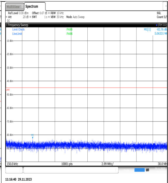
NTVN_N7_PC3_15_20_H_TID12_NS_01_0.15_3_0_#1
