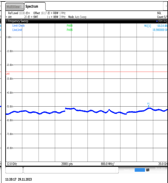
NTVN_N7_PC3_15_20_H_TID13_NS_01_12000_20000_#1
