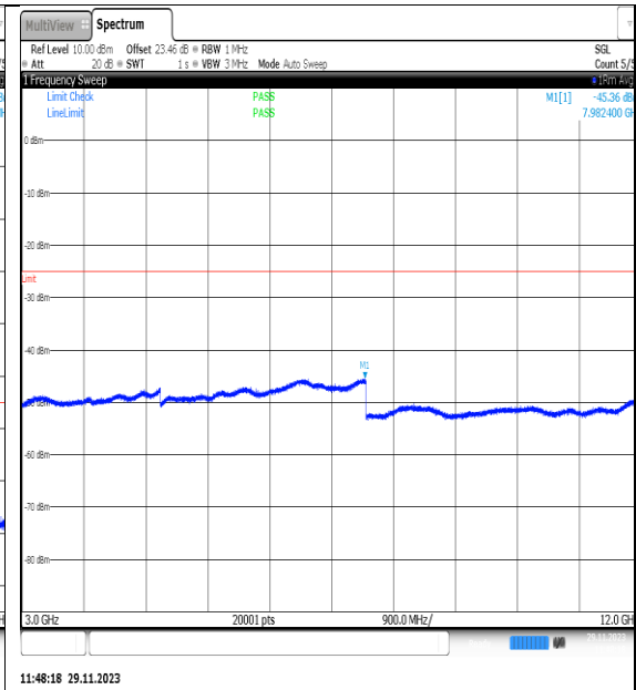
NTVN_N7_PC3_15_20_H_TID26_NS_01_3000_1_2000_#1
