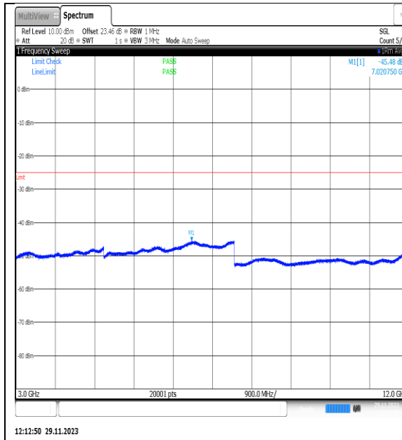
NTNV_N7_PC3_15_25_L_TID10_NS_01_3000_1 2000_#1
