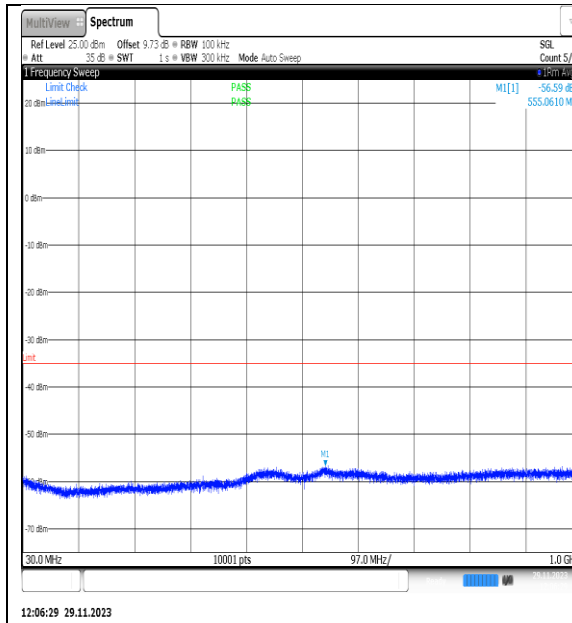
NTNV_N7_PC3_15_25_L_TID7_NS_01_30_1000 _#1
