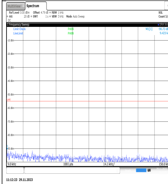
NTVN_N7_PC3_15_20_H_TID10_NS_01_0.009_0.15_#1
