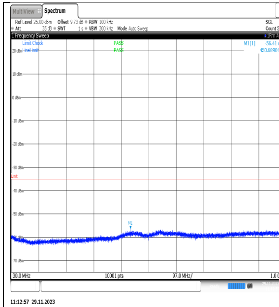
NTVN_N7_PC3_15_20_H_TID10_NS_01_30_100_0_#1
