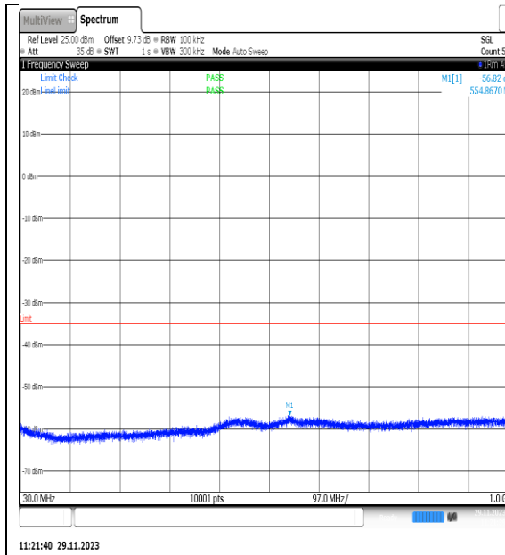
NTVN_N7_PC3_15_20_H_TID14_NS_01_30_100_0_#1
