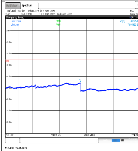
NTVN_N7_PC3_15_20_H_TID27_NS_01_3000_1_2000_#1
