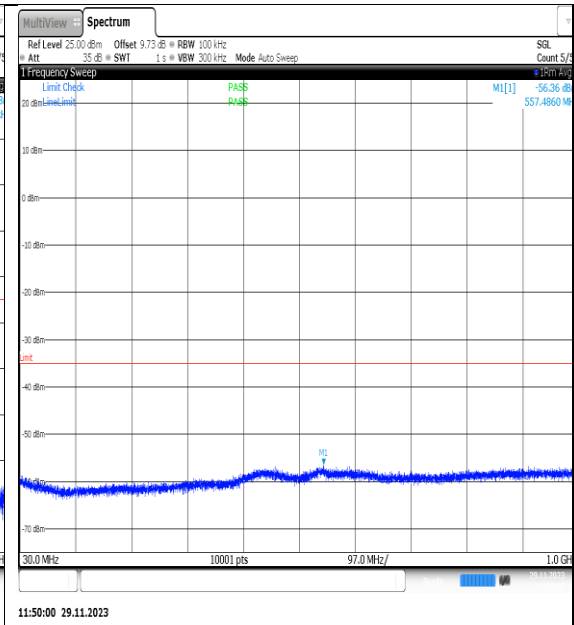
NTVN_N7_PC3_15_20_H_TID27_NS_01_30_100_0_#1
