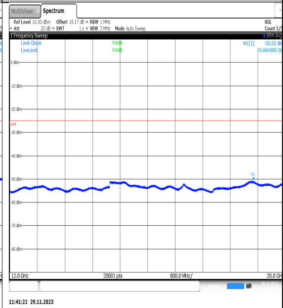
NTVN_N7_PC3_15_20_H_TID23_NS_01_12000_20000_#1
