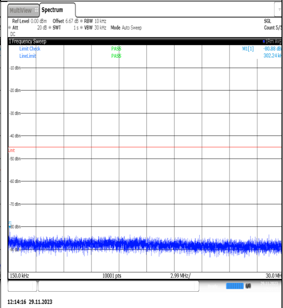
NTNV_N7_PC3_15_25_L_TID11_NS_01_0.15_30_#1
