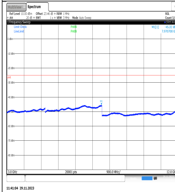
NTVN_N7_PC3_15_20_H_TID23_NS_01_3000_1_2000_#1
