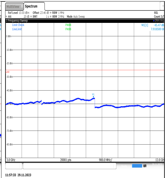
NTVN_N7_PC3_15_25_L_TID3_NS_01_3000_12 000_#1
