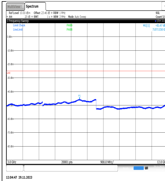
NTNV_N7_PC3_15_25_L_TID6_NS_01_3000_12_000_#1
