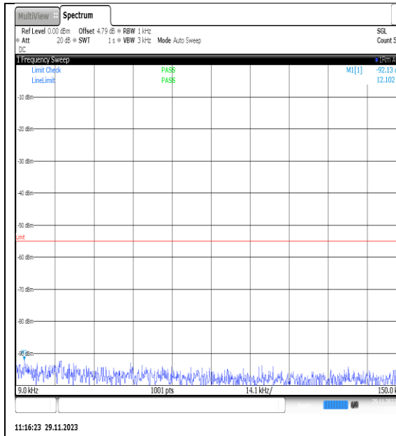
NTVN_N7_PC3_15_20_H_TID12_NS_01_0.009_0.15_#1
