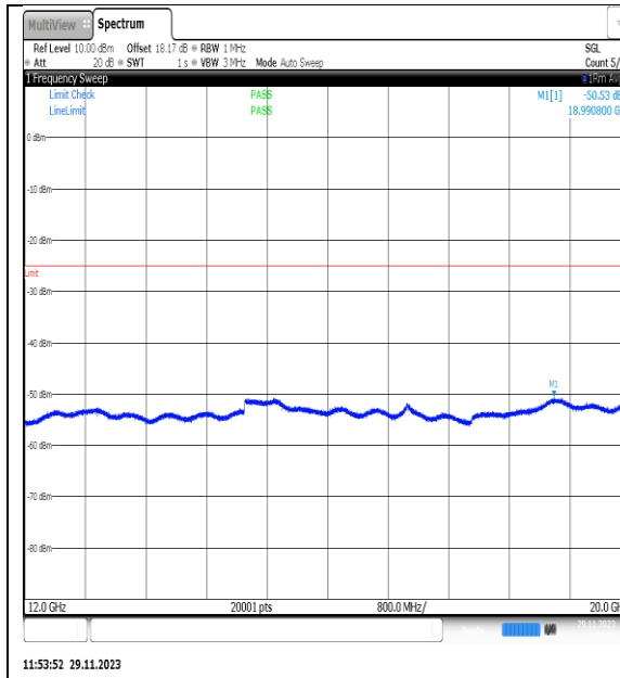
NTVN_N7_PC3_15_25_L_TID1_NS_01_12000_2_0000_#1
