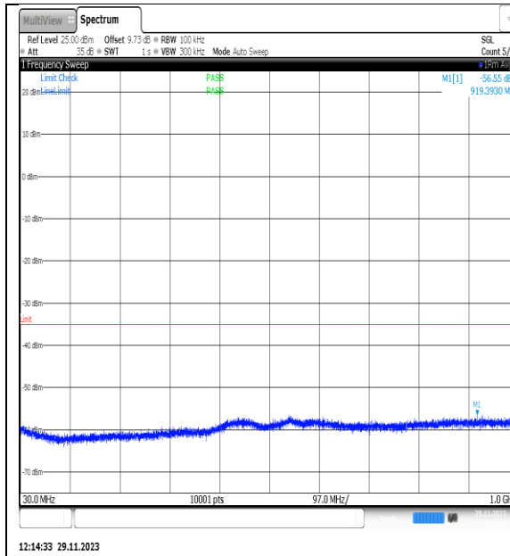
NTVN_N7_PC3_15_25_L_TID11_NS_01_30_100_0_#1
