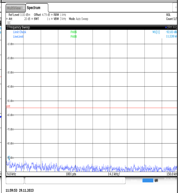
NTVN_N7_PC3_15_25_L_TID4_NS_01_0.009_0. 15_#1
