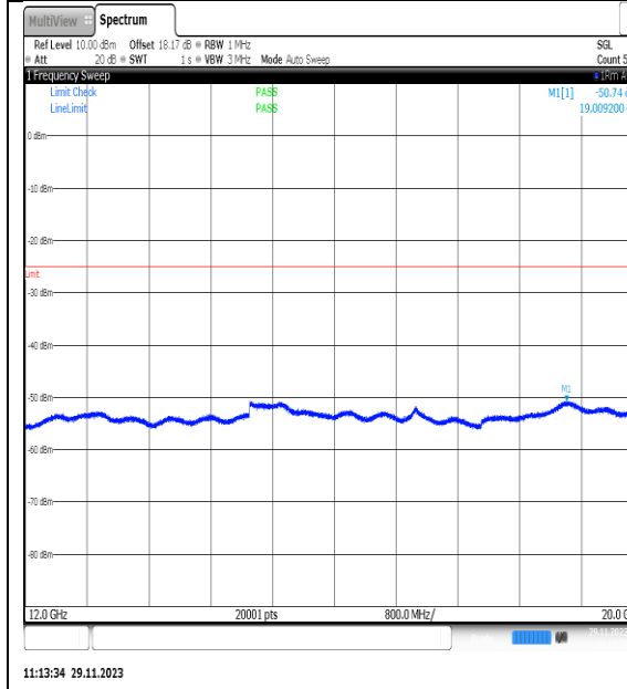
NTVN_N7_PC3_15_20_H_TID10_NS_01_12000_20000_#1
