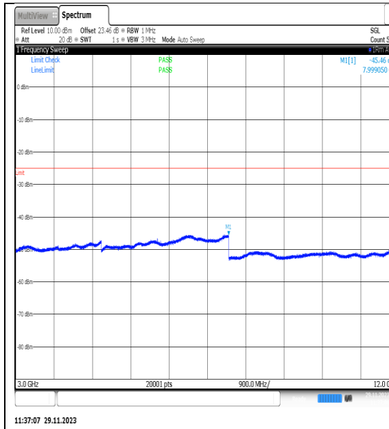
NTVN_N7_PC3_15_20_H_TID21_NS_01_3000_1_2000_#1
