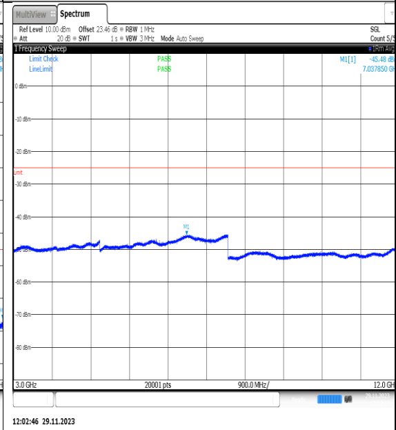
NTNV_N7_PC3_15_25_L_TID5_NS_01_3000_12000_#1
