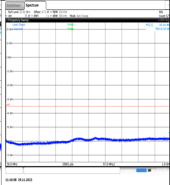
NTVN_N7_PC3_15_20_H_TID9_NS_01_30_1000_#1
