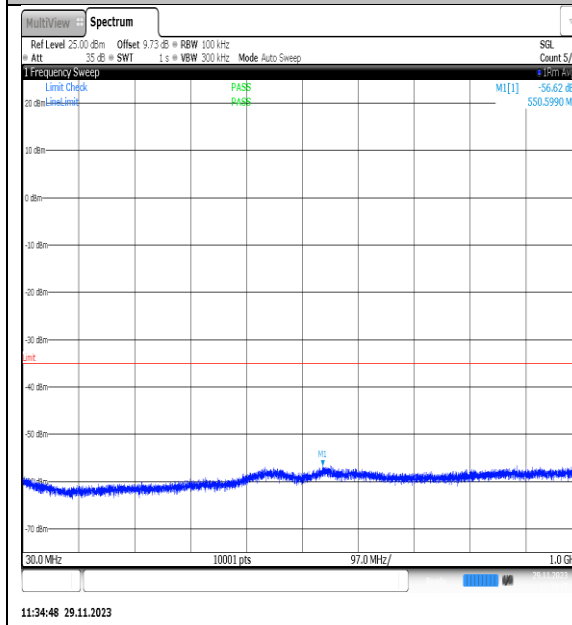
NTVN_N7_PC3_15_20_H_TID20_NS_01_30_100_0_#1
