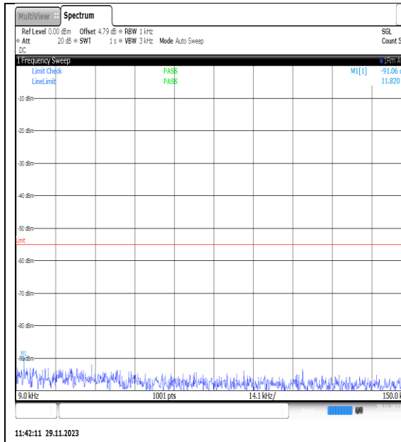
NTVN_N7_PC3_15_20_H_TID24_NS_01_0.009_0.15_#1
