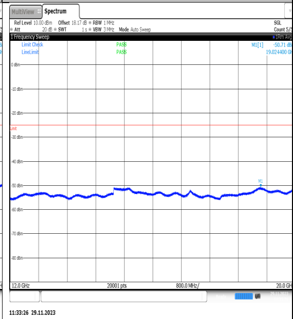
NTVN_N7_PC3_15_20_H_TID19_NS_01_12000_20000_#1
