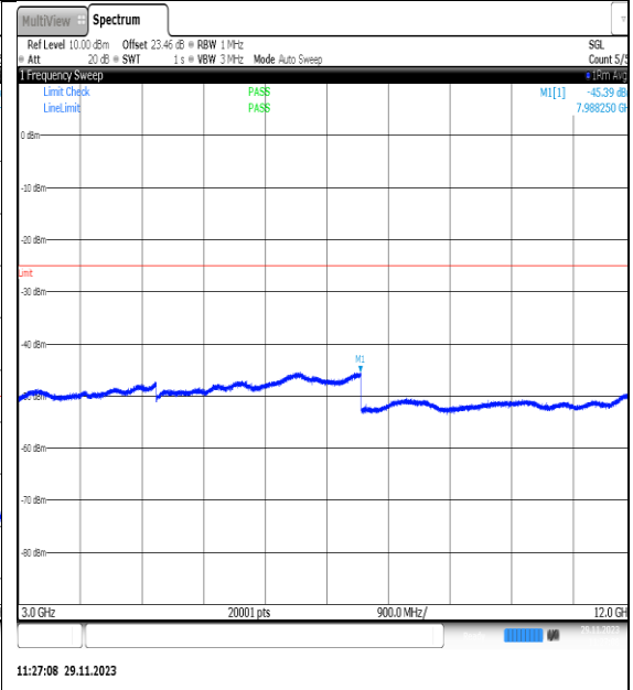
NTVN_N7_PC3_15_20_H_TID16_NS_01_3000_1_2000_#1
