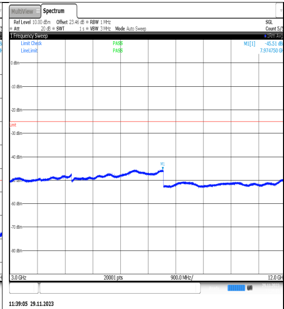
NTVN_N7_PC3_15_20_H_TID22_NS_01_3000_1_2000_#1
