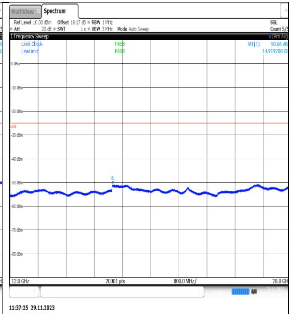
NTVN_N7_PC3_15_20_H_TID21_NS_01_12000_20000_#1
