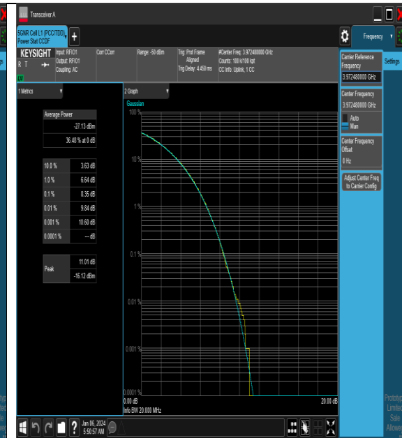
NTNV_N77-3700-3980_PC2_30_15_H_TID3_#1
