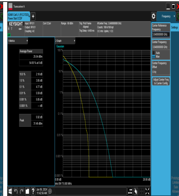
NTNV_N77-3700-3980_PC2_30_60_M_TID1_#1
