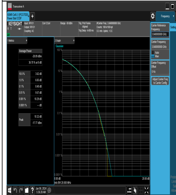
NTNV_N77-3700-3980_PC2_30_15_M_TID5_#1
