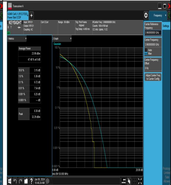
NTNV_N77-3700-3980_PC2_30_40_H_TID3_#1
