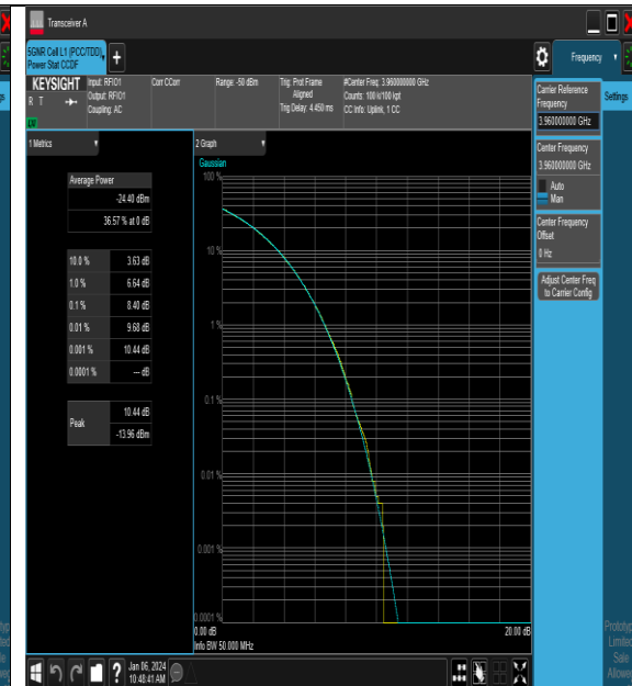
NTNV_N77-3700-3980_PC2_30_40_H_TID5_#1
