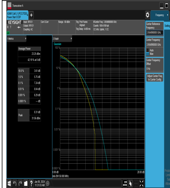
NTNV_N77-3700-3980_PC2_30_50_H_TID4_#1
