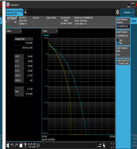
NTNV_N77-3700-3980_PC2_30_15_H_TID2_#1
