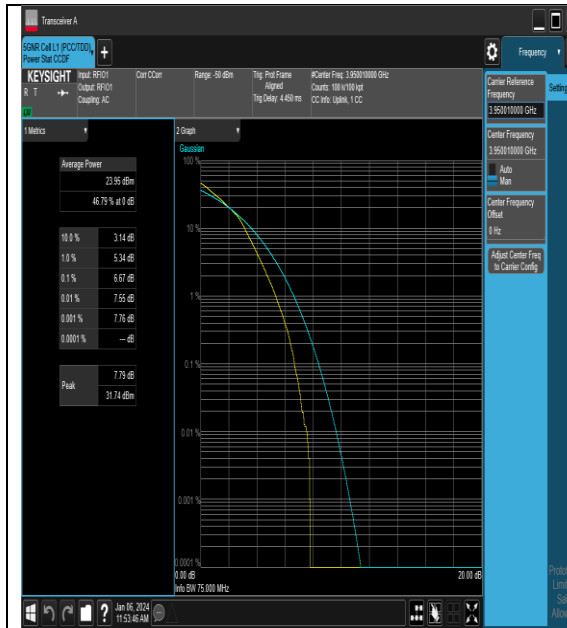
NTNV_N77-3700-3980_PC2_30_60_H_TID3_#1
