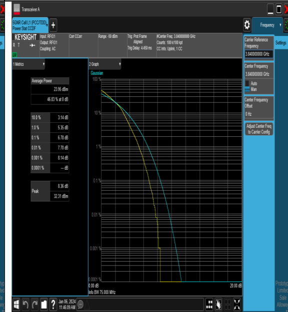
NTNV_N77-3700-3980_PC2_30_60_M_TID3_#1
