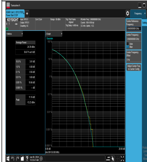
NTNV_N77-3700-3980_PC2_30_40_H_TID1_#1
