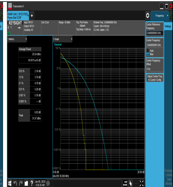
NTNV_N77-3700-3980_PC2_30_30_M_TID1_#1
