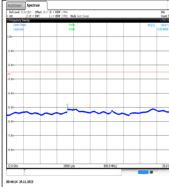
NTVN_N7_PC3_15_5_M_TID16_NS_01_12000_20000_#1
