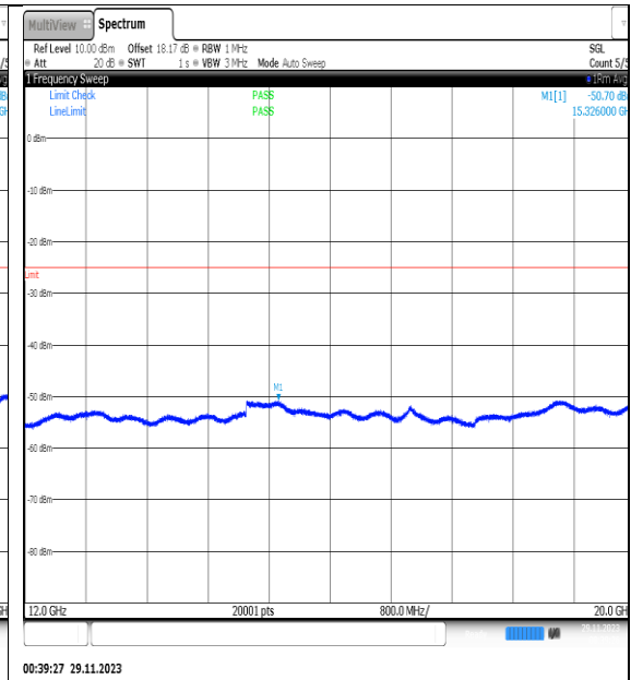
NTVN_N7_PC3_15_5_M_TID15_NS_01_12000_20000_#1
