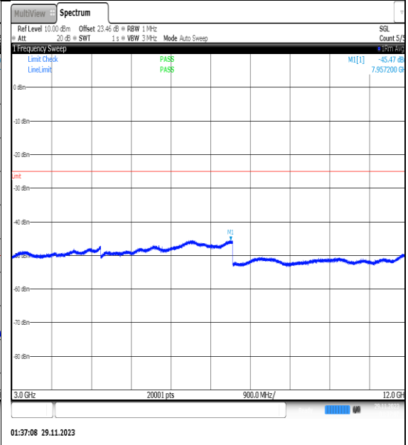
NTVN_N7_PC3_15_5_H_TID3_NS_01_3000_120_00_#1
