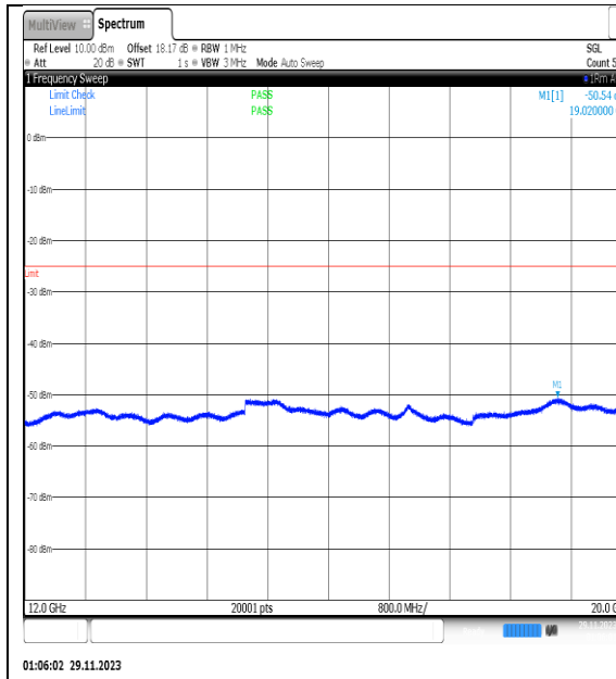
NTVN_N7_PC3_15_5_M_TID22_NS_01_12000_20000_#1
