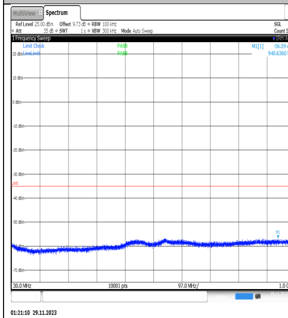
NTVN_N7_PC3_15_5_M_TID26_NS_01_30_100_0_#1
