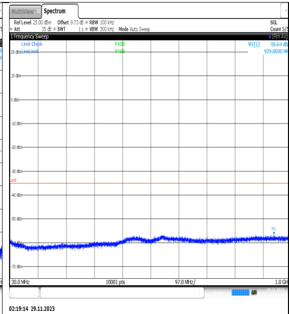
NTVN_N7_PC3_15_5_H_TID14_NS_01_30_1000 _#1
