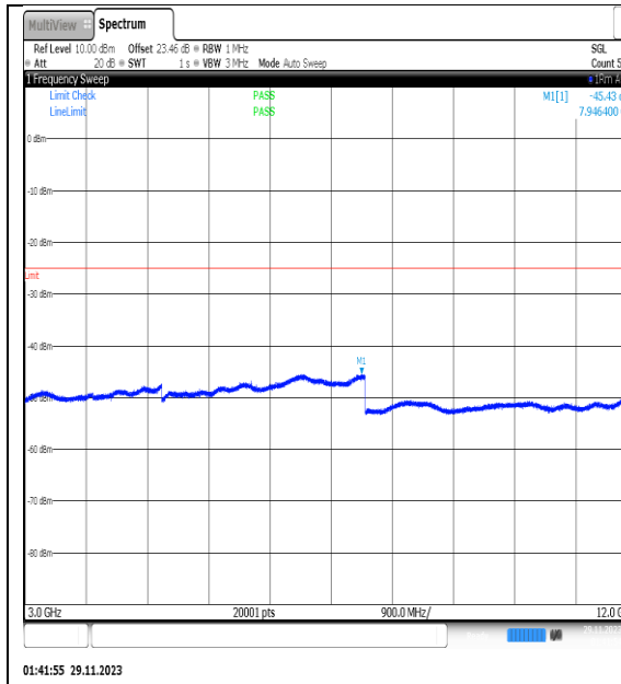
NTVN_N7_PC3_15_5_H_TID4_NS_01_3000_120_00_#1
