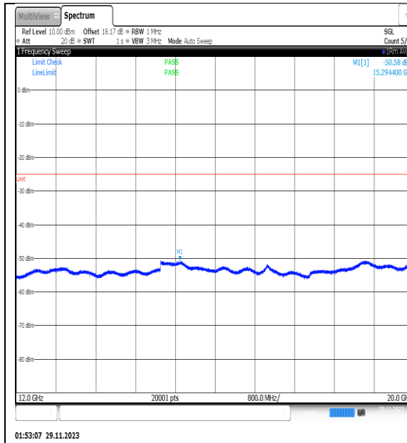
NTVN_N7_PC3_15_5_H_TID7_NS_01_12000_2000_#1
