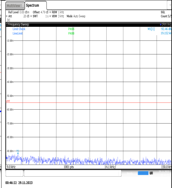
NTVN_N7_PC3_15_5_M_TID17_NS_01_0.009_0.15_#1
