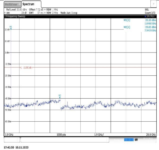
Band2-1.4MHz-16QAM-18900-1RB#0-Range2:1000~20000MHz
