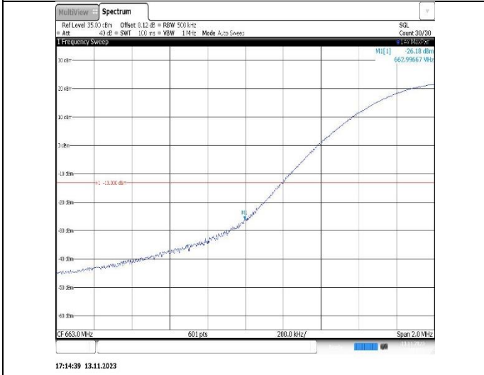
Band71-20MHz-QPSK-133222-100RB#0
