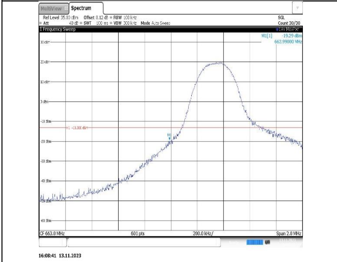
Band71-5MHz-16QAM-133147-25RB#0
