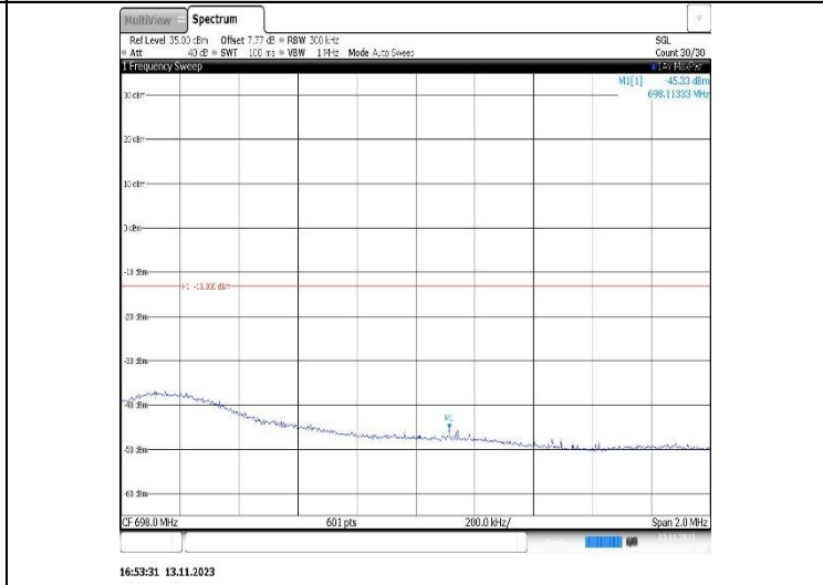
Band71-15MHz-16QAM-133397-75RB#0
