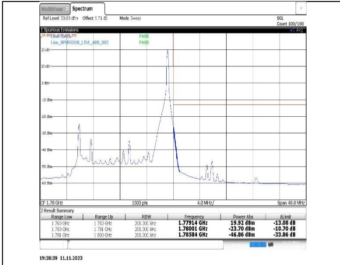
Band66-15MHz-16QAM-132047-1RB#0
