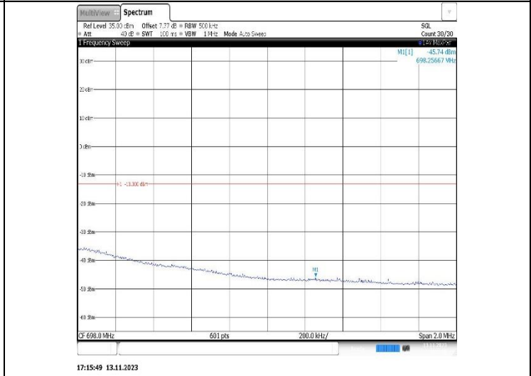
Band71-20MHz-16QAM-133372-100RB#0
