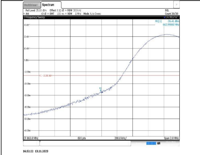
Band71-15MHz-QPSK-133197-75RB#0
