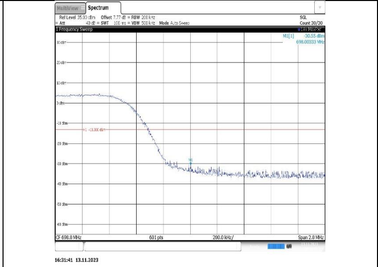
Band71-10MHz-16QAM-133172-1RB#49
