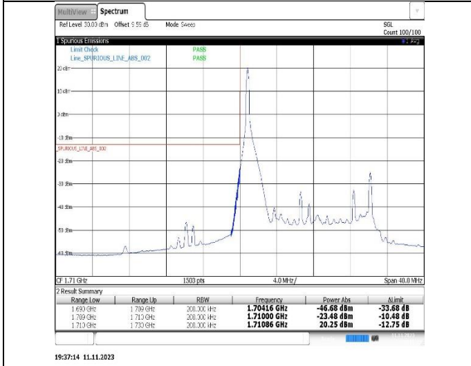
Band66-15MHz-16QAM-132597-1RB#74
