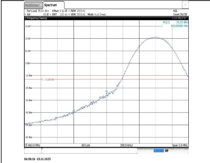
Band71-10MHz-16QAM-133172-50RB#0
