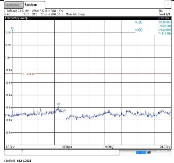
Band2-1.4MHz-16QAM-18607-1RB#0-Range2:1000~20000MHz
