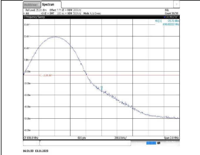
Band71-15MHz-QPSK-133197-1RB#0
