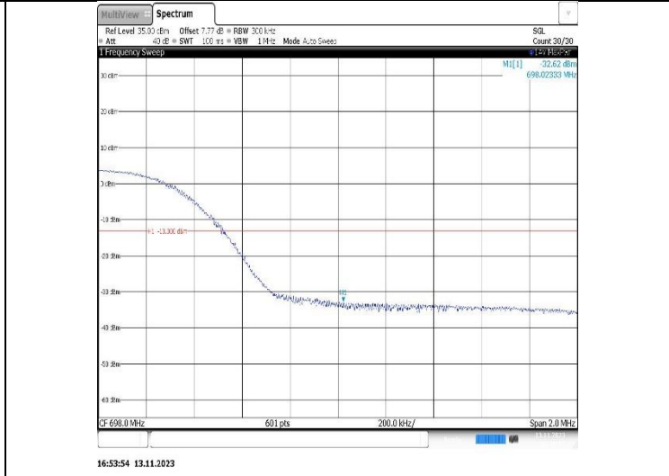
Band71-15MHz-16QAM-133197-1RB#74
