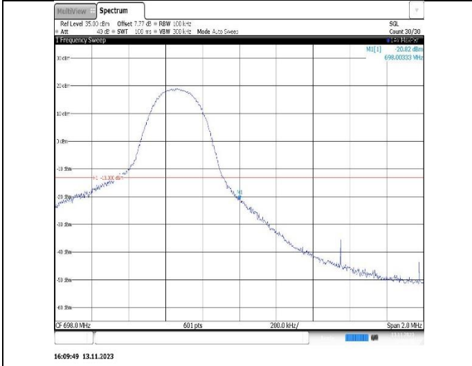
Band71-5MHz-16QAM-133147-1RB#0
