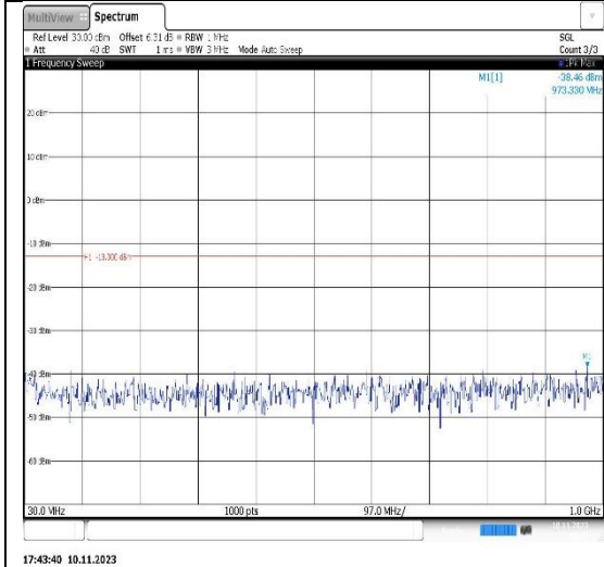
Band2-1.4MHz-16QAM-18607-1RB#0-Range1:30~1000MHz
