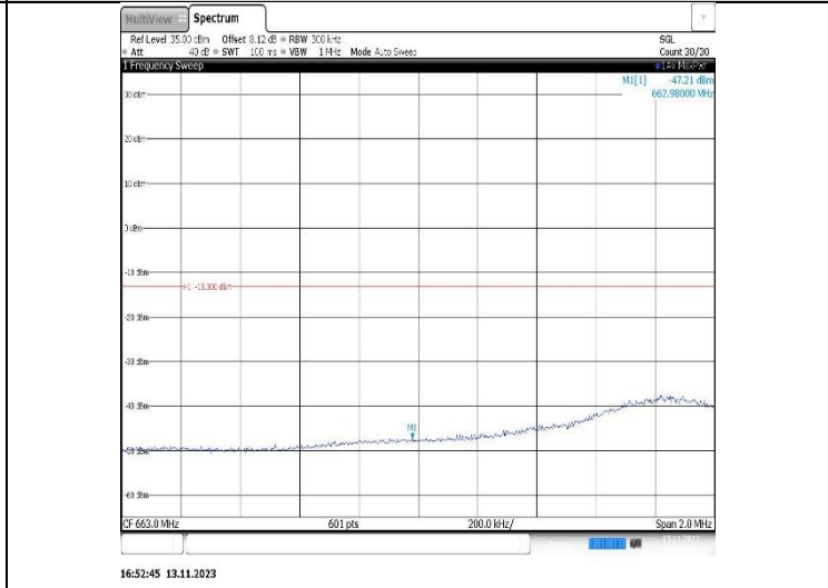
Band71-15MHz-16QAM-133397-1RB#0
