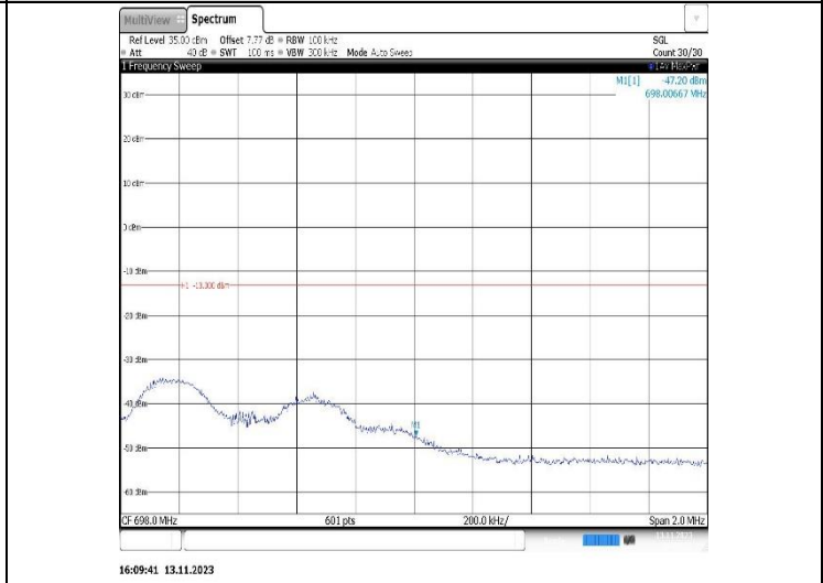
Band71-5MHz-16QAM-133447-25RB#0
