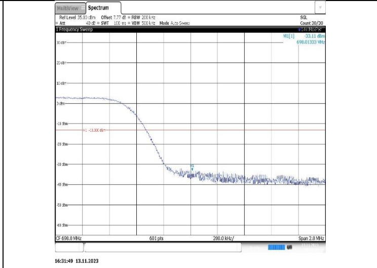
Band71-15MHz-QPSK-133197-1RB#74
