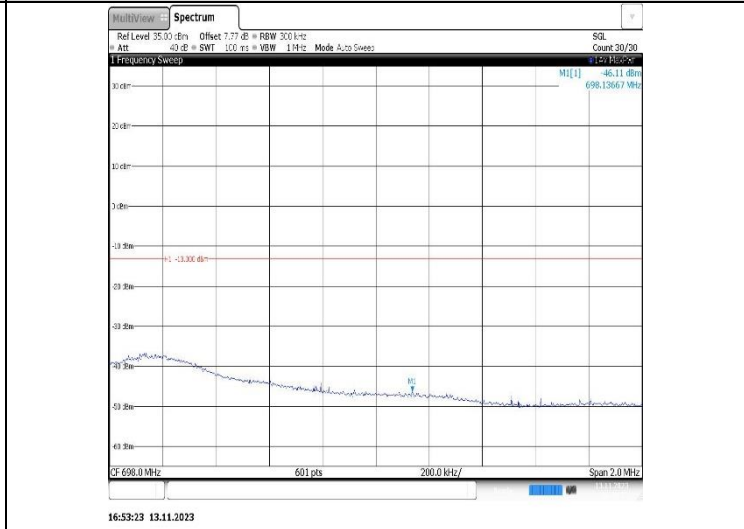
Band71-15MHz-QPSK-133397-75RB#0
