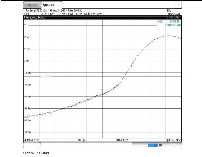
Band71-15MHz-16QAM-133197-75RB#0
