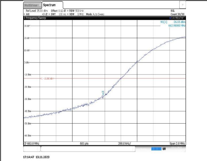
Band71-20MHz-16QAM-133222-100RB#0
