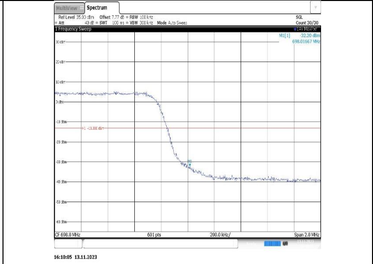
Band71-5MHz-16QAM-133147-1RB#24
