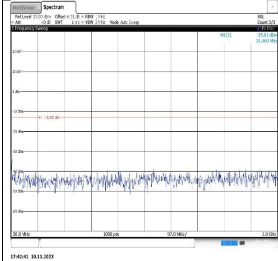
Band2-1.4MHz-16QAM-18900-1RB#0-Range1:30~1000MHz
