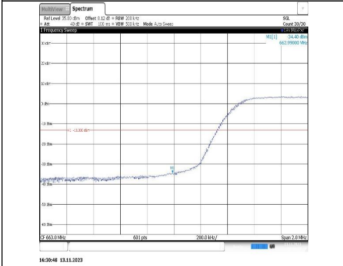
Band71-10MHz-16QAM-133422-1RB#49
