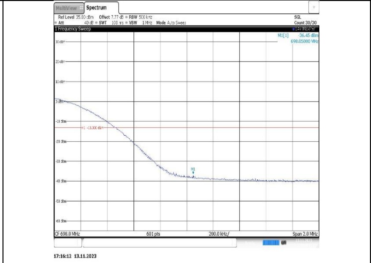
Band71-20MHz-16QAM-133222-1RB#99
