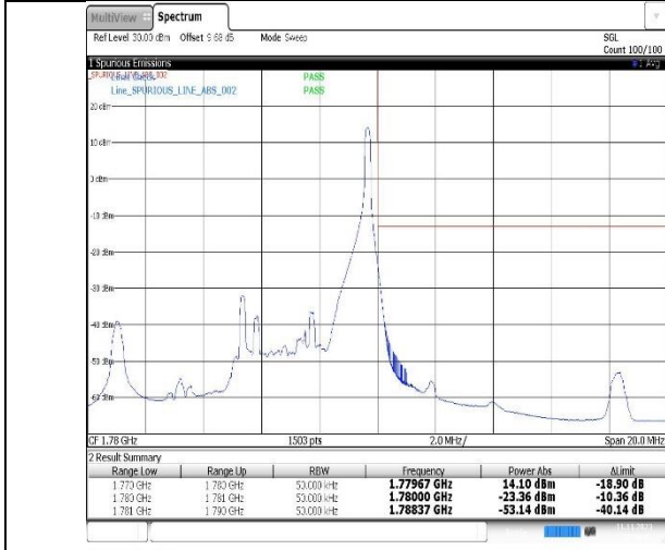
Band66-10MHz-QPSK-132022-1RB#0
