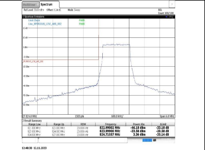
Band26(824-849)-1.4MHz-16QAM-27033-6RB#0
