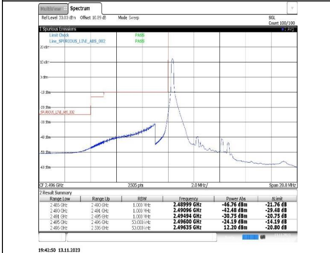
Band41-5MHz-16QAM-39675-1RB#0
