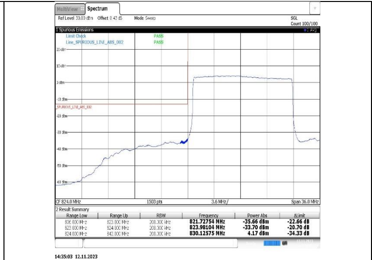
Band26(824-849)-15MHz-16QAM-26865-75RB#0
