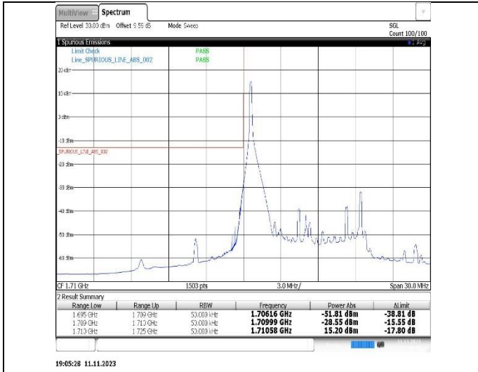
Band66-10MHz-16QAM-132622-1RB#49
