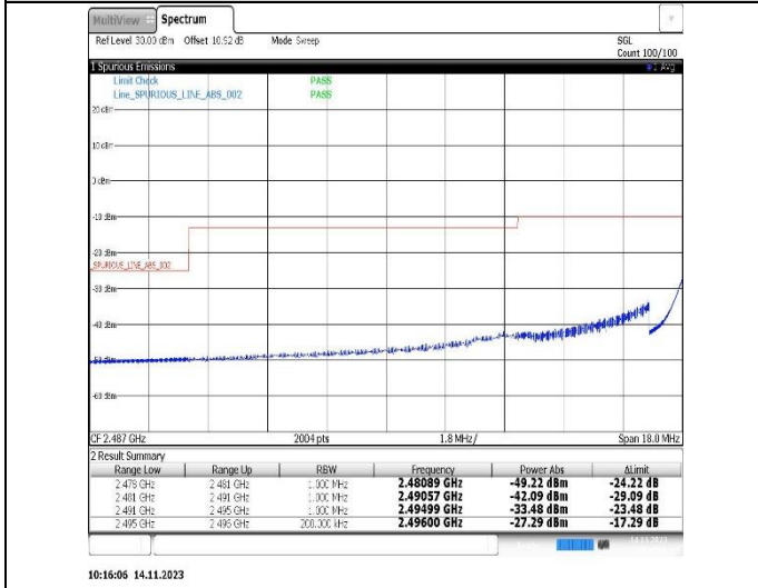
10:16:06 14.11.2023 Band41-20MHz-QPSK-39750-1RB#99
