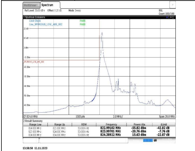
Band26(824-849)-5MHz-16QAM-27015-1RB#24
