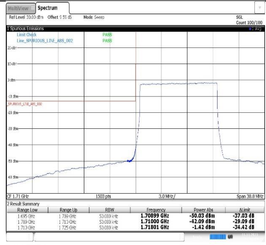
Band66-10MHz-QPSK-132622-50RB#0
