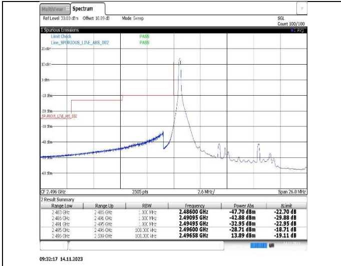
09:32:17 14.11.2023 Band41-10MHz-16QAM-41540-1RB#49
