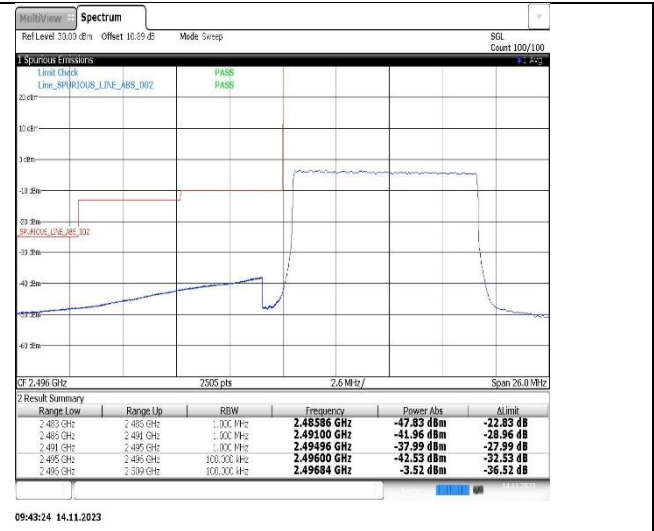
09:43:24 14.11.2023 Band41-10MHz-16QAM-41540-50RB#0
