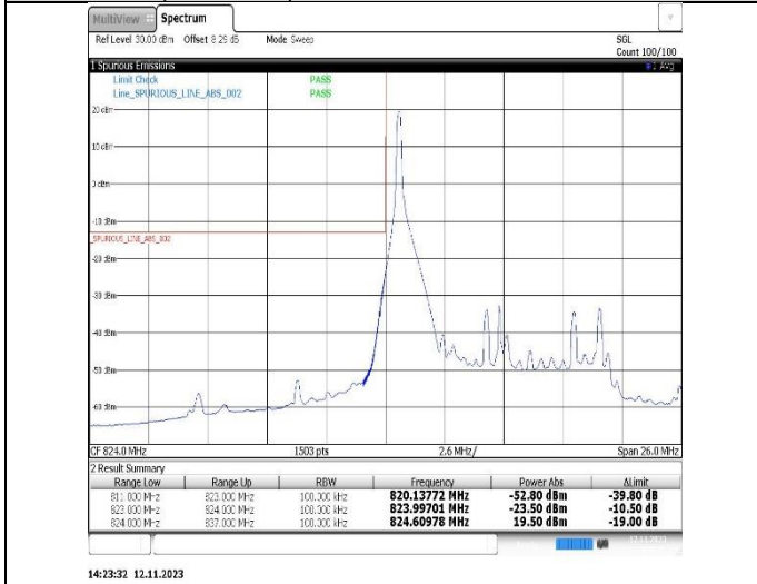
Band26(824-849)-10MHz-16QAM-26840-1RB#0
