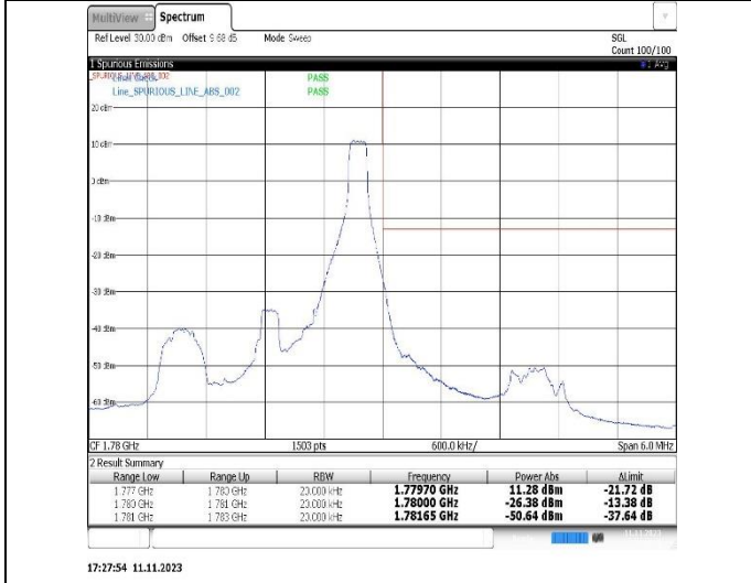
Band66-1.4MHz-16QAM-131979-1RB#0
