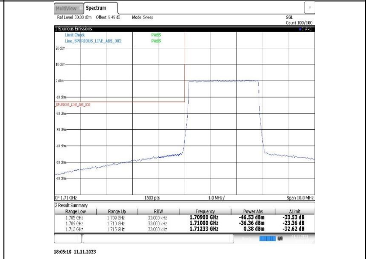
Band66-3MHz-16QAM-132657-15RB#0
