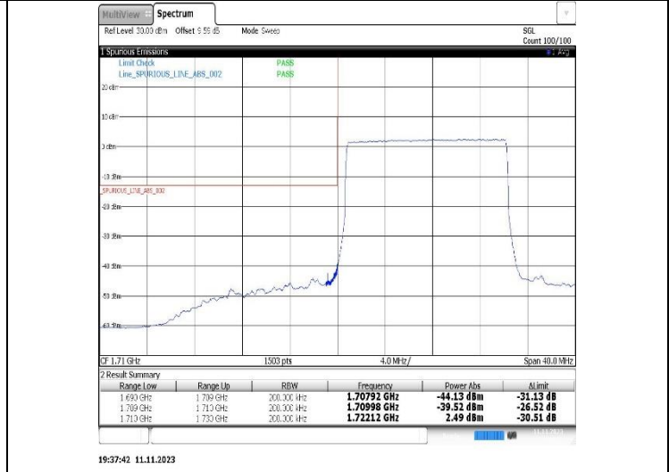
Band66-15MHz-QPSK-132597-75RB#0
