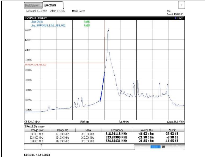
Band26(824-849)-15MHz-16QAM-26865-1RB#0
