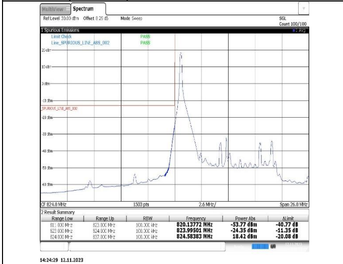
Band26(824-849)-15MHz-QPSK-26865-1RB#0
