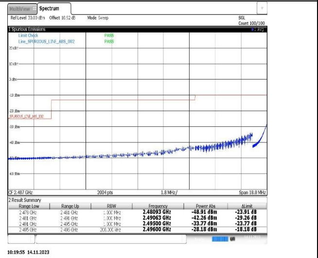
10:19:55 14.11.2023 Band41-20MHz-QPSK-39750-100RB#0
