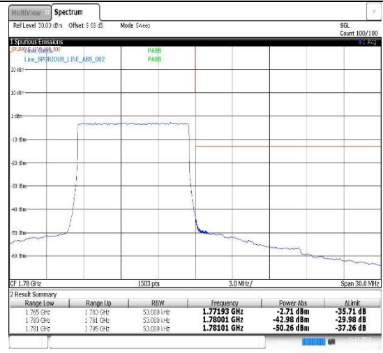
Band66-10MHz-16QAM-132022-50RB#0
