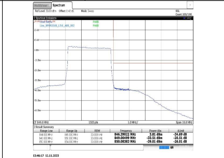
Band26(824-849)-5MHz-QPSK-26815-25RB#0
