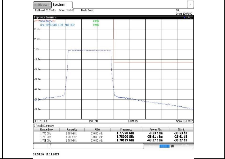
Band66-5MHz-QPSK-131997-25RB#0
