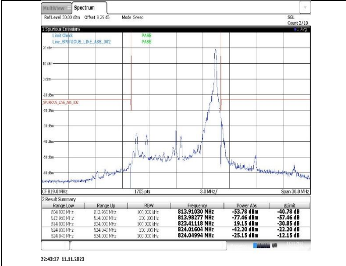
Band26(824-849)-1.4MHz-QPSK-26797-1RB#0
