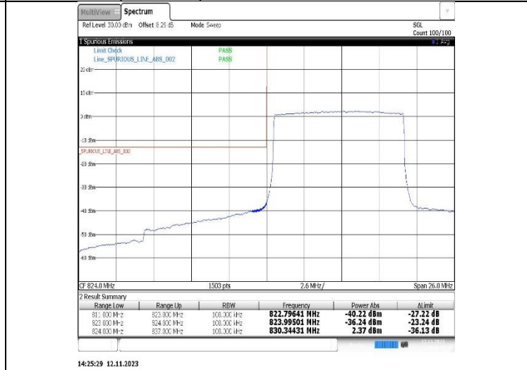
Band26(824-849)-10MHz-16QAM-26840-50RB#0
