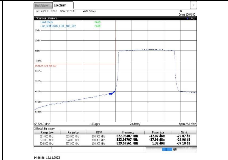
Band26(824-849)-15MHz-QPSK-26865-75RB#0
