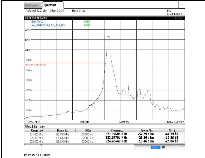
Band26(824-849)-3MHz-16QAM-27025-1RB#14
