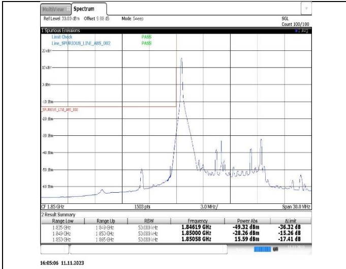
Band25-10MHz-QPSK-26640-1RB#49
