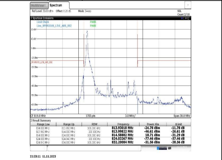
Band26(814-824)-10MHz-16QAM-26740-50RB#0
