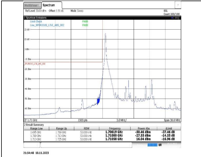
Band4-10MHz-QPSK-20350-1RB#49
