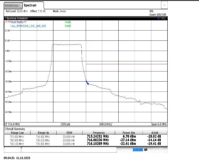
09:54:31 11.11.2023 Band12-1.4MHz-16QAM-23017-6RB#0
