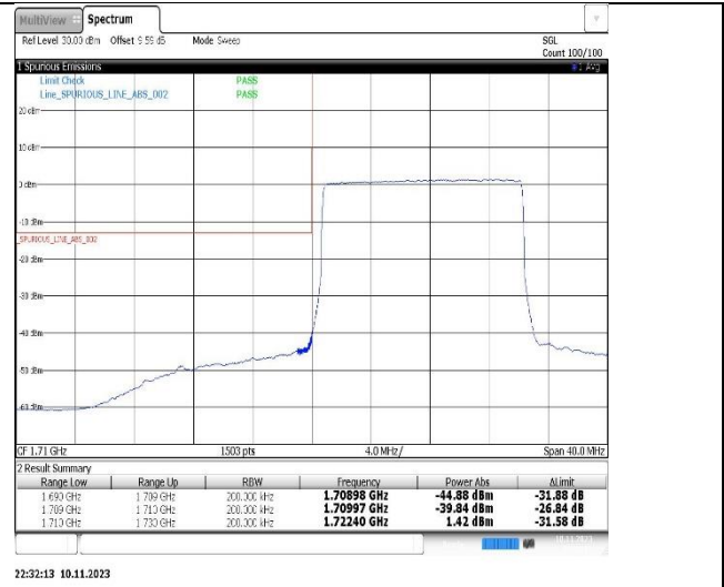
Band4-15MHz-16QAM-20325-75RB#0
