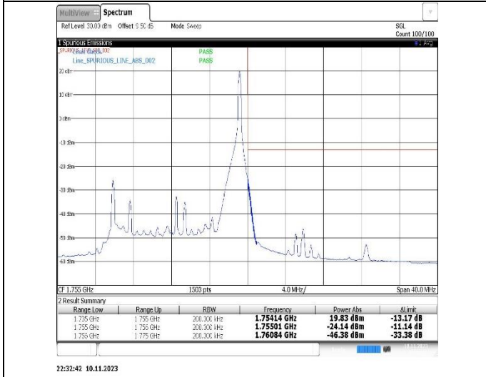
Band4-15MHz-QPSK-20325-1RB#74
