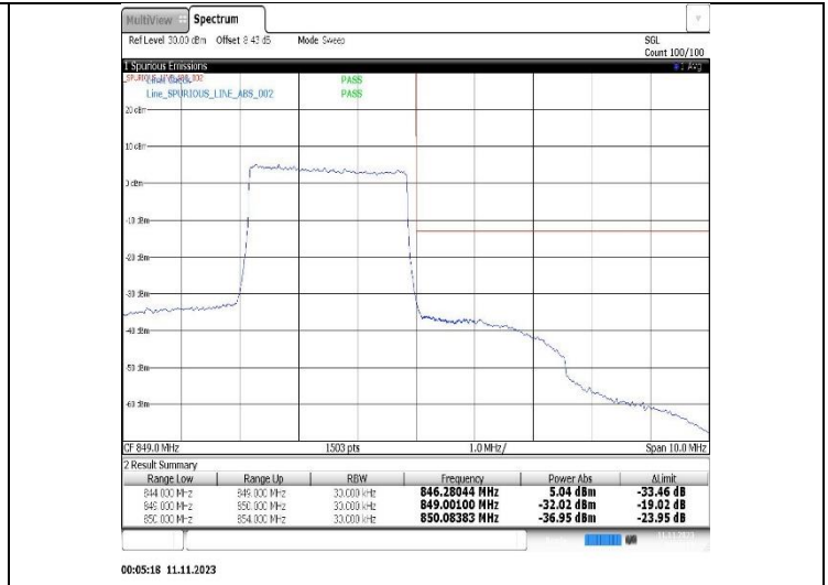
Band5-3MHz-16QAM-20415-15RB#0
