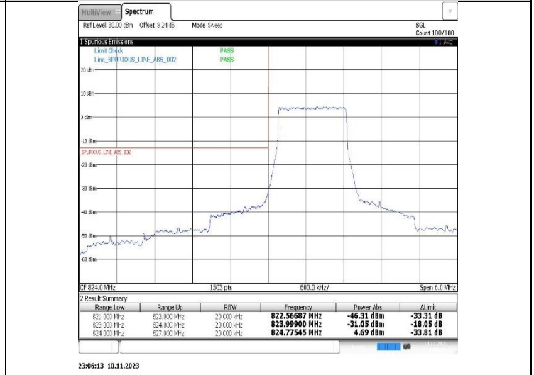
Band5-1.4MHz-QPSK-20643-6RB#0
