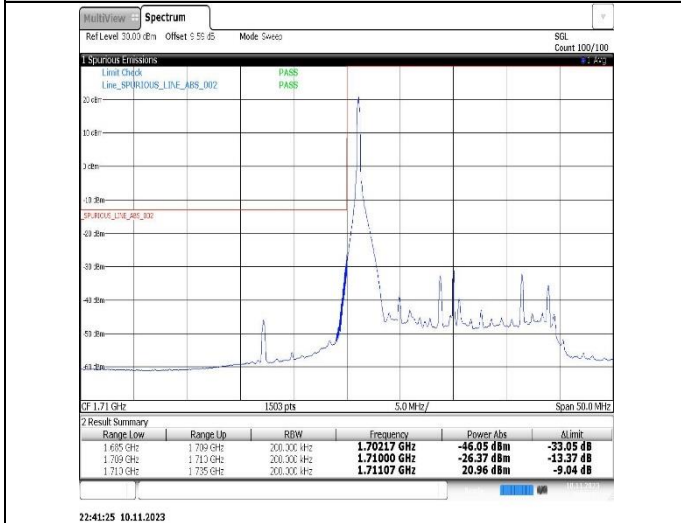
Band4-20MHz-16QAM-20050-1RB#0
