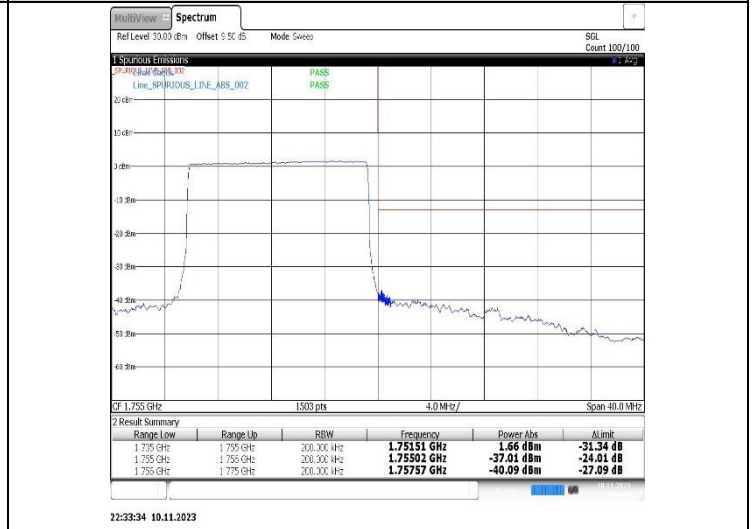
Band4-15MHz-QPSK-20325-75RB#0
