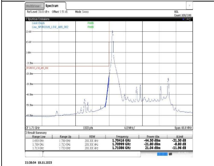
Band4-15MHz-QPSK-20025-1RB#0
