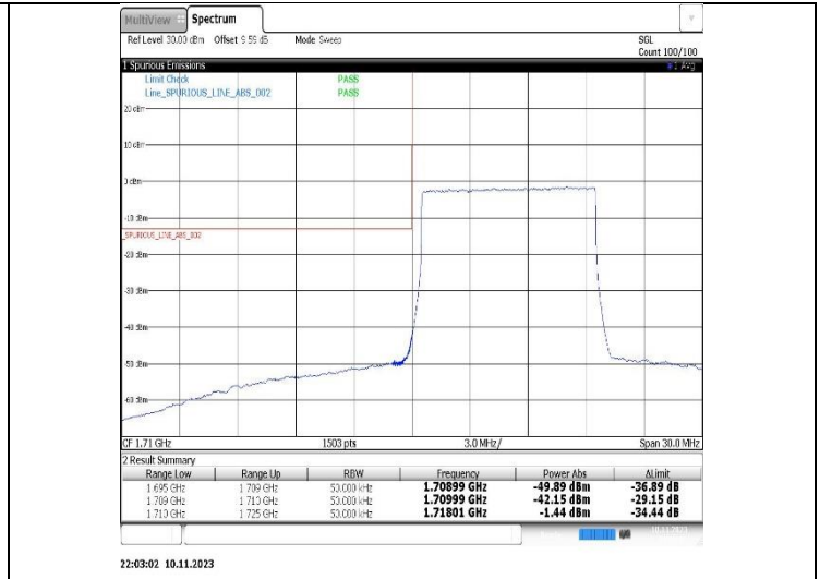
Band4-10MHz-QPSK-20350-50RB#0
