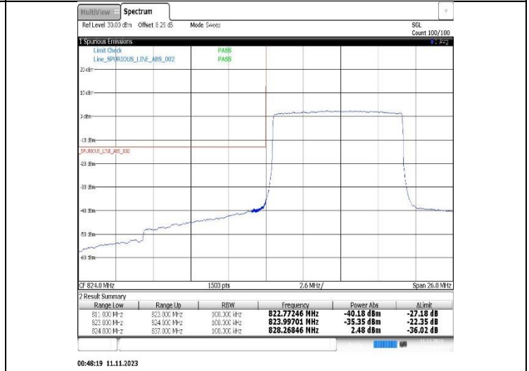
Band5-10MHz-QPSK-20450-50RB#0
