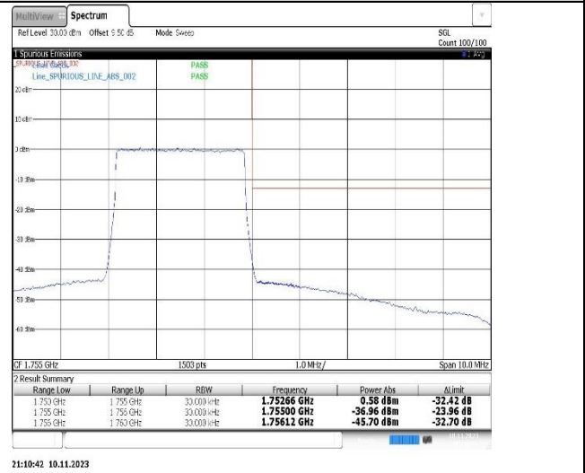
Band4-3MHz-16QAM-19965-15RB#0
