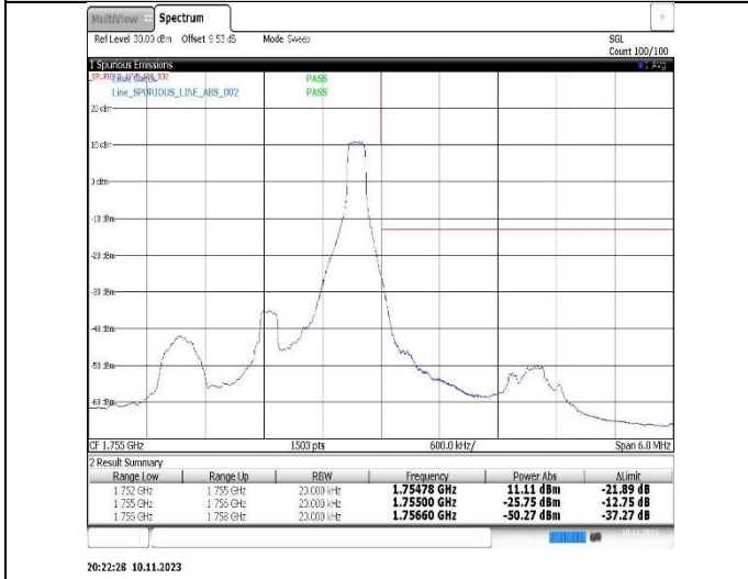
Band4-1.4MHz-QPSK-20393-6RB#0
