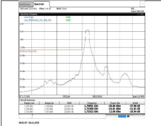
Band4-1.4MHz-QPSK-20393-1RB#5
