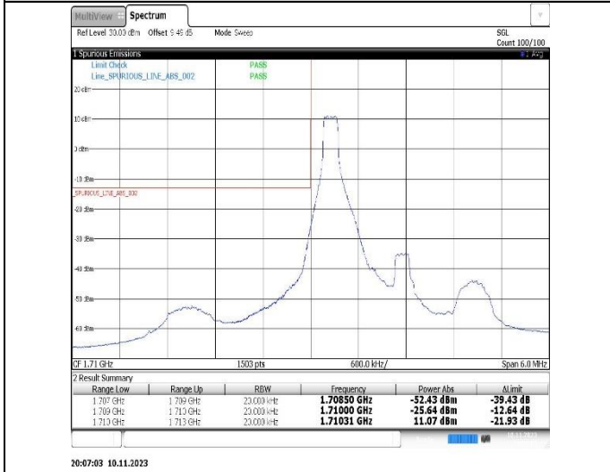
Band4-1.4MHz-16QAM-19957-6RB#0
