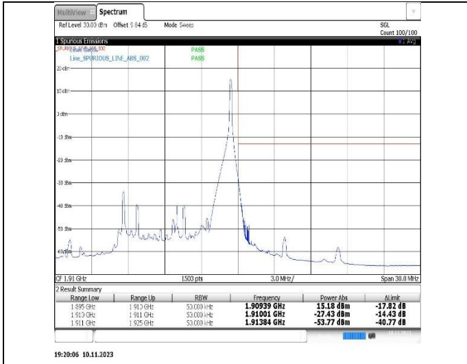
Band2-15MHz-QPSK-18675-1RB#0
