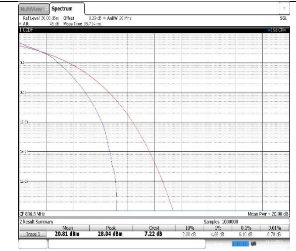
Band26(824-849)-15MHz-16QAM-26915-75RB#0
