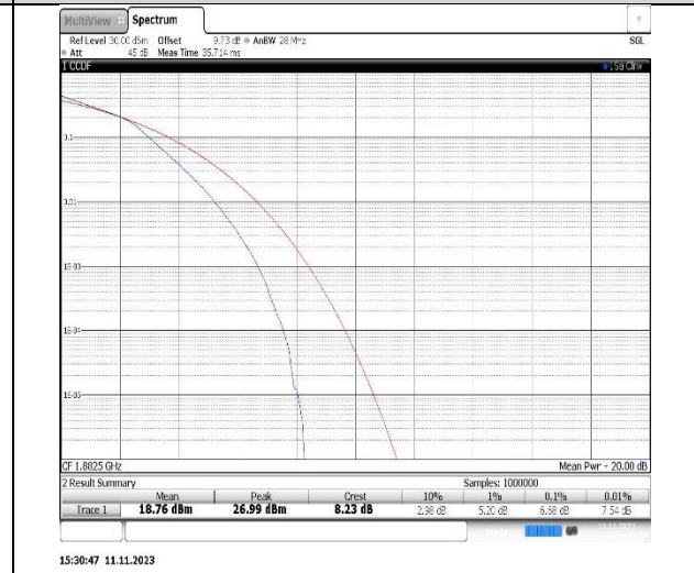
Band25-5MHz-16QAM-26365-25RB#0
