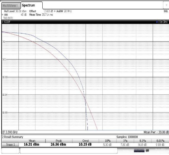
Band41-5MHz-QPSK-40620-25RB#0
