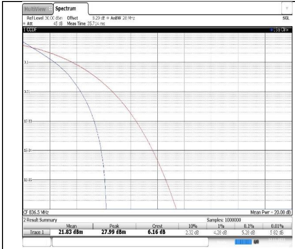
Band26(824-849)-15MHz-QPSK-26915-75RB#0
