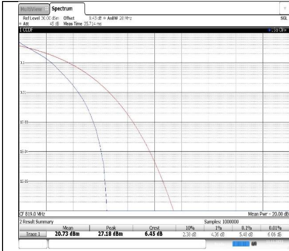
Band26(814-824)-10MHz-QPSK-26740-50RB#0
