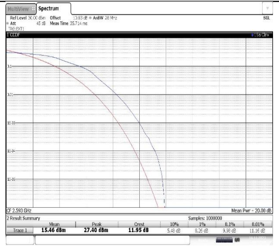
Band41-5MHz-16QAM-40620-25RB#0
