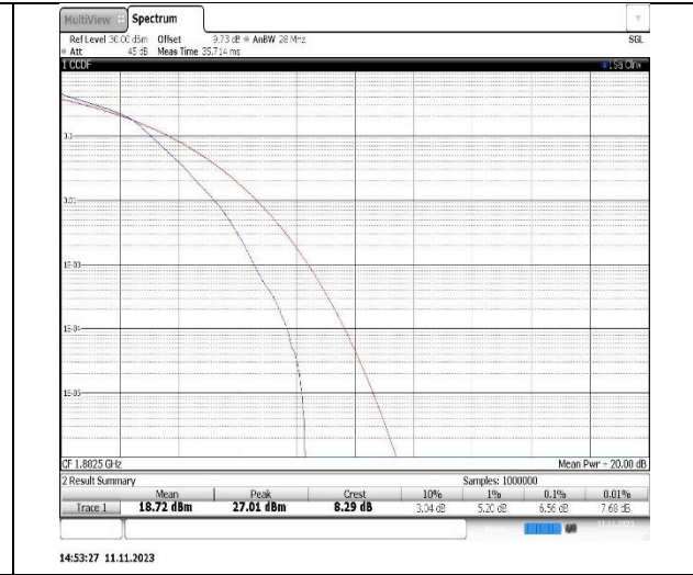
Band25-3MHz-16QAM-26365-15RB#0
