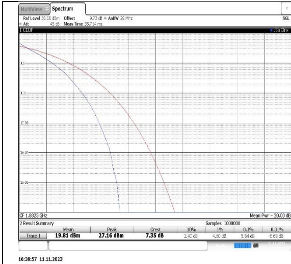
Band25-15MHz-QPSK-26365-75RB#0
