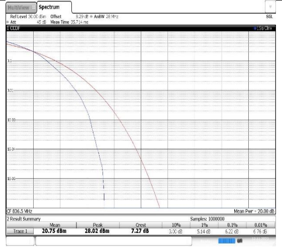
Band26(824-849)-15MHz-16QAM-26915-75RB#0
