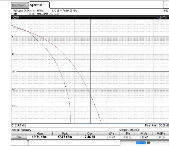
Band26(814-824)-10MHz-16QAM-26740-50RB#0
