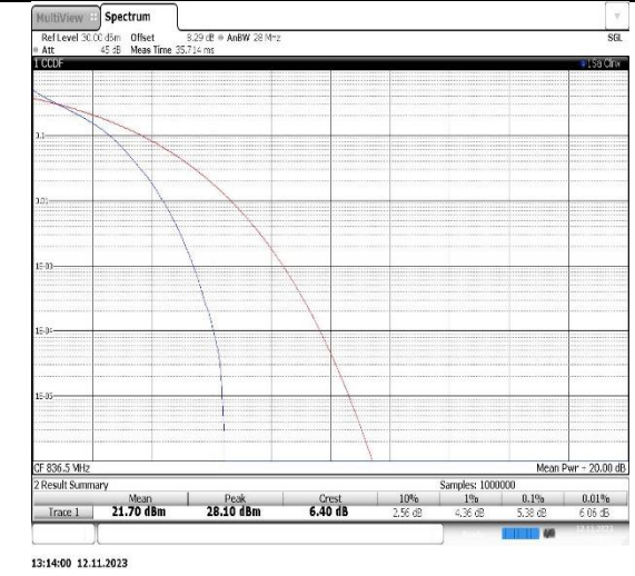
Band26(824-849)-1.4MHz-QPSK-26915-6RB#0
