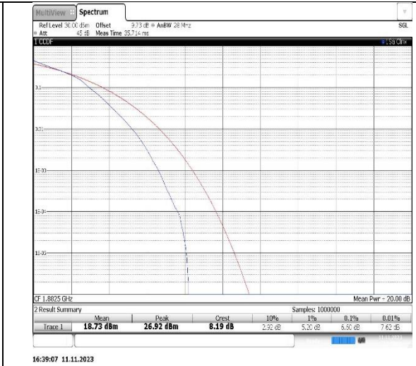
Band25-15MHz-16QAM-26365-75RB#0
