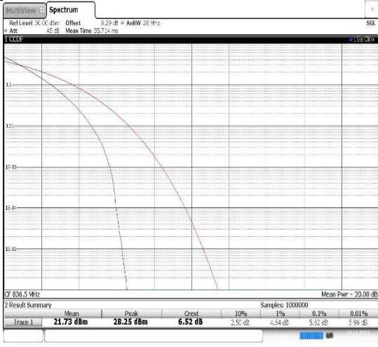
Band26(824-849)-15MHz-QPSK-26915-75RB#0
