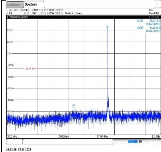
Band71-10MHz-QPSK-133297-1RB#0-Range1:30~1000MHz
