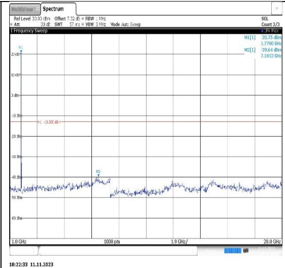
Band66-3MHz-16QAM-131987-1RB#0- Range2:1000~20000MHz
