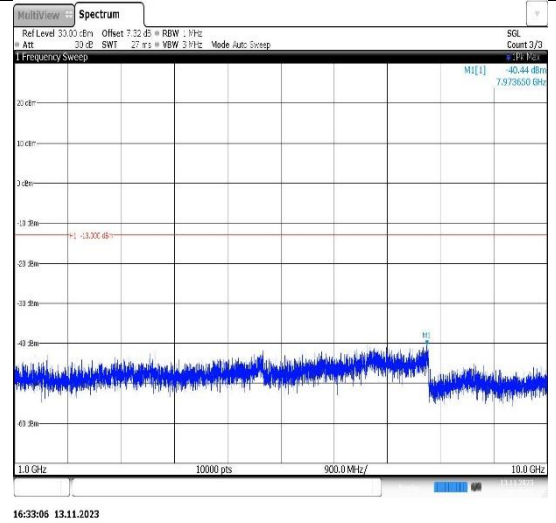
Band71-10MHz-QPSK-133422-1RB#0-Range2:1000~10000MHz
