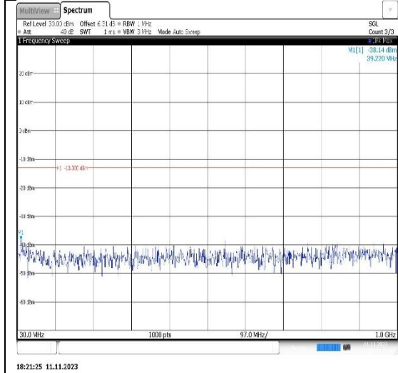
Band66-3MHz-16QAM-132322-1RB#0- Range1:30~1000MHz
