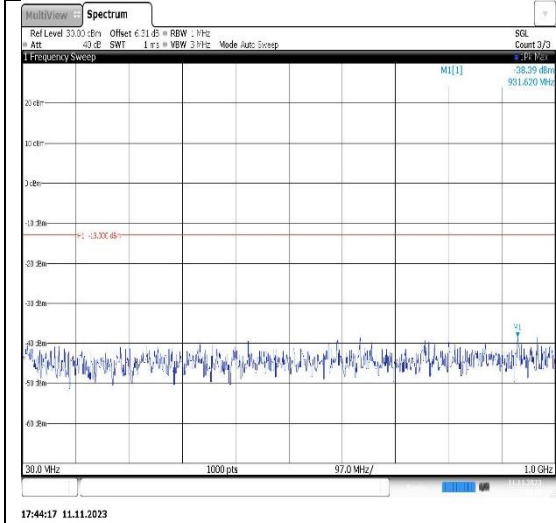
Band66-1.4MHz-QPSK-132665-1RB#0- Range1:30~1000MHz
