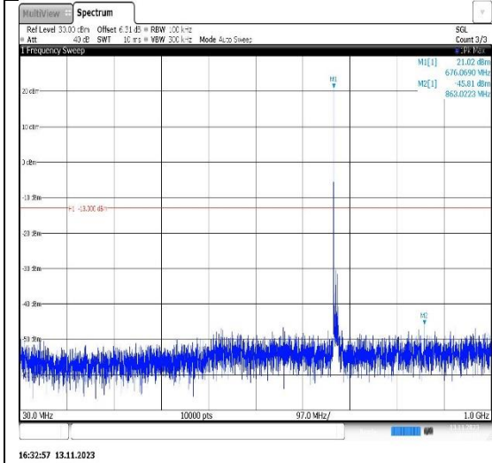
Band71-10MHz-QPSK-133422-1RB#0-Range1:30~1000MHz
