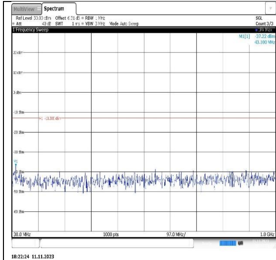
Band66-3MHz-16QAM-131987-1RB#0- Range1:30~1000MHz
