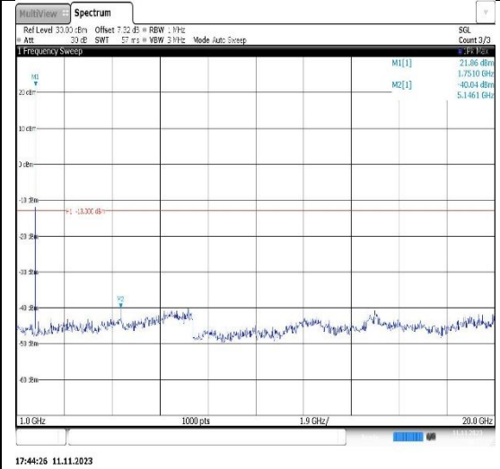
Band66-1.4MHz-QPSK-132665-1RB#0- Range2:1000~20000MHz
