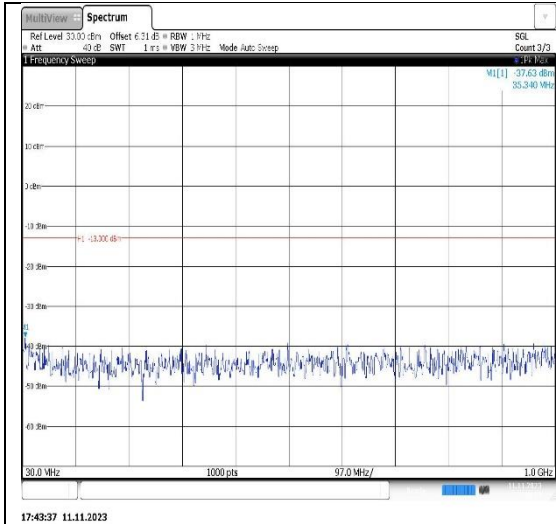
Band66-1.4MHz-QPSK-132322-1RB#0- Range1:30~1000MHz
