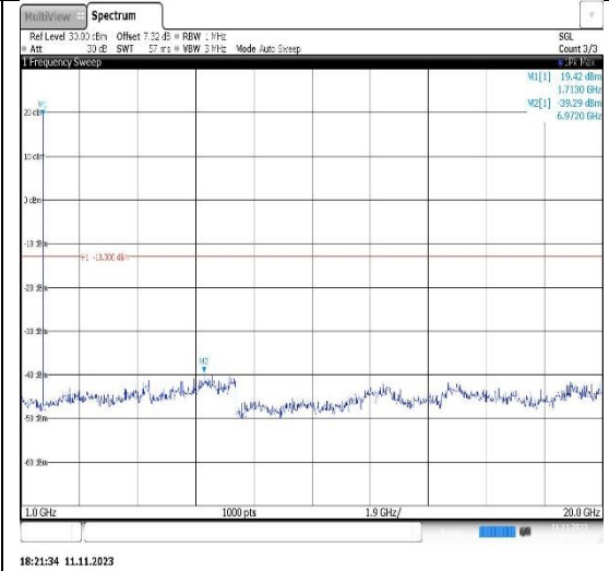
Band66-3MHz-16QAM-132322-1RB#0- Range2:1000~20000MHz
