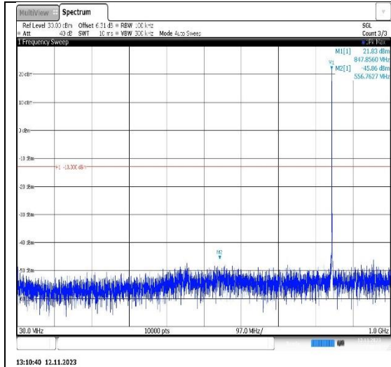
Band26(824-849)-1.4MHz-16QAM-26797-1RB#0-Range1:30~1000MHz
