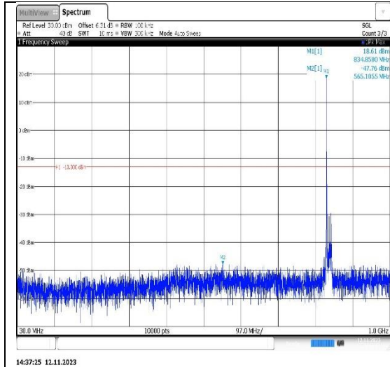
Band26(824-849)-15MHz-16QAM-26865-1RB#0-Range1:30~1000MHz
