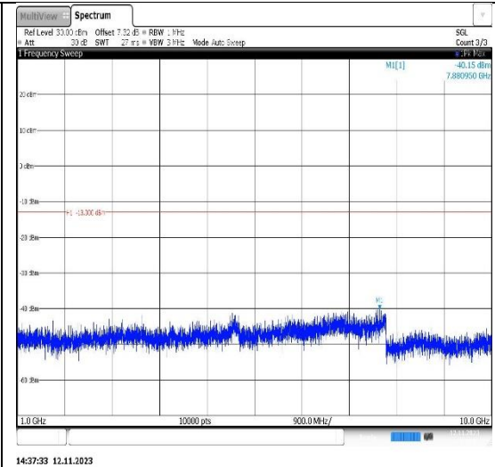
Band26(824-849)-15MHz-16QAM-26865-1RB#0-Range2:1000~10000MHz
