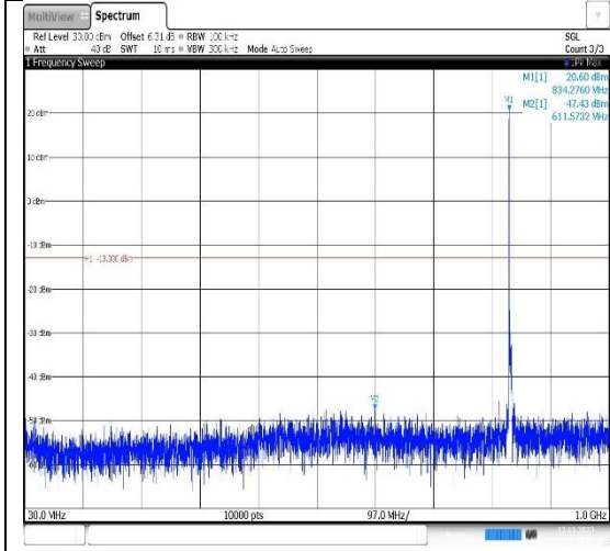
Band26(824-849)-5MHz-QPSK-26915-1RB#0-Range1:30~1000MHz
