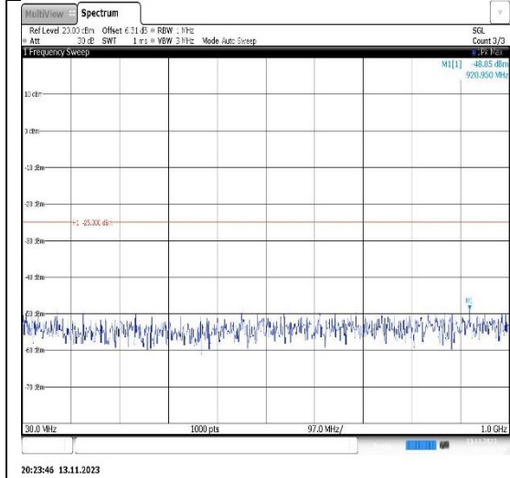
Band41-5MHz-QPSK-41565-1RB#0- Range1:30~1000MHz
