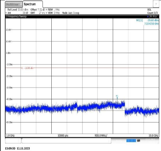
Band26(824-849)-1.4MHz-16QAM-26915-1RB#0-Range2:1000~10000MHz
