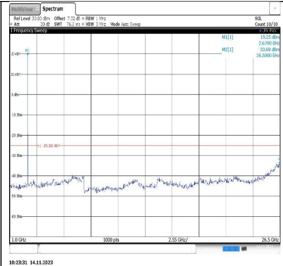
Band41-15MHz-16QAM-39725-1RB#0-Range2:1000~26500MHz
