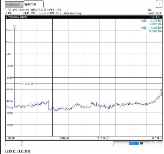
Band41-20MHz-16QAM-40620-1RB#0-Range2:1000~26500MHz
