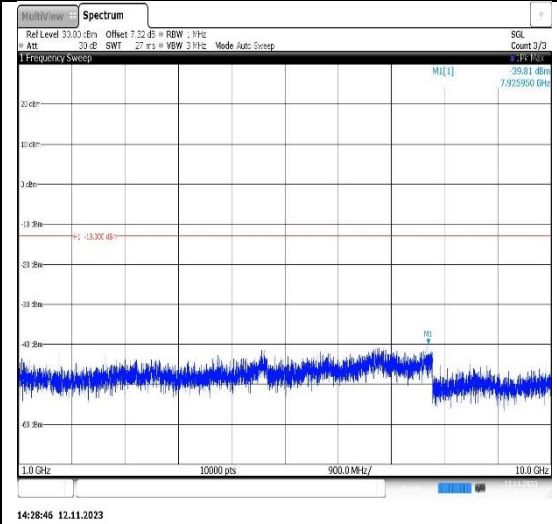
Band26(824-849)-10MHz-16QAM-26840-1RB#0-Range2:1000~10000MHz
