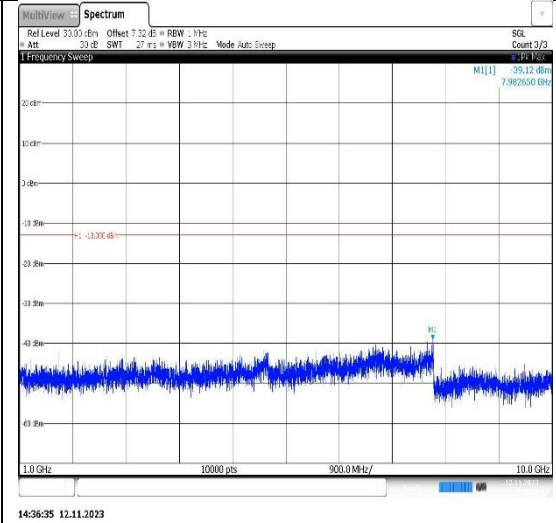
Band26(824-849)-15MHz-16QAM-26915-1RB#0-Range2:1000~10000MHz
