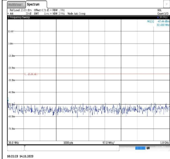
Band41-15MHz-16QAM-40620-1RB#0-Range1:30~1000MHz
