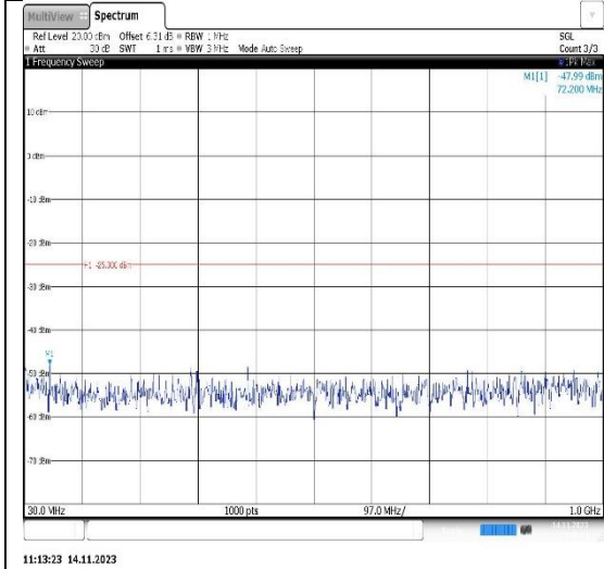
Band41-20MHz-16QAM-40620-1RB#0-Range1:30~1000MHz
