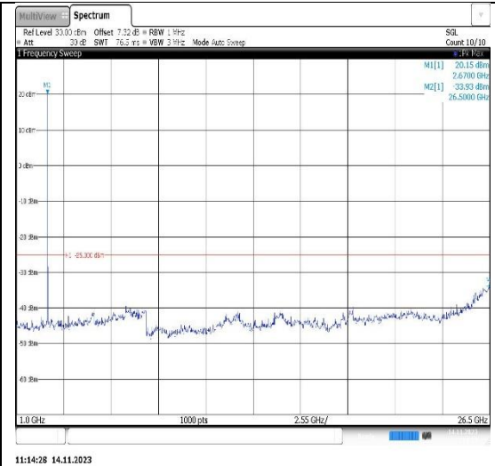
Band41-20MHz-16QAM-39750-1RB#0-Range2:1000~26500MHz
