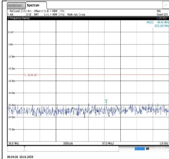
Band41-5MHz-16QAM-39675-1RB#0- Range1:30~1000MHz
