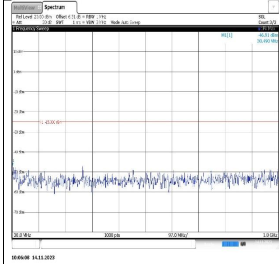
Band41-10MHz-16QAM-40620-1RB#0-Range1:30~1000MHz
