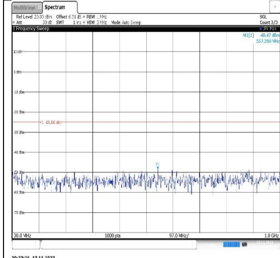
Band41-5MHz-16QAM-40620-1RB#0- Range1:30~1000MHz
