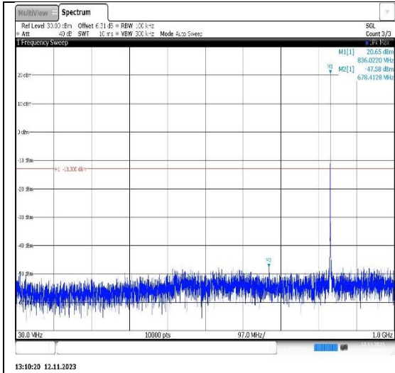
Band26(824-849)-1.4MHz-16QAM-27033-1RB#0-Range1:30~1000MHz
