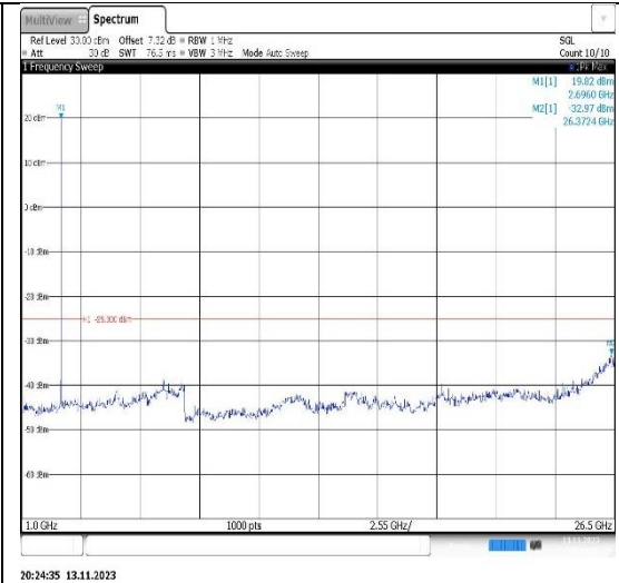
Band41-5MHz-16QAM-39675-1RB#0- Range2:1000~26500MHz
