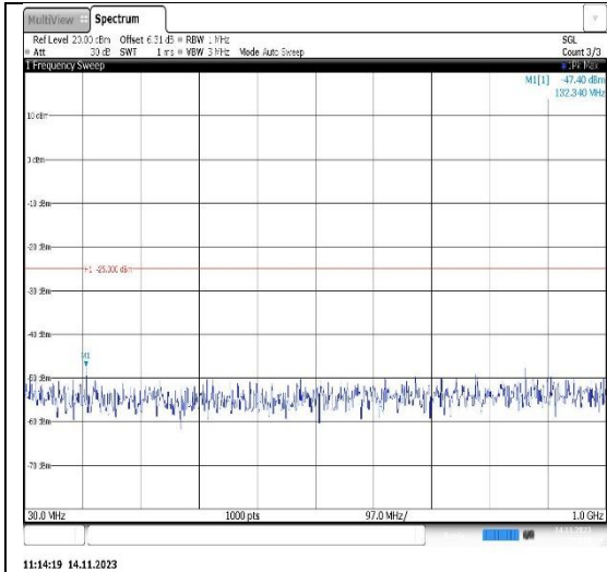
Band41-20MHz-16QAM-39750-1RB#0-Range1:30~1000MHz
