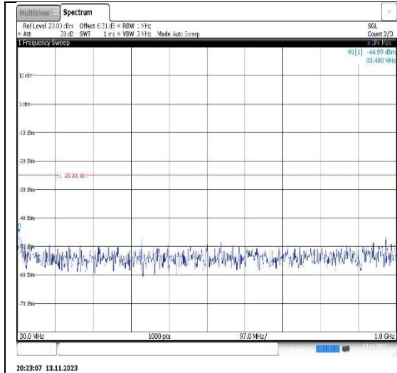
Band41-5MHz-QPSK-40620-1RB#0- Range1:30~1000MHz
