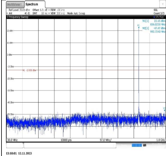
Band26(824-849)-1.4MHz-QPSK-27033-1RB#0-Range1:30~1000MHz
