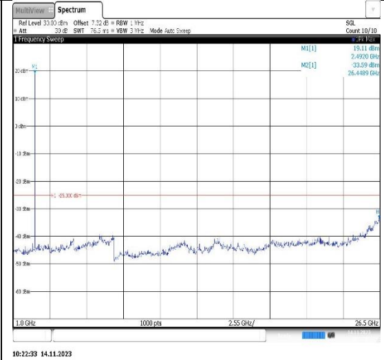
Band41-15MHz-16QAM-40620-1RB#0-Range2:1000~26500MHz
