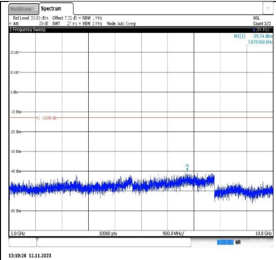
Band26(824-849)-1.4MHz-16QAM-27033-1RB#0-Range2:1000~10000MHz
