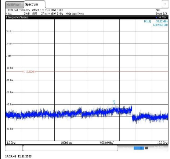
Band26(824-849)-10MHz-16QAM-26915-1RB#0-Range2:1000~10000MHz
