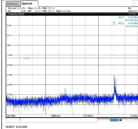
Band26(824-849)-15MHz-16QAM-26915-1RB#0-Range1:30~1000MHz
