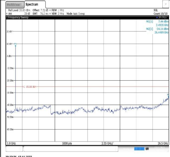
Band41-5MHz-16QAM-40620-1RB#0- Range2:1000~26500MHz
