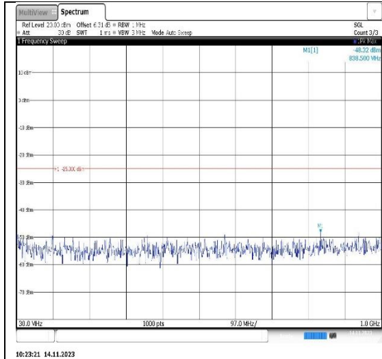
Band41-15MHz-16QAM-39725-1RB#0-Range1:30~1000MHz
