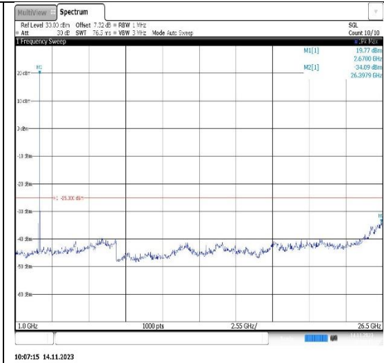
Band41-10MHz-16QAM-39700-1RB#0-Range2:1000~26500MHz
