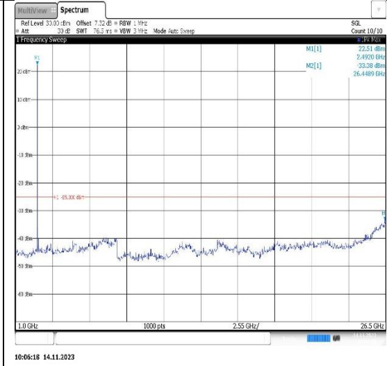
Band41-10MHz-16QAM-40620-1RB#0-Range2:1000~26500MHz
