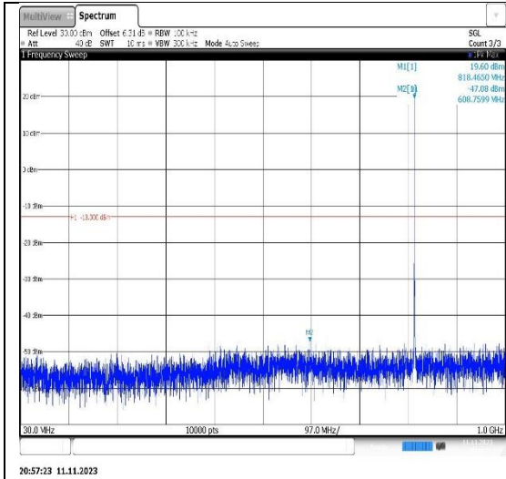
Band26(814-824)-1.4MHz-16QAM-26783-1RB#0-Range1:30~1000MHz
