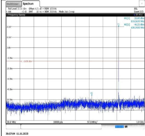
Band26(814-824)-1.4MHz-QPSK-26783-1RB#0-Range1:30~1000MHz
