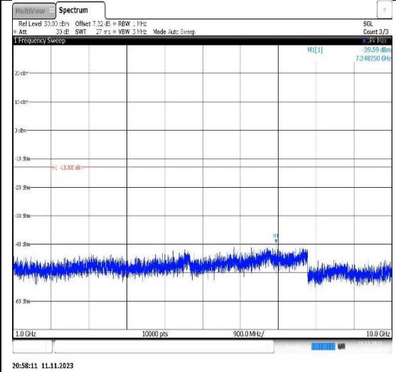
Band26(814-824)-3MHz-QPSK-26705-1RB#0-Range2:1000~10000MHz
