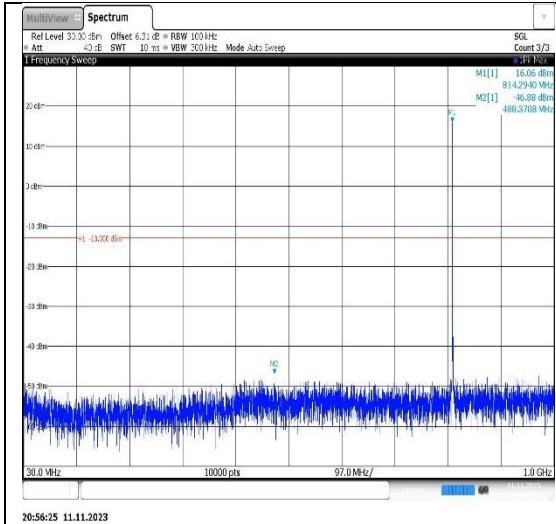
Band26(814-824)-1.4MHz-QPSK-26740-1RB#0-Range1:30~1000MHz
