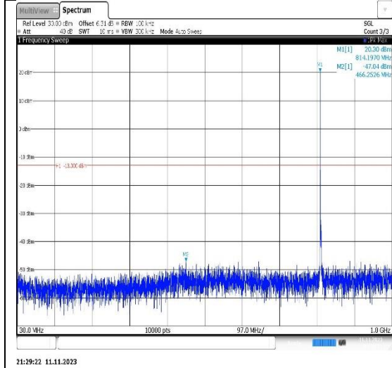
Band26(814-824)-3MHz-16QAM-26740-1RB#0-Range1:30~1000MHz
