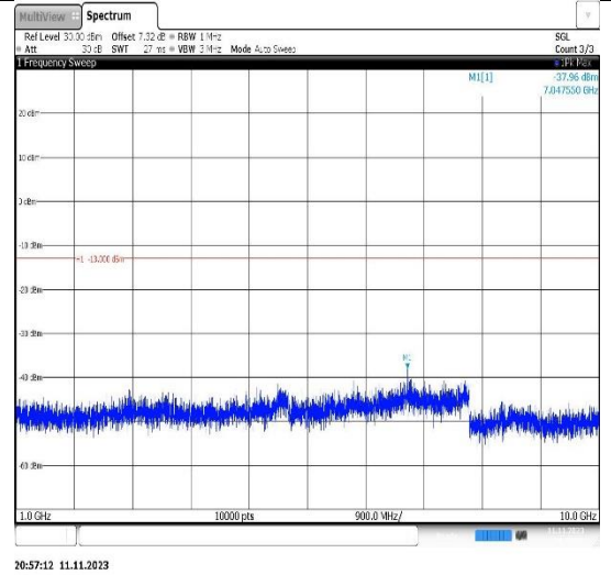
Band26(814-824)-1.4MHz-QPSK-26783-1RB#0-Range2:1000~10000MHz
