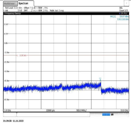
Band26(814-824)-3MHz-16QAM-26740-1RB#0-Range2:1000~10000MHz
