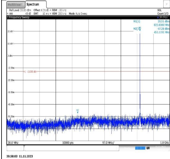
Band26(814-824)-3MHz-QPSK-26705-1RB#0-Range1:30~1000MHz
