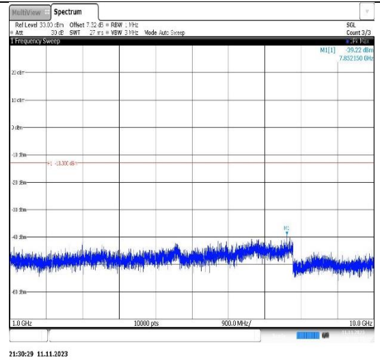
Band26(814-824)-3MHz-16QAM-26705-1RB#0-Range2:1000~10000MHz
