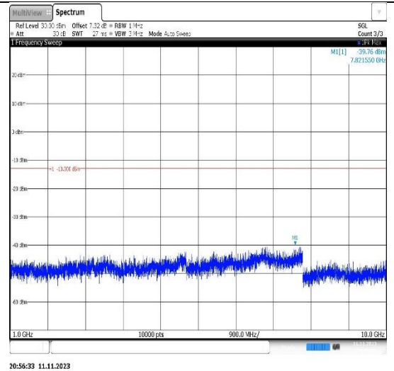
Band26(814-824)-1.4MHz-QPSK-26740-1RB#0-Range2:1000~10000MHz
