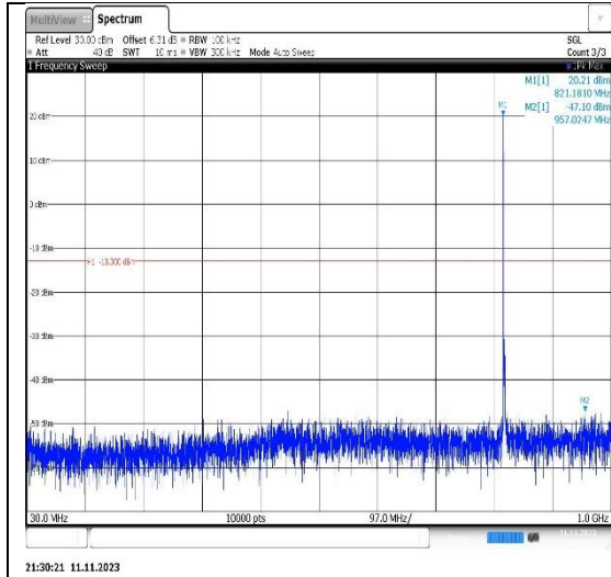
Band26(814-824)-3MHz-16QAM-26705-1RB#0-Range1:30~1000MHz
