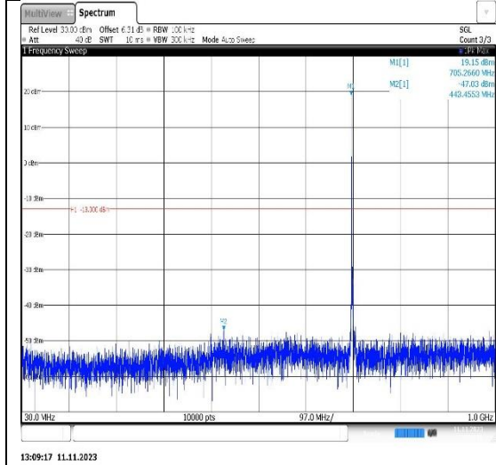
Band12-5MHz-QPSK-23155-1RB#0- Range1:30~1000MHz
