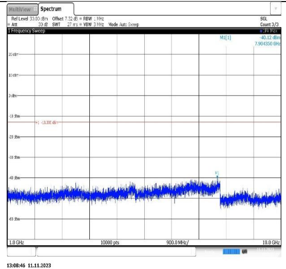
Band12-5MHz-QPSK-23095-1RB#0- Range2:1000~10000MHz
