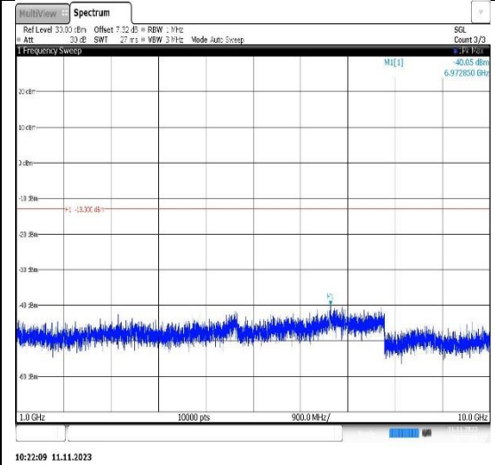
Band12-3MHz-QPSK-23165-1RB#0- Range2:1000~10000MHz
