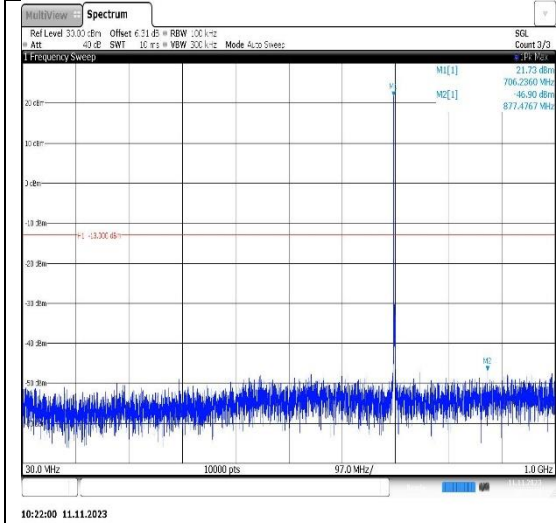
Band12-3MHz-QPSK-23165-1RB#0- Range1:30~1000MHz
