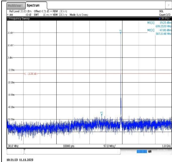
Band12-3MHz-QPSK-23095-1RB#0- Range1:30~1000MHz
