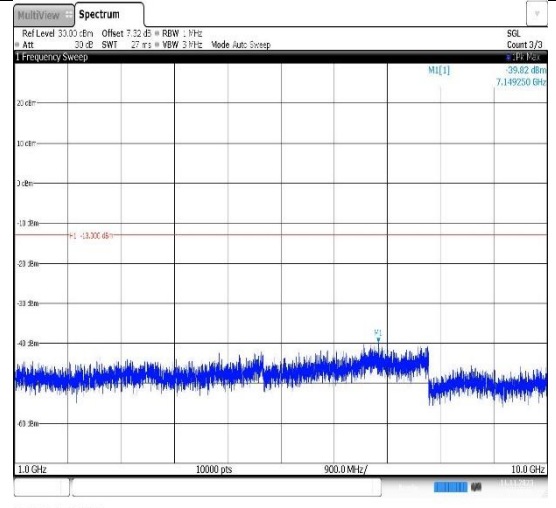
09:58:07 11.11.2023 Band12-1.4MHz-QPSK-23173-1RB#0-Range2:1000~10000MHz
