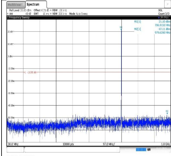
09:57:59 11.11.2023 Band12-1.4MHz-QPSK-23173-1RB#0-Range1:30~1000MHz
