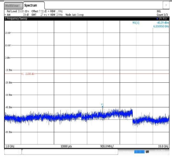
09:57:28 11.11.2023 Band12-1.4MHz-QPSK-23095-1RB#0-Range2:1000~10000MHz
