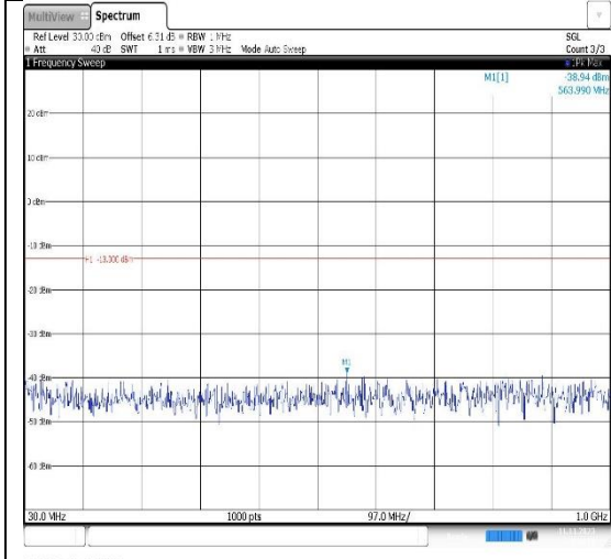
Band25-1.4MHz-QPSK-26683-1RB#0-Range1:30~1000MHz
