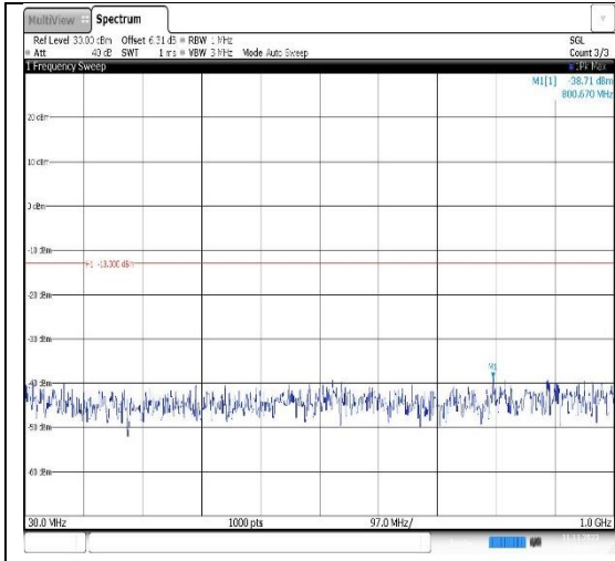
Band25-1.4MHz-QPSK-26365-1RB#0-Range1:30~1000MHz
