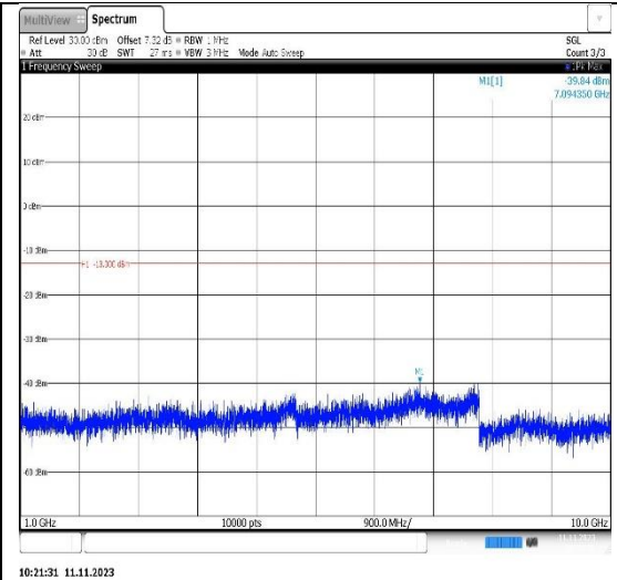
Band12-3MHz-QPSK-23095-1RB#0- Range2:1000~10000MHz
