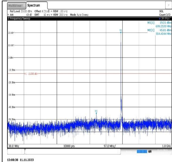
Band12-5MHz-QPSK-23095-1RB#0- Range1:30~1000MHz
