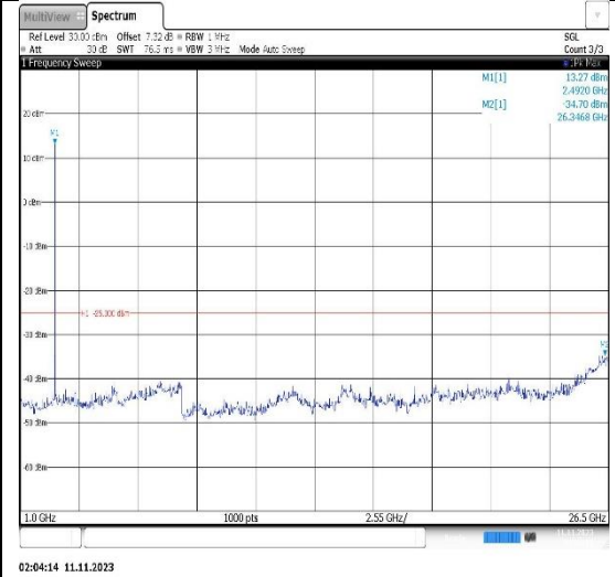
Band7-15MHz-16QAM-21100-1RB#0- Range2:1000~26500MHz
