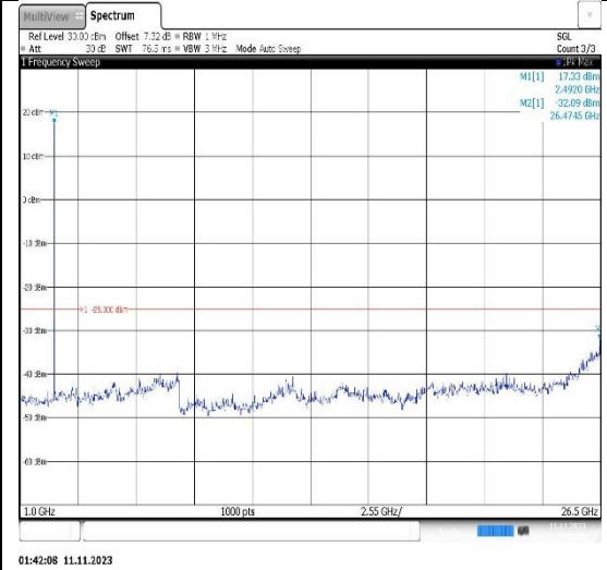
Band7-10MHz-16QAM-21100-1RB#0- Range2:1000~26500MHz
