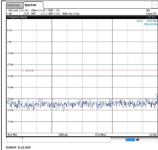
Band7-15MHz-QPSK-21100-1RB#0- Range1:30~1000MHz
