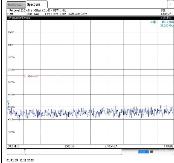
Band7-10MHz-16QAM-21100-1RB#0- Range1:30~1000MHz
