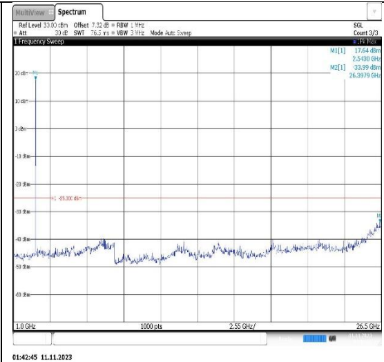
Band7-10MHz-16QAM-21400-1RB#0- Range2:1000~26500MHz
