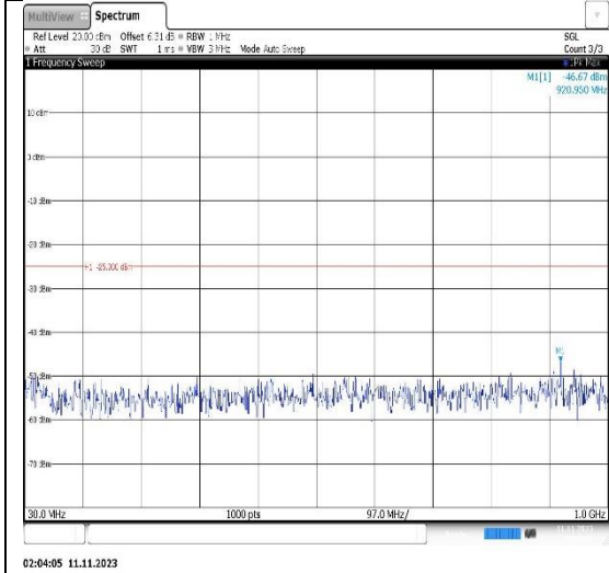
Band7-15MHz-16QAM-21100-1RB#0- Range1:30~1000MHz
