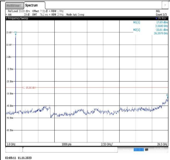
Band7-15MHz-16QAM-20825-1RB#0- Range2:1000~26500MHz
