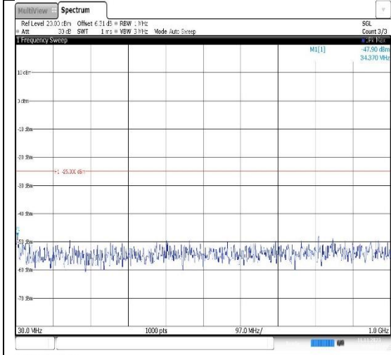
Band7-15MHz-QPSK-21375-1RB#0- Range1:30~1000MHz
