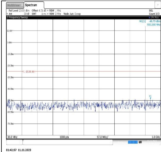
Band7-10MHz-16QAM-20800-1RB#0- Range1:30~1000MHz
