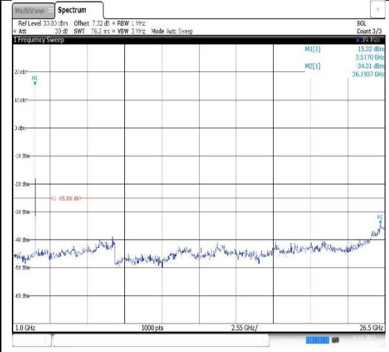
Band7-15MHz-QPSK-21375-1RB#0- Range2:1000~26500MHz
