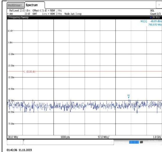
Band7-10MHz-16QAM-21400-1RB#0- Range1:30~1000MHz
