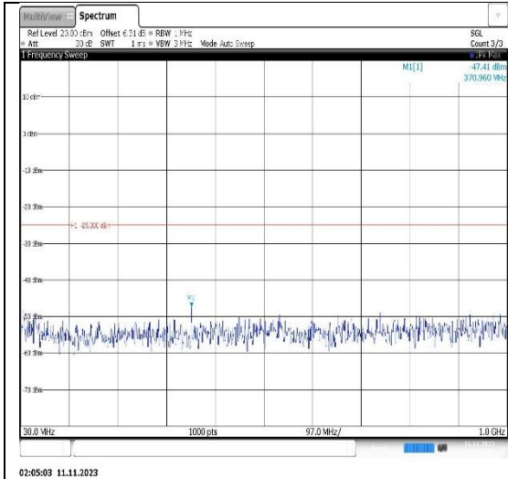
Band7-15MHz-16QAM-20825-1RB#0- Range1:30~1000MHz
