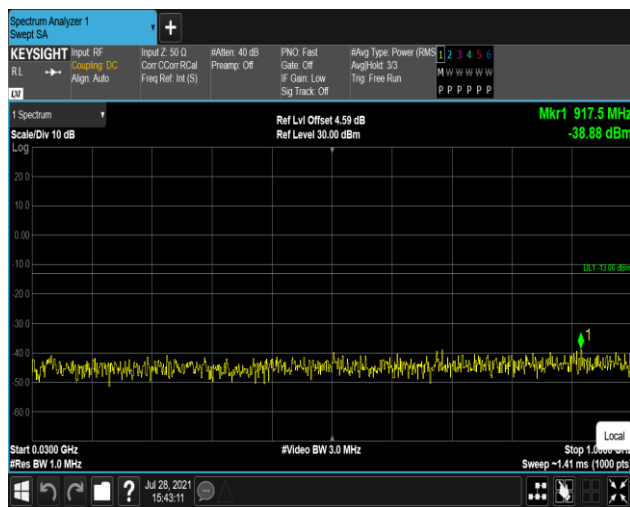
Band25-1.4MHz-16QAM-26365:30~1000MHz
