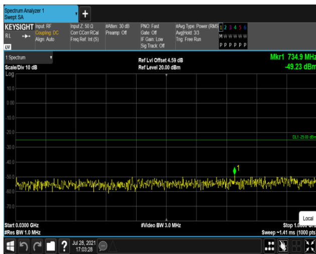
Band41-5MHz-16QAM-40065:30~1000MHz
