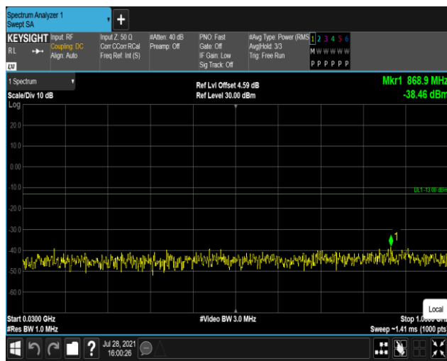
Band25-20MHz-16QAM-26365:30~1000MHz
