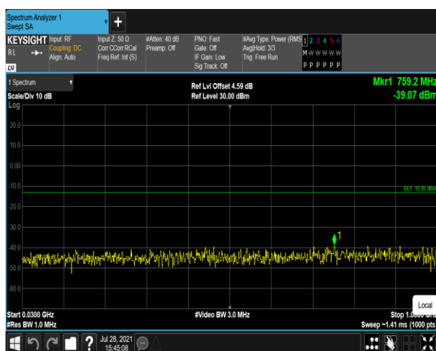
Band25-1.4MHz-16QAM-26683:30~1000MHz
