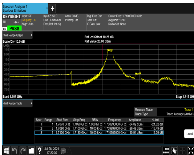
Band66-1.4MHz-16QAM-131979-6RB#0
