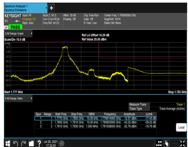
Band66-1.4MHz-QPSK-132665-6RB#0
