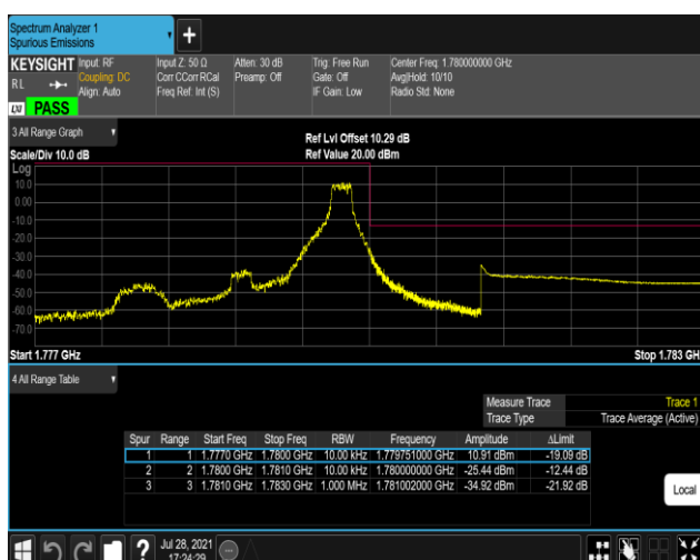
Band66-1.4MHz-16QAM-132665-1RB#5
