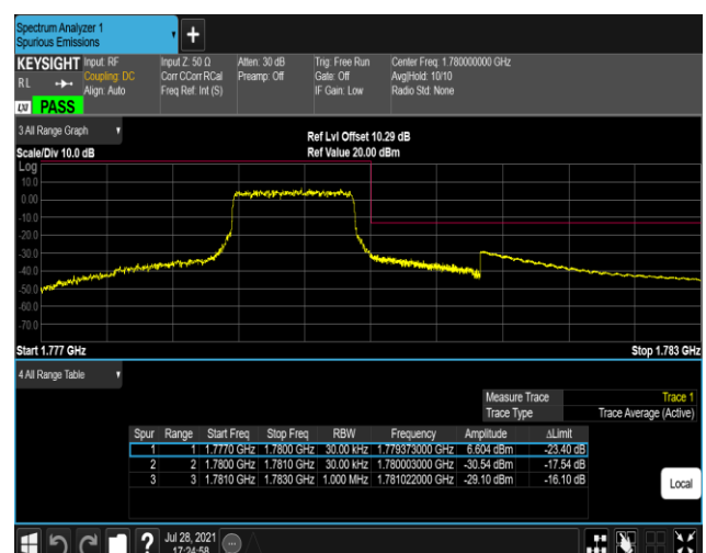
Band66-1.4MHz-16QAM-132665-6RB#0
