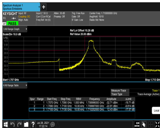
Band66-1.4MHz-QPSK-131979-6RB#0
