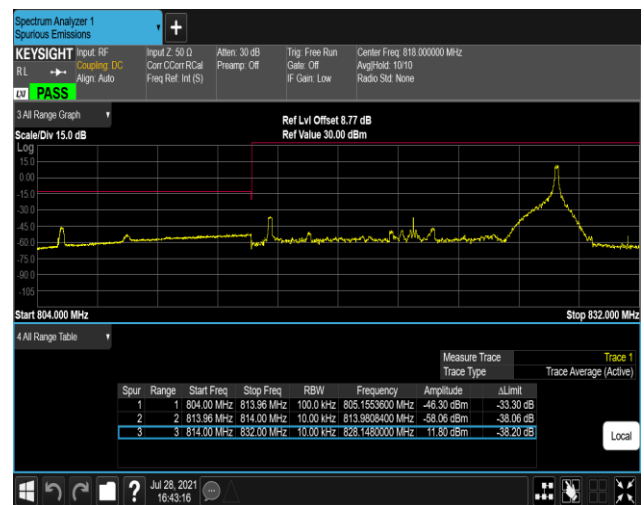
Band26-15MHz-QPSK-26865-1RB#0
