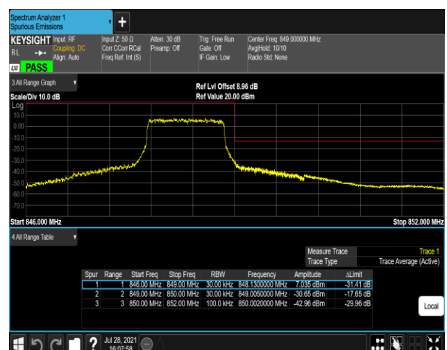
Band26-1.4MHz-QPSK-27033-6RB#0
