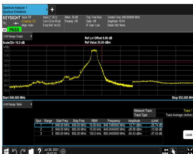
Band26-1.4MHz-QPSK-27033-1RB#5
