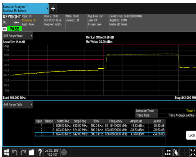
Band26-15MHz-16QAM-26965-1RB#74
