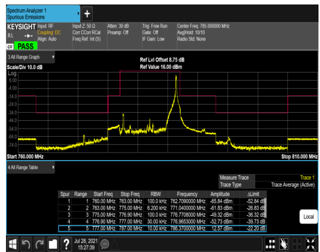
Band13-10MHz-16QAM-23230-1RB#0
