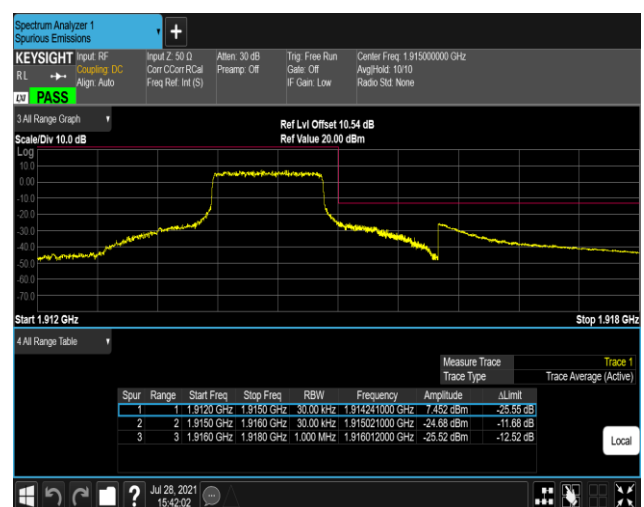
Band25-1.4MHz-QPSK-26683-6RB#0
