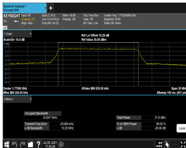
Band66-10MHz-16QAM-132322-50RB#0
