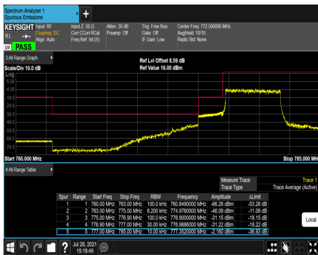
Band13-5MHz-16QAM-23255-1RB#24
