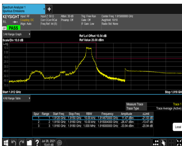
Band25-1.4MHz-16QAM-26683-1RB#5
