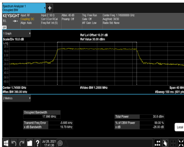
Band66-20MHz-16QAM-132322-100RB#0
