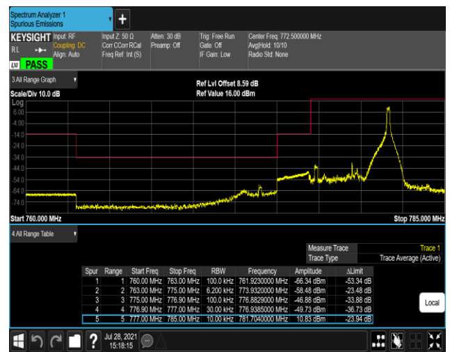
Band13-5MHz-16QAM-23255-1RB#0
