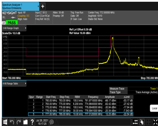
Band13-5MHz-QPSK-23205-25RB#0
