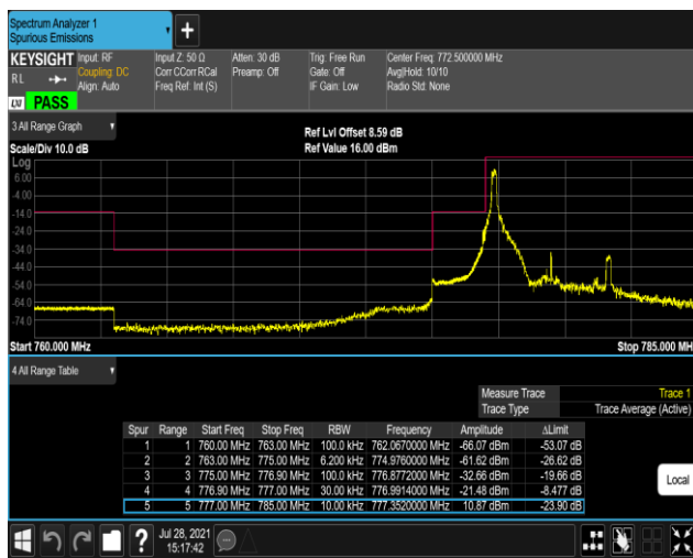
Band13-5MHz-16QAM-23205-25RB#0
