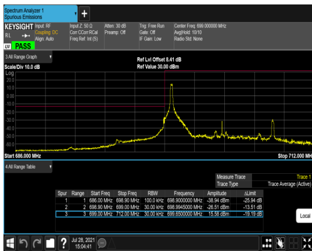
Band12-10MHz-QPSK-23060-50RB#0
