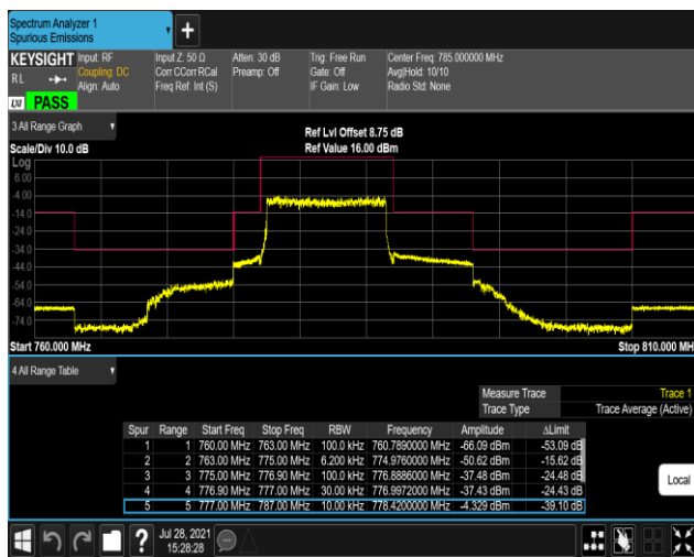
Band13-10MHz-16QAM-23230-1RB#49
