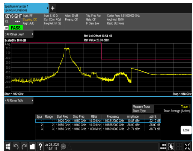
Band25-1.4MHz-16QAM-26683-6RB#0
