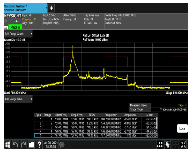
Band13-10MHz-16QAM-23230-50RB#0
