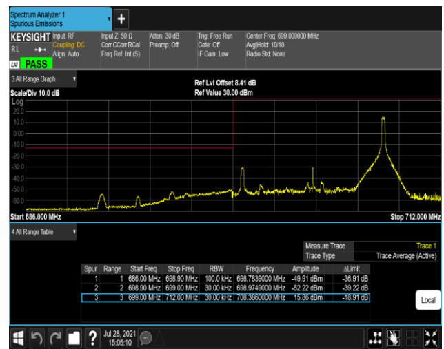
Band12-10MHz-QPSK-23130-1RB#0
