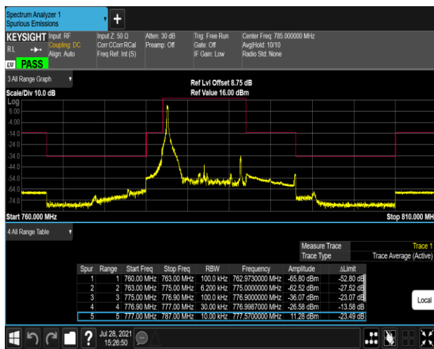
Band13-10MHz-QPSK-23230-50RB#0
