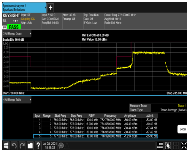
Band13-5MHz-QPSK-23255-1RB#24
