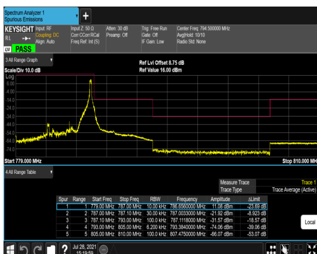
Band13-5MHz-16QAM-23255-1RB#24
