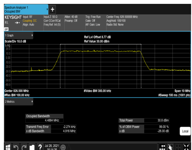
Band26-5MHz-16QAM-26815-25RB#0
