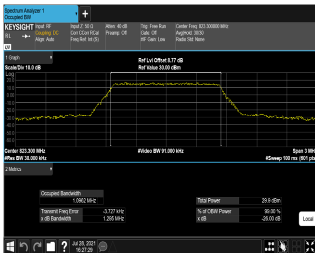
Band26-1.4MHz-16QAM-26783-6RB#0
