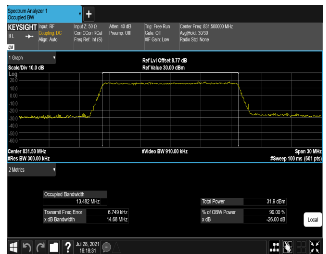
Band26-15MHz-QPSK-26865-75RB#0
