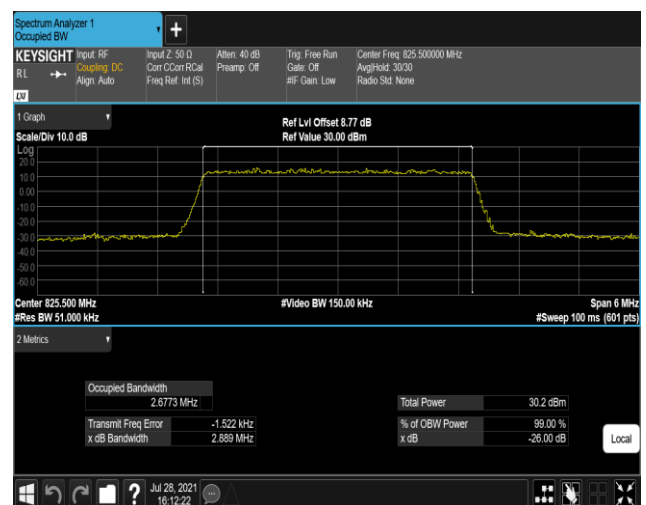
Band26-3MHz-16QAM-26805-15RB#0
