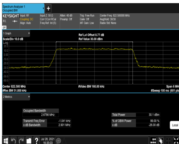
Band26-3MHz-16QAM-26775-15RB#0
