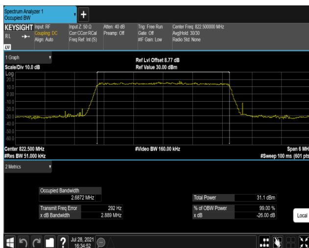
Band26-3MHz-QPSK-26775-15RB#0
