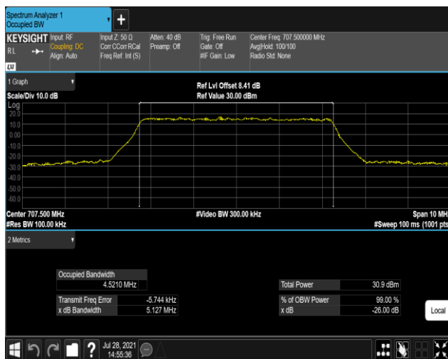
Band12-5MHz-16QAM-23095-25RB#0
