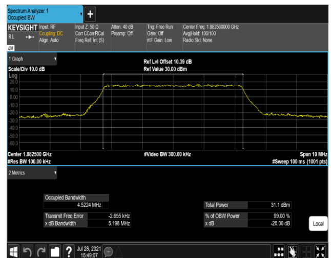
Band25-5MHz-16QAM-26065-25RB#0
