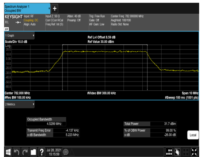
Band13-5MHz-16QAM-23205-25RB#0
