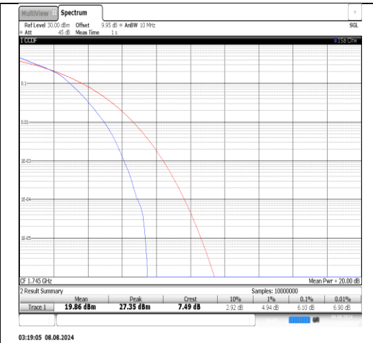
Band66-15MHz-16QAM-132322-75RB#0-PASS
