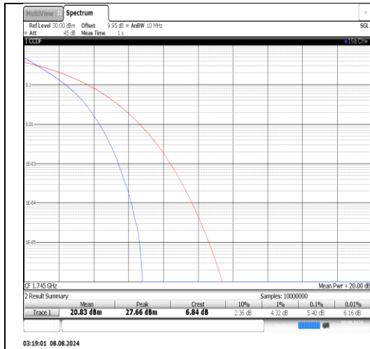
Band66-15MHz-QPSK-132322-75RB#0-PASS
