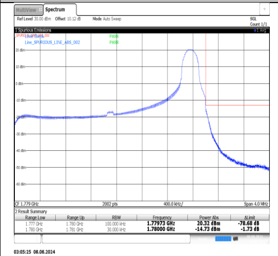
Band66-3MHz-16QAM-131987-15RB#0-PASS
