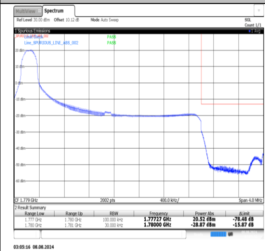
Band66-3MHz-16QAM-132657-1RB#14-PASS
