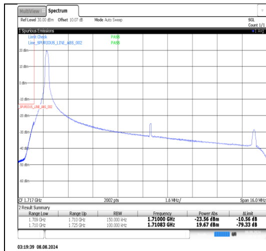
Band66-15MHz-QPSK-132047-1RB#74-PASS
