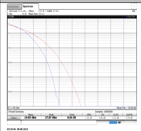
Band66-20MHz-16QAM-132322-100RB#0-PASS
