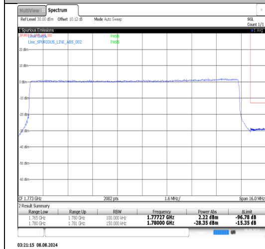
Band66-15MHz-QPSK-132597-75RB#0-PASS
