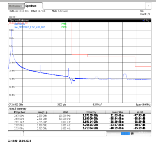
Band41-20MHz-16QAM-41490-1RB#0-PASS
