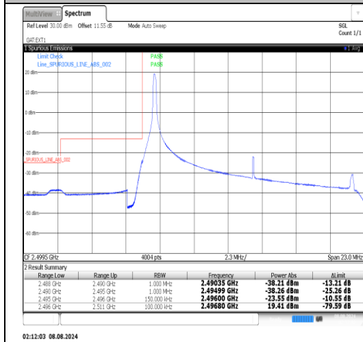
Band41-15MHz-16QAM-39725-1RB#74-PASS
