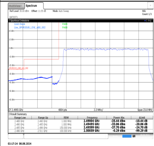
Band41-15MHz-16QAM-41515-1RB#0-PASS
