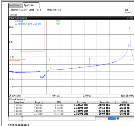
Band41-20MHz-16QAM-41490-100RB#0-PASS
