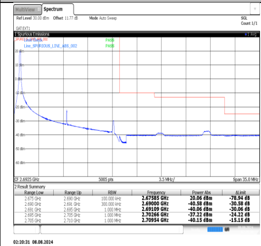
Band41-15MHz-16QAM-41515-1RB#74-PASS
