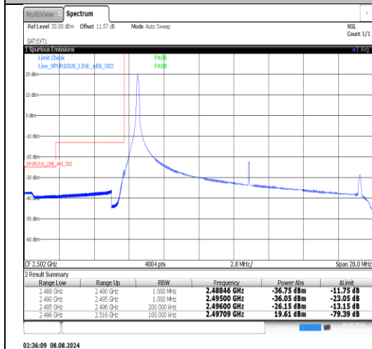
Band41-20MHz-16QAM-39750-1RB#99-PASS
