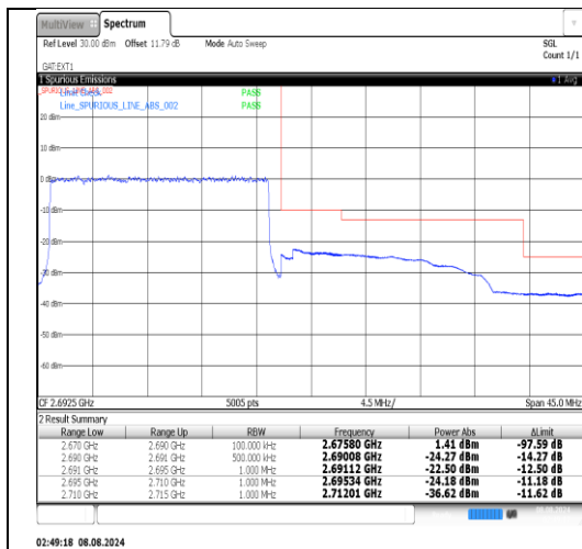
Band41-20MHz-16QAM-39750-1RB#0-PASS
