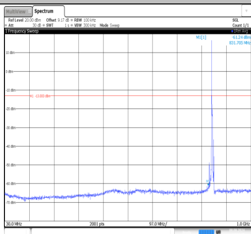
Band26(824-849)-5MHz-QPSK-27015-1RB#0-30~1000-PASS
