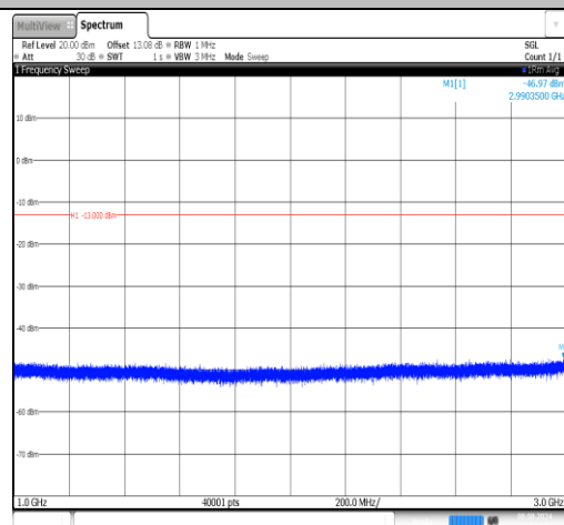
Band26(824-849)-5MHz-QPSK-27015-1RB#0-1000~3000-PASS
