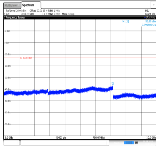
Band26(824-849)-15MHz-16QAM-26965-1RB#0- 3000~10000-PASS
