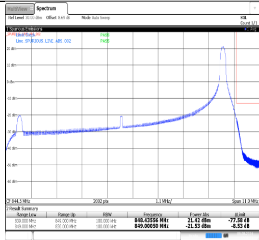
Band26(824-849)-10MHz-16QAM-26990-1RB#49-PASS
