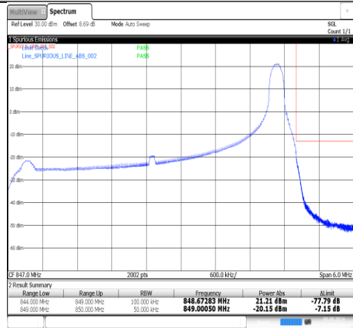
Band26(824-849)-5MHz-16QAM-27015-1RB#24-PASS
