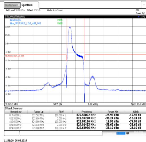
Band26(814-824)-1.4MHz-QPSK-26783-1RB#5-PASS
