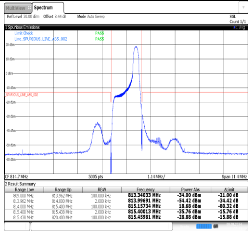
Band26(814-824)-1.4MHz-16QAM-26697-1RB#5-PASS
