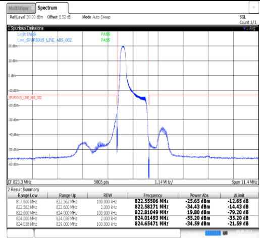
Band26(814-824)-1.4MHz-16QAM-26783-1RB#0-PASS
