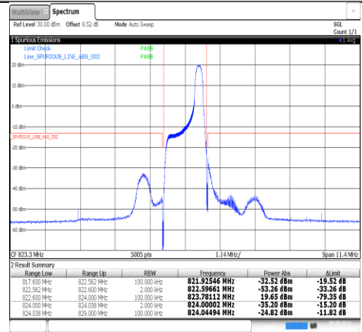
Band26(814-824)-1.4MHz-16QAM-26783-1RB#5-PASS
