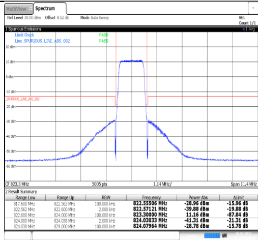
Band26(814-824)-1.4MHz-16QAM-26783-6RB#0-PASS
