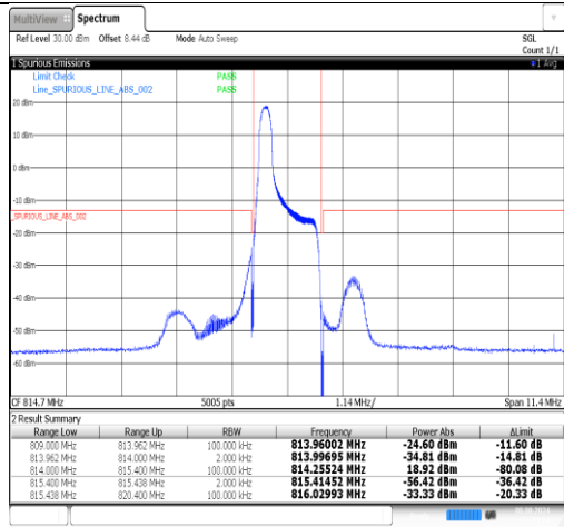
Band26(814-824)-1.4MHz-16QAM-26697-1RB#5-PASS
