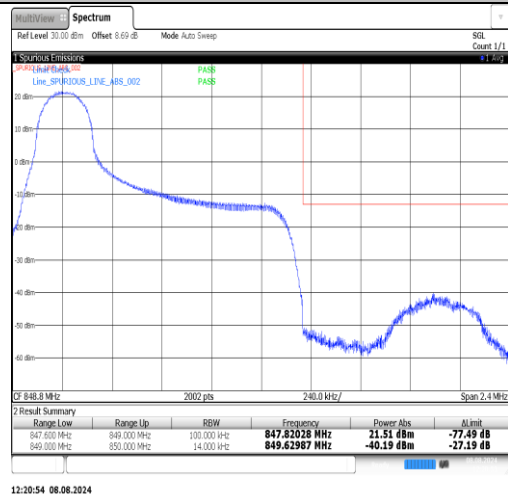
Band26(824-849)-1.4MHz-QPSK-27033-1RB#5-PASS
