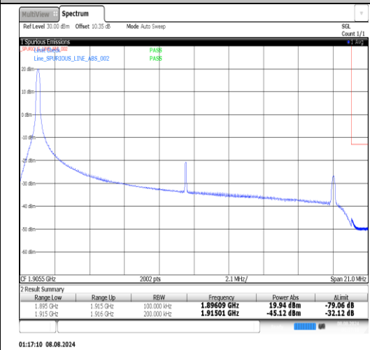
Band25-20MHz-16QAM-26590-1RB#0-PASS
