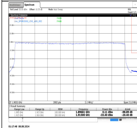
Band25-20MHz-16QAM-26590-100RB#0-PASS
