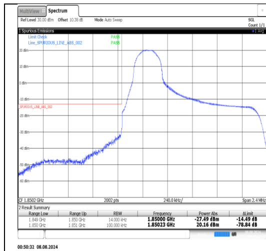
Band25-1.4MHz-QPSK-26047-1RB#5-PASS
