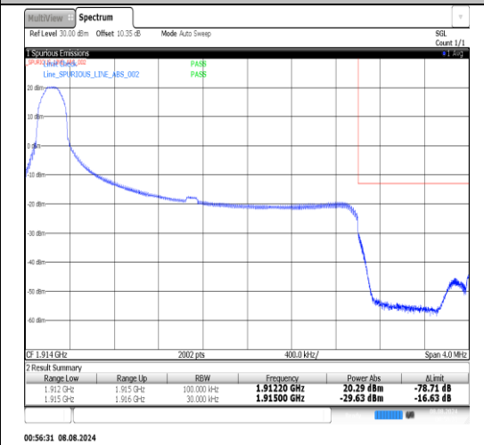
Band25-3MHz-QPSK-26675-1RB#14-PASS
