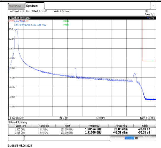
Band25-10MHz-16QAM-26640-1RB#49-PASS
