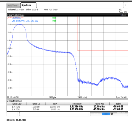
Band25-1.4MHz-16QAM-26683-1RB#5-PASS
