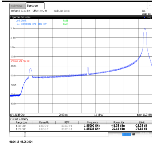
Band25-10MHz-16QAM-26640-50RB#0-PASS
