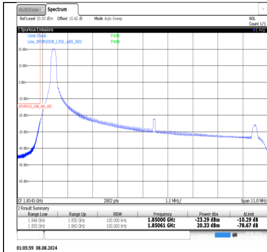
Band25-10MHz-16QAM-26090-1RB#49-PASS
