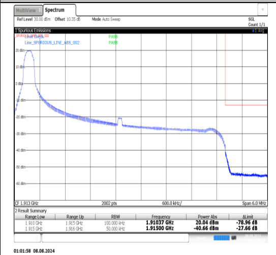
Band25-5MHz-16QAM-26665-1RB#24-PASS
