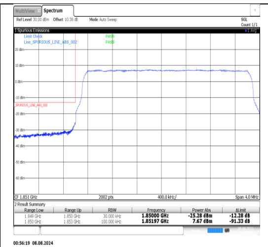
Band25-3MHz-16QAM-26675-1RB#0-PASS
