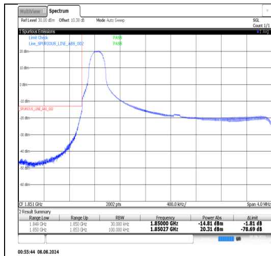
Band25-3MHz-16QAM-26055-1RB#14-PASS
