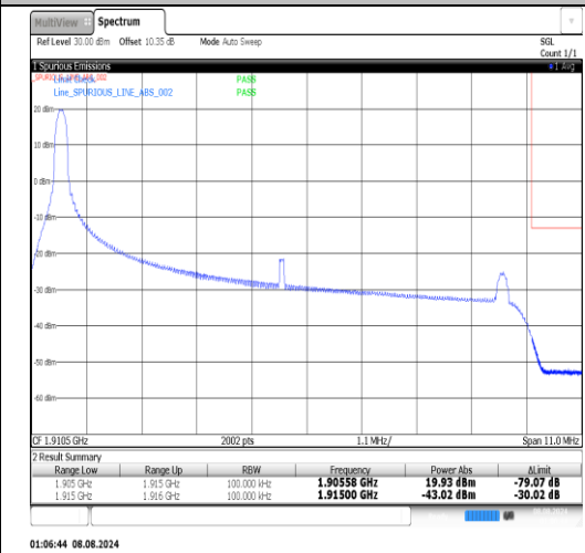
Band25-10MHz-QPSK-26640-1RB#49-PASS
