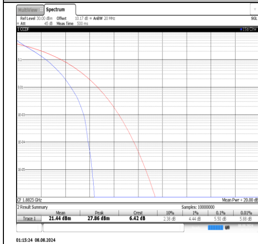
Band25-15MHz-QPSK-26365-75RB#0-PASS
