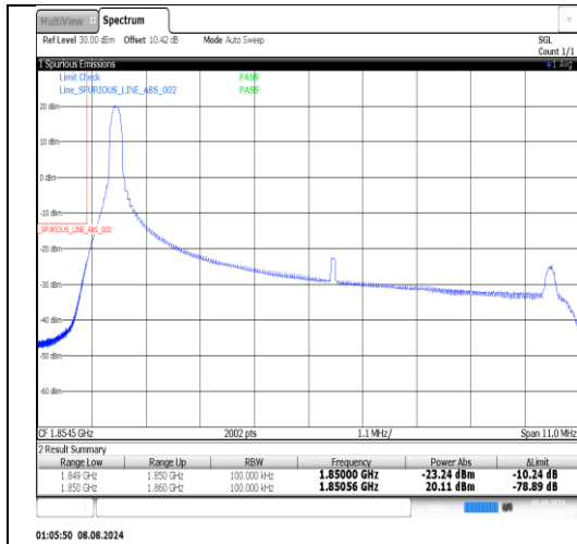
Band25-10MHz-QPSK-26090-1RB#49-PASS
