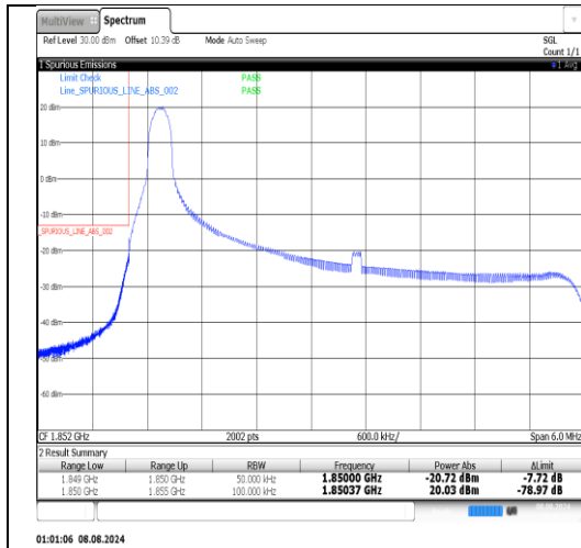
Band25-5MHz-16QAM-26065-1RB#24-PASS
