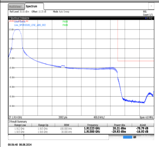
Band25-3MHz-16QAM-26675-1RB#14-PASS
