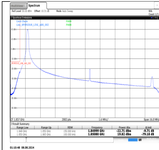
Band25-15MHz-QPSK-26115-1RB#74-PASS
