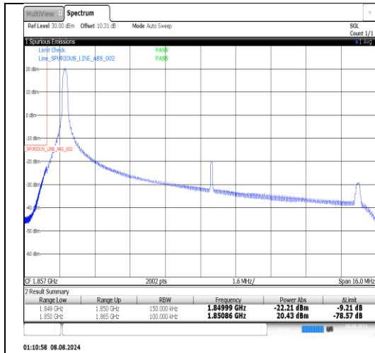
Band25-15MHz-16QAM-26115-1RB#74-PASS
