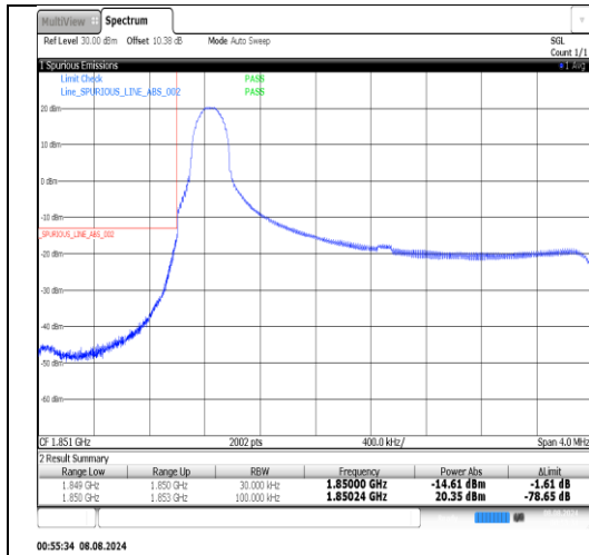
Band25-3MHz-QPSK-26055-1RB#14-PASS
