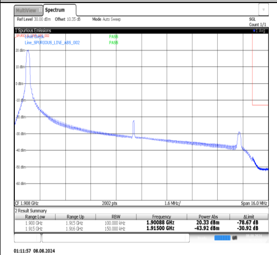
Band25-15MHz-16QAM-26615-1RB#74-PASS
