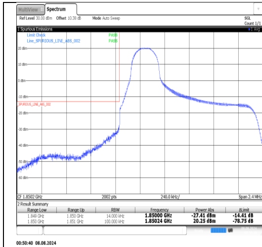
Band25-1.4MHz-16QAM-26047-1RB#5-PASS
