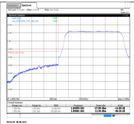
Band25-1.4MHz-QPSK-26683-1RB#0-PASS
