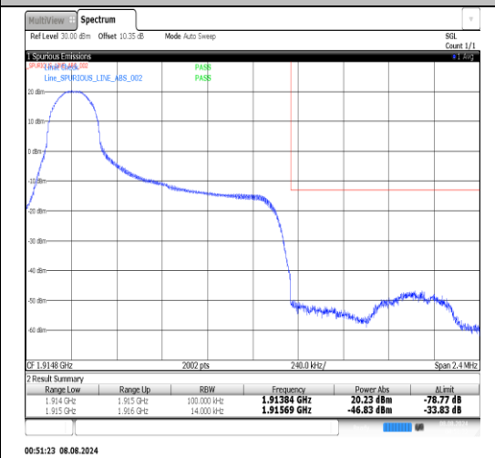
Band25-1.4MHz-QPSK-26683-1RB#5-PASS
