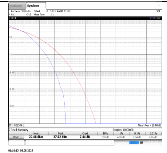
Band25-15MHz-16QAM-26365-75RB#0-PASS
