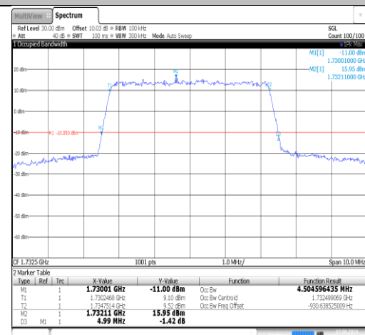
Band4-5MHz-16QAM-20175-25RB#0-PASS
