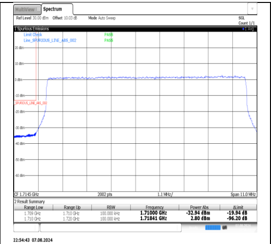
Band4-10MHz-16QAM-20350-1RB#0-PASS
