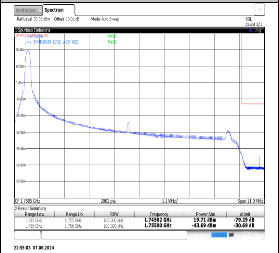
Band4-10MHz-16QAM-20350-1RB#49-PASS
