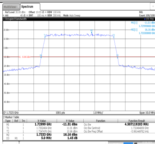
Band4-5MHz-QPSK-20175-25RB#0-PASS
