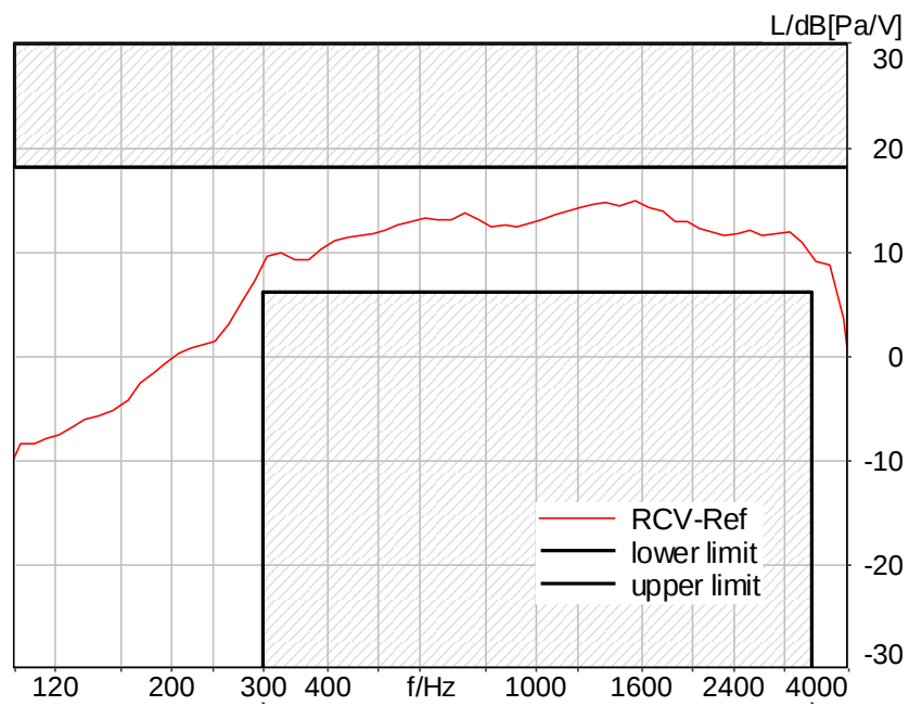
Figure C.4-3 – WLAN 2.4GHz 8N FF Narrowband Frequency Response
