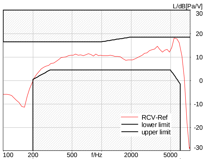
Figure C.3-78 – LTE Band 66 2N DF Wideband Frequency Response
