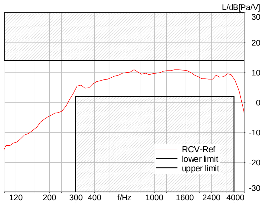
Figure C.3-73 – LTE Band 66 2N FF Narrowband Frequency Response
