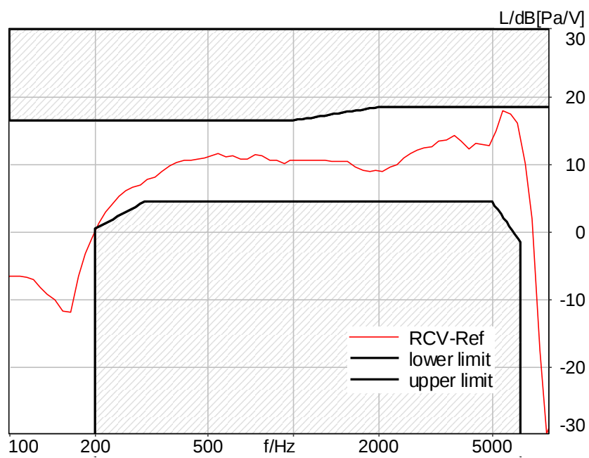
Figure C.4-6 – WLAN 2.4GHz 2N DF Wideband Frequency Response
