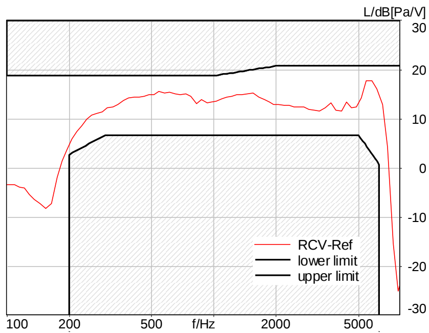
Figure C.3-55 – LTE Band 25 8N FF Wideband Frequency Response
