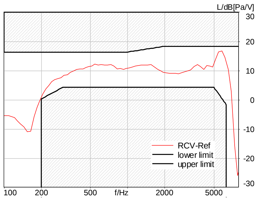
Figure C.3-69 – LTE Band 41 2N FF Wideband Frequency Response
