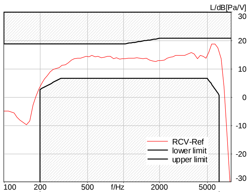
Figure C.3-80 – LTE Band 66 8N DF Wideband Frequency Response
