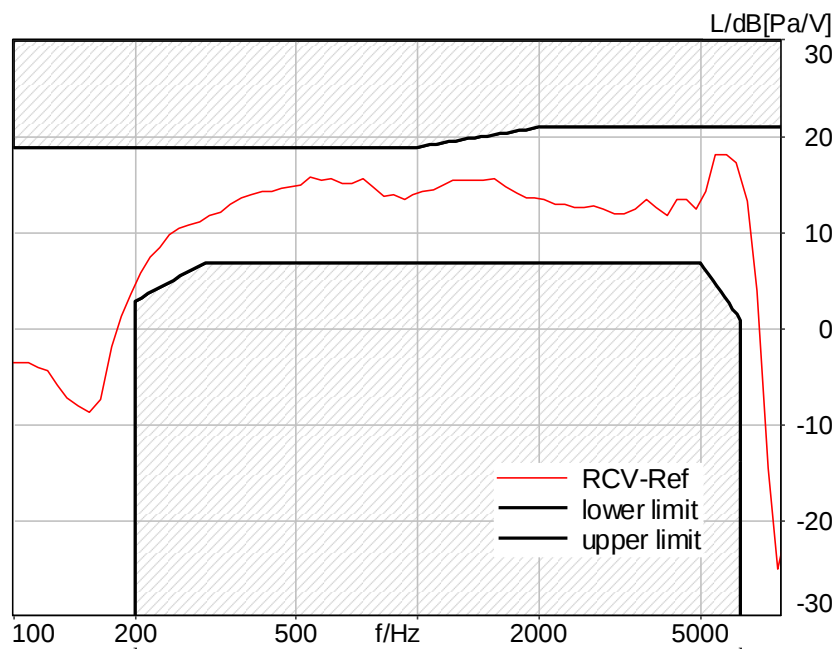
Figure C.3-71 – LTE Band 41 8N FF Wideband Frequency Response
