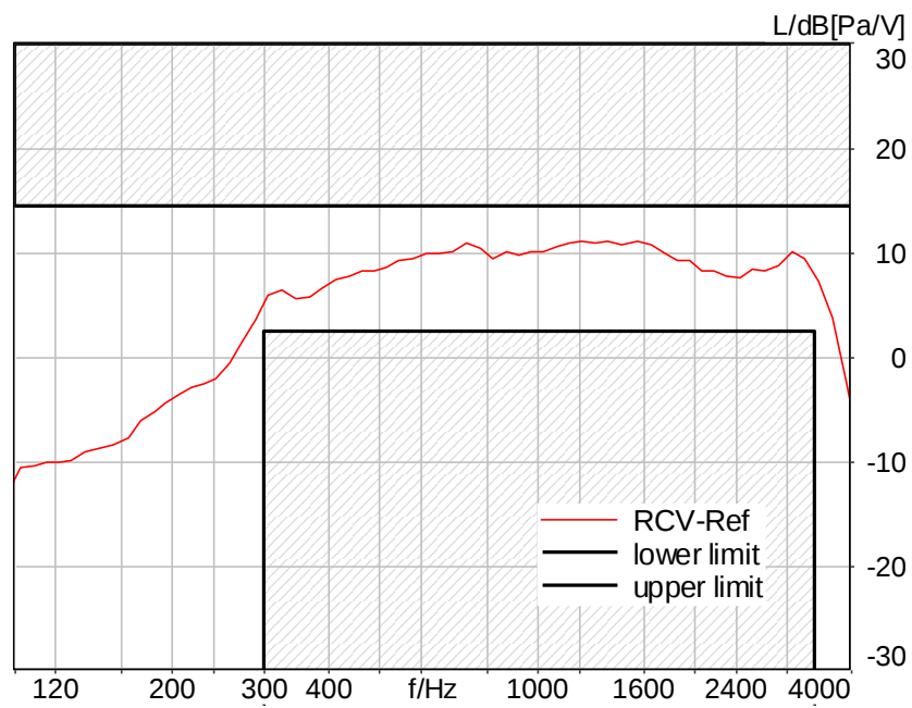
Figure C.3-65 – LTE Band 41 2N FF Narrowband Frequency Response
