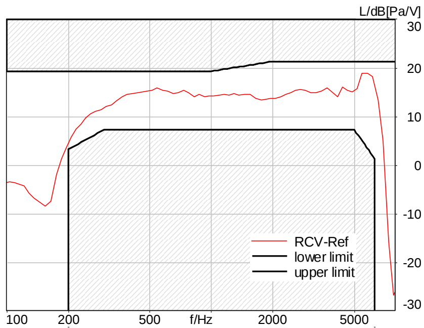
Figure C.3-64 – LTE Band 26 8N DF Wideband Frequency Response
