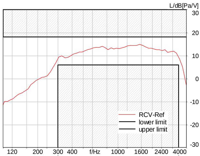
Figure C.3-75 – LTE Band 66 8N FF Narrowband Frequency Response
