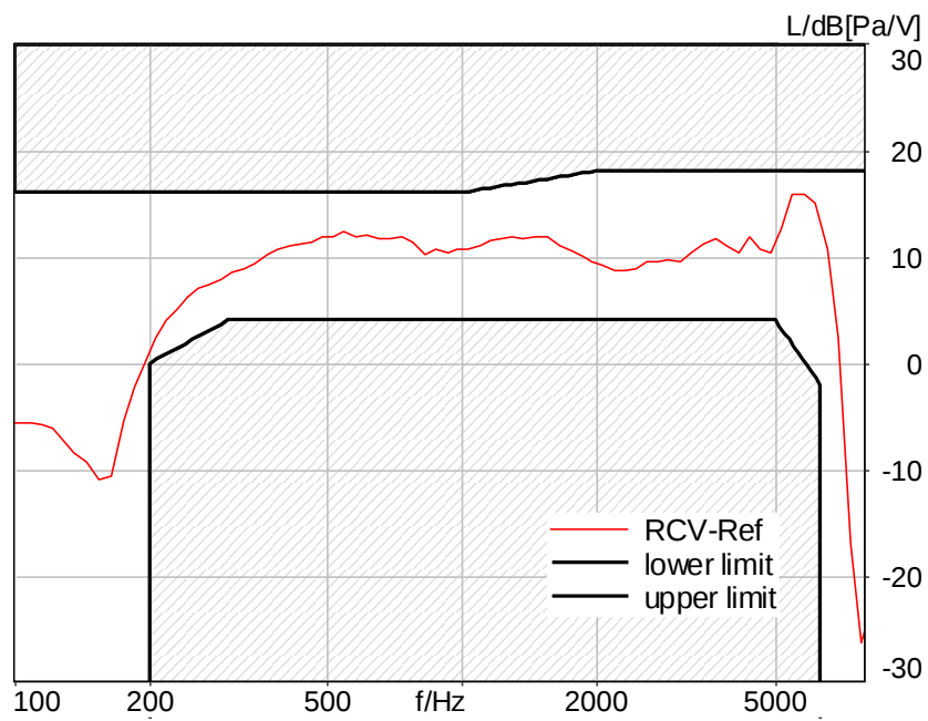
Figure C.3-53 – LTE Band 25 2N FF Wideband Frequency Response
