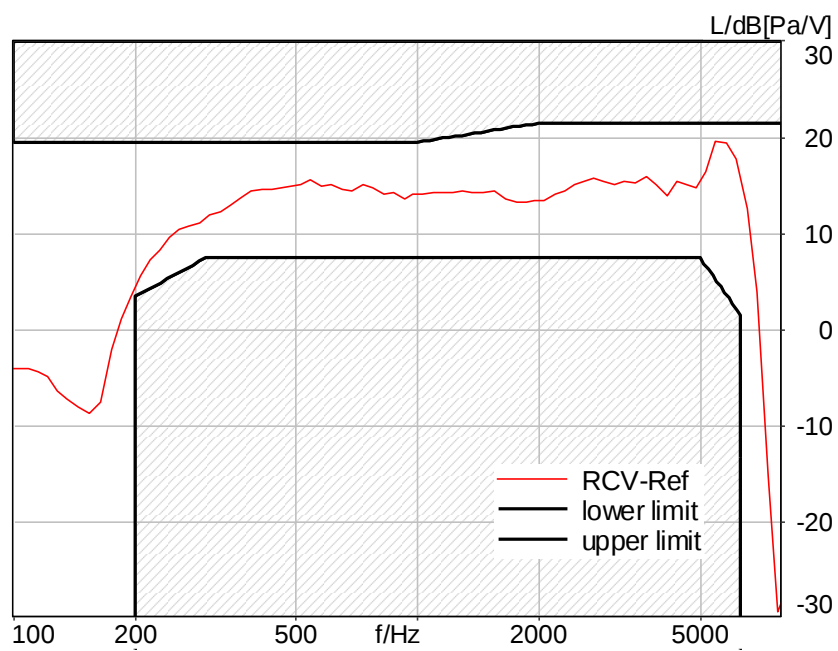
Figure C.4-8 – WLAN 2.4GHz 8N DF Wideband Frequency Response
