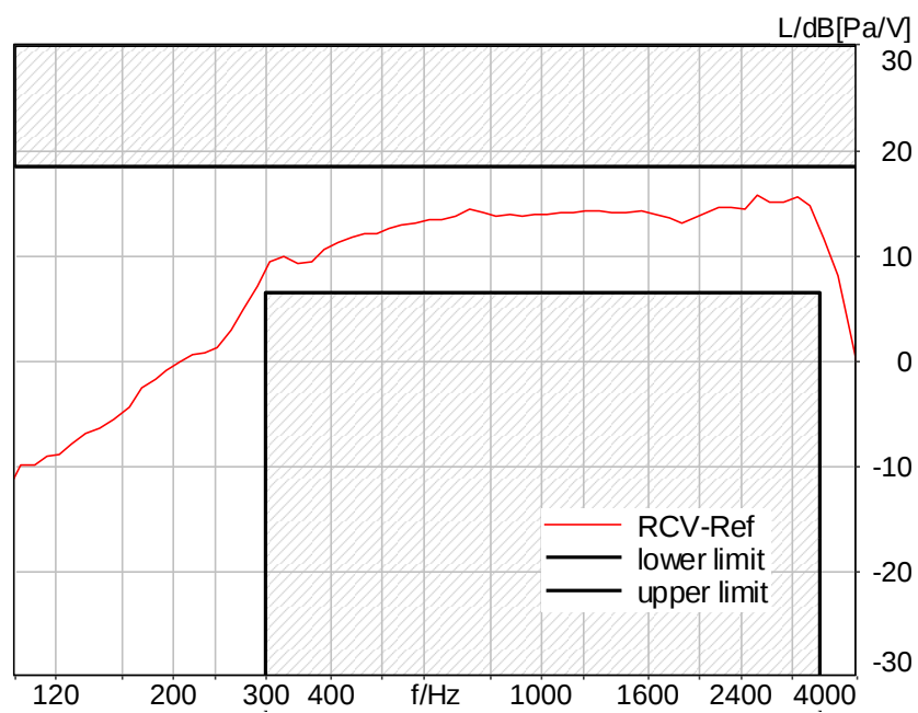
Figure C.3-60 – LTE Band 26 8N DF Narrowband Frequency Response
