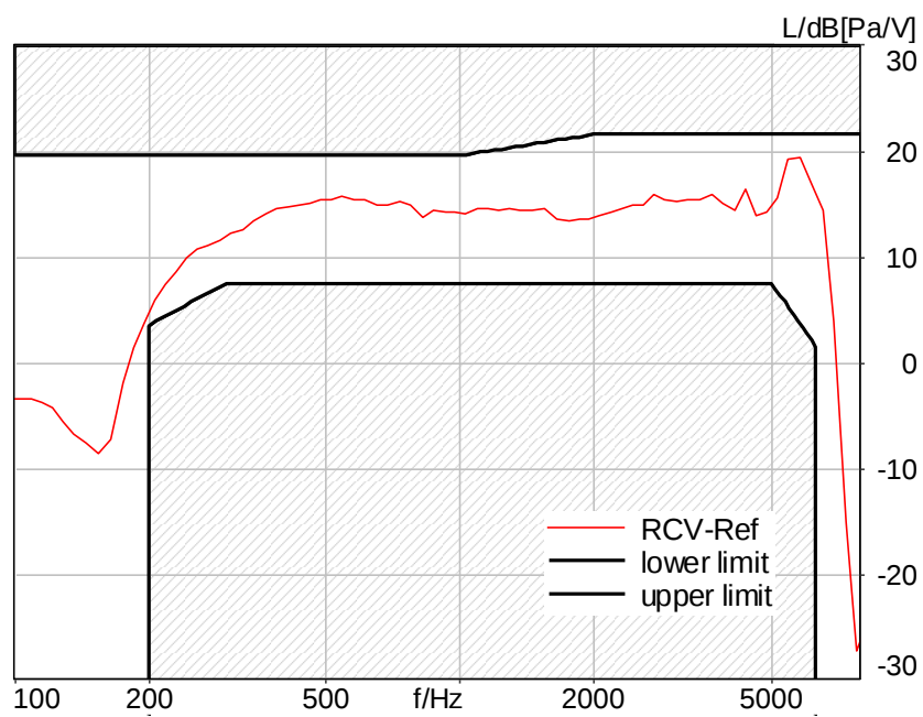
Figure C.3-56 – LTE Band 25 8N DF Wideband Frequency Response
