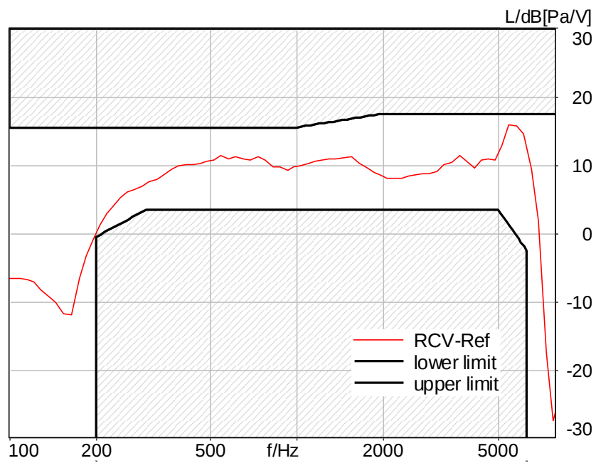
Figure C.4-5 – WLAN 2.4GHz 2N FF Wideband Frequency Response
