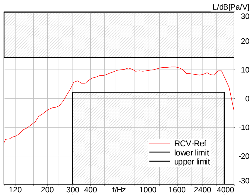
Figure C.3-49 – LTE Band 25 2N FF Narrowband Frequency Response
