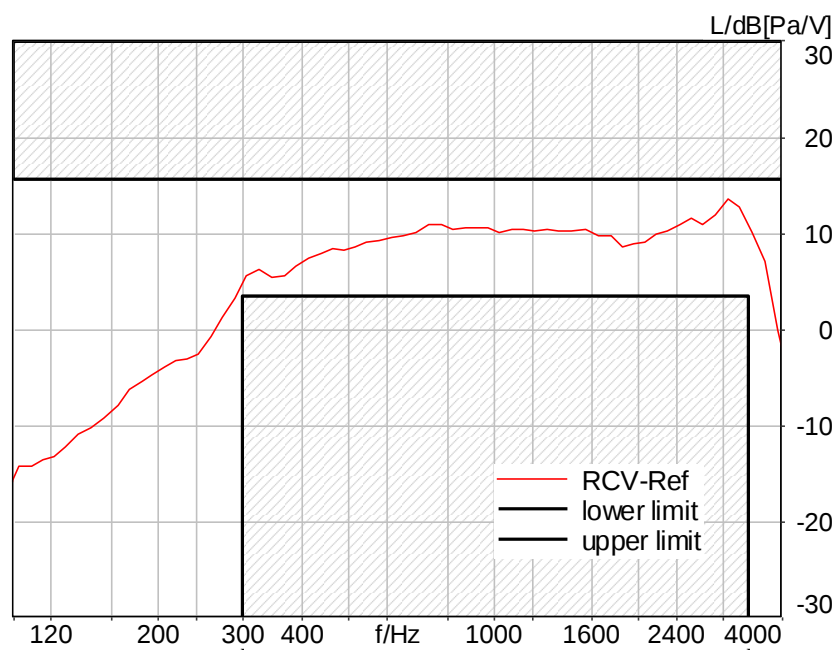
Figure C.3-50 – LTE Band 25 2N DF Narrowband Frequency Response
