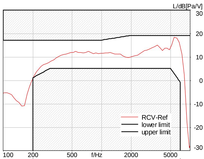
Figure C.3-70 – LTE Band 41 2N DF Wideband Frequency Response
