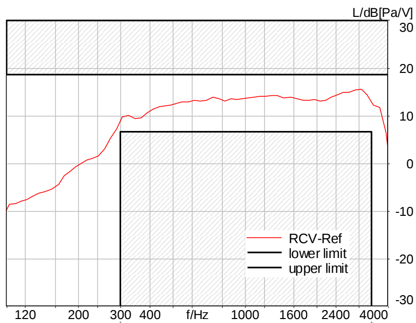
Figure C.4-4 – WLAN 2.4GHz 8N DF Narrowband Frequency Response
