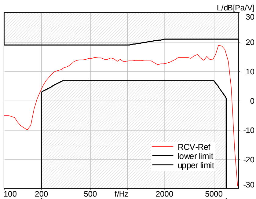
Figure C.3-88 – LTE Band 71 8N DF Wideband Frequency Response
