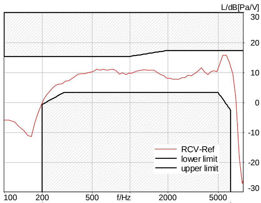
Figure C.3-77 – LTE Band 66 2N FF Wideband Frequency Response
