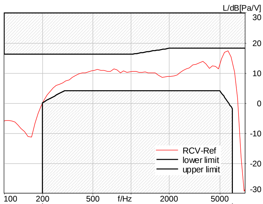
Figure C.3-86 – LTE Band 71 2N DF Wideband Frequency Response
