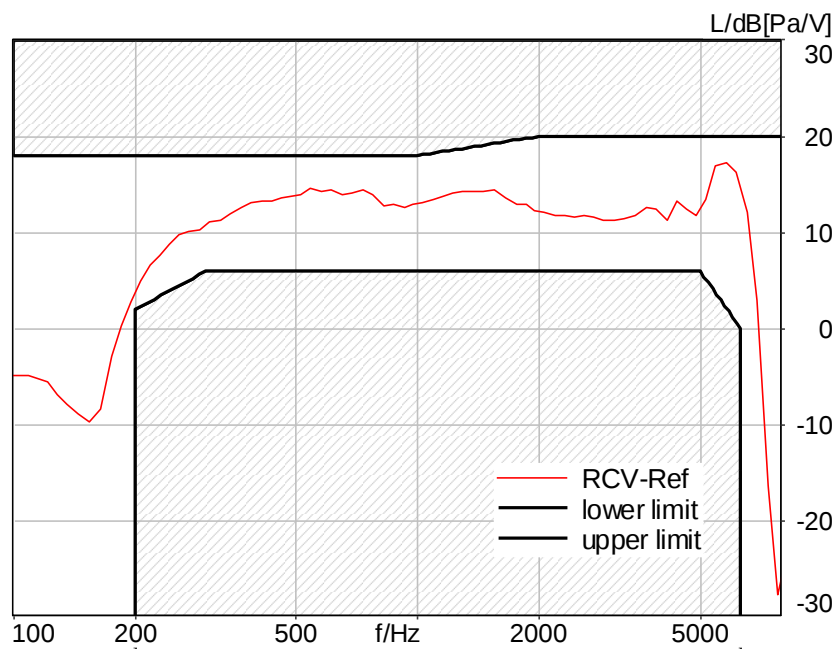
Figure C.3-79 – LTE Band 66 8N FF Wideband Frequency Response
