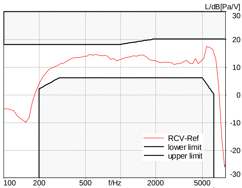
Figure C.3-87 – LTE Band 71 8N FF Wideband Frequency Response
