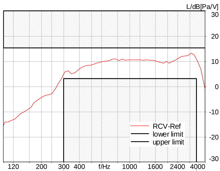
Figure C.3-82 – LTE Band 71 2N DF Narrowband Frequency Response
