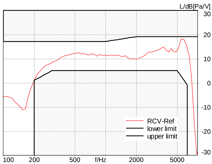
Figure C.3-62 – LTE Band 26 2N DF Wideband Frequency Response
