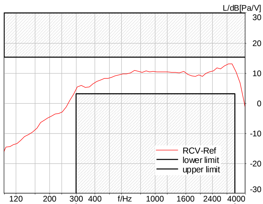
Figure C.3-58 – LTE Band 26 2N DF Narrowband Frequency Response
