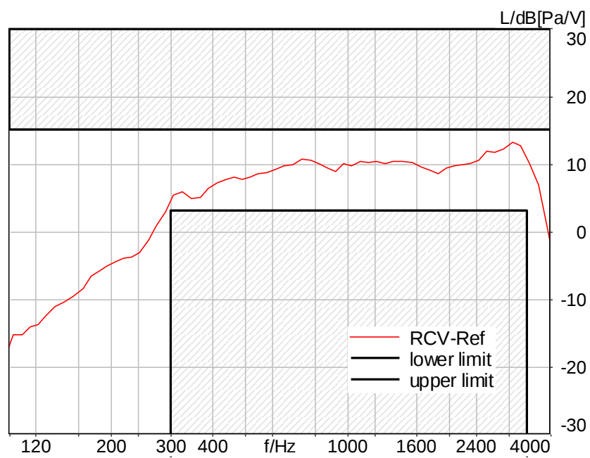
Figure C.3-74 – LTE Band 66 2N DF Narrowband Frequency Response
