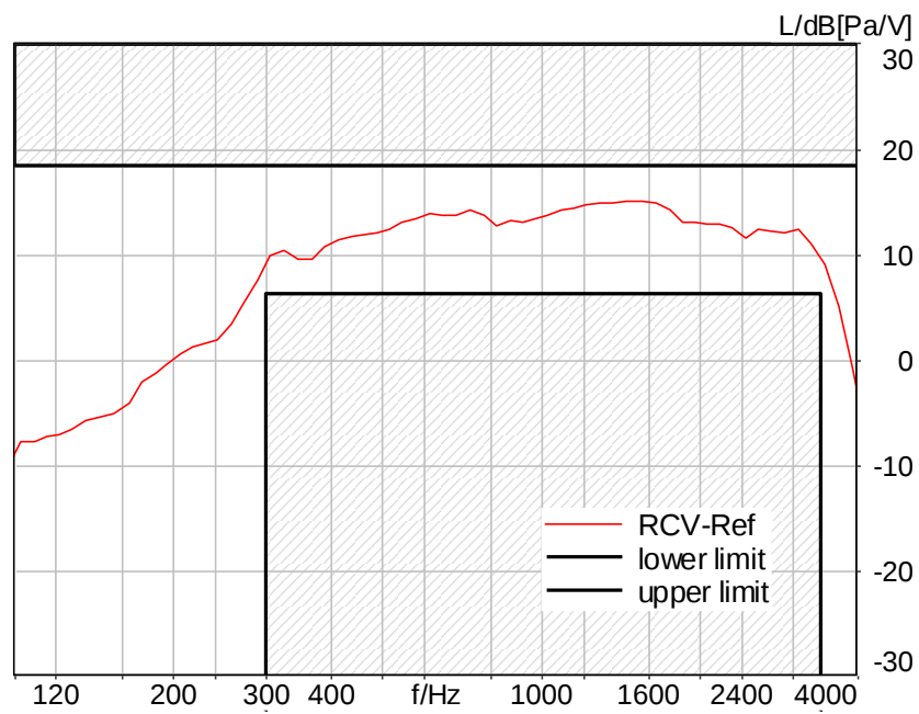
Figure C.3-67 – LTE Band 41 8N FF Narrowband Frequency Response
