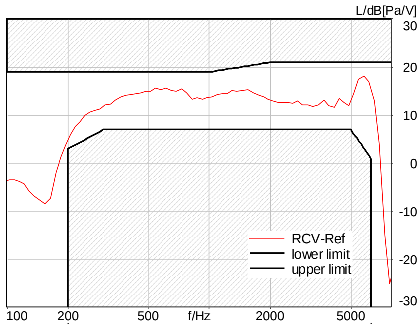
Figure C.3-63 – LTE Band 26 8N FF Wideband Frequency Response
