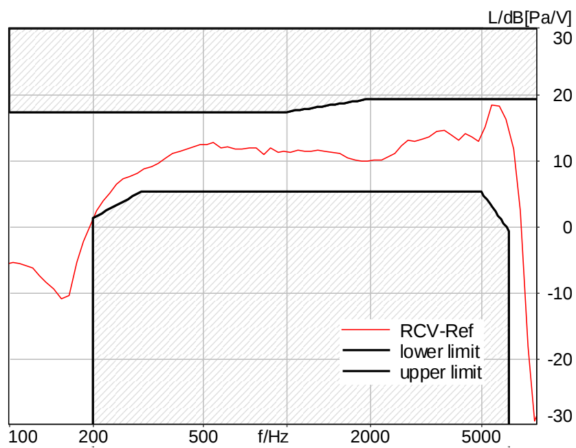
Figure C.3-54 – LTE Band 25 2N DF Wideband Frequency Response
