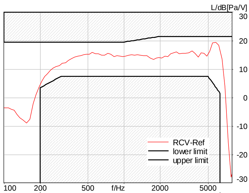
Figure C.3-72 – LTE Band 41 8N DF Wideband Frequency Response
