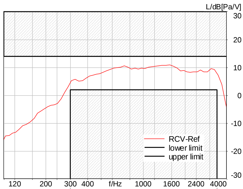
Figure C.3-57 – LTE Band 26 2N FF Narrowband Frequency Response
