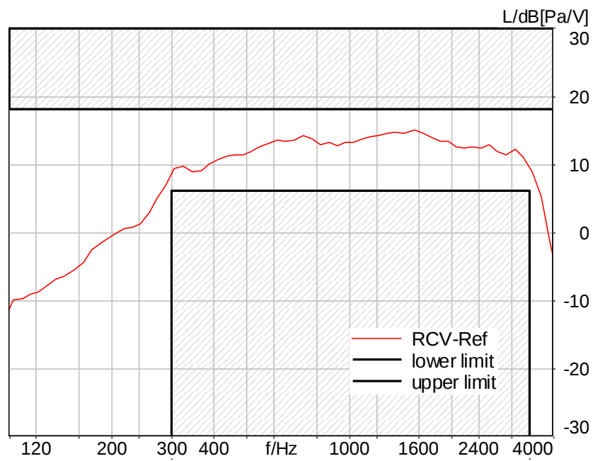
Figure C.3-59 – LTE Band 26 8N FF Narrowband Frequency Response
