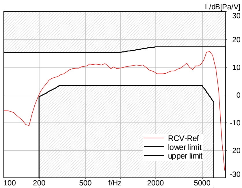
Figure C.3-85 – LTE Band 71 2N FF Wideband Frequency Response
