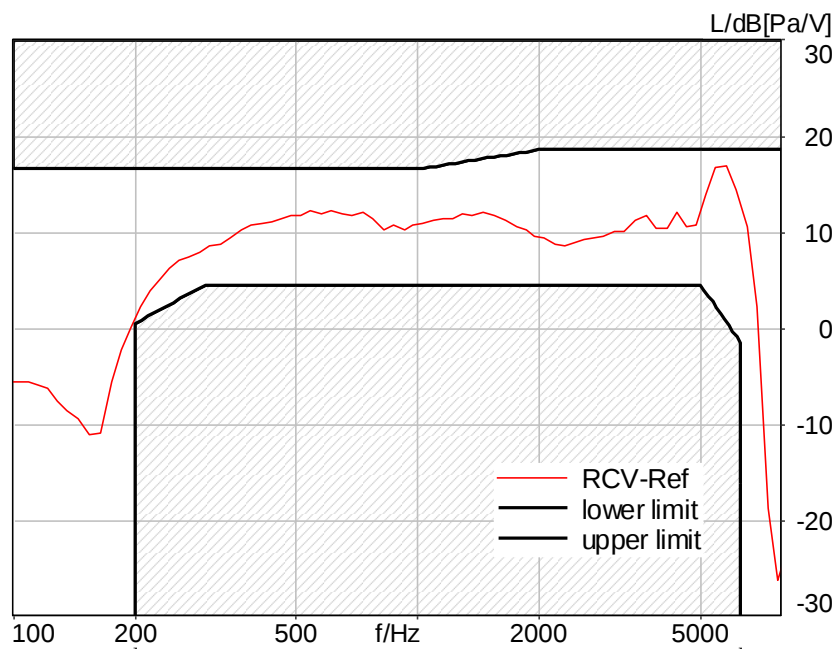
Figure C.3-61 – LTE Band 26 2N FF Wideband Frequency Response
