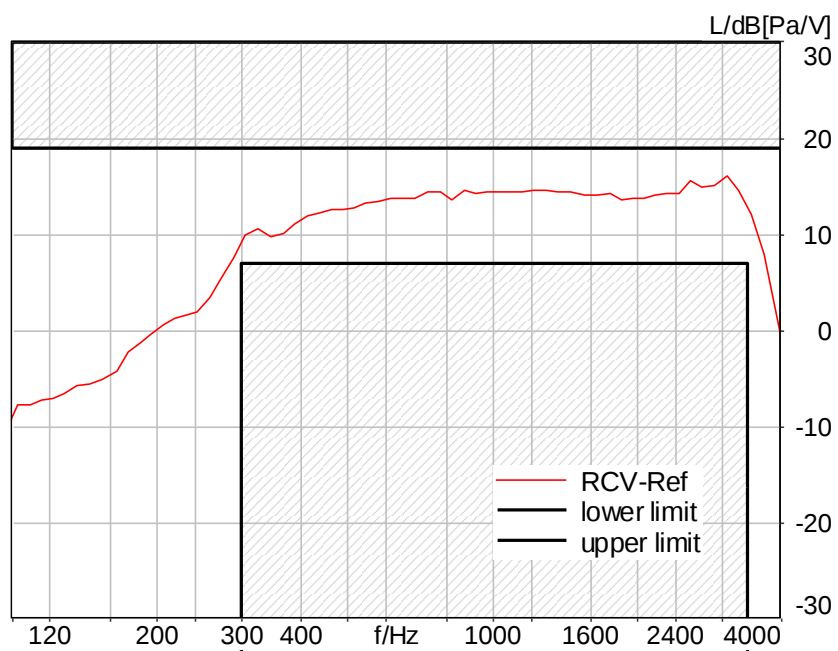
Figure C.3-68 – LTE Band 41 8N DF Narrowband Frequency Response
