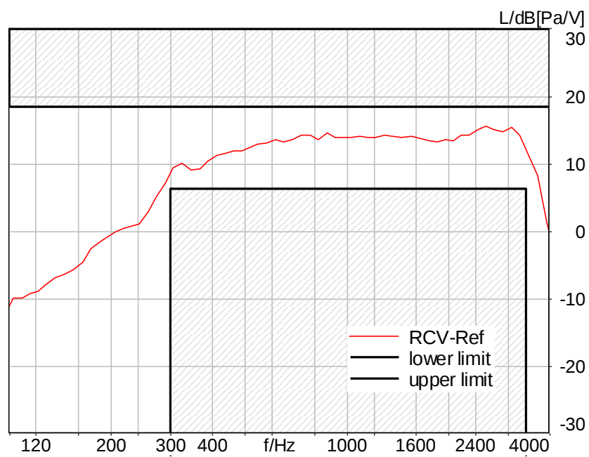
Figure C.3-84 – LTE Band 71 8N DF Narrowband Frequency Response
