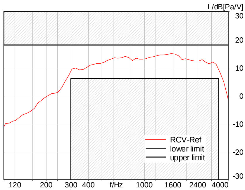
Figure C.3-51 – LTE Band 25 8N FF Narrowband Frequency Response
