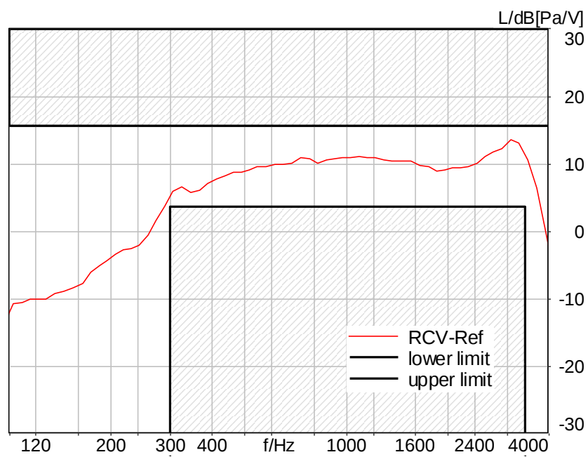
Figure C.3-66 – LTE Band 41 2N DF Narrowband Frequency Response
