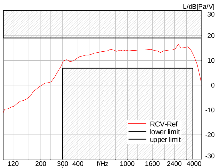
Figure C.3-52 – LTE Band 25 8N DF Narrowband Frequency Response
