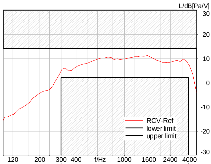
Figure C.3-81 – LTE Band 71 2N FF Narrowband Frequency Response
