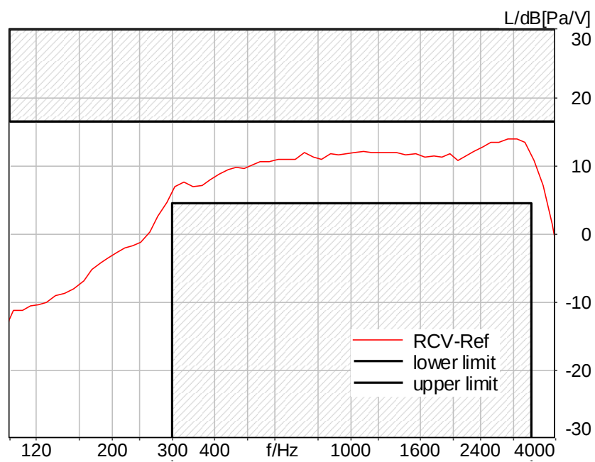
Figure C.2-4 – WCDMA Band II 8N Narrowband DF Frequency Response
