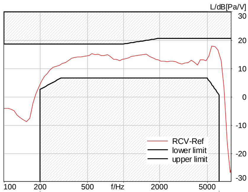
Figure C.4-7 – WLAN 2.4GHz 8N FF Wideband Frequency Response
