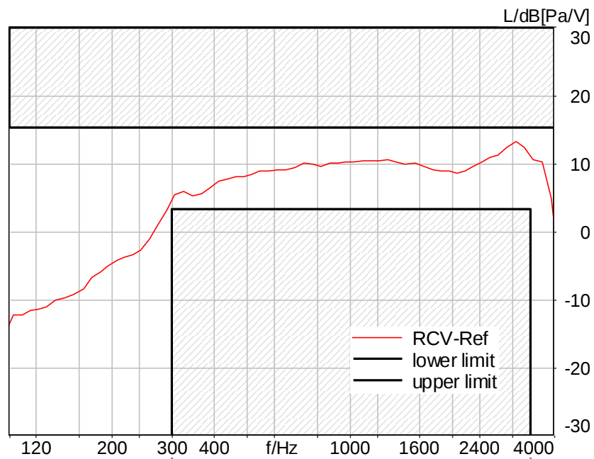
Figure C.4-2 – WLAN 2.4GHz 2N DF Narrowband Frequency Response
