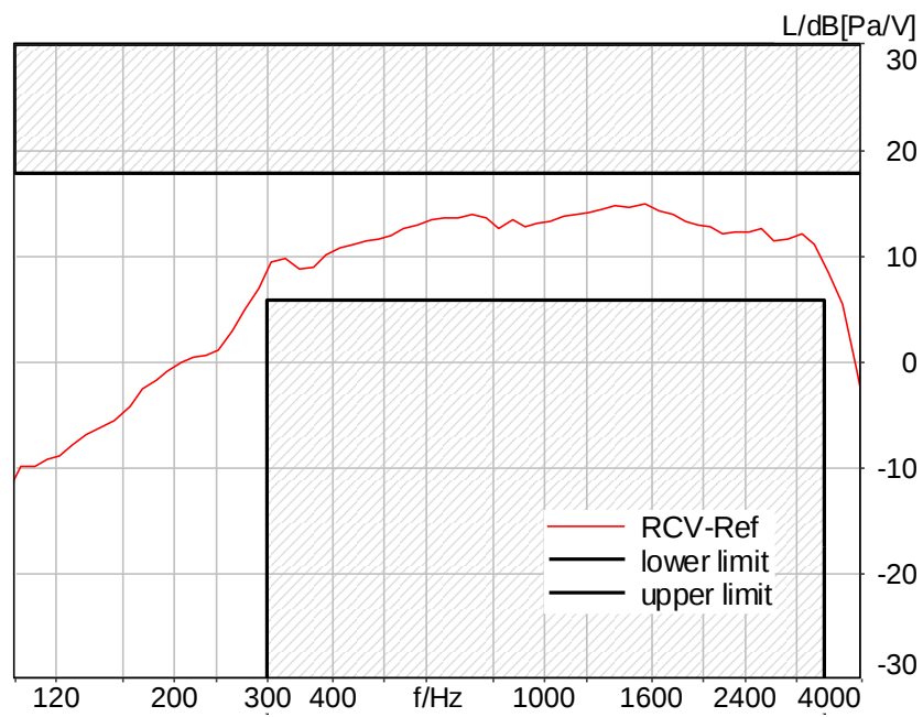
Figure C.3-83 – LTE Band 71 8N FF Narrowband Frequency Response
