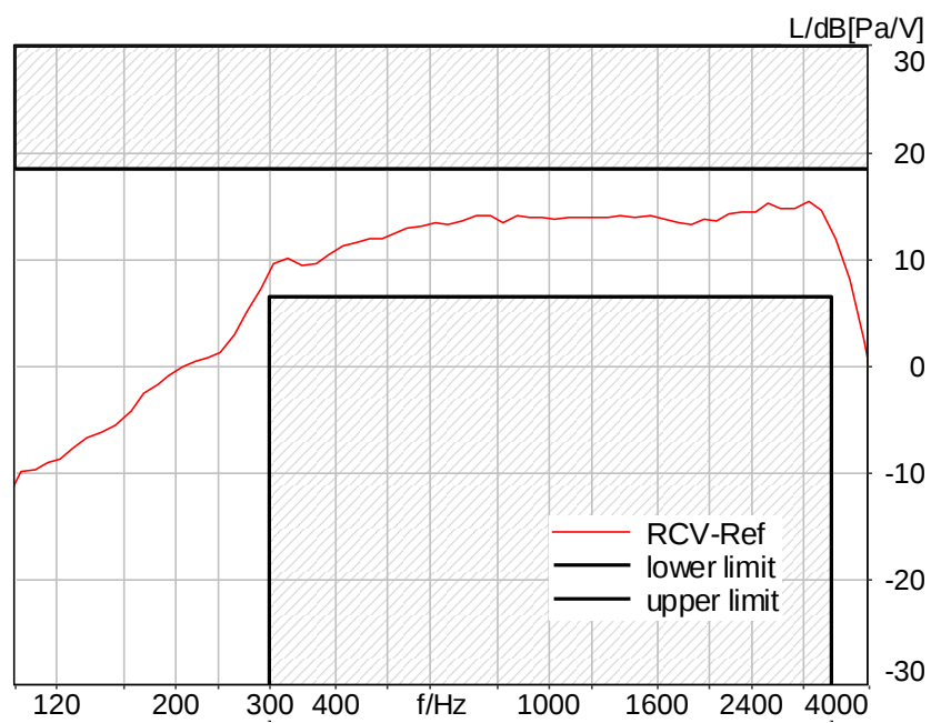
Figure C.3-76 – LTE Band 66 8N DF Narrowband Frequency Response
