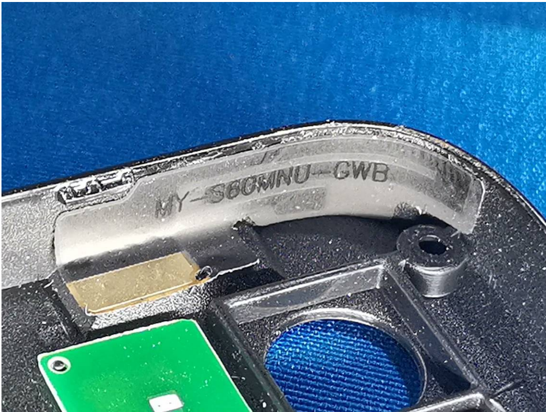
Bluetooth/Wi-Fi Antenna
