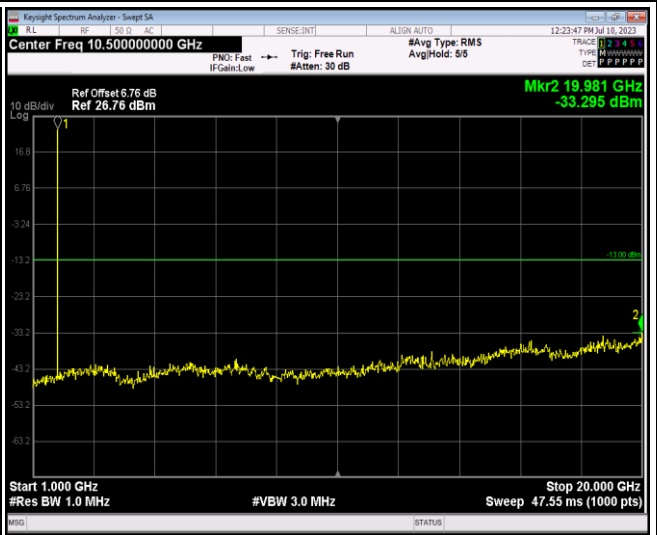
Band66-1.4MHz-16QAM-131979-1RB#0-Range2:1000~20000MHz
