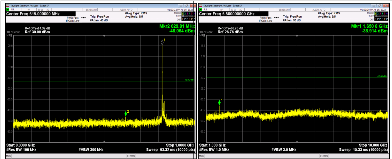
Band26-15MHz-16QAM-26915-1RB#0-Range1:30~1000MHz
