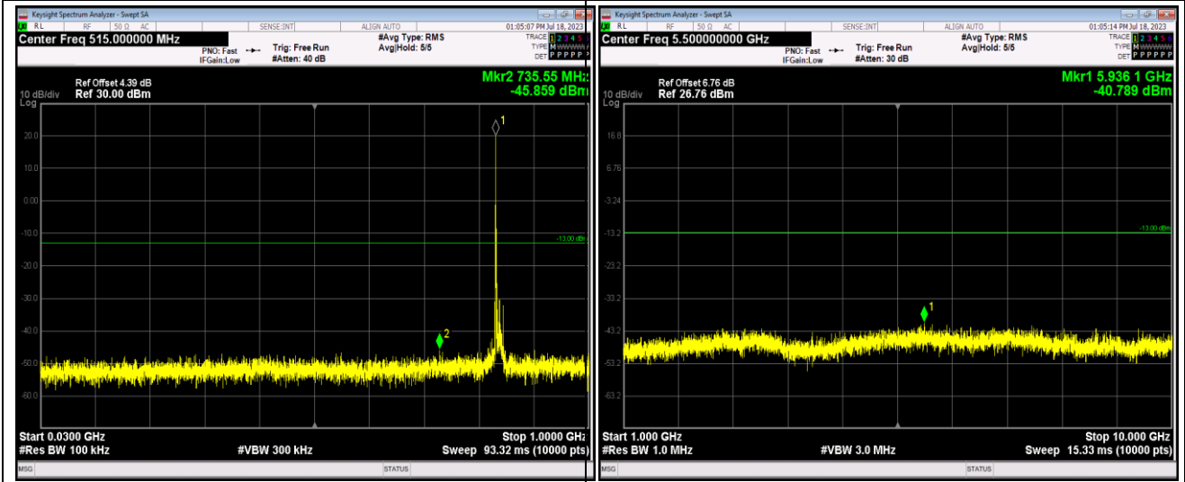
Band26-15MHz-16QAM-26965-1RB#0-Range1:30~1000MHz
