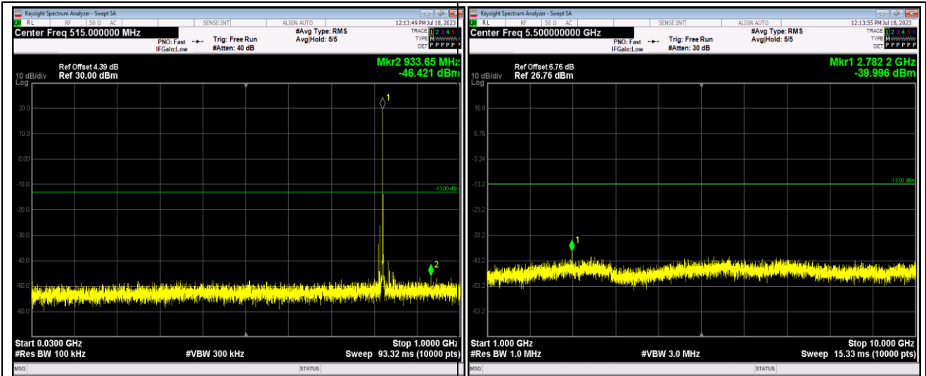
Band26-1.4MHz-16QAM-26915-1RB#0-Range1:30 ~1000MHz
