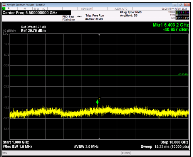
Band26-1.4MHz-QPSK-26740-1RB#0-Range2:1000~10000MHz
